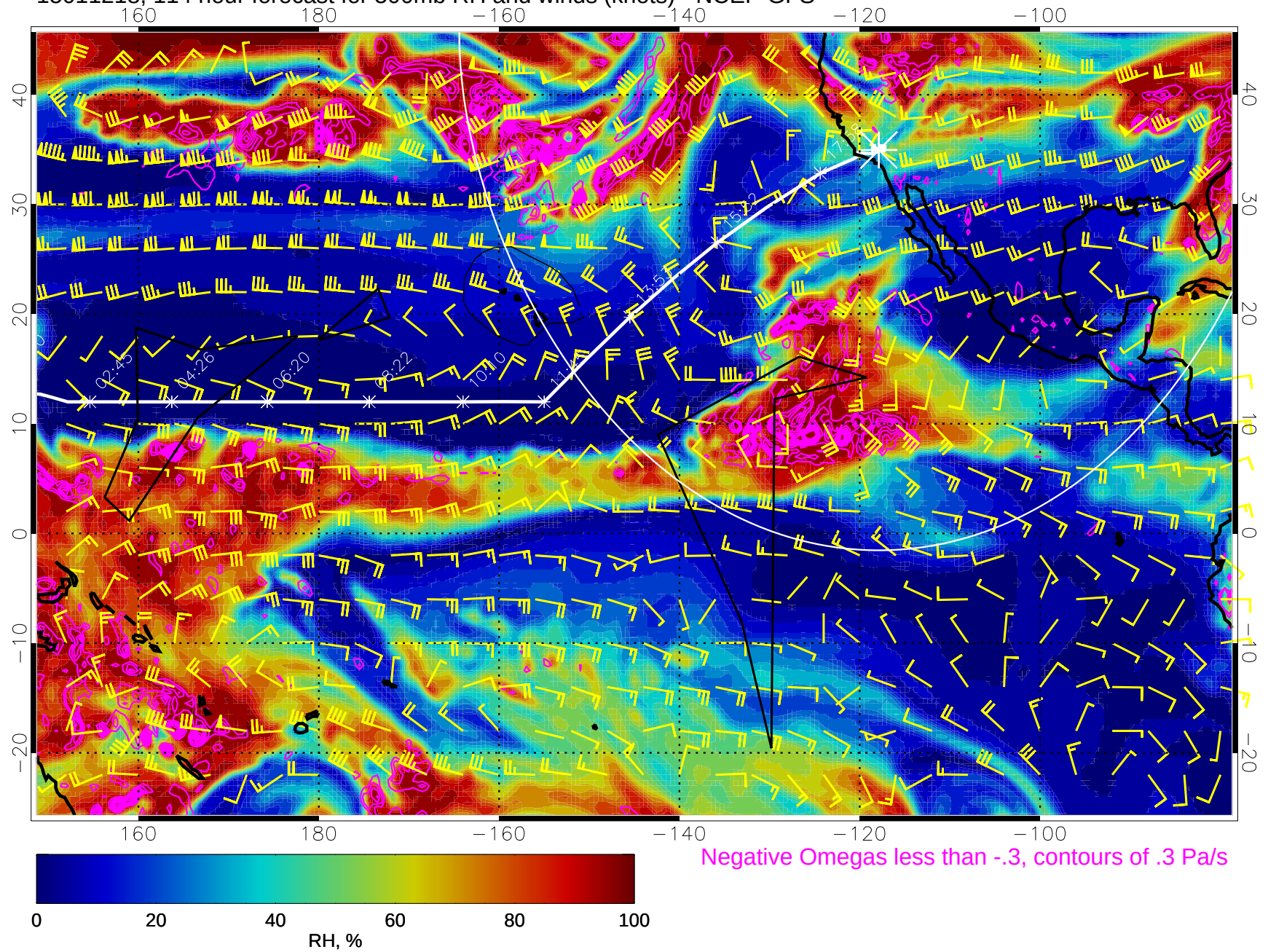
15011218, 114 hour forecast for 500mb RH and winds (knots) - NCEP GFS
