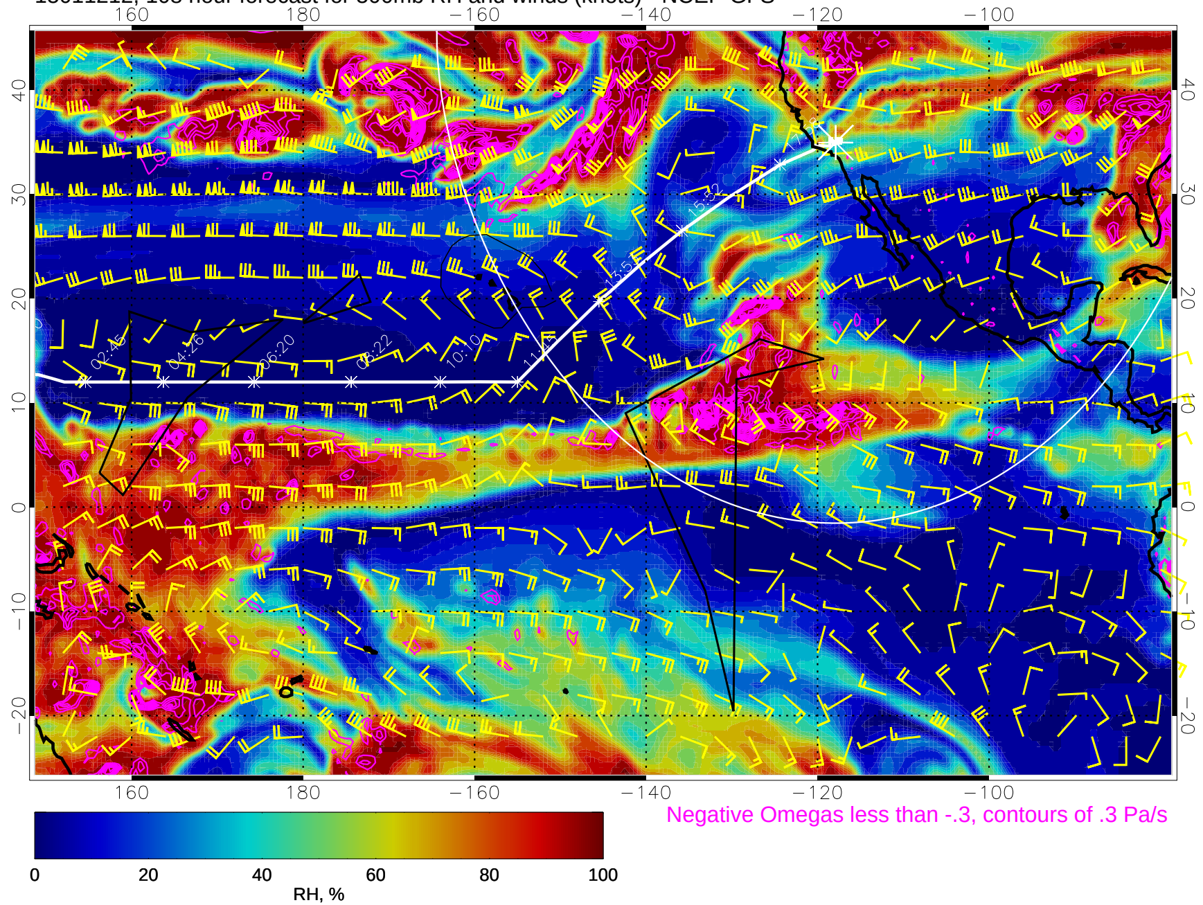
15011212, 108 hour forecast for 500mb RH and winds (knots) - NCEP GFS
