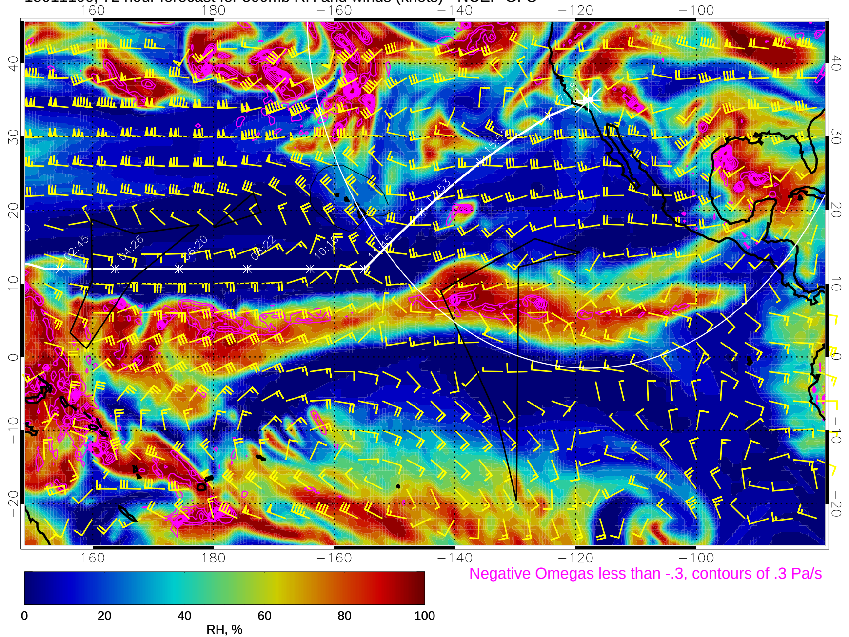
15011100, 72 hour forecast for 500mb RH and winds (knots) - NCEP GFS
