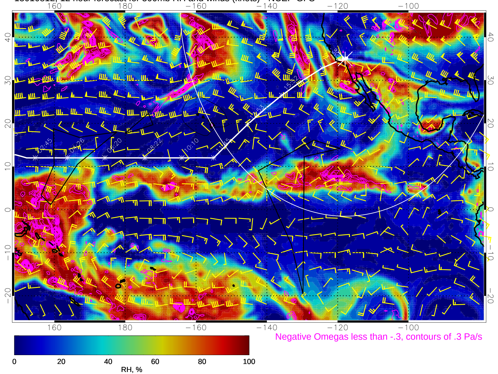
15010812, 12 hour forecast for 500mb RH and winds (knots) - NCEP GFS
