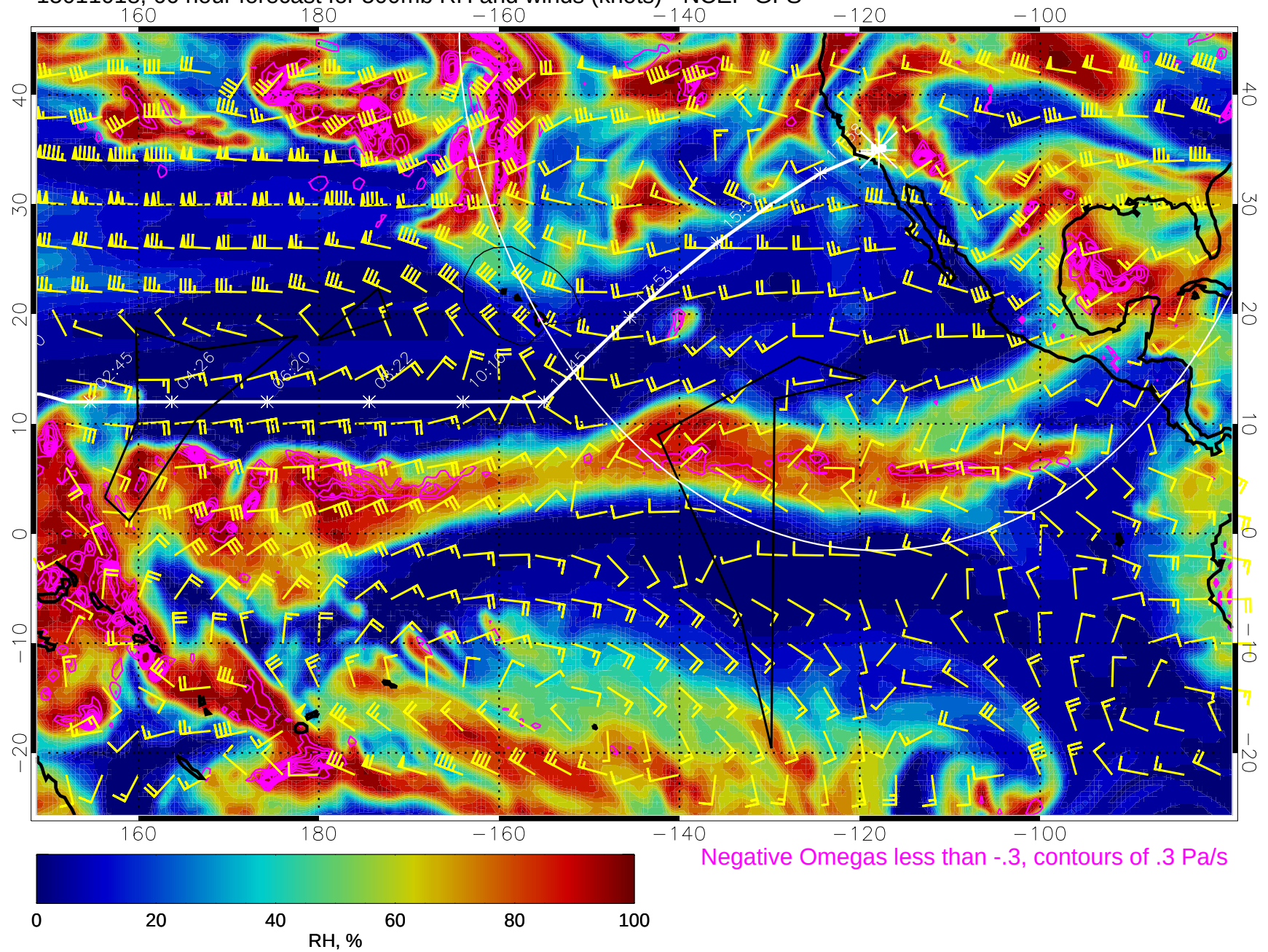
15011018, 66 hour forecast for 500mb RH and winds (knots) - NCEP GFS
