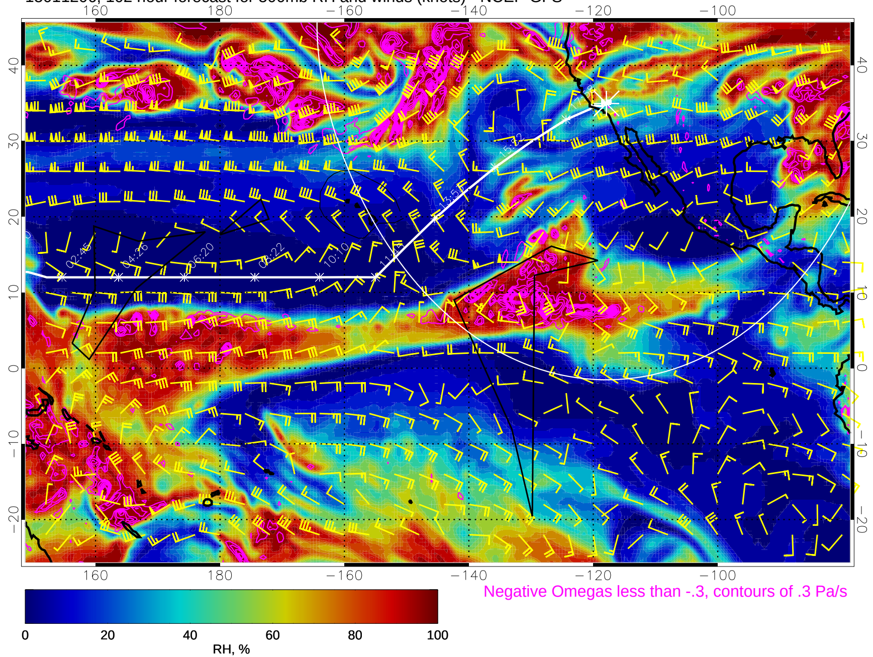
15011206, 102 hour forecast for 500mb RH and winds (knots) - NCEP GFS
