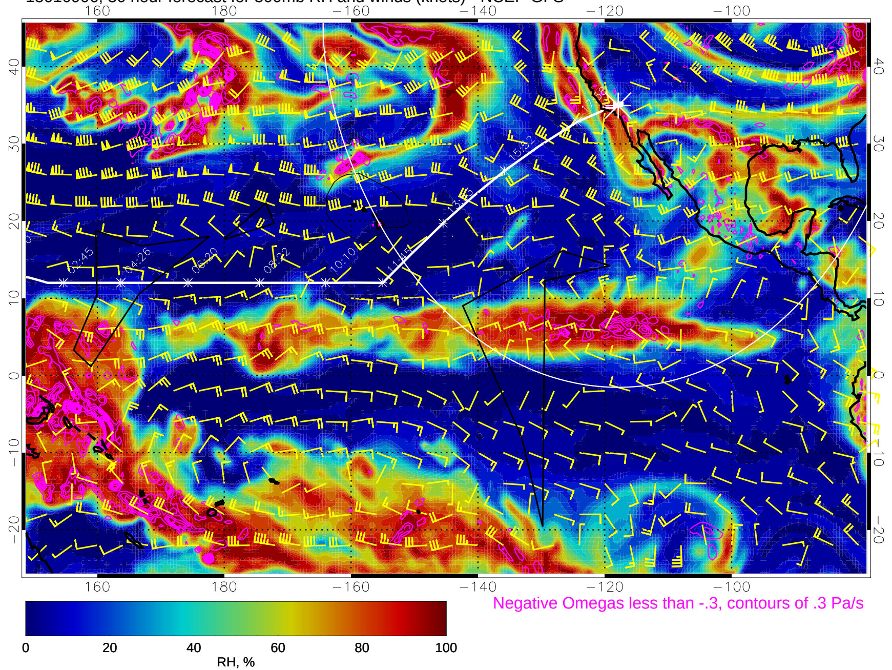
15010906, 30 hour forecast for 500mb RH and winds (knots) - NCEP GFS
