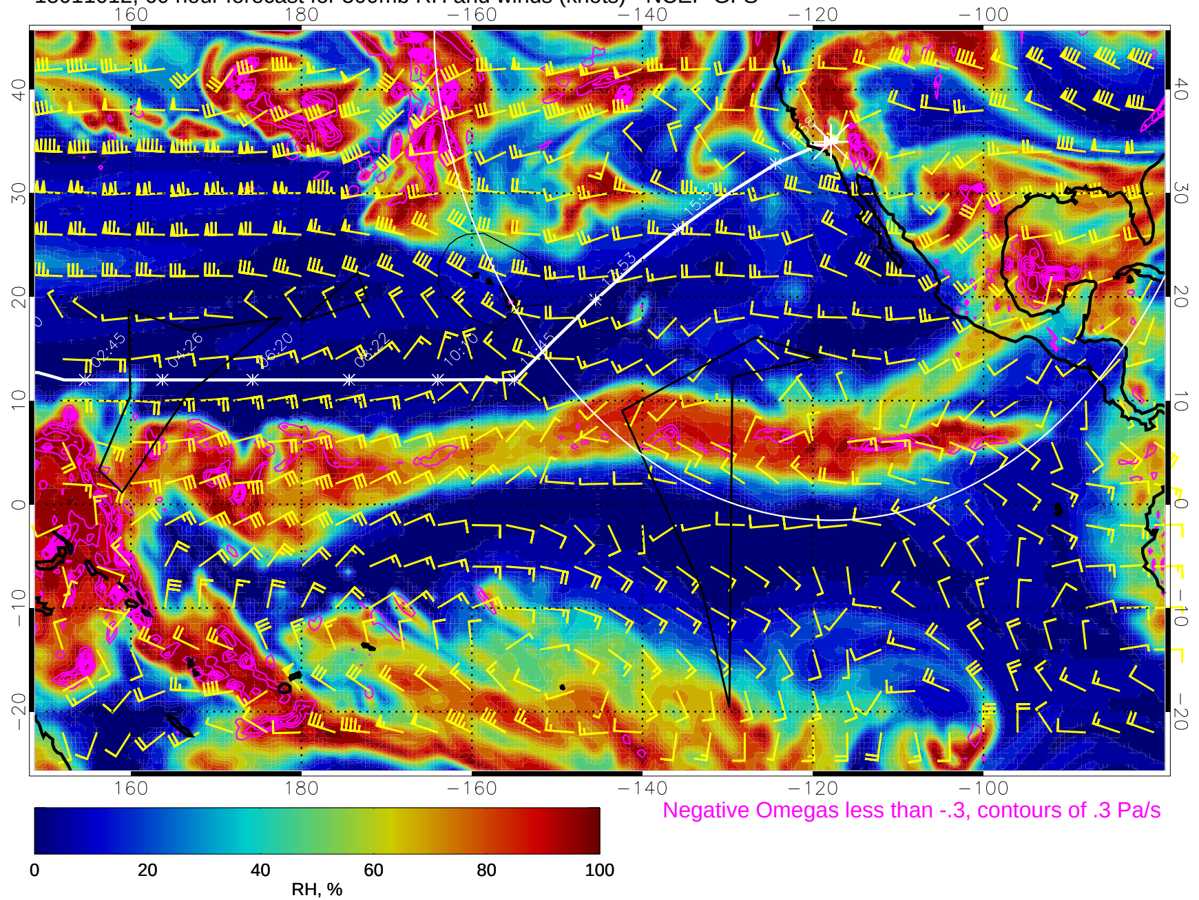
15011012, 60 hour forecast for 500mb RH and winds (knots) - NCEP GFS
