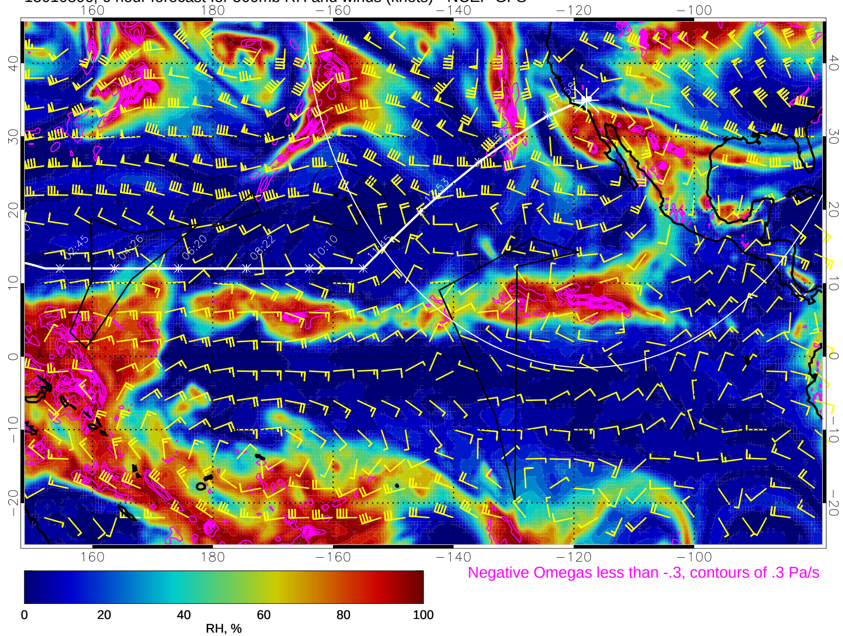
15010806, 6 hour forecast for 500mb RH and winds (knots) - NCEP GFS
