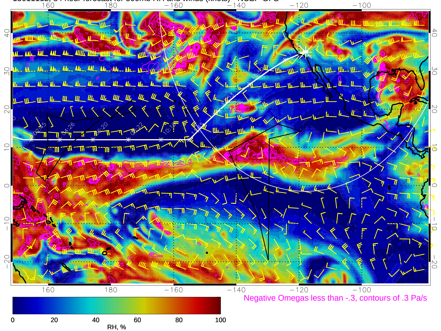
15011112, 84 hour forecast for 500mb RH and winds (knots) - NCEP GFS
