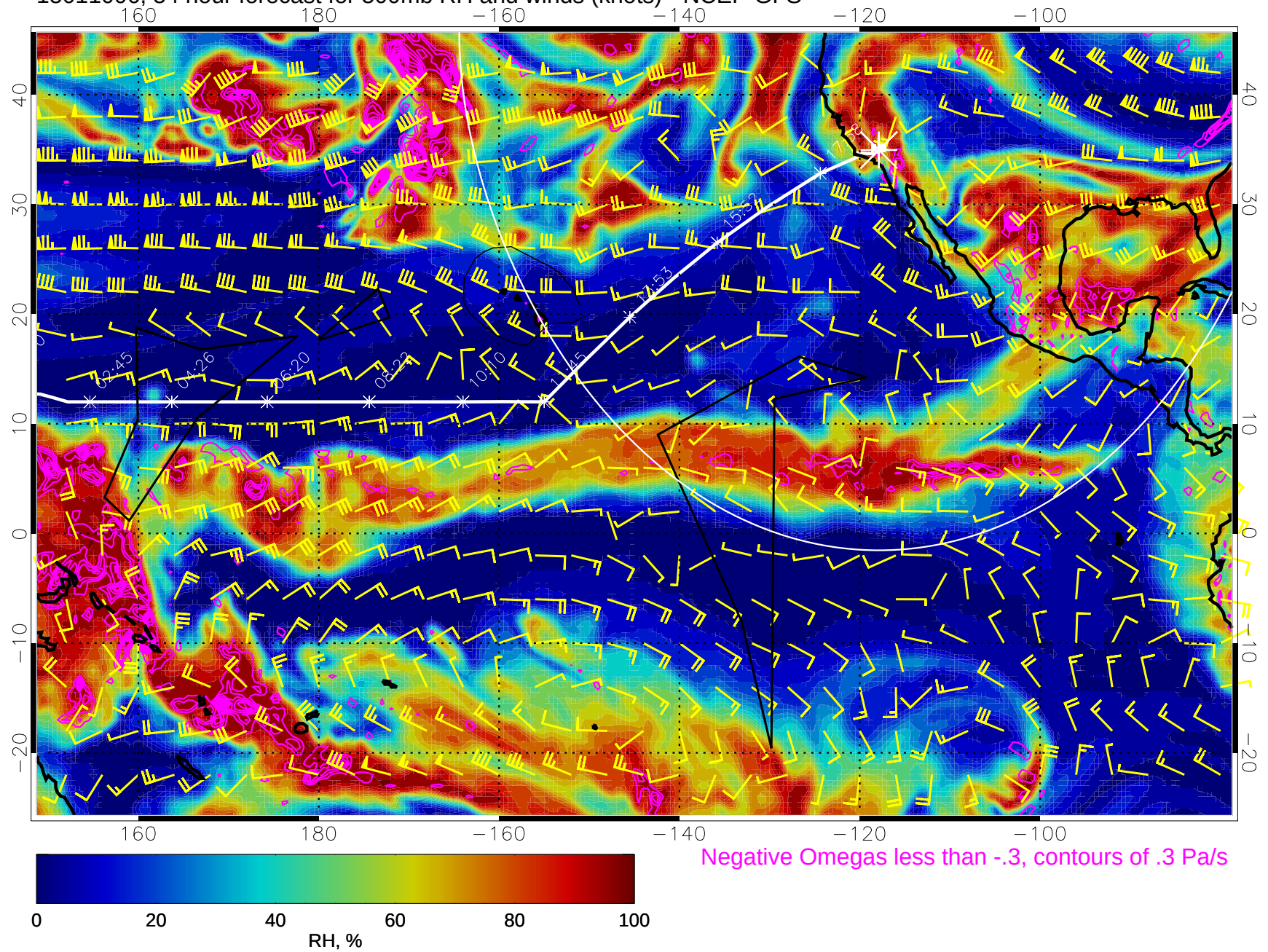
15011006, 54 hour forecast for 500mb RH and winds (knots) - NCEP GFS
