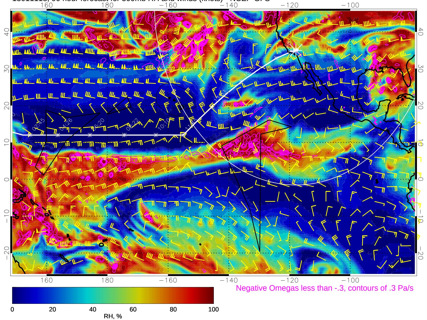
15011118, 90 hour forecast for 500mb RH and winds (knots) - NCEP GFS
