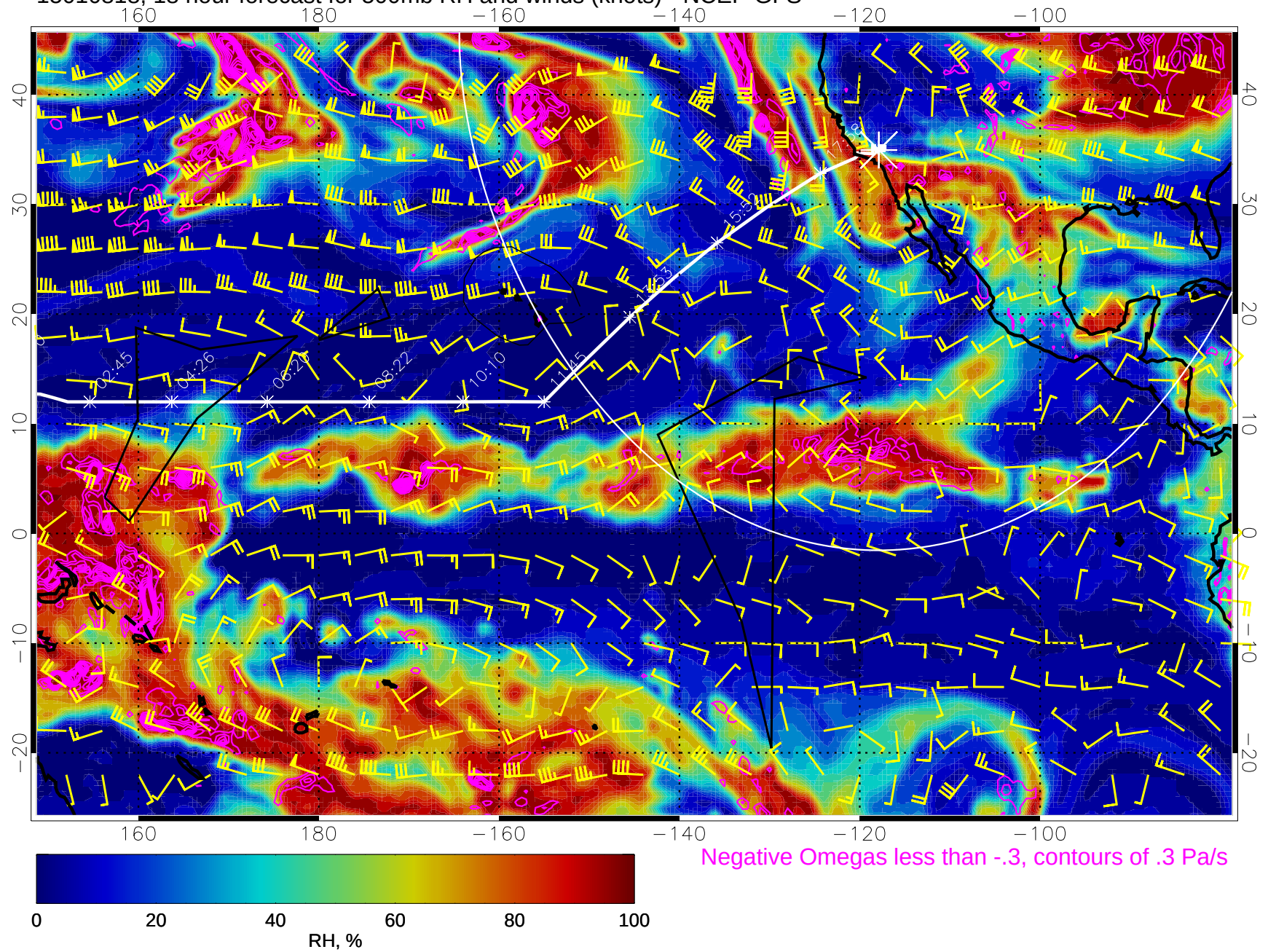
15010818, 18 hour forecast for 500mb RH and winds (knots) - NCEP GFS
