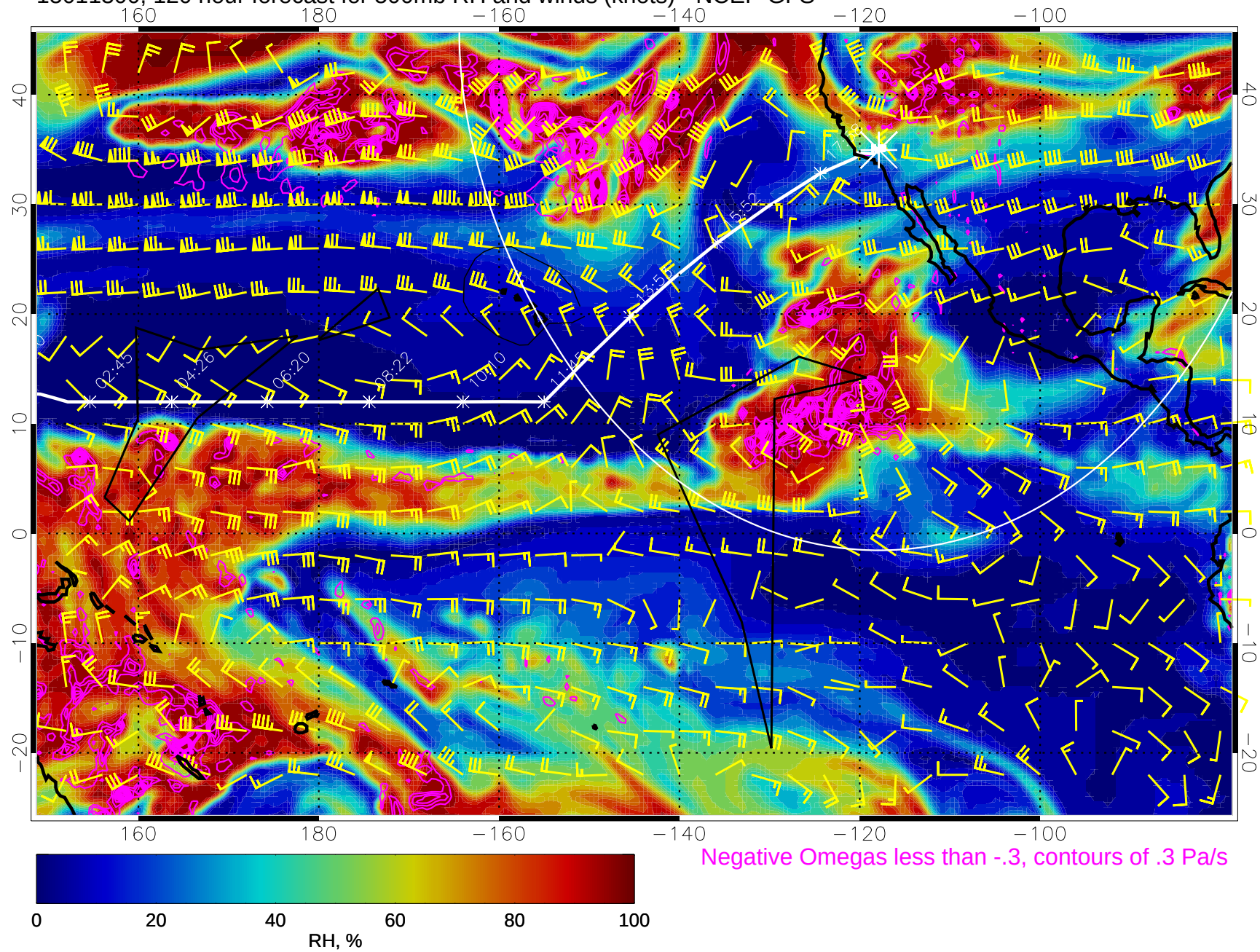
15011300, 120 hour forecast for 500mb RH and winds (knots) - NCEP GFS
