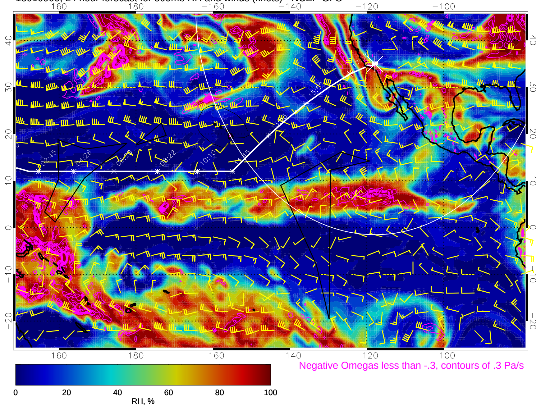
15010900, 24 hour forecast for 500mb RH and winds (knots) - NCEP GFS
