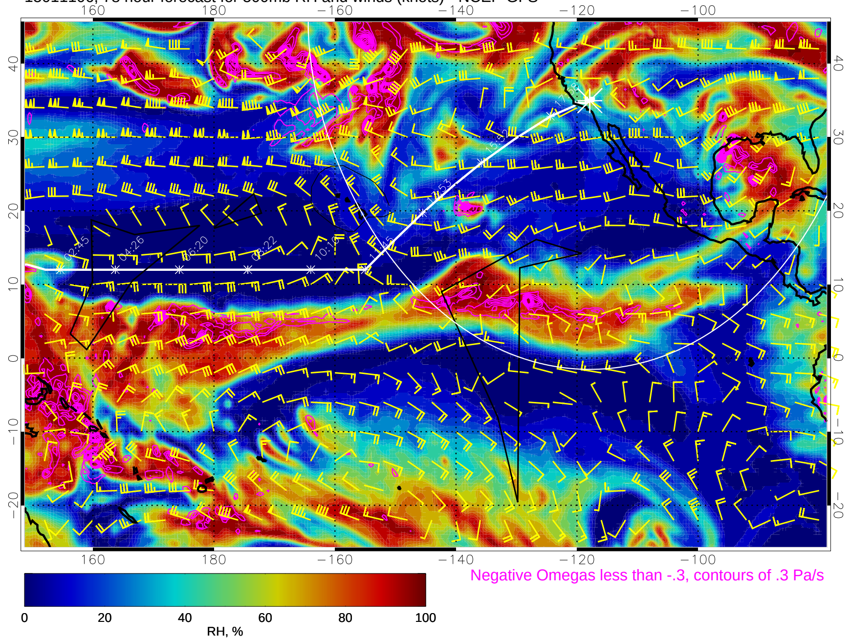
15011106, 78 hour forecast for 500mb RH and winds (knots) - NCEP GFS
