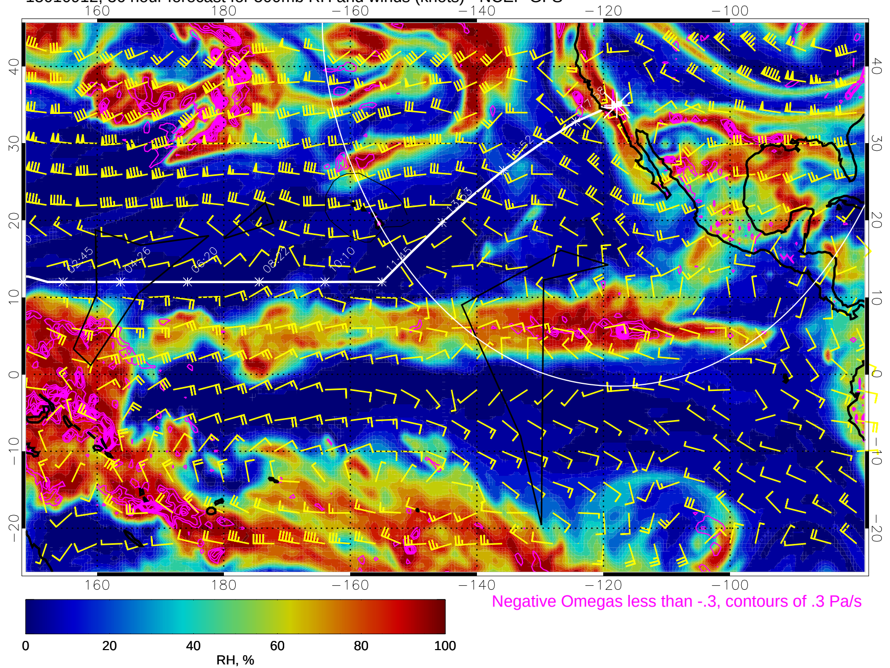
15010912, 36 hour forecast for 500mb RH and winds (knots) - NCEP GFS
