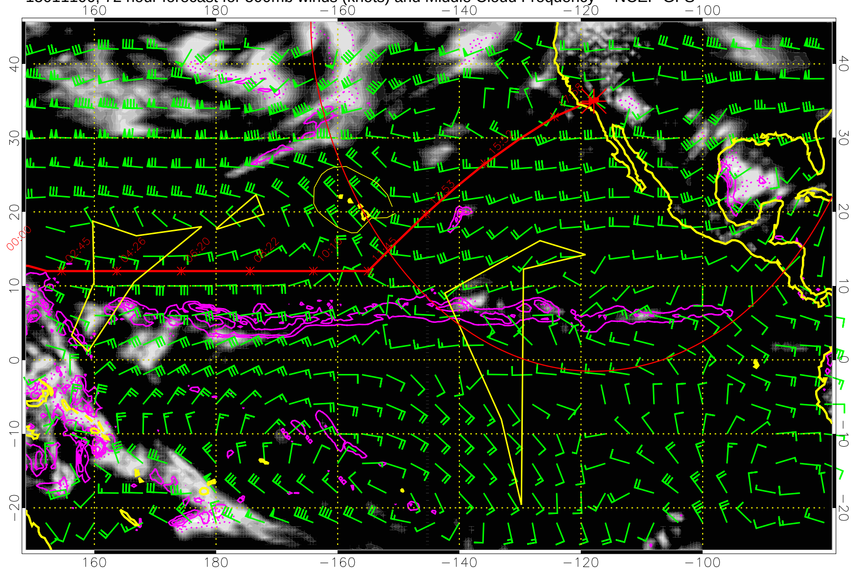
15011100, 72 hour forecast for 500mb winds (knots) and Middle Cloud Frequency -- NCEP GFS
