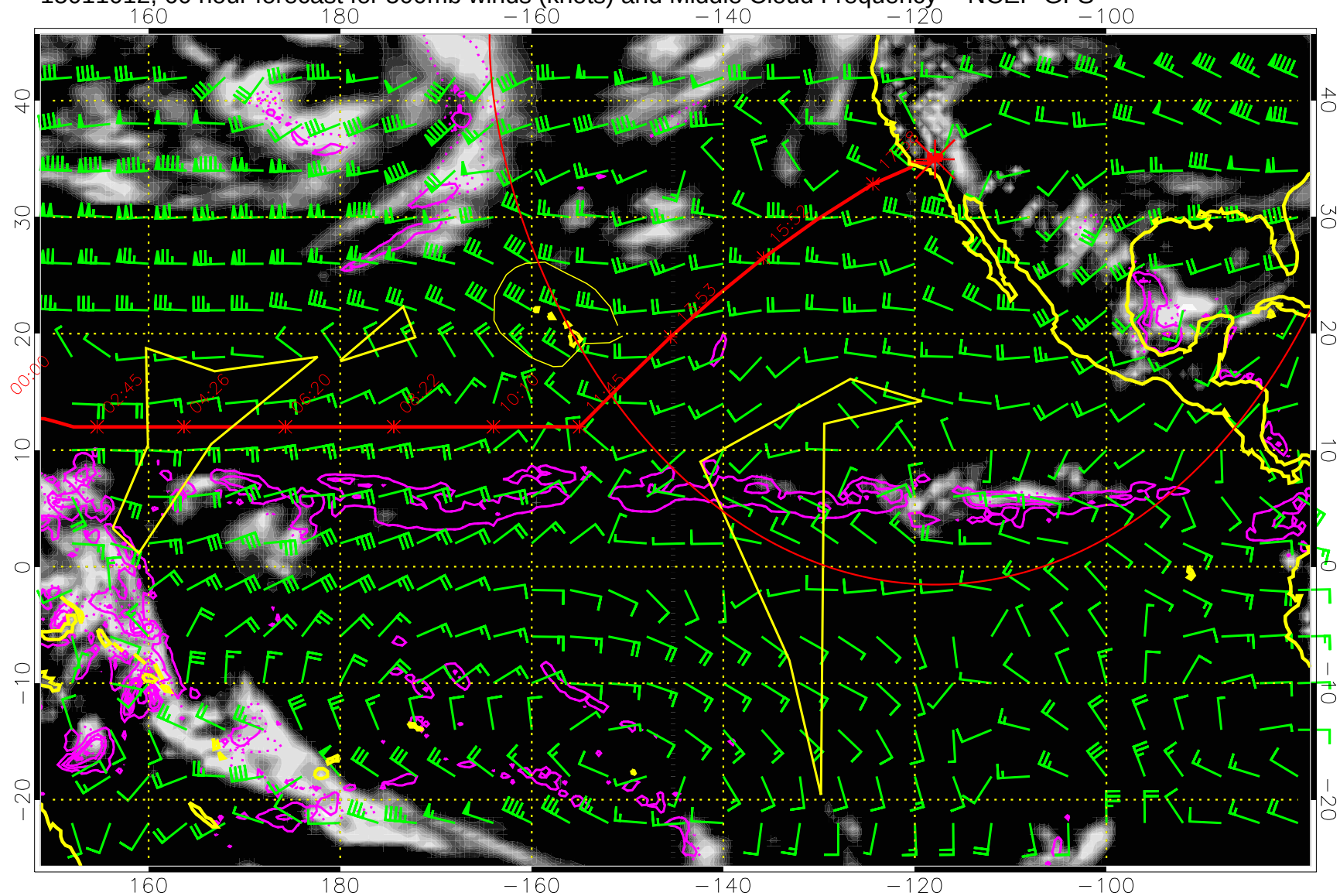
15011012, 60 hour forecast for 500mb winds (knots) and Middle Cloud Frequency -- NCEP GFS
