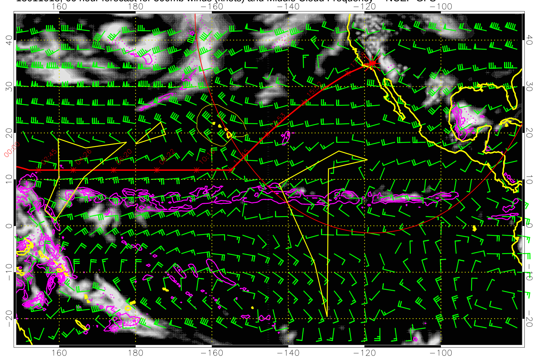
15011018, 66 hour forecast for 500mb winds (knots) and Middle Cloud Frequency -- NCEP GFS
