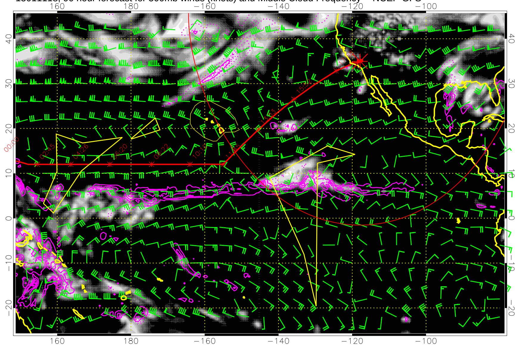
15011118, 90 hour forecast for 500mb winds (knots) and Middle Cloud Frequency -- NCEP GFS
