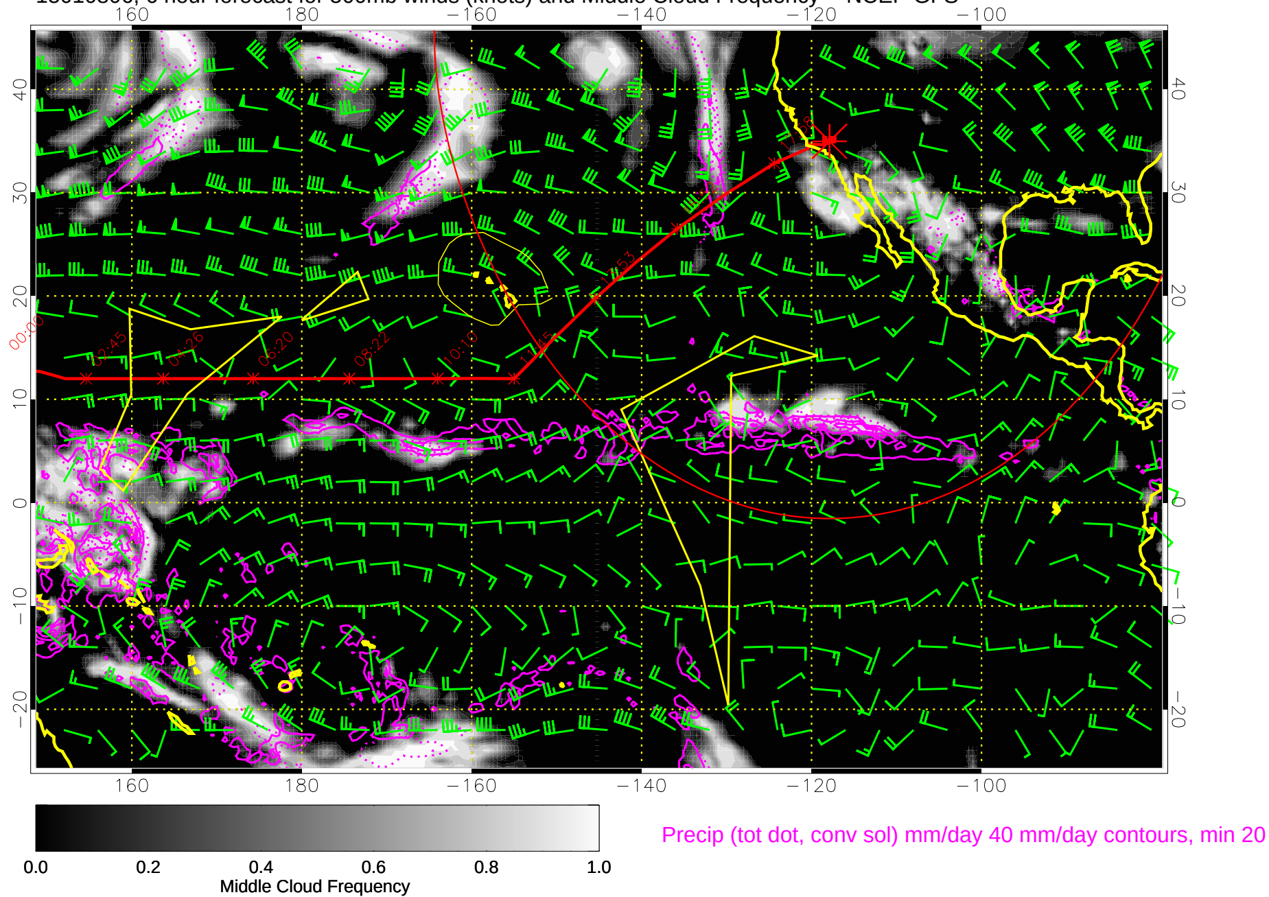
15010806, 6 hour forecast for 500mb winds (knots) and Middle Cloud Frequency -- NCEP GFS
