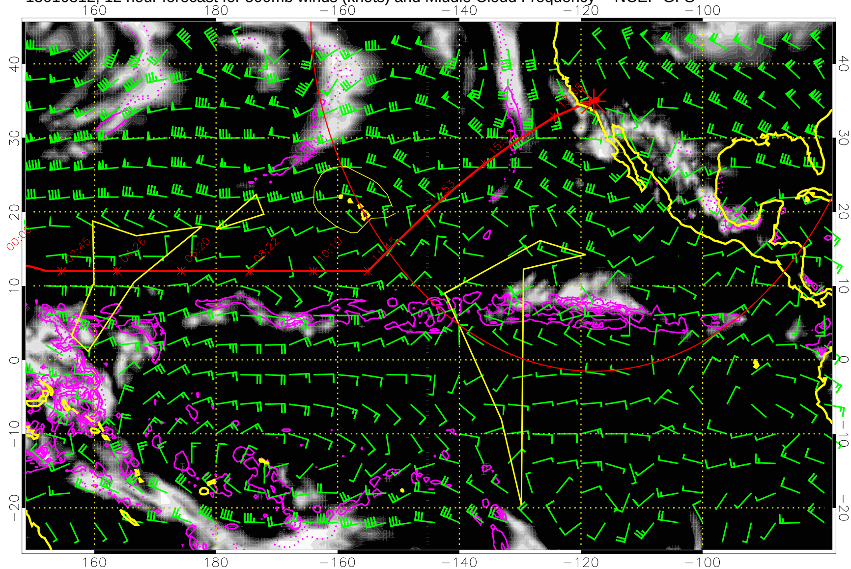
15010812, 12 hour forecast for 500mb winds (knots) and Middle Cloud Frequency -- NCEP GFS
