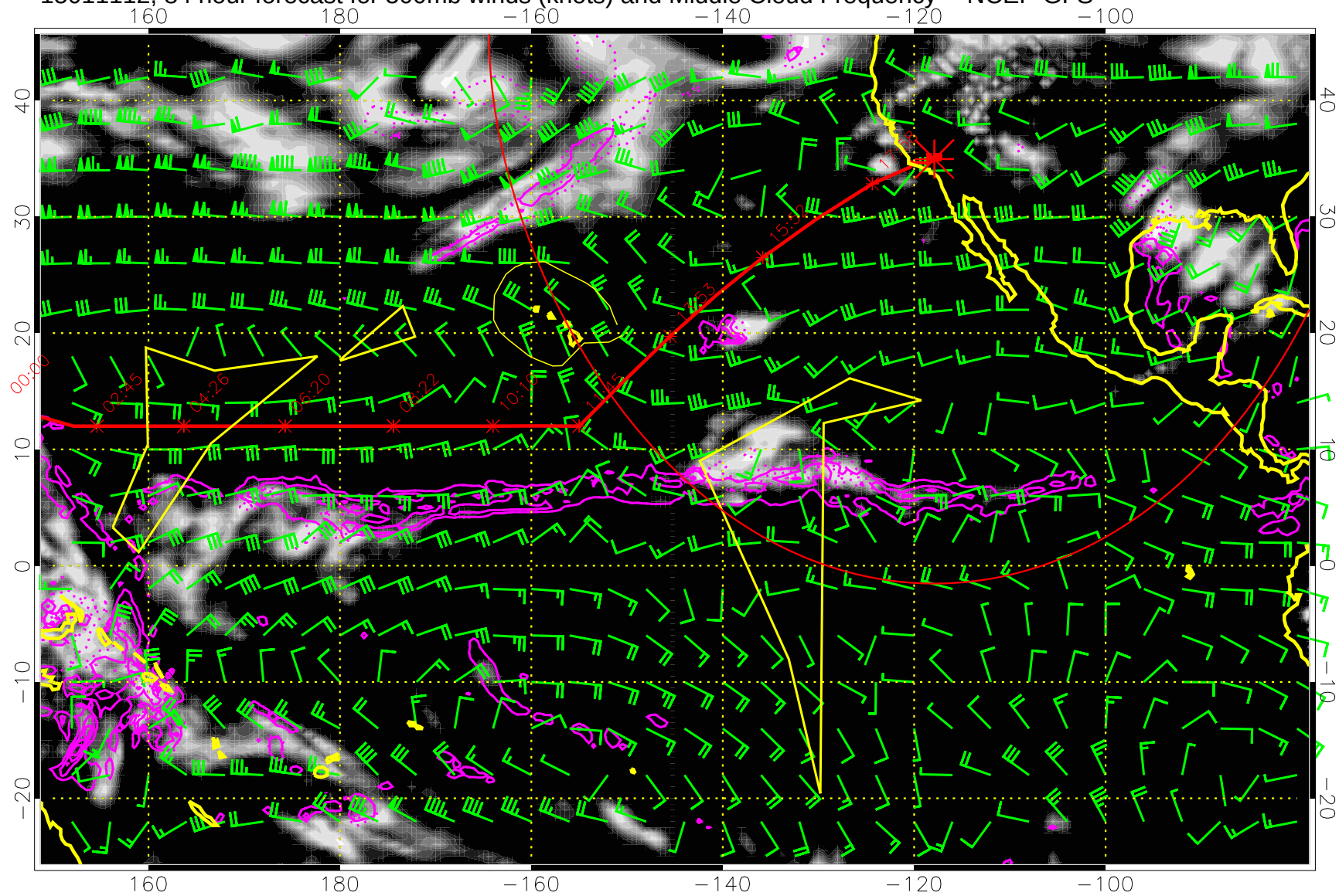
15011112, 84 hour forecast for 500mb winds (knots) and Middle Cloud Frequency -- NCEP GFS
