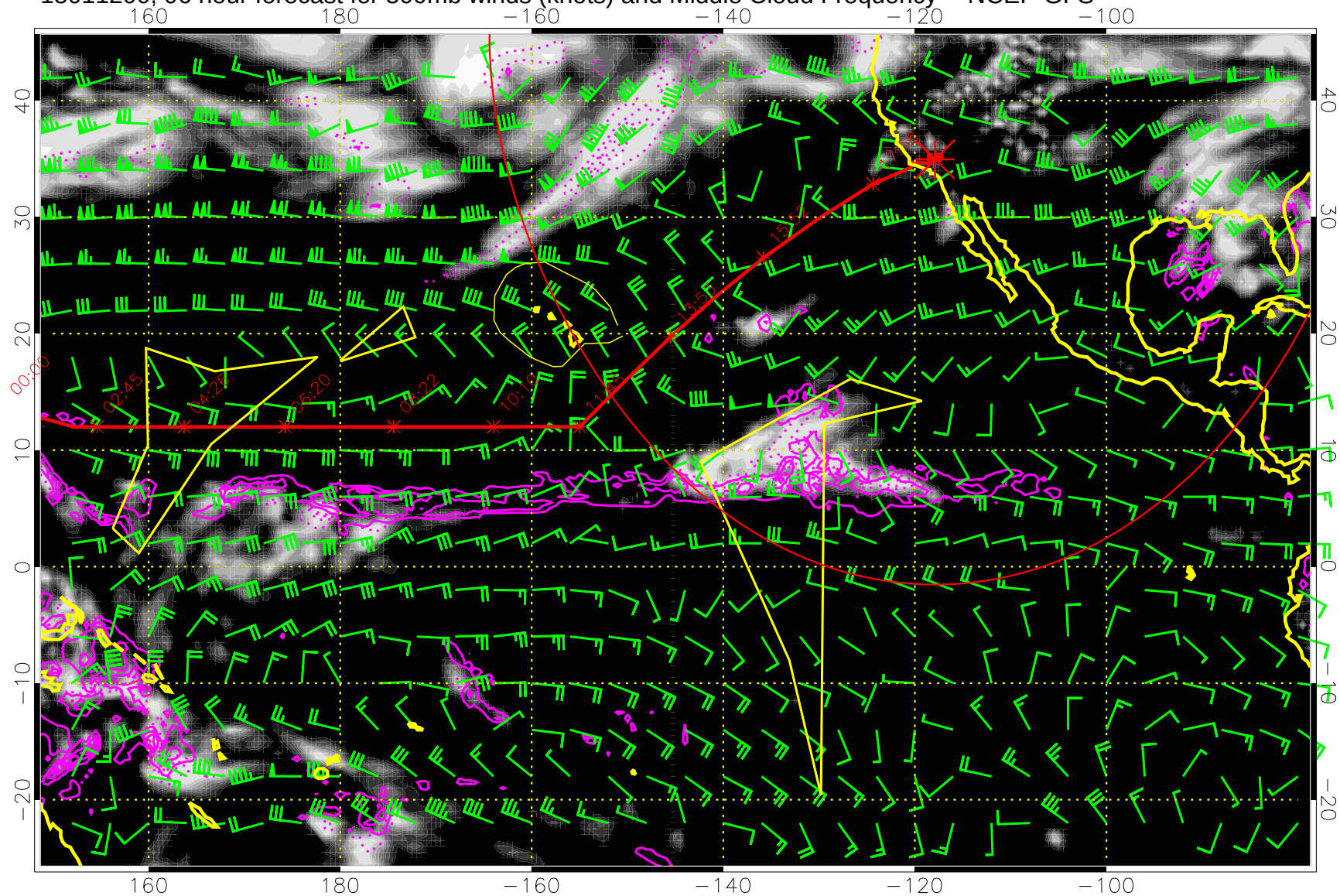
15011200, 96 hour forecast for 500mb winds (knots) and Middle Cloud Frequency -- NCEP GFS
