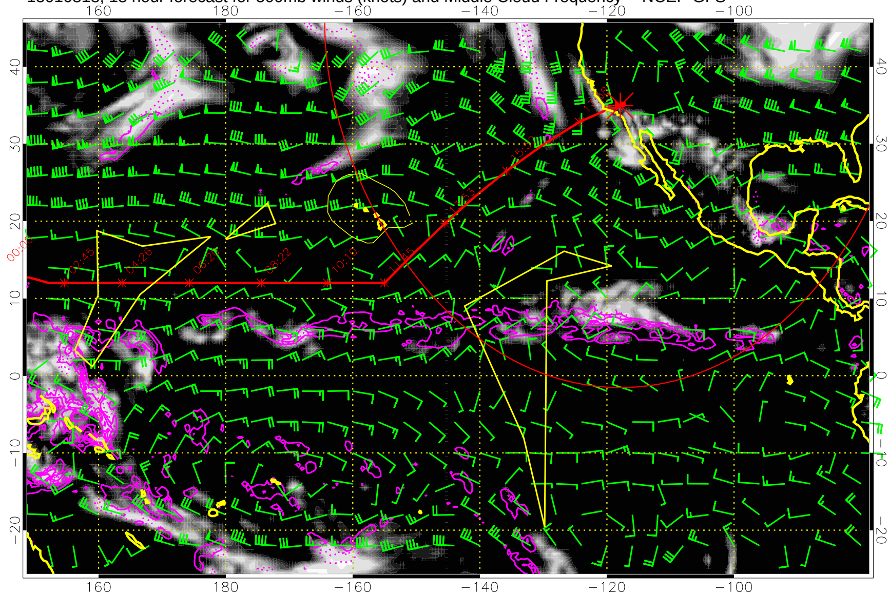
15010818, 18 hour forecast for 500mb winds (knots) and Middle Cloud Frequency -- NCEP GFS
