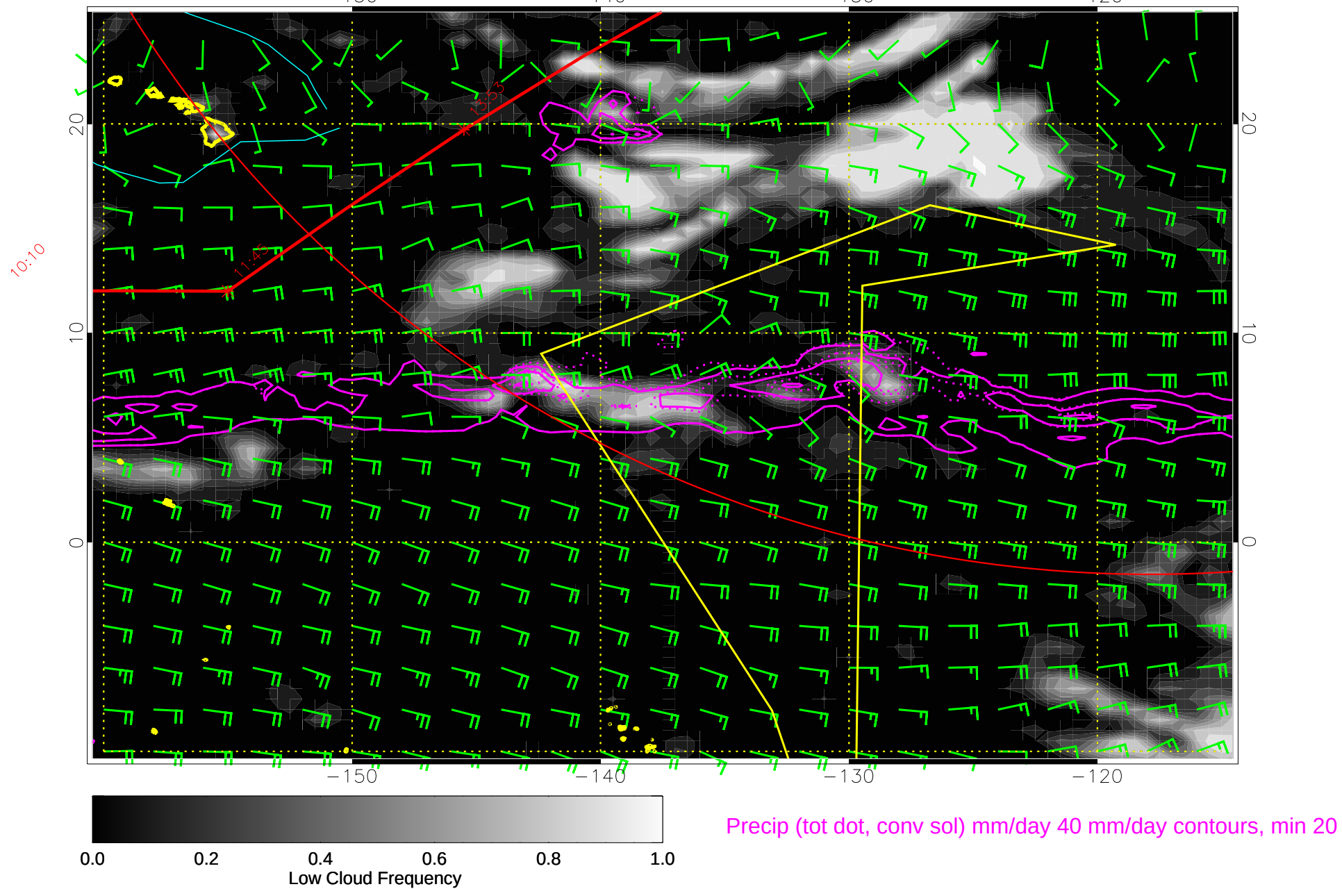
15011112, 84 hour forecast for 850mb winds (knots) and Low Cloud Frequency -- NCEP GFS
