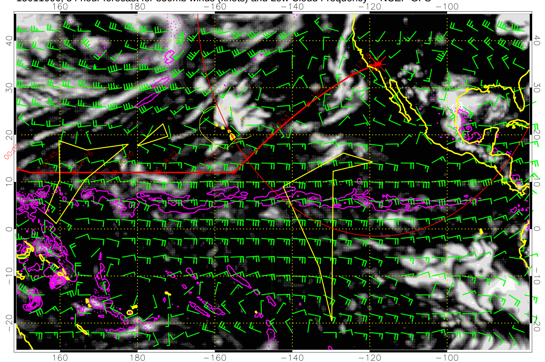
15011006, 54 hour forecast for 850mb winds (knots) and Low Cloud Frequency -- NCEP GFS
