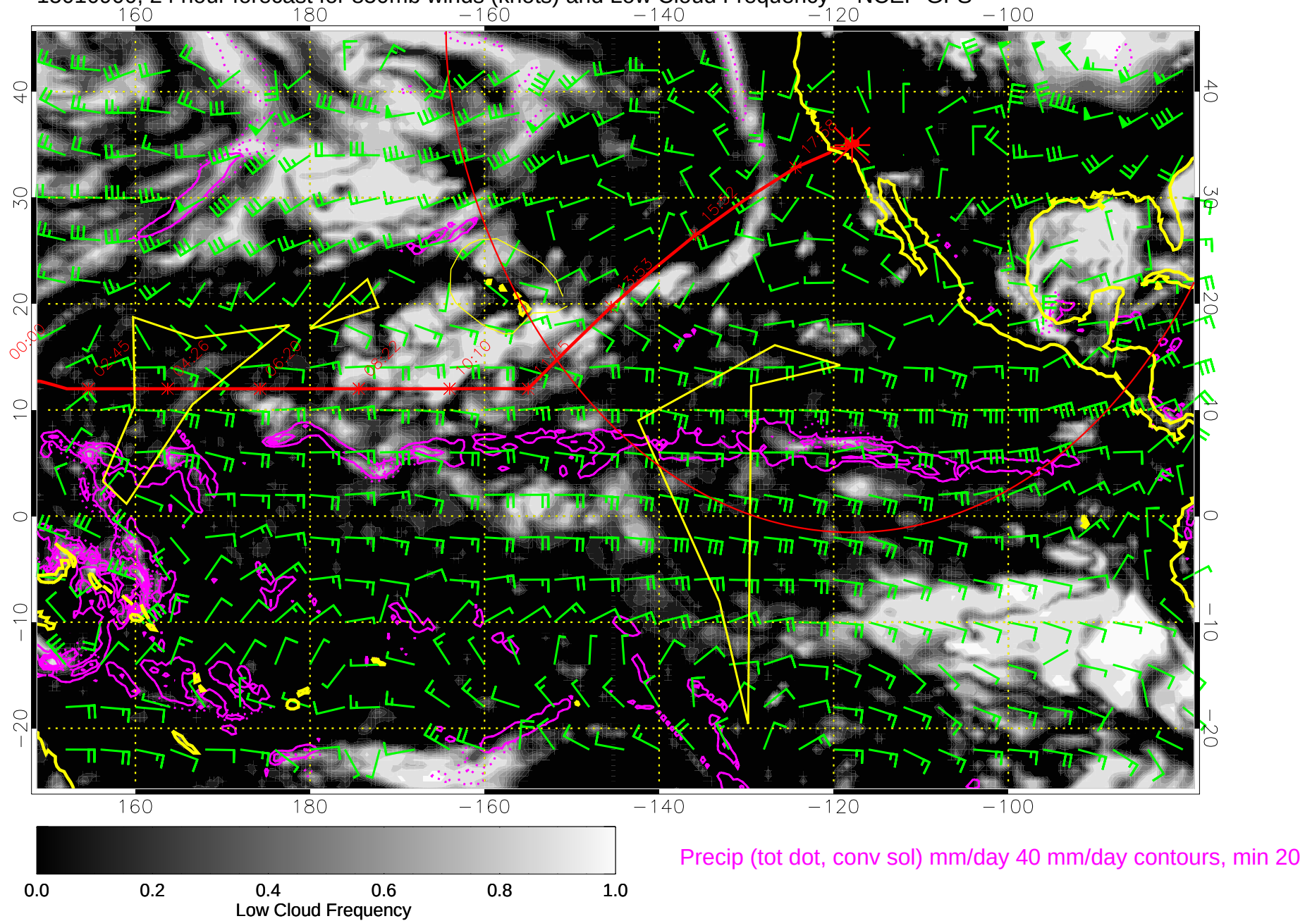
15010900, 24 hour forecast for 850mb winds (knots) and Low Cloud Frequency -- NCEP GFS
