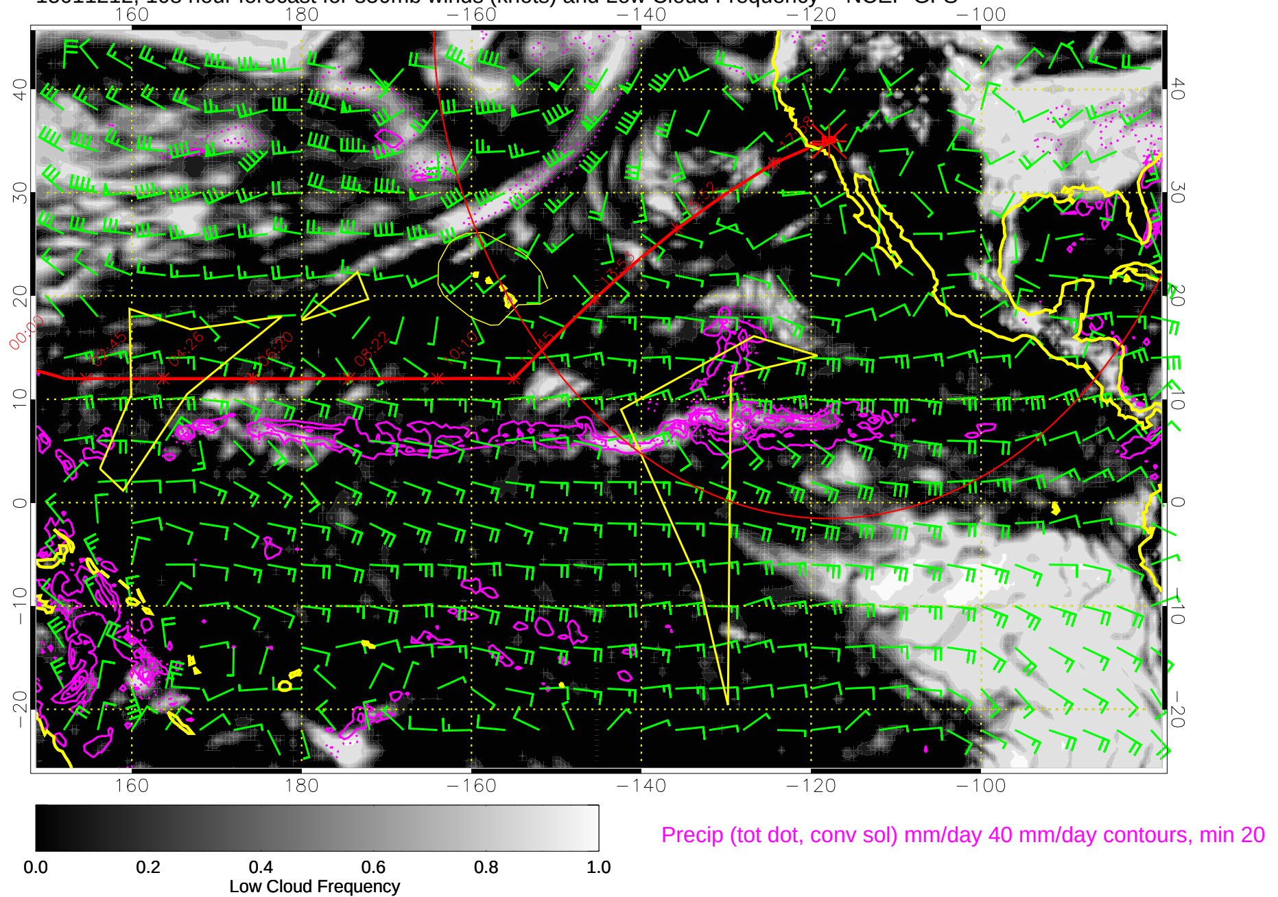
15011212, 108 hour forecast for 850mb winds (knots) and Low Cloud Frequency -- NCEP GFS
