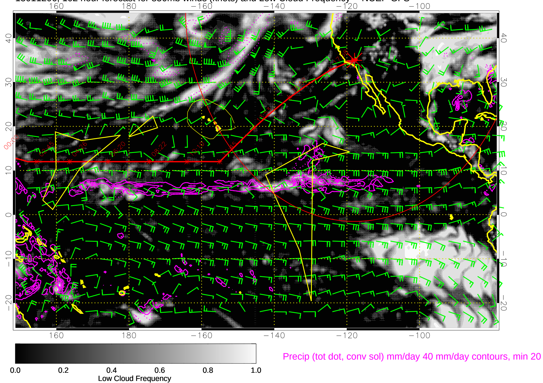
15011206, 102 hour forecast for 850mb winds (knots) and Low Cloud Frequency -- NCEP GFS
