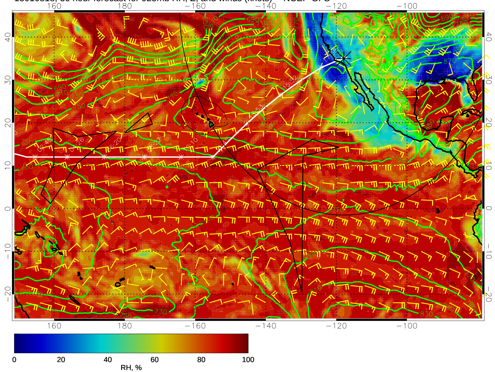
15010818, 30 hour forecast for 925mb RH, Z, and winds (knots) -- NCEP GFS
