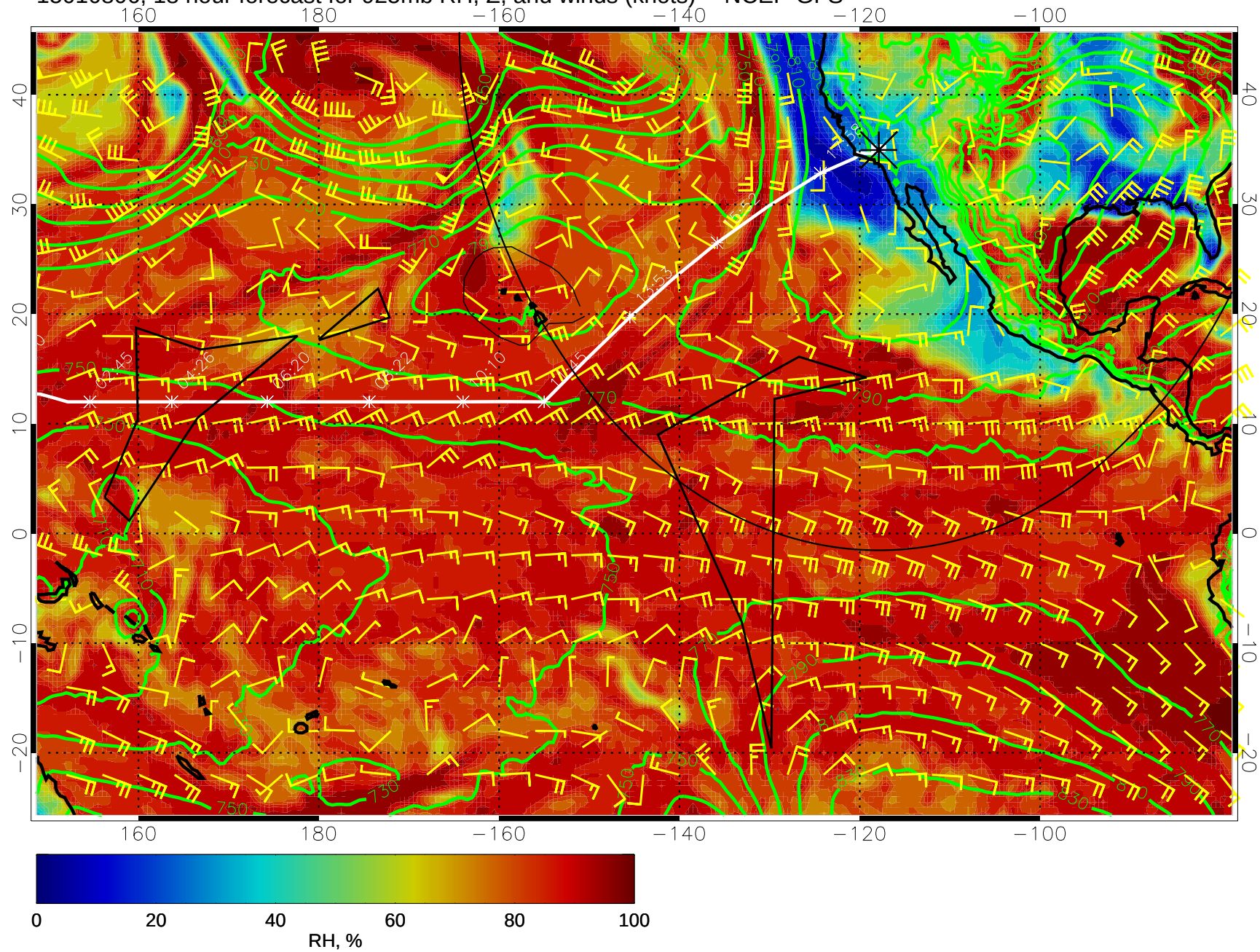
15010806, 18 hour forecast for 925mb RH, Z, and winds (knots) -- NCEP GFS
