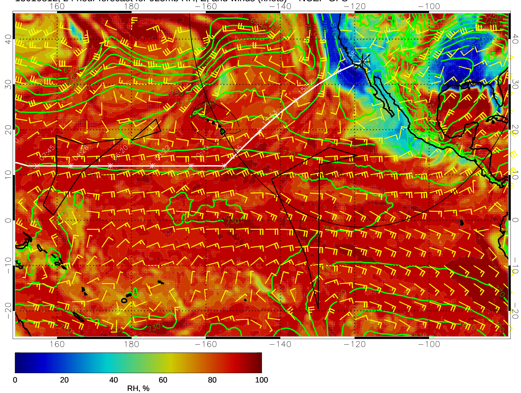
15010812, 24 hour forecast for 925mb RH, Z, and winds (knots) -- NCEP GFS
