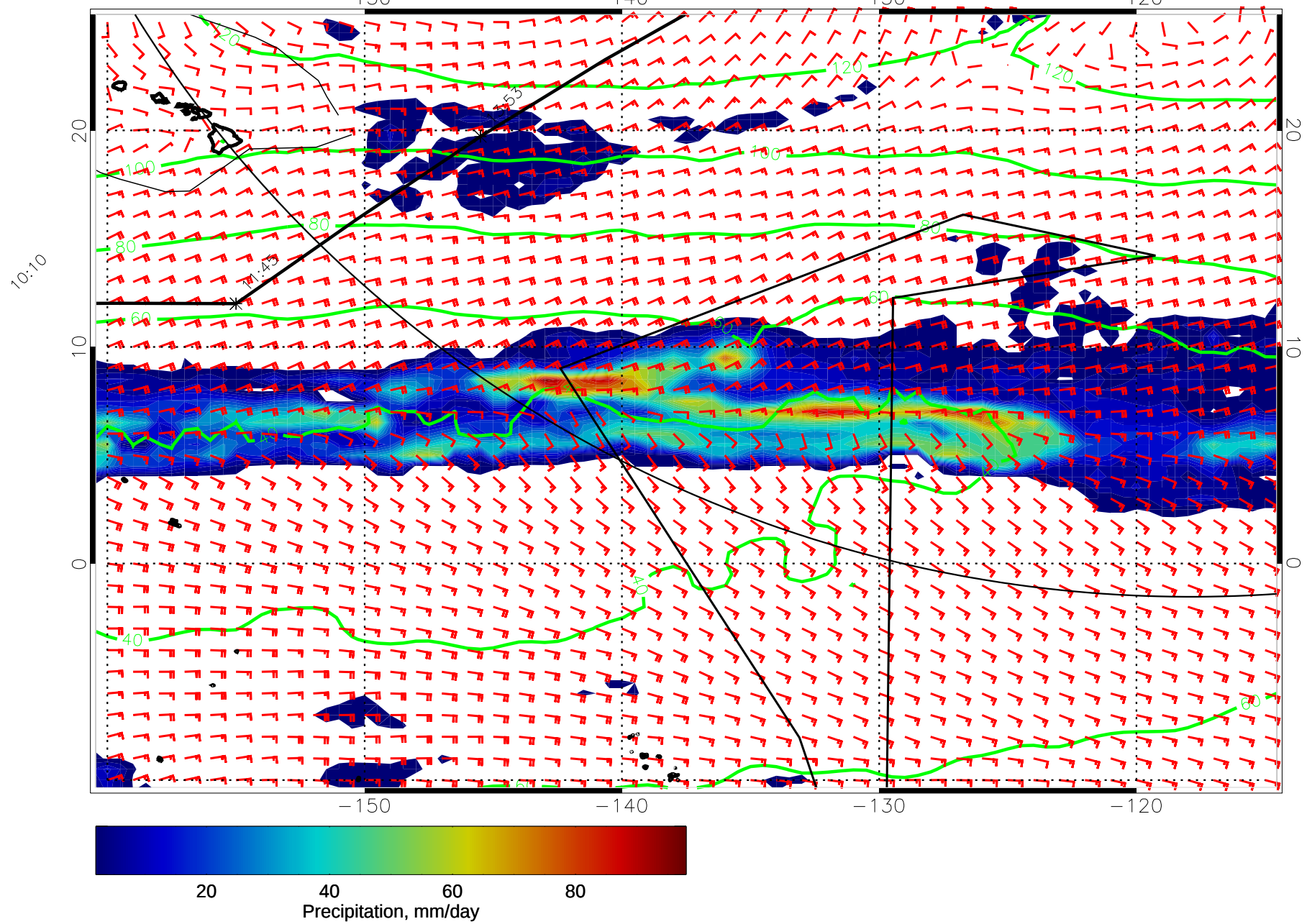
15011100, 84 hour forecast for precip, 1000mb Z, and winds (knots) -- NCEP GFS
