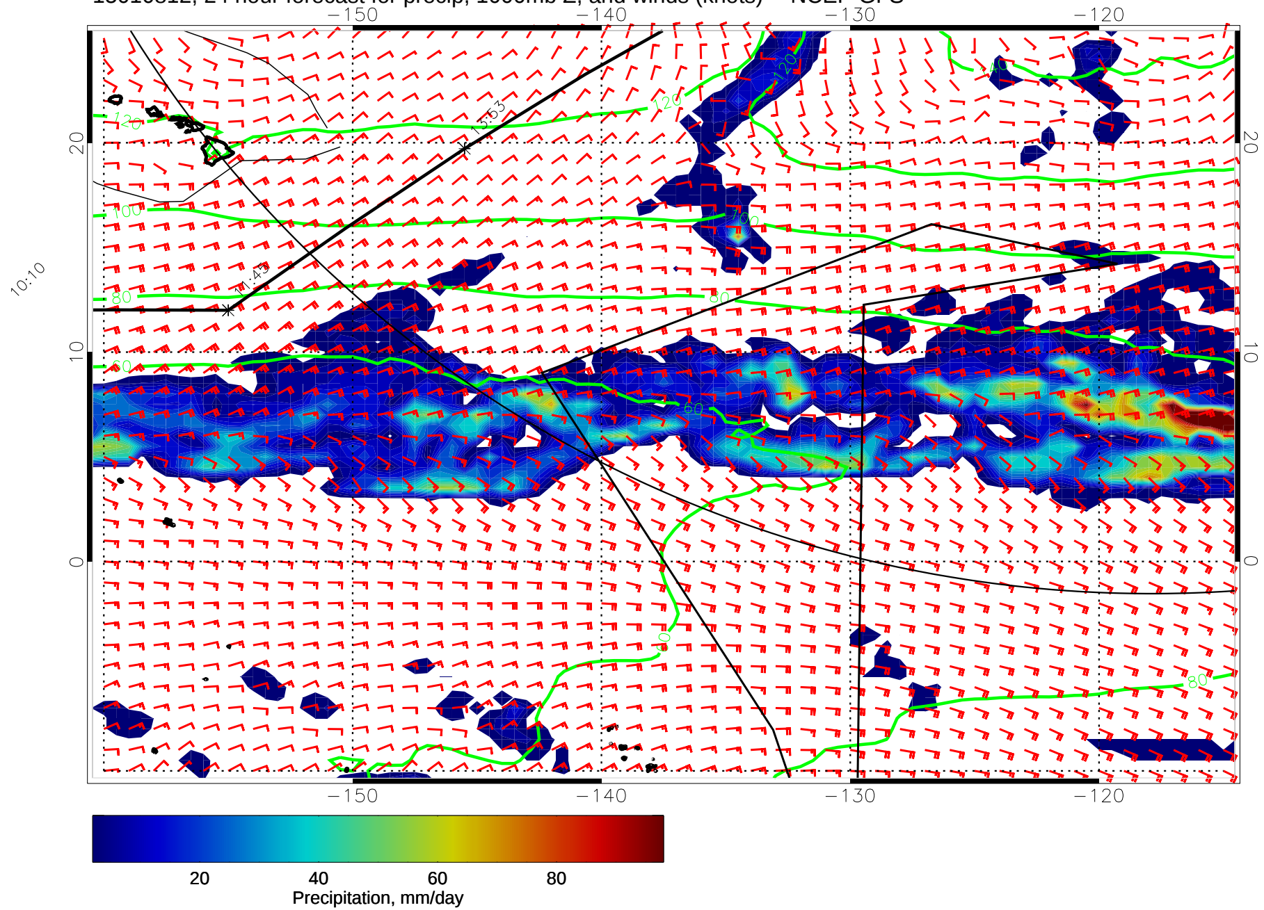
15010812, 24 hour forecast for precip, 1000mb Z, and winds (knots) -- NCEP GFS
