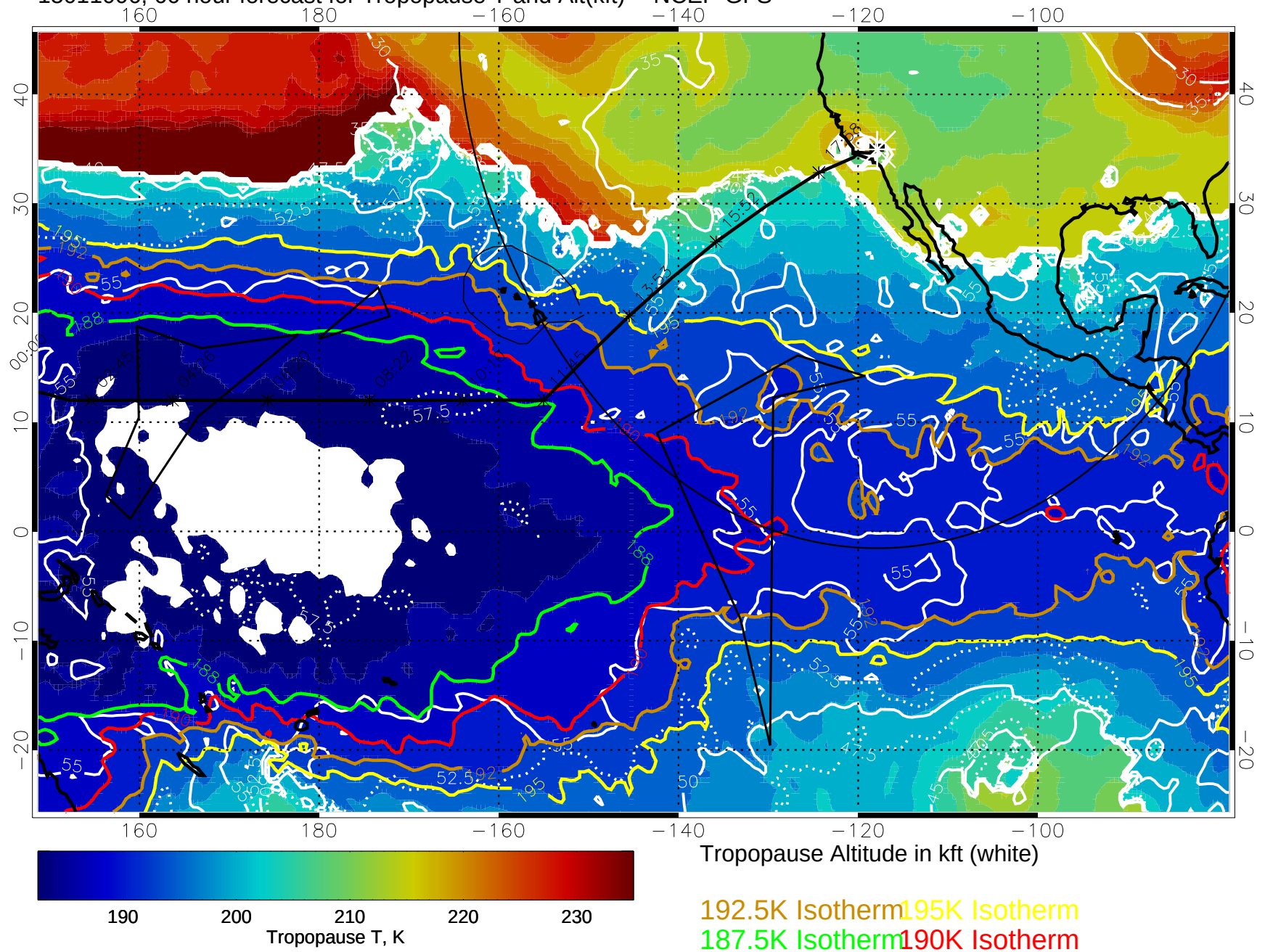
15011006, 66 hour forecast for Tropopause T and Alt(kft) -- NCEP GFS
