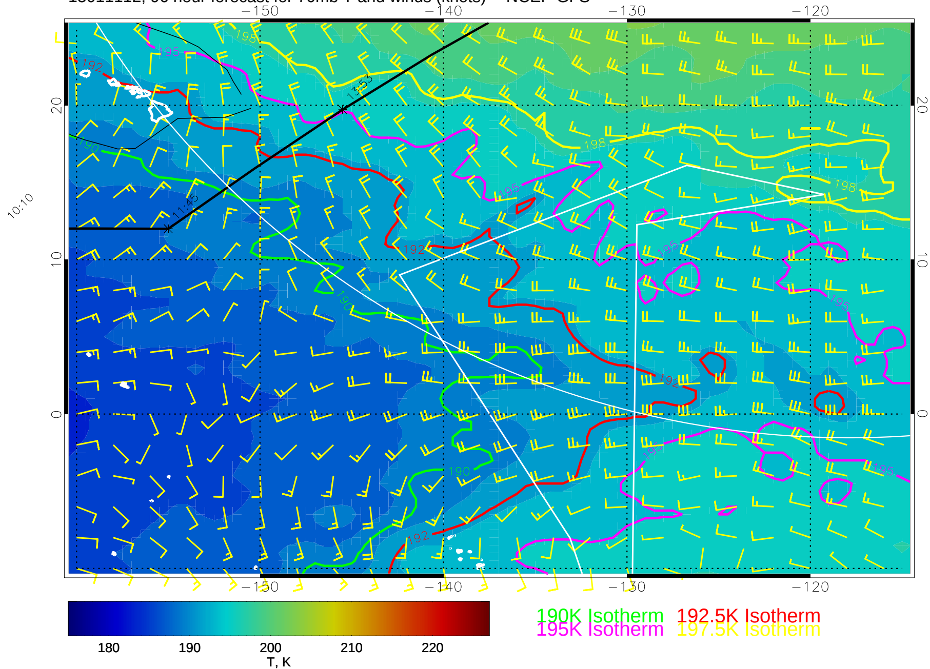
15011112, 96 hour forecast for 70mb T and winds (knots) -- NCEP GFS
