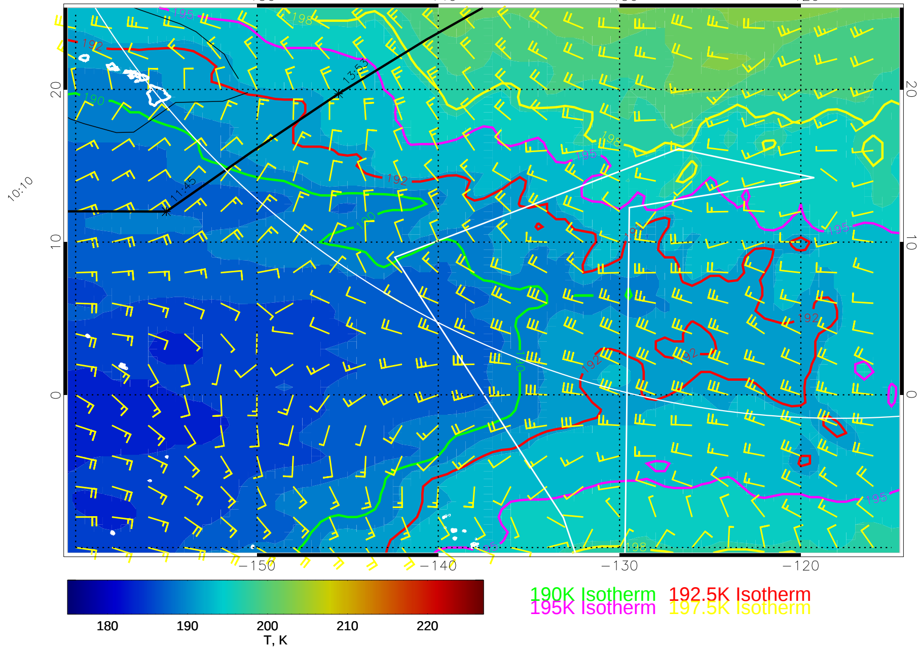
15011206, 114 hour forecast for 70mb T and winds (knots) -- NCEP GFS
