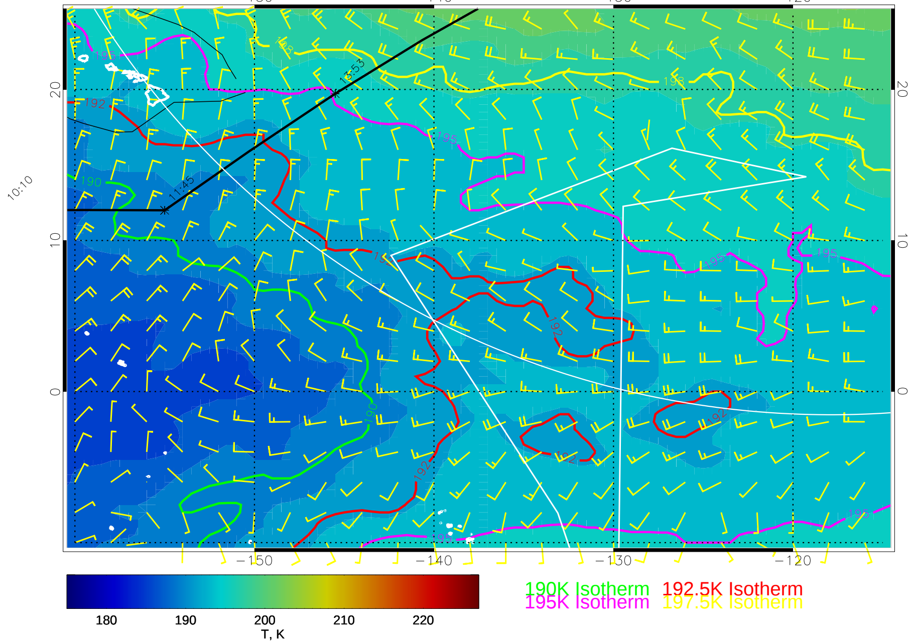
15011006, 66 hour forecast for 70mb T and winds (knots) -- NCEP GFS
