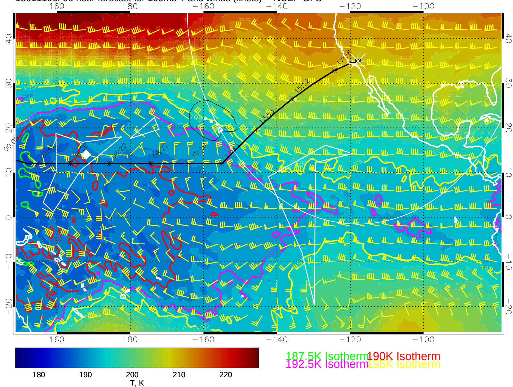
15011106, 90 hour forecast for 100mb T and winds (knots) -- NCEP GFS
