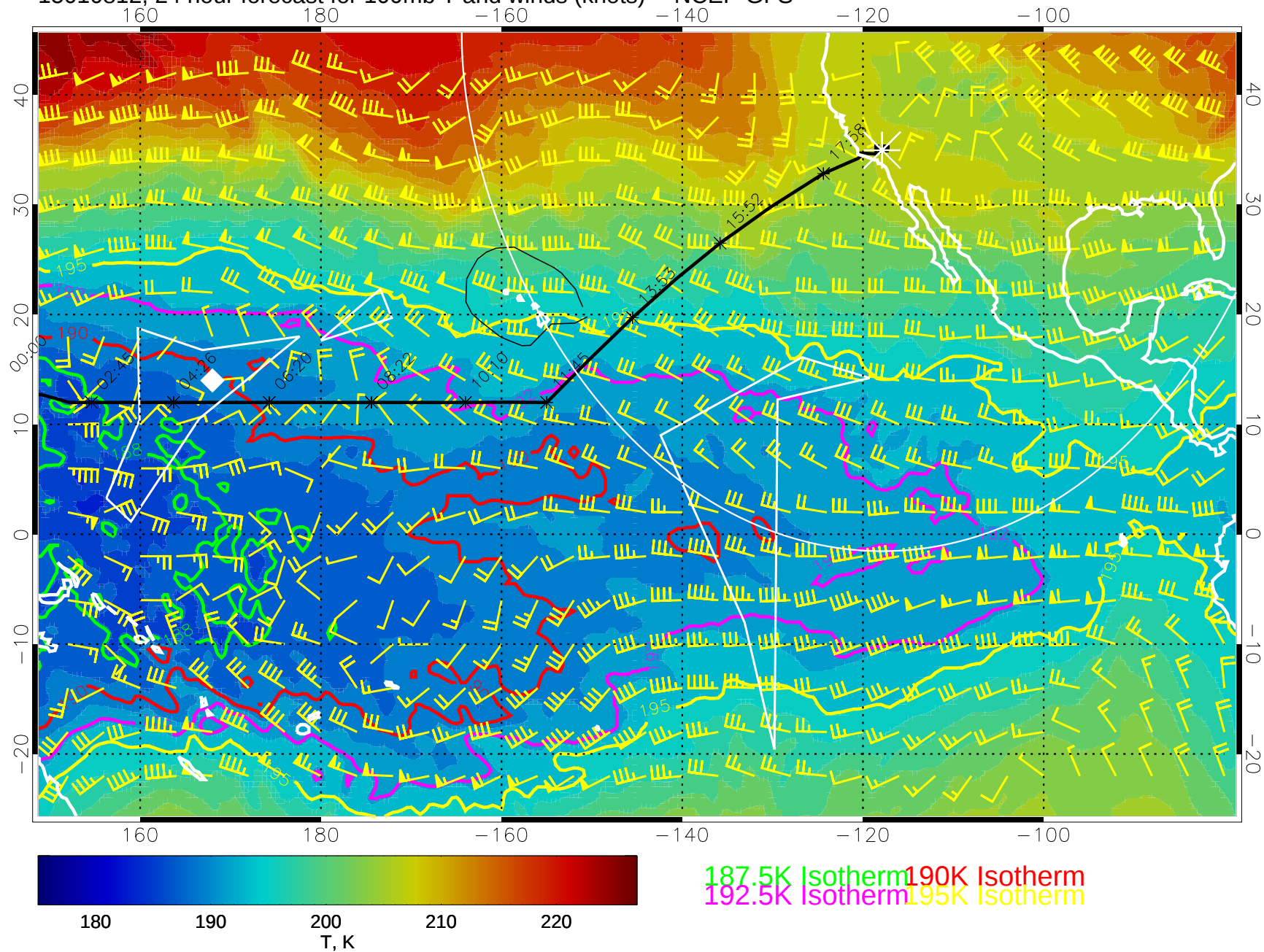
15010812, 24 hour forecast for 100mb T and winds (knots) -- NCEP GFS
