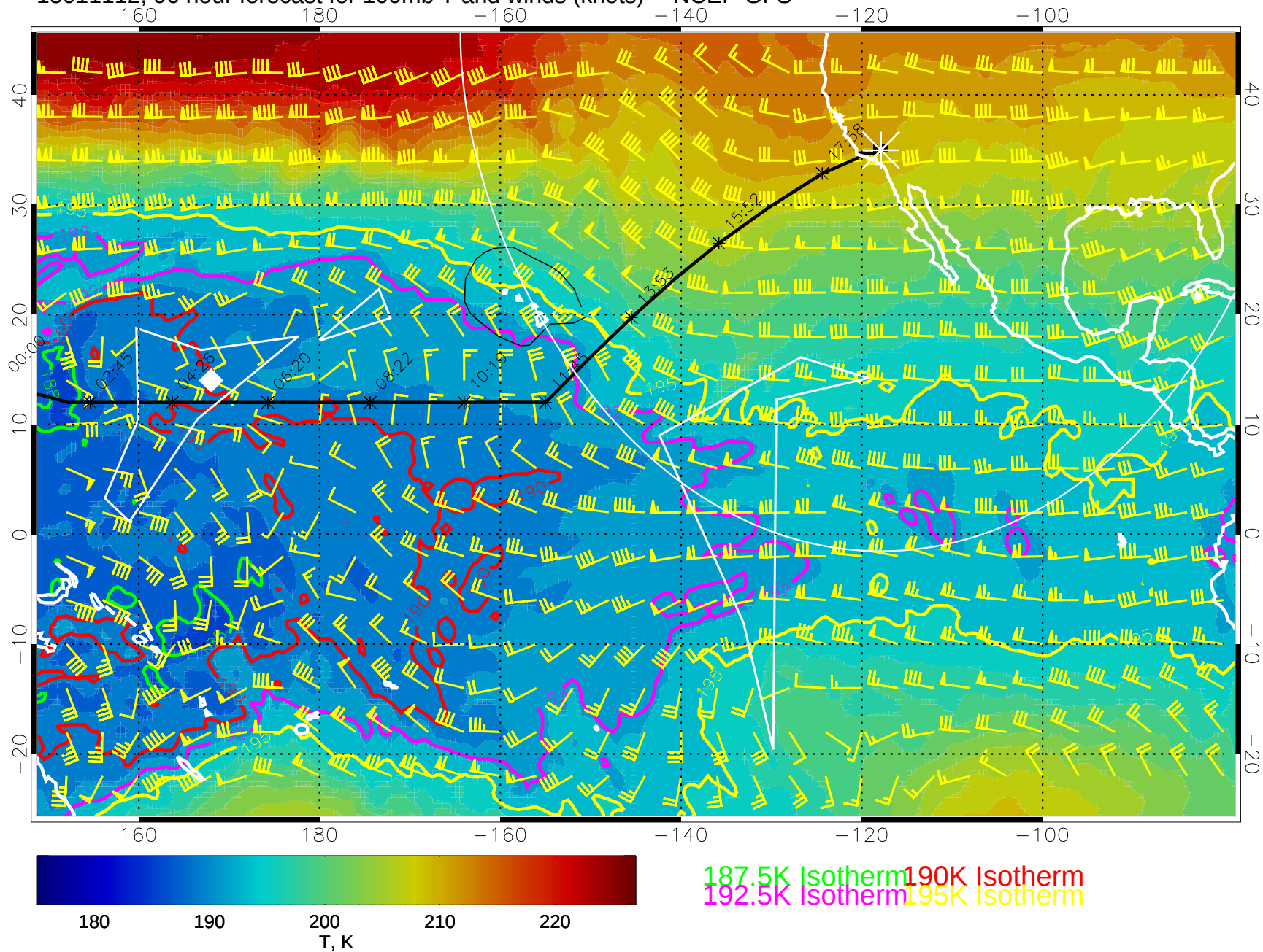
15011112, 96 hour forecast for 100mb T and winds (knots) -- NCEP GFS
