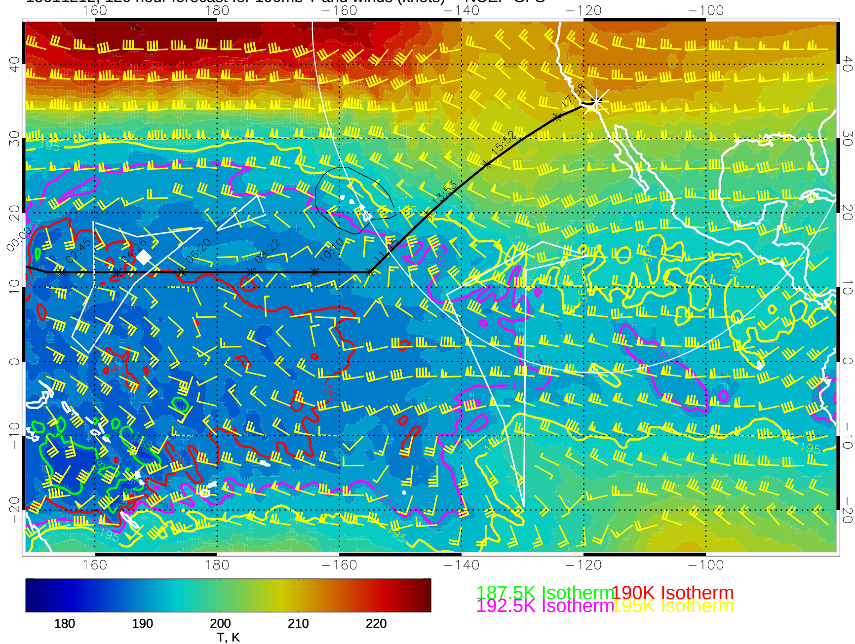
15011212, 120 hour forecast for 100mb T and winds (knots) -- NCEP GFS
