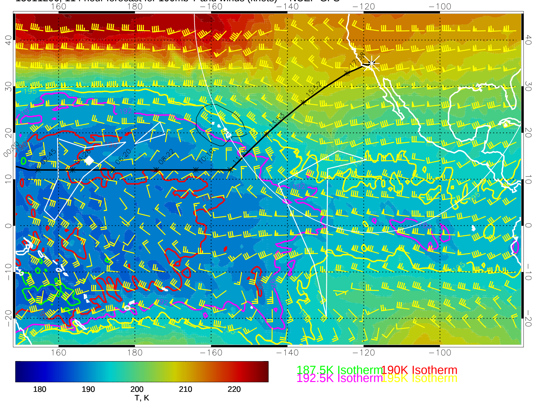
15011206, 114 hour forecast for 100mb T and winds (knots) -- NCEP GFS
