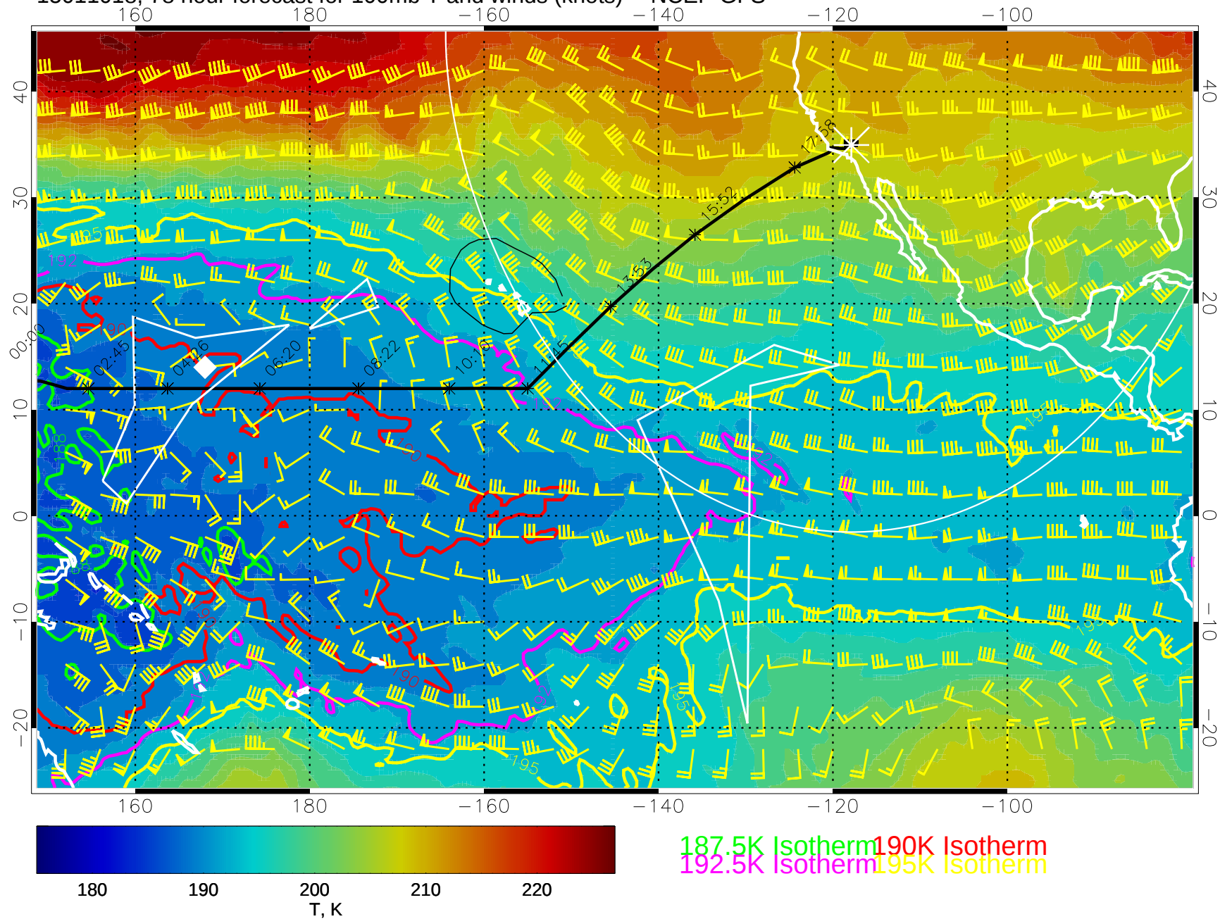
15011018, 78 hour forecast for 100mb T and winds (knots) -- NCEP GFS
