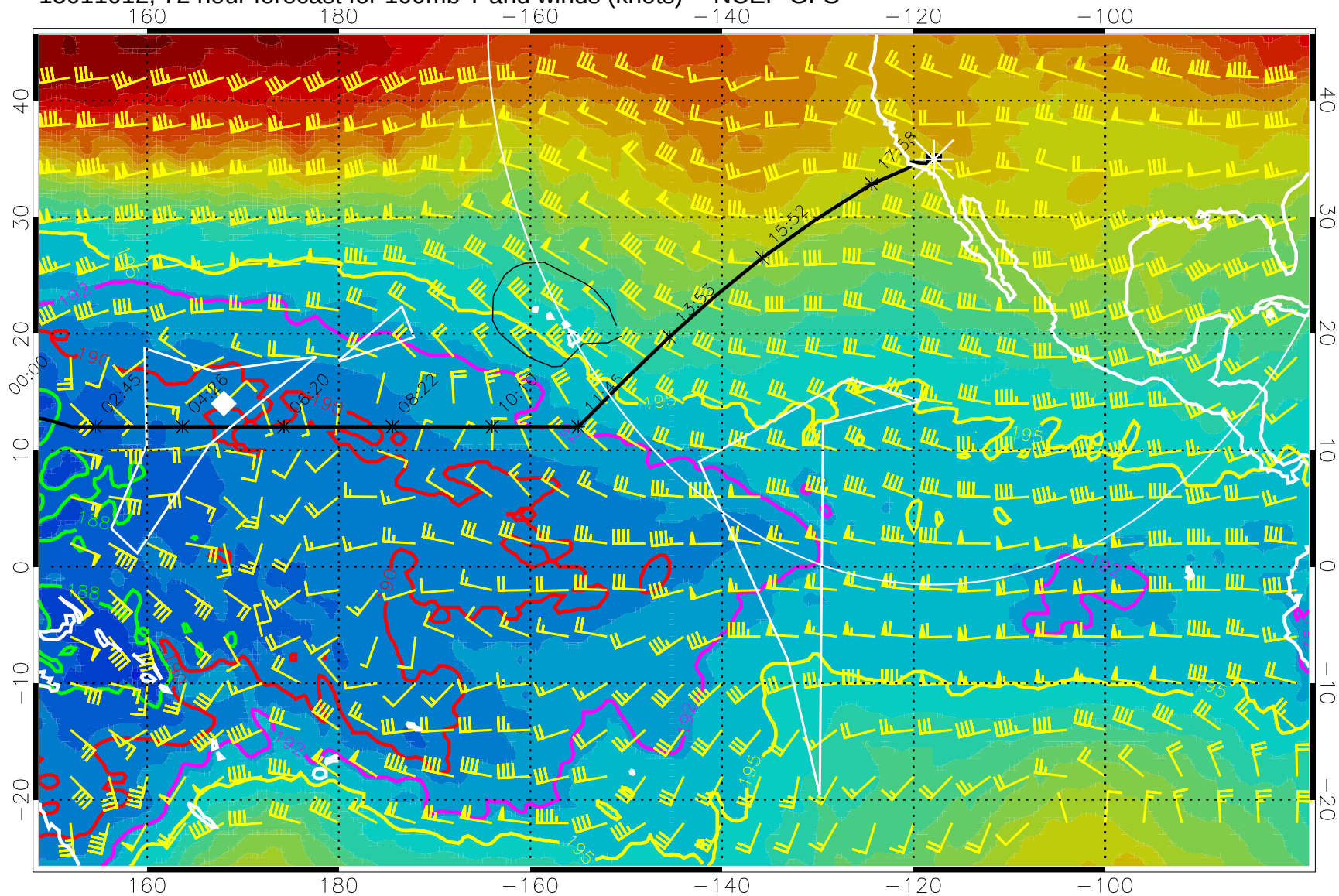
15011012, 72 hour forecast for 100mb T and winds (knots) -- NCEP GFS
