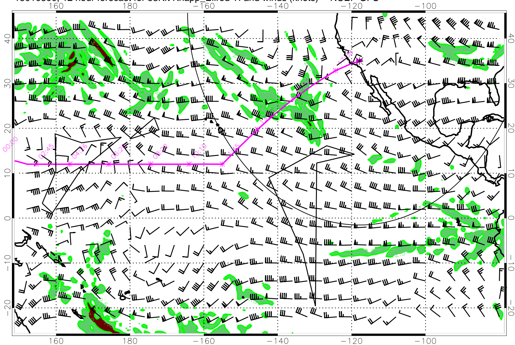
15010800, 12 hour forecast for 53Kft Knapp_Ellrod TI and winds (knots) -- NCEP GFS
