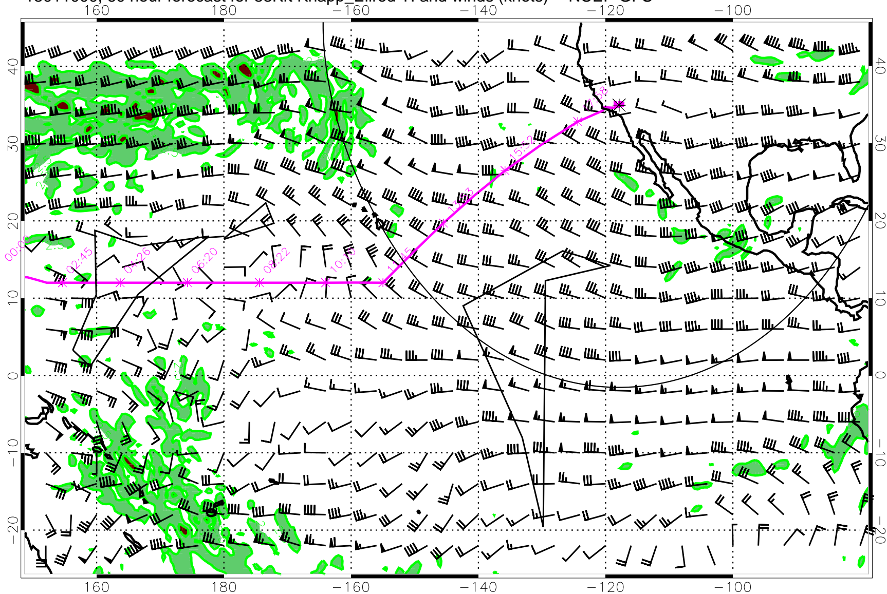
15011000, 60 hour forecast for 53Kft Knapp_Ellrod TI and winds (knots) -- NCEP GFS
