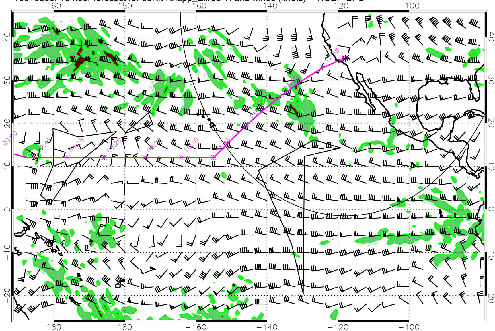
15010806, 18 hour forecast for 53Kft Knapp_Ellrod TI and winds (knots) -- NCEP GFS
