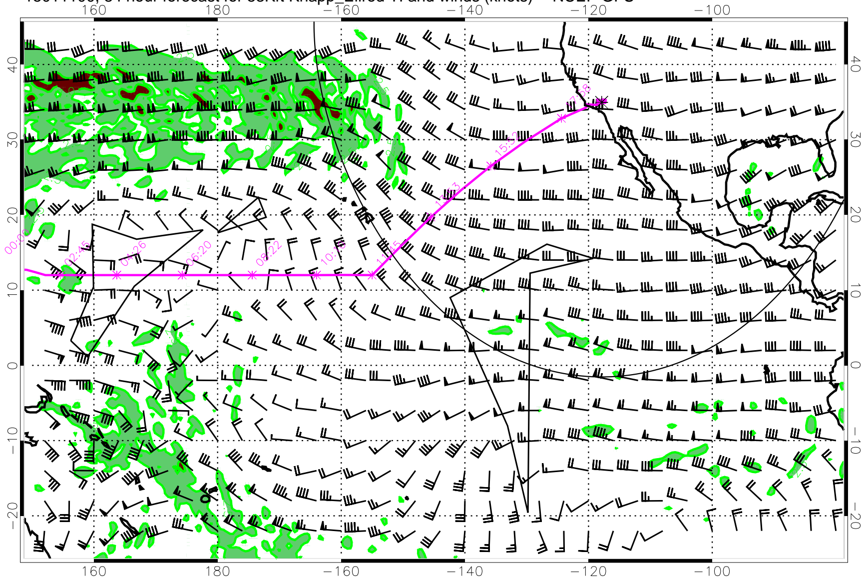
15011100, 84 hour forecast for 53Kft Knapp_Ellrod TI and winds (knots) -- NCEP GFS
