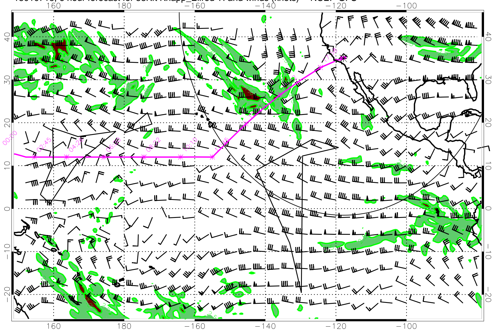
15010718, 6 hour forecast for 53Kft Knapp_Ellrod TI and winds (knots) -- NCEP GFS
