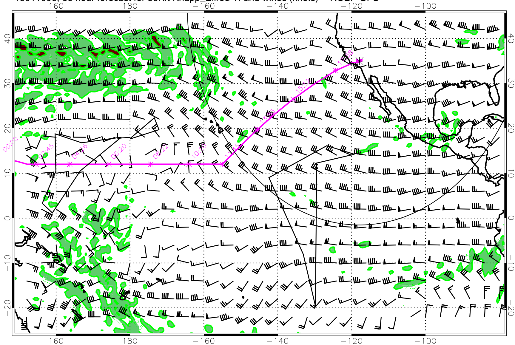
15011006, 66 hour forecast for 53Kft Knapp_Ellrod TI and winds (knots) -- NCEP GFS
