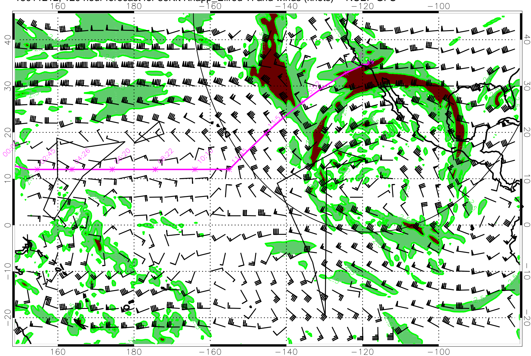
15011212, 120 hour forecast for 36Kft Knapp_Ellrod TI and winds (knots) -- NCEP GFS
