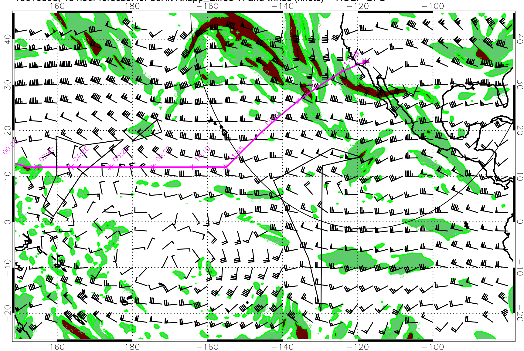
15010806, 18 hour forecast for 36Kft Knapp_Ellrod TI and winds (knots) -- NCEP GFS
