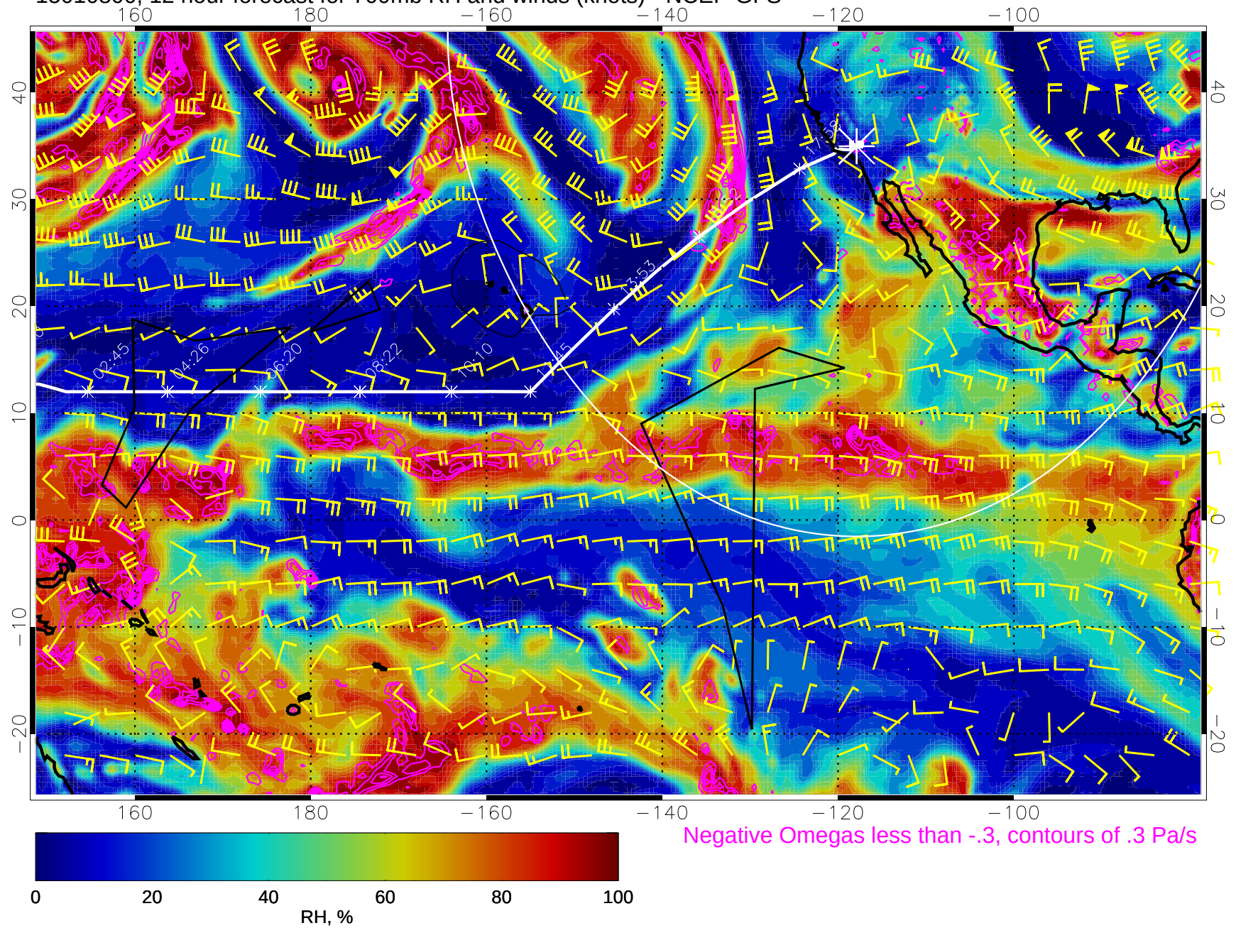
15010800, 12 hour forecast for 700mb RH and winds (knots) - NCEP GFS
