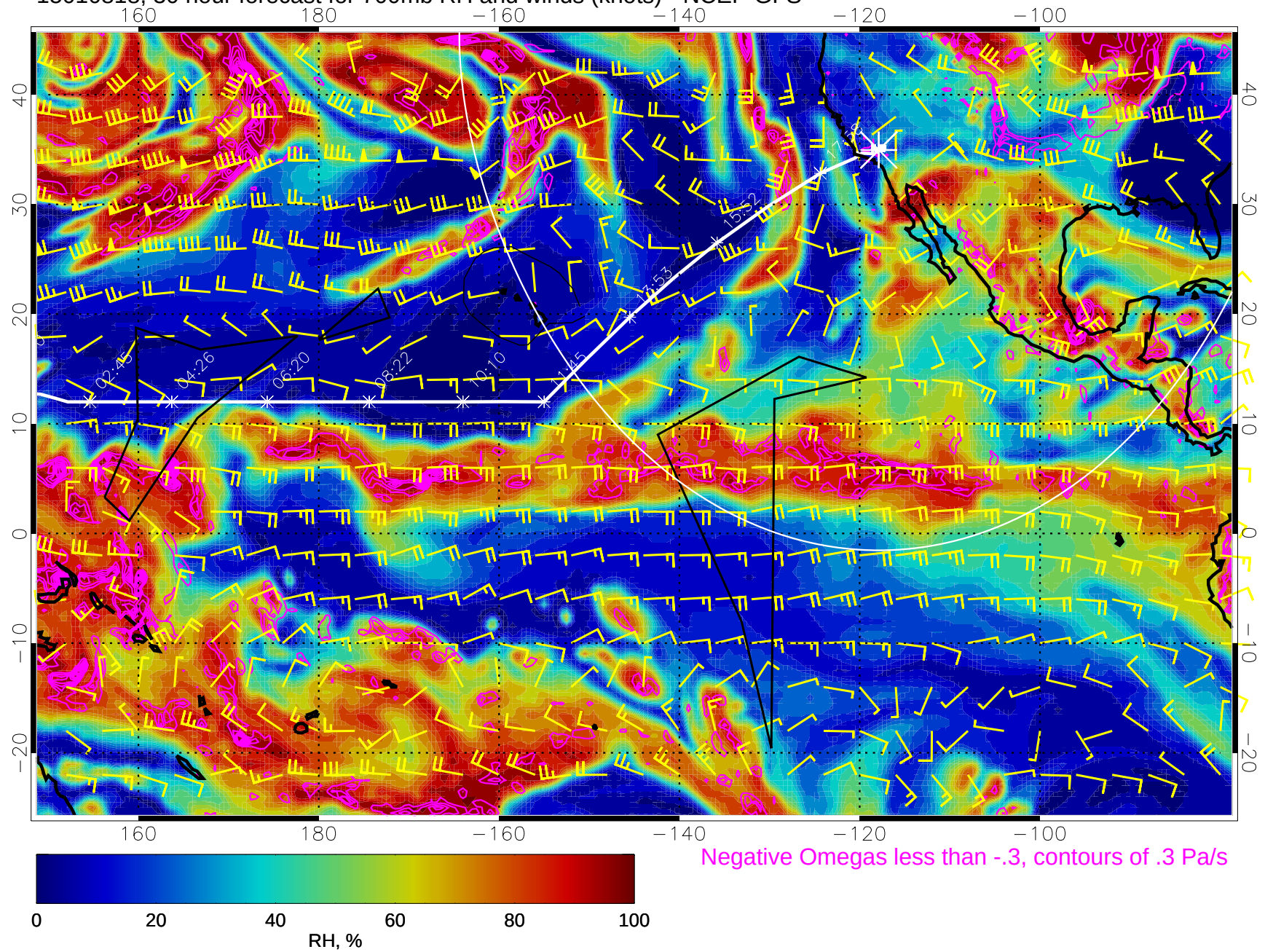
15010818, 30 hour forecast for 700mb RH and winds (knots) - NCEP GFS
