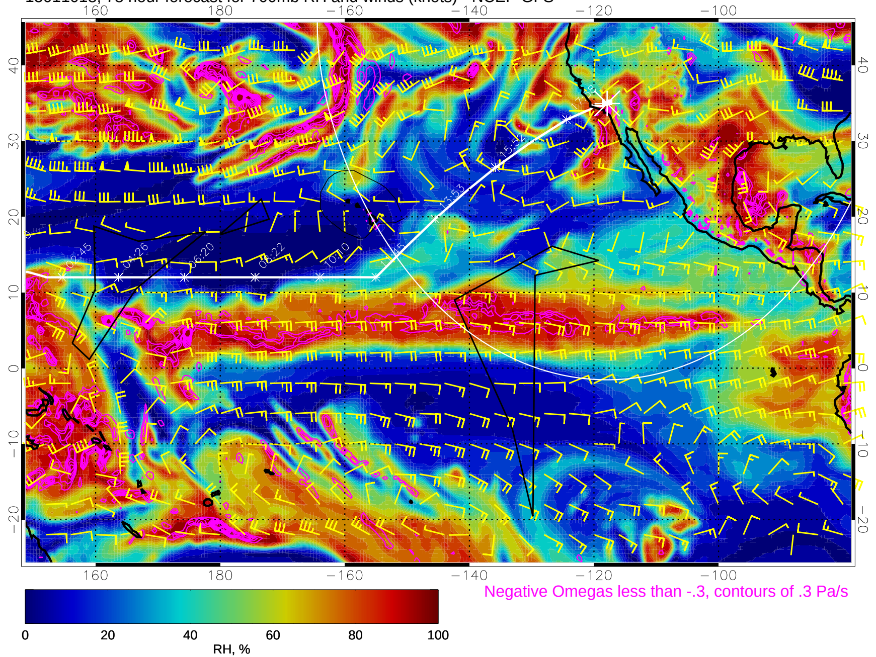
15011018, 78 hour forecast for 700mb RH and winds (knots) - NCEP GFS
