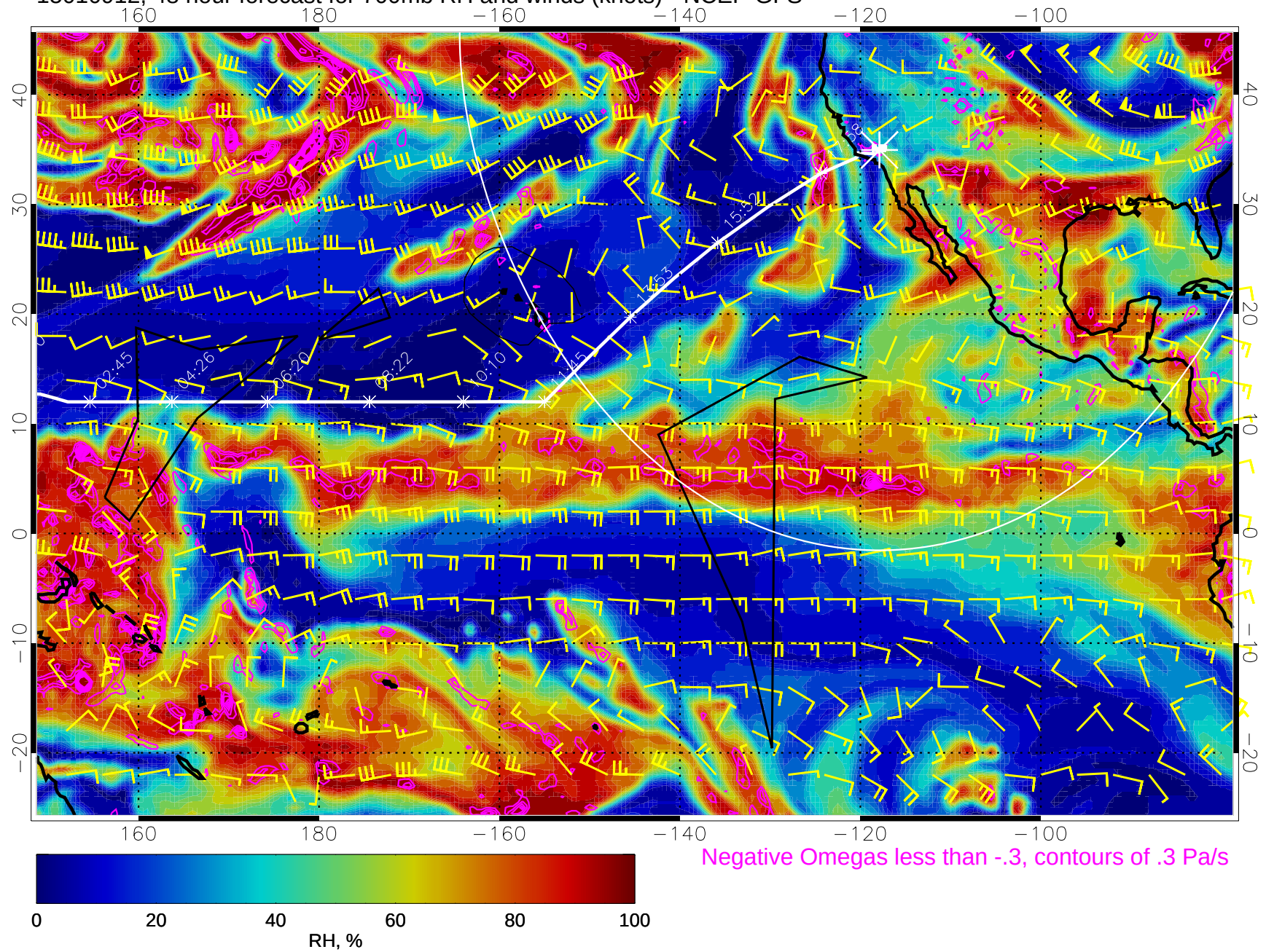
15010912, 48 hour forecast for 700mb RH and winds (knots) - NCEP GFS
