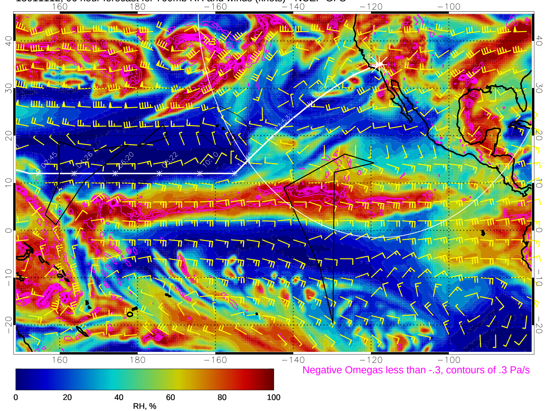
15011112, 96 hour forecast for 700mb RH and winds (knots) - NCEP GFS
