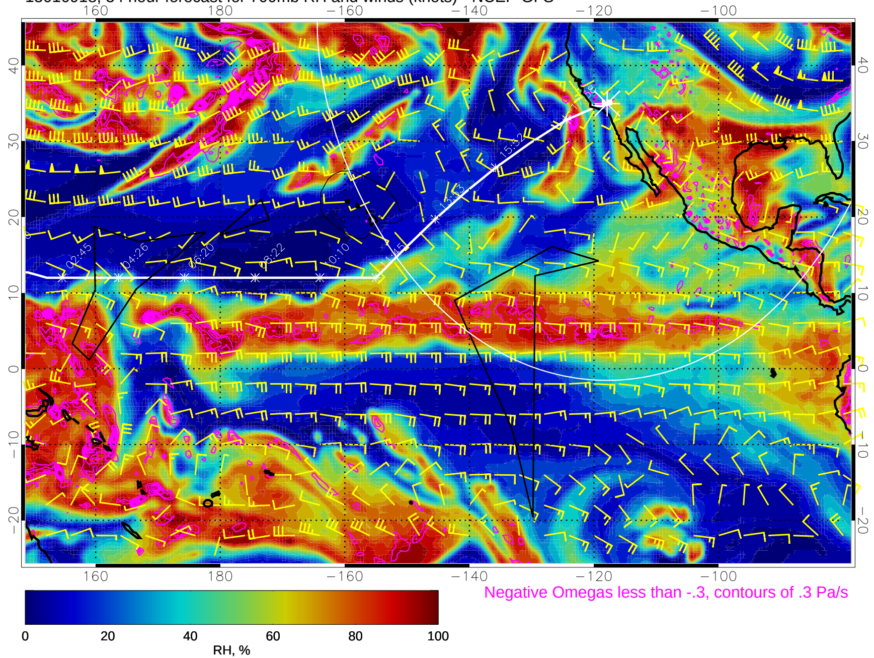
15010918, 54 hour forecast for 700mb RH and winds (knots) - NCEP GFS
