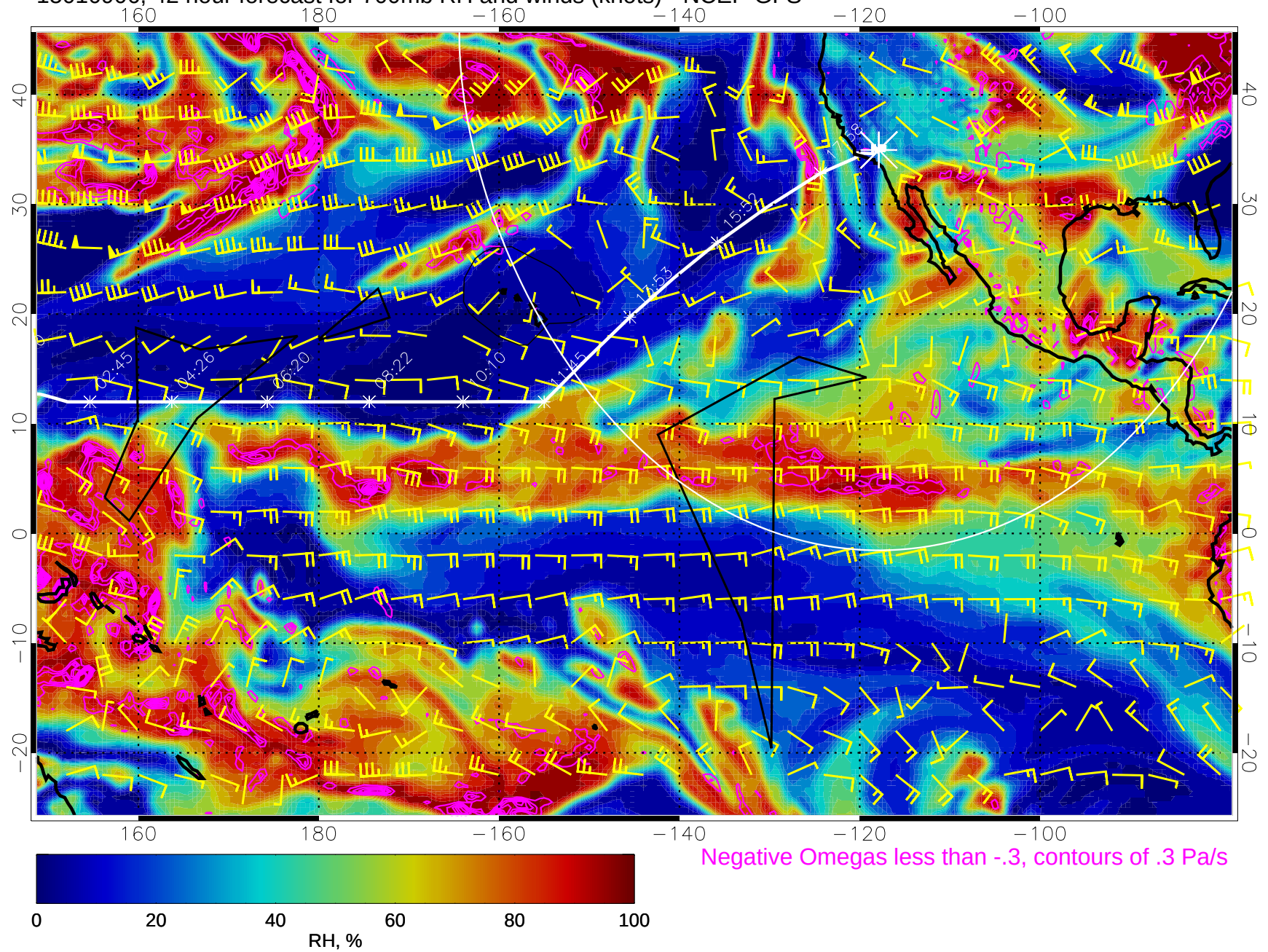
15010906, 42 hour forecast for 700mb RH and winds (knots) - NCEP GFS
