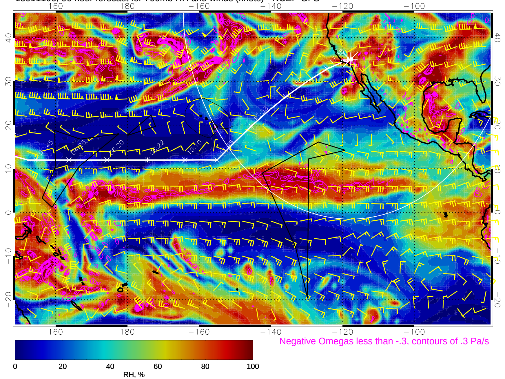
15011106, 90 hour forecast for 700mb RH and winds (knots) - NCEP GFS
