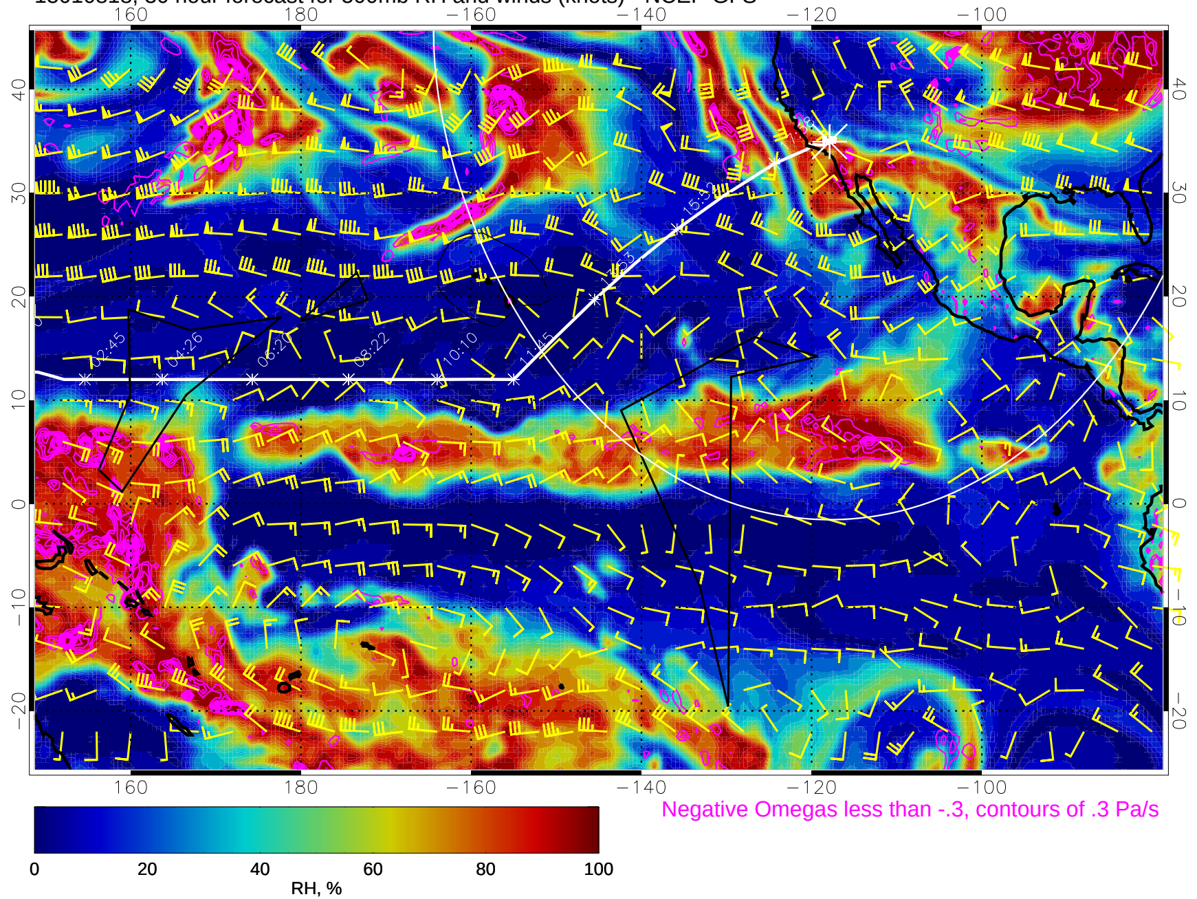
15010818, 30 hour forecast for 500mb RH and winds (knots) - NCEP GFS
