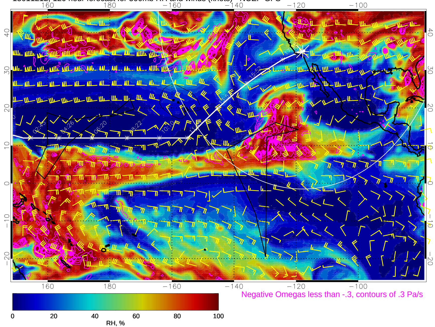
15011212, 120 hour forecast for 500mb RH and winds (knots) - NCEP GFS
