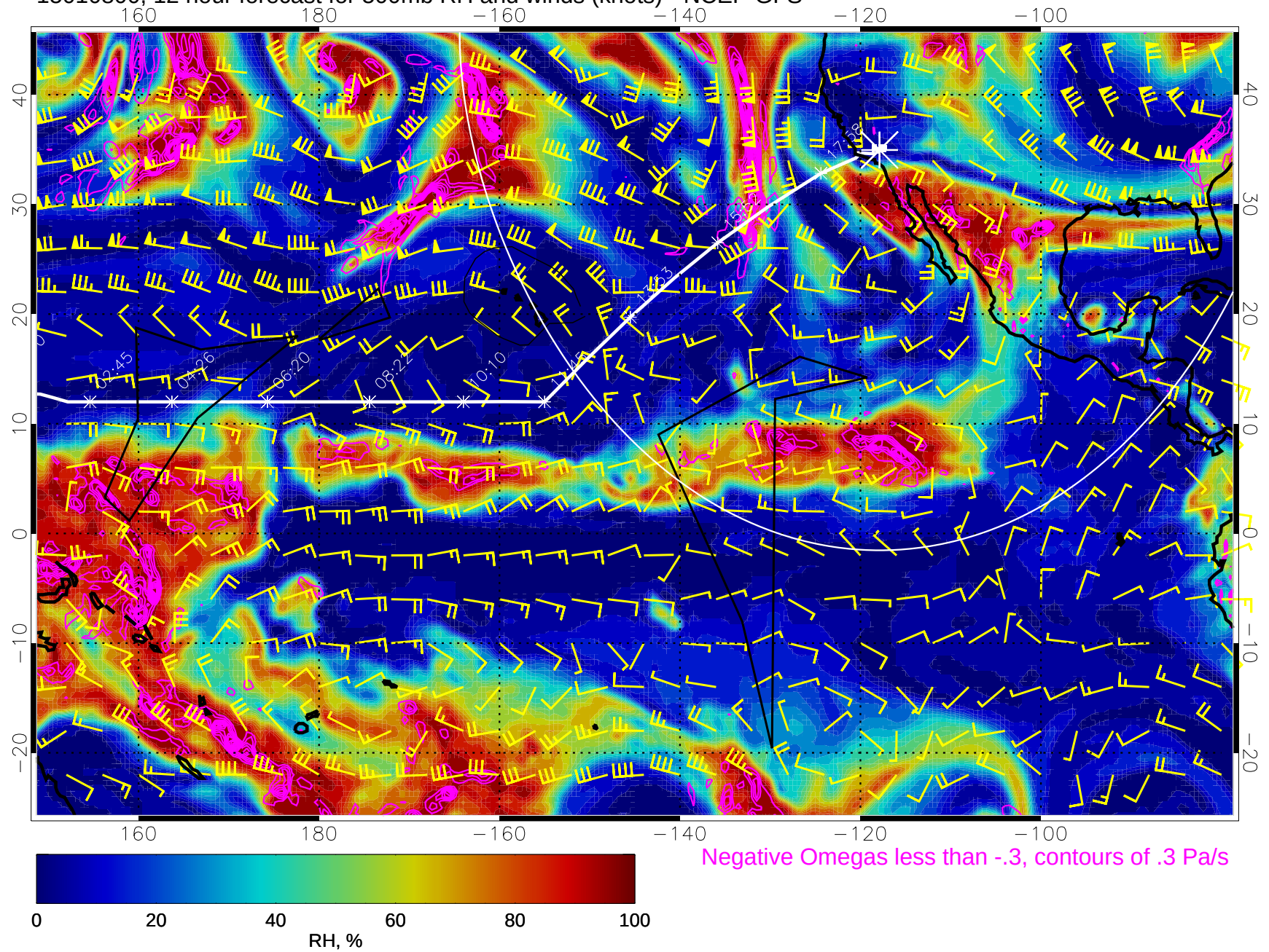
15010800, 12 hour forecast for 500mb RH and winds (knots) - NCEP GFS
