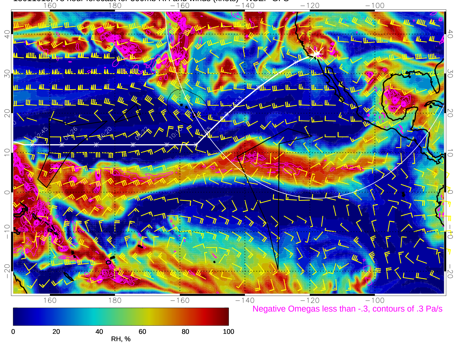
15011018, 78 hour forecast for 500mb RH and winds (knots) - NCEP GFS
