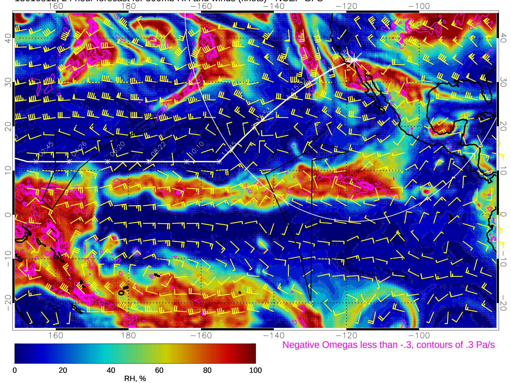
15010812, 24 hour forecast for 500mb RH and winds (knots) - NCEP GFS
