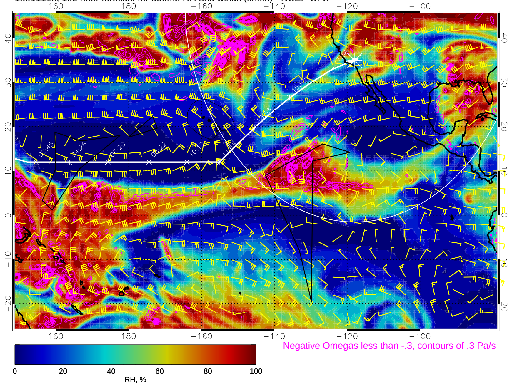
15011118, 102 hour forecast for 500mb RH and winds (knots) - NCEP GFS
