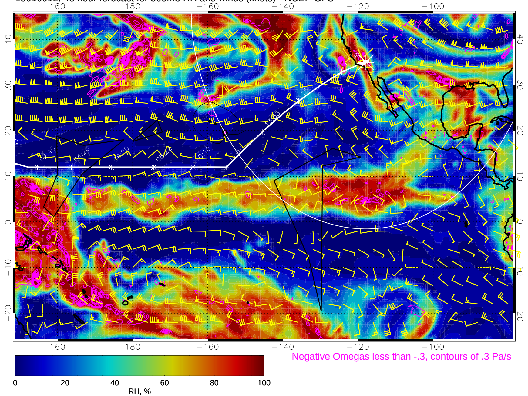
15010912, 48 hour forecast for 500mb RH and winds (knots) - NCEP GFS
