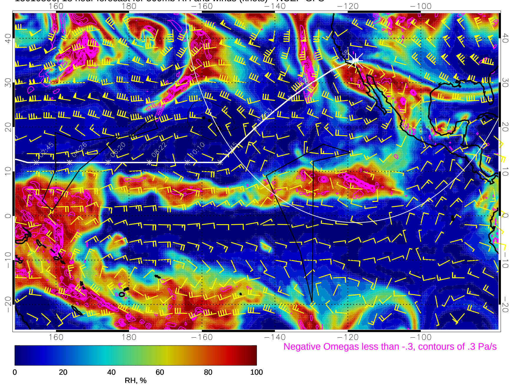
15010806, 18 hour forecast for 500mb RH and winds (knots) - NCEP GFS
