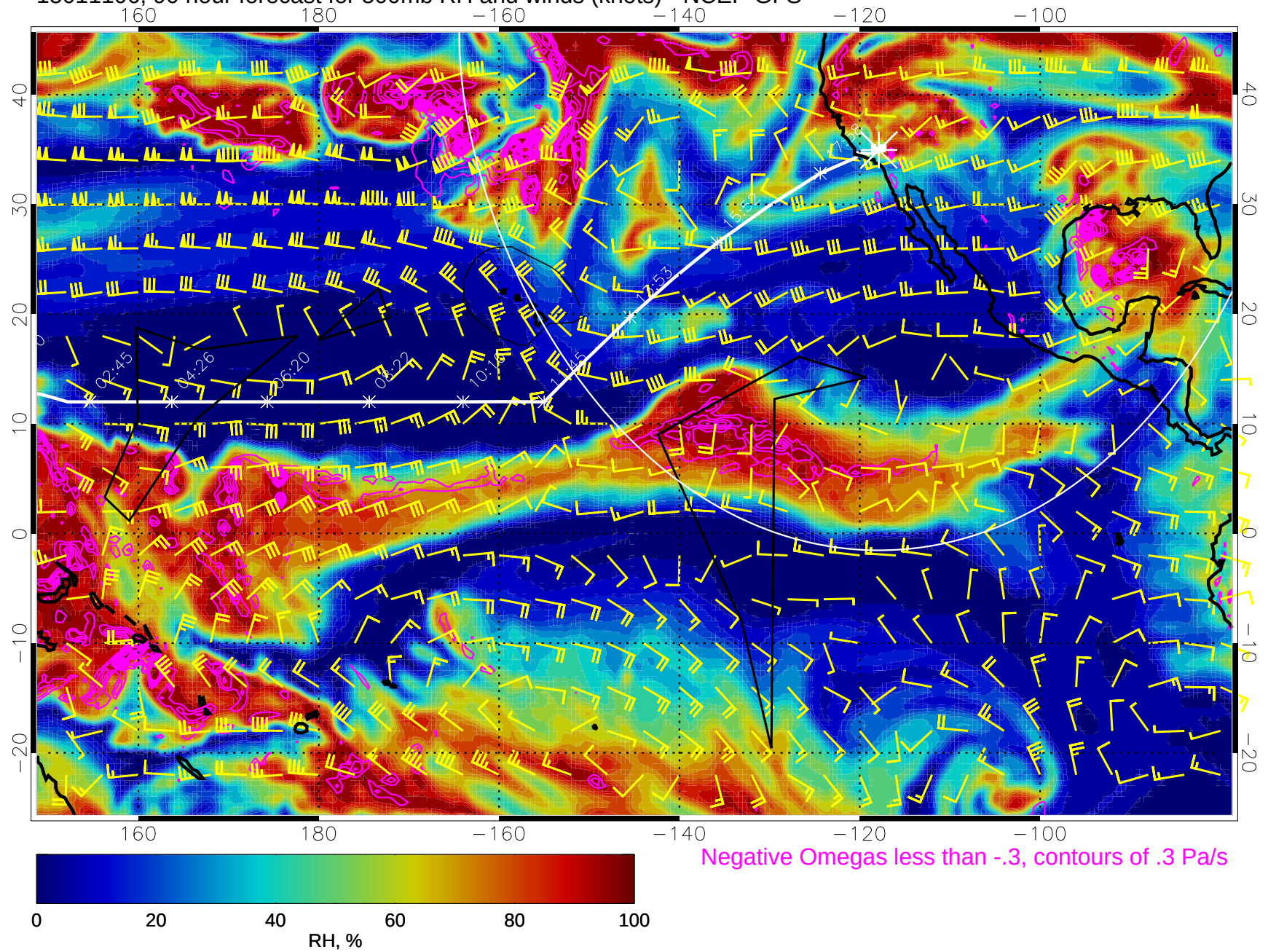
15011106, 90 hour forecast for 500mb RH and winds (knots) - NCEP GFS
