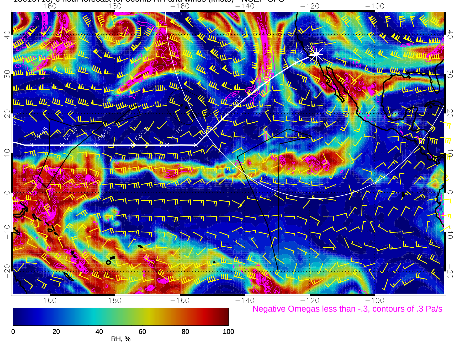
15010718, 6 hour forecast for 500mb RH and winds (knots) - NCEP GFS
