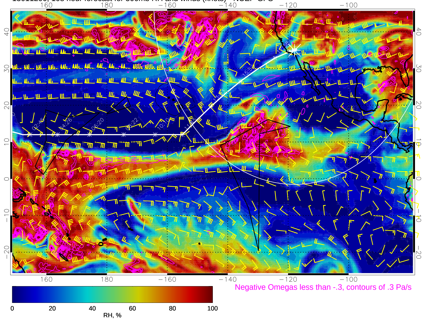
15011200, 108 hour forecast for 500mb RH and winds (knots) - NCEP GFS
