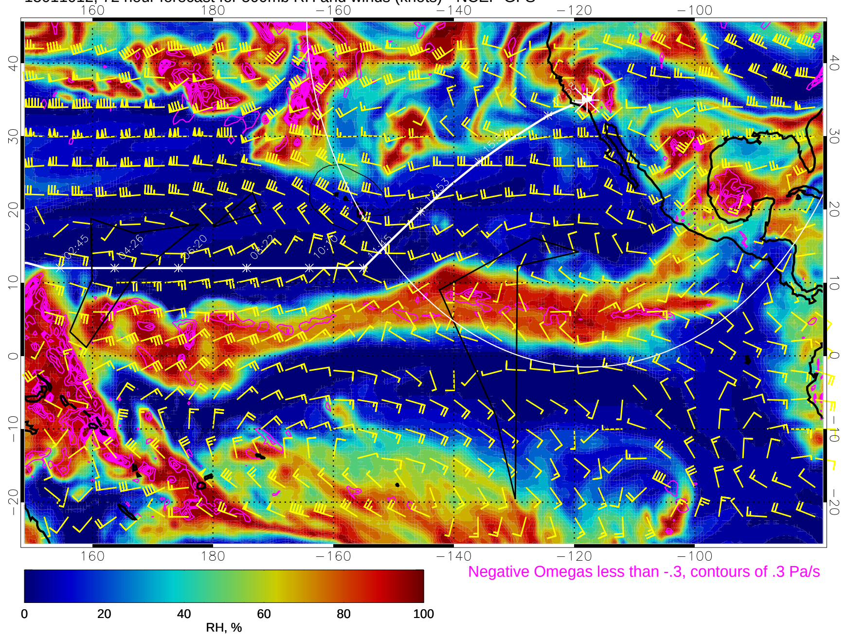
15011012, 72 hour forecast for 500mb RH and winds (knots) - NCEP GFS
