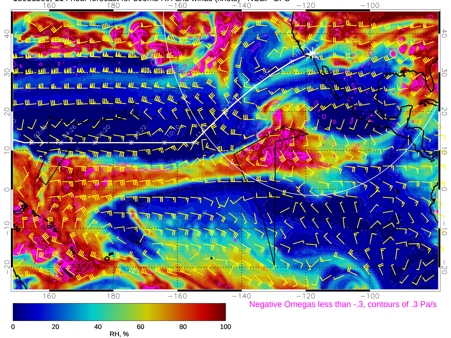
15011206, 114 hour forecast for 500mb RH and winds (knots) - NCEP GFS
