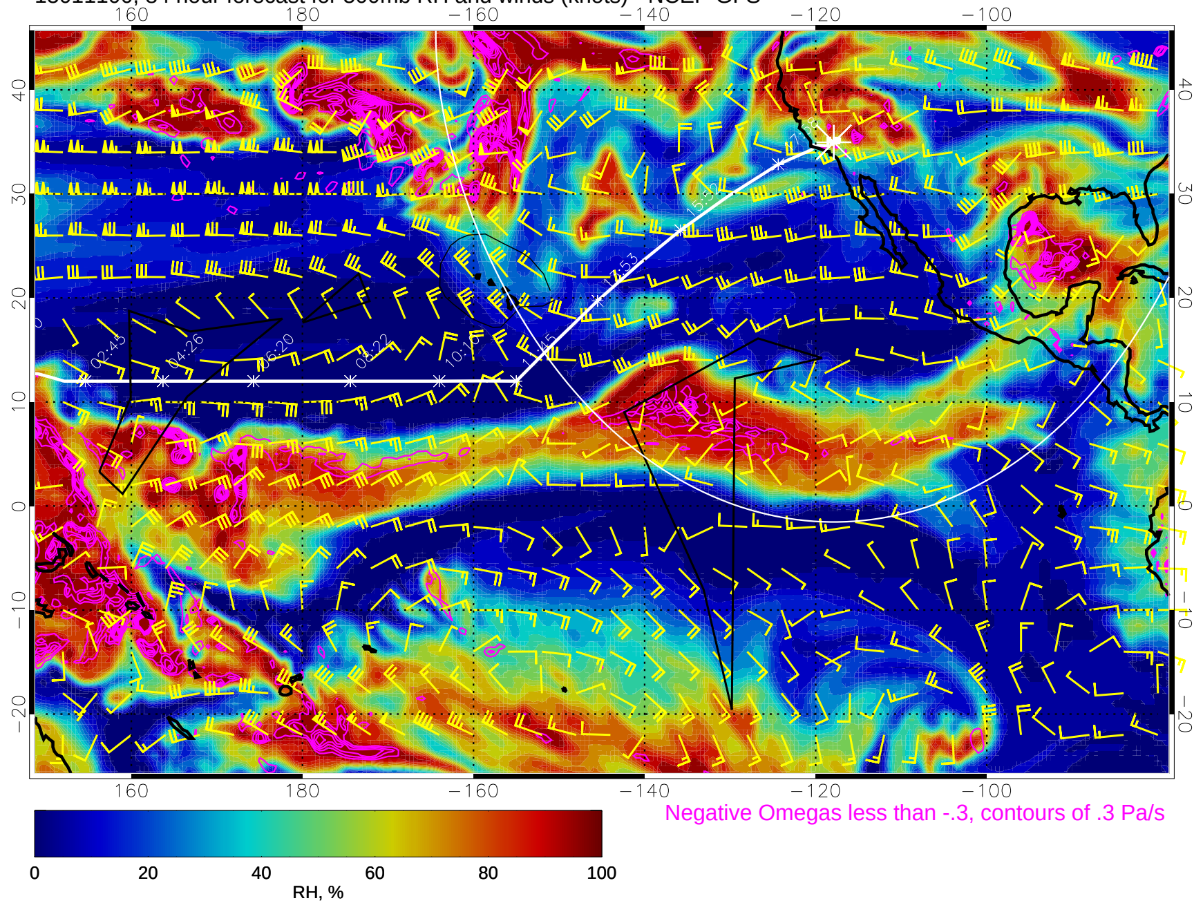
15011100, 84 hour forecast for 500mb RH and winds (knots) - NCEP GFS
