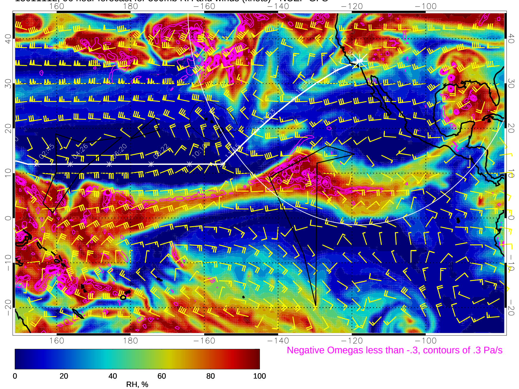
15011112, 96 hour forecast for 500mb RH and winds (knots) - NCEP GFS
