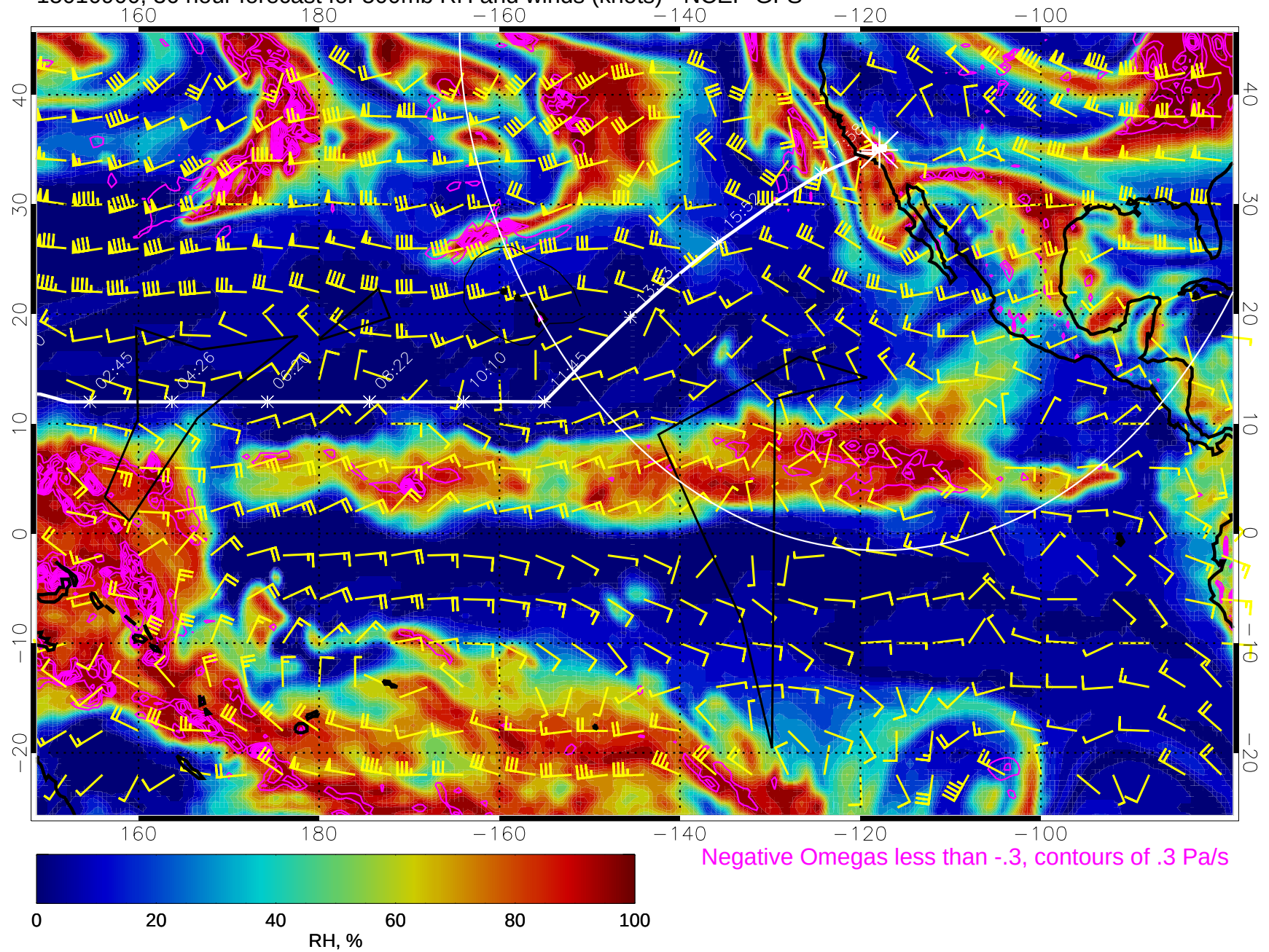
15010900, 36 hour forecast for 500mb RH and winds (knots) - NCEP GFS
