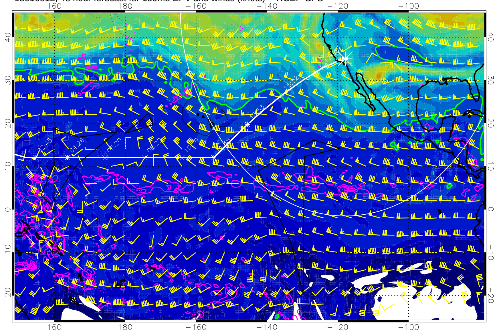
15010912, 48 hour forecast for 150mb EPV and winds (knots) -- NCEP GFS
