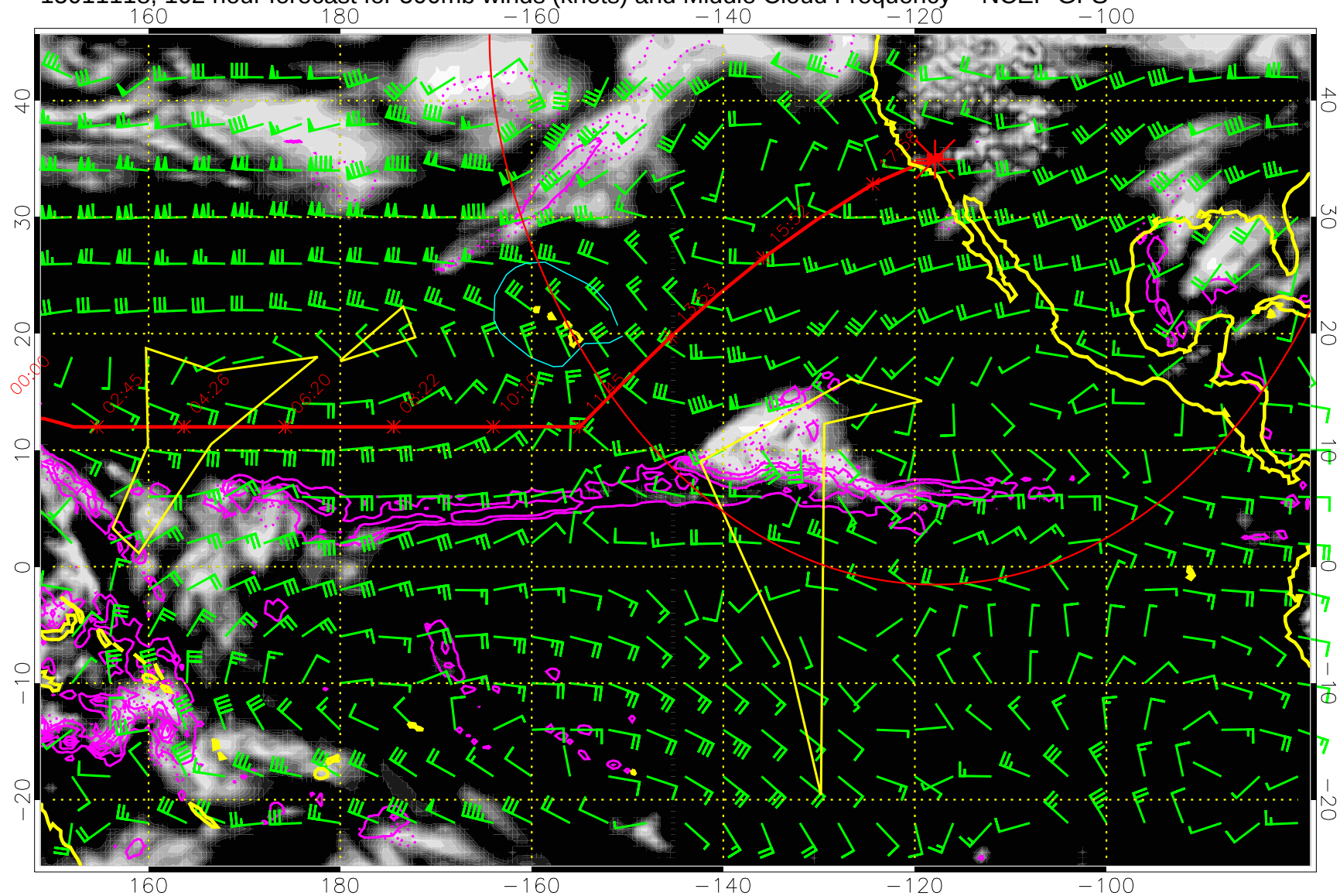
15011118, 102 hour forecast for 500mb winds (knots) and Middle Cloud Frequency -- NCEP GFS
