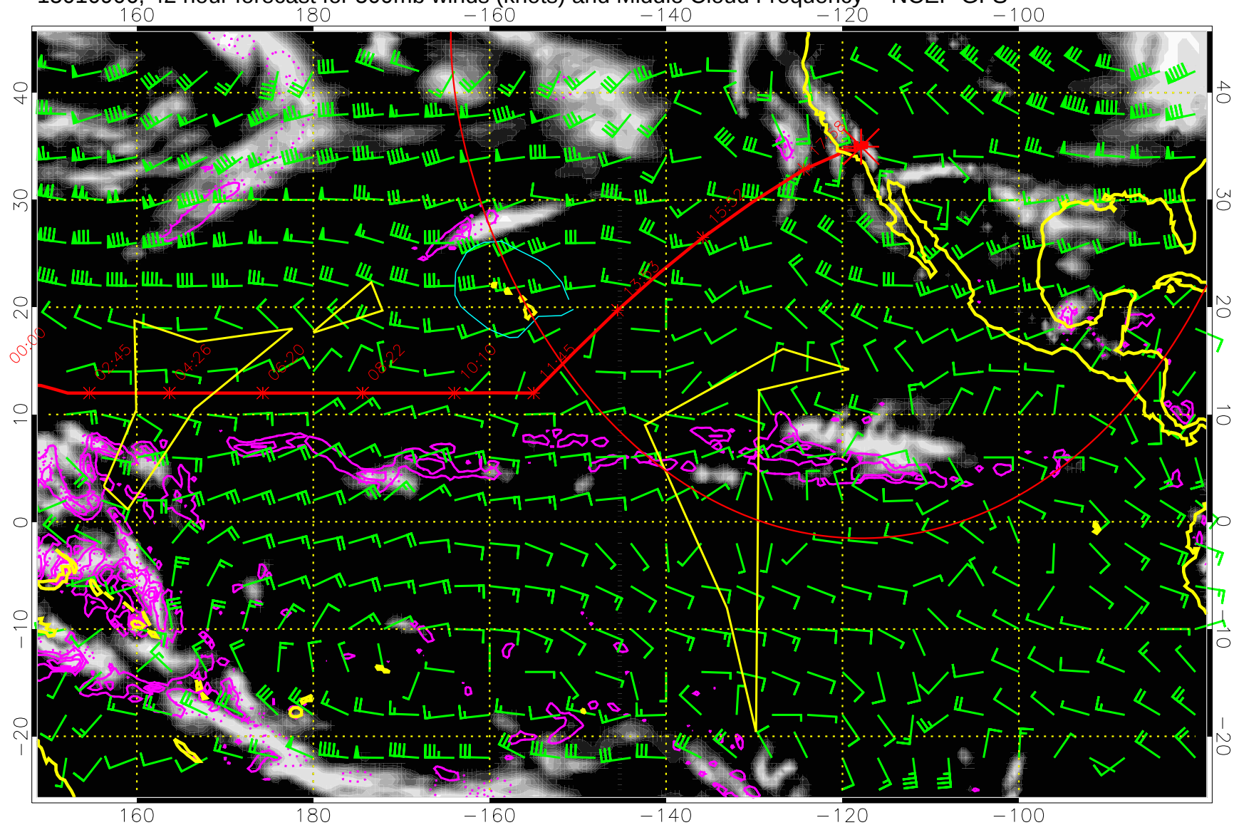
15010906, 42 hour forecast for 500mb winds (knots) and Middle Cloud Frequency -- NCEP GFS
