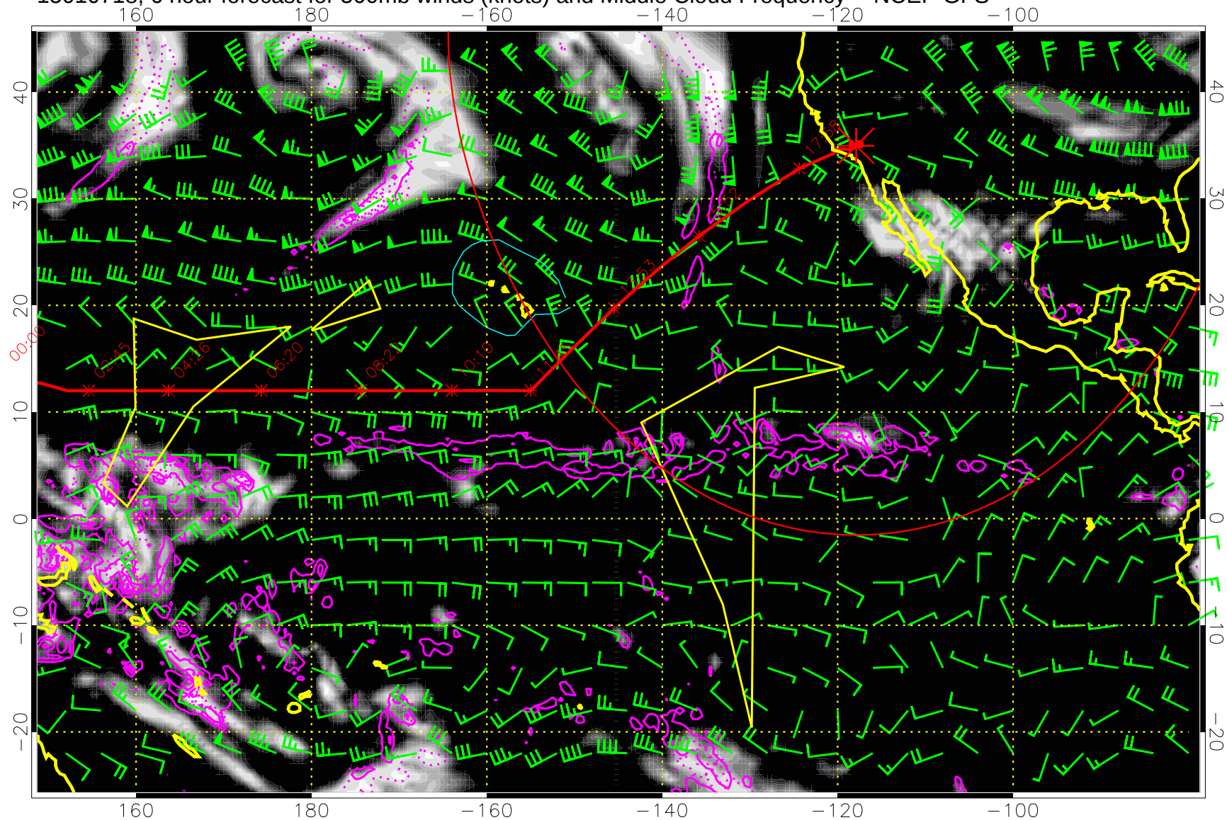
15010718, 6 hour forecast for 500mb winds (knots) and Middle Cloud Frequency -- NCEP GFS
