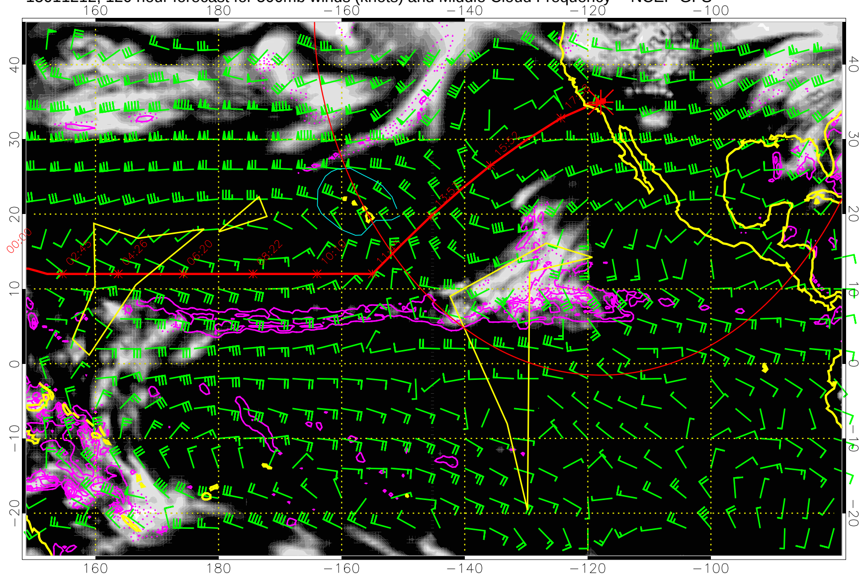
15011212, 120 hour forecast for 500mb winds (knots) and Middle Cloud Frequency -- NCEP GFS
