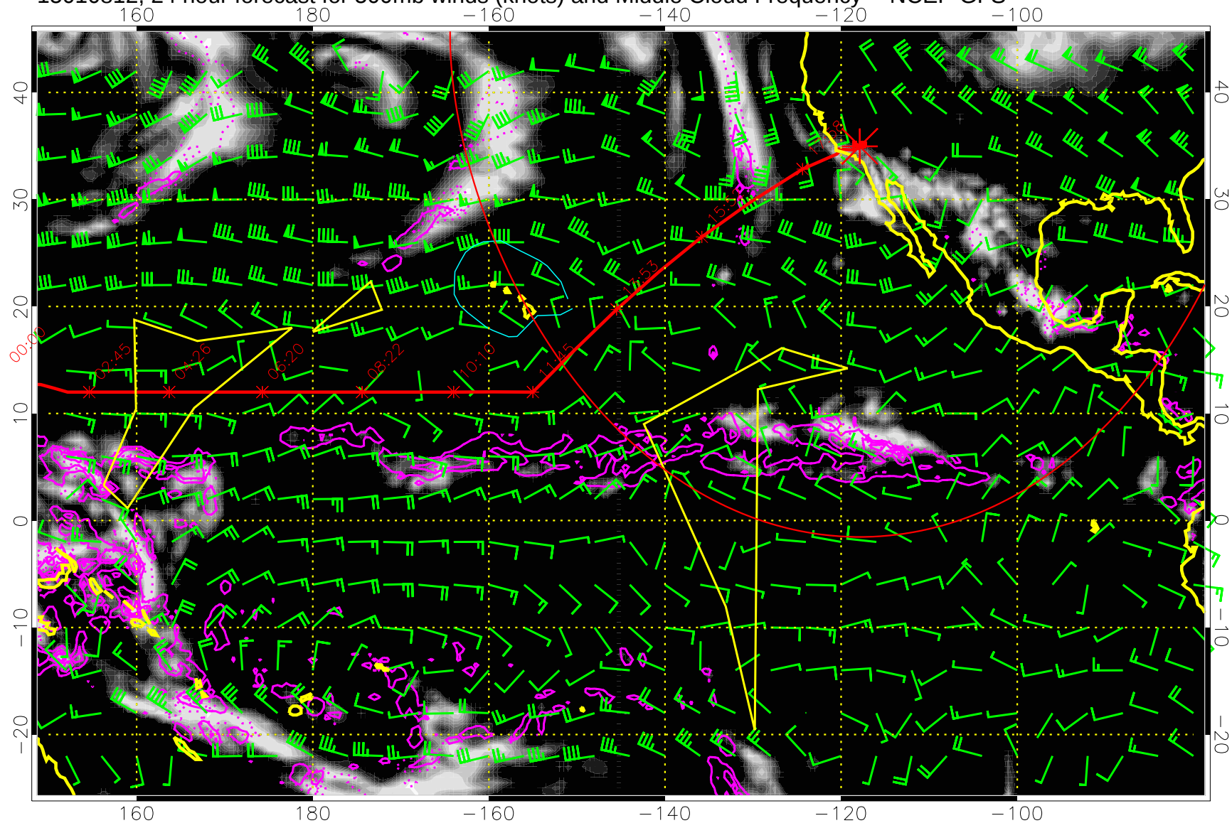
15010812, 24 hour forecast for 500mb winds (knots) and Middle Cloud Frequency -- NCEP GFS
