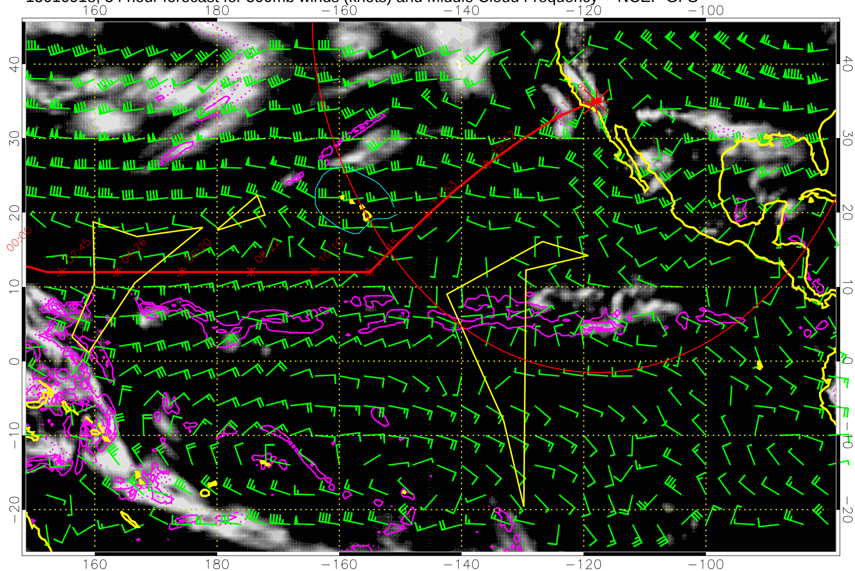
15010918, 54 hour forecast for 500mb winds (knots) and Middle Cloud Frequency -- NCEP GFS
