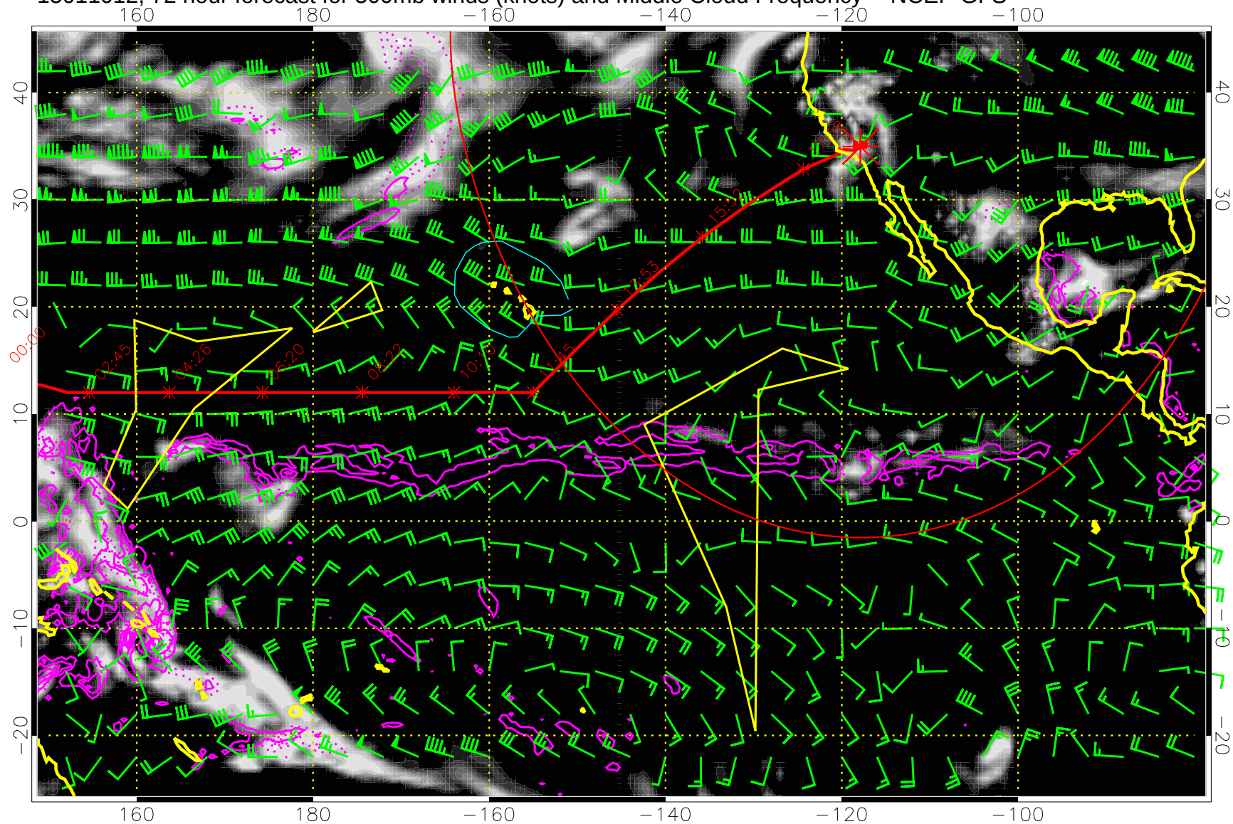
15011012, 72 hour forecast for 500mb winds (knots) and Middle Cloud Frequency -- NCEP GFS
