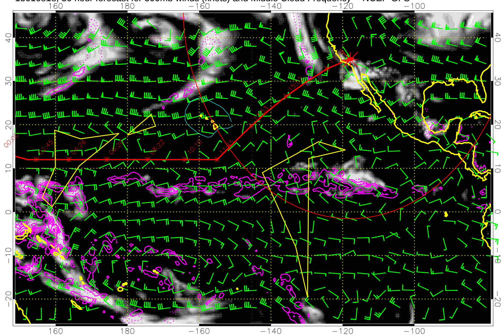
15010818, 30 hour forecast for 500mb winds (knots) and Middle Cloud Frequency -- NCEP GFS
