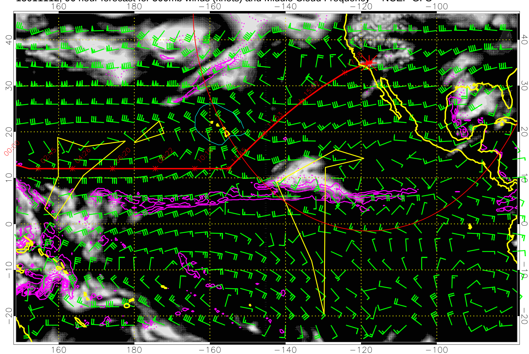
15011112, 96 hour forecast for 500mb winds (knots) and Middle Cloud Frequency -- NCEP GFS
