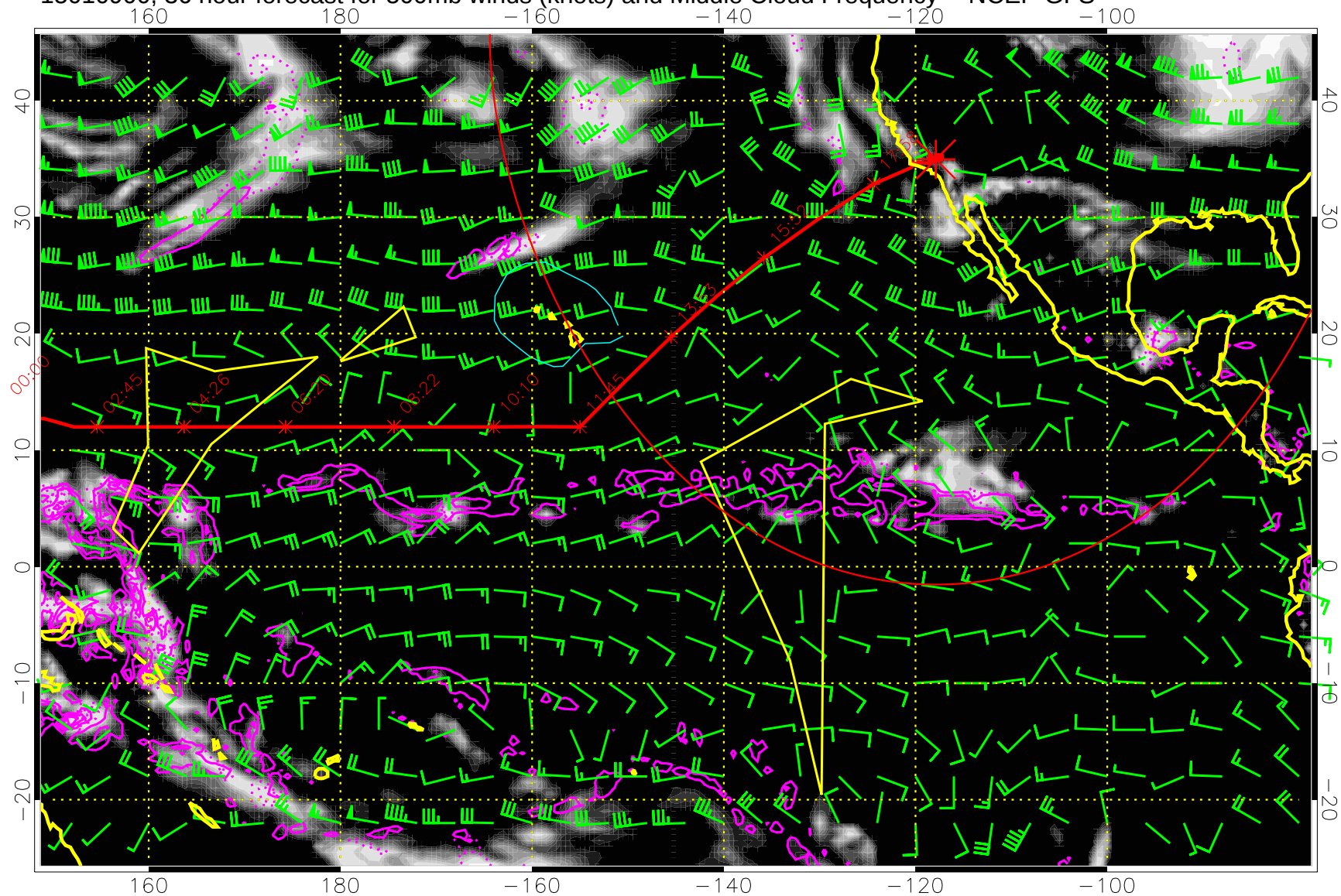
15010900, 36 hour forecast for 500mb winds (knots) and Middle Cloud Frequency -- NCEP GFS
