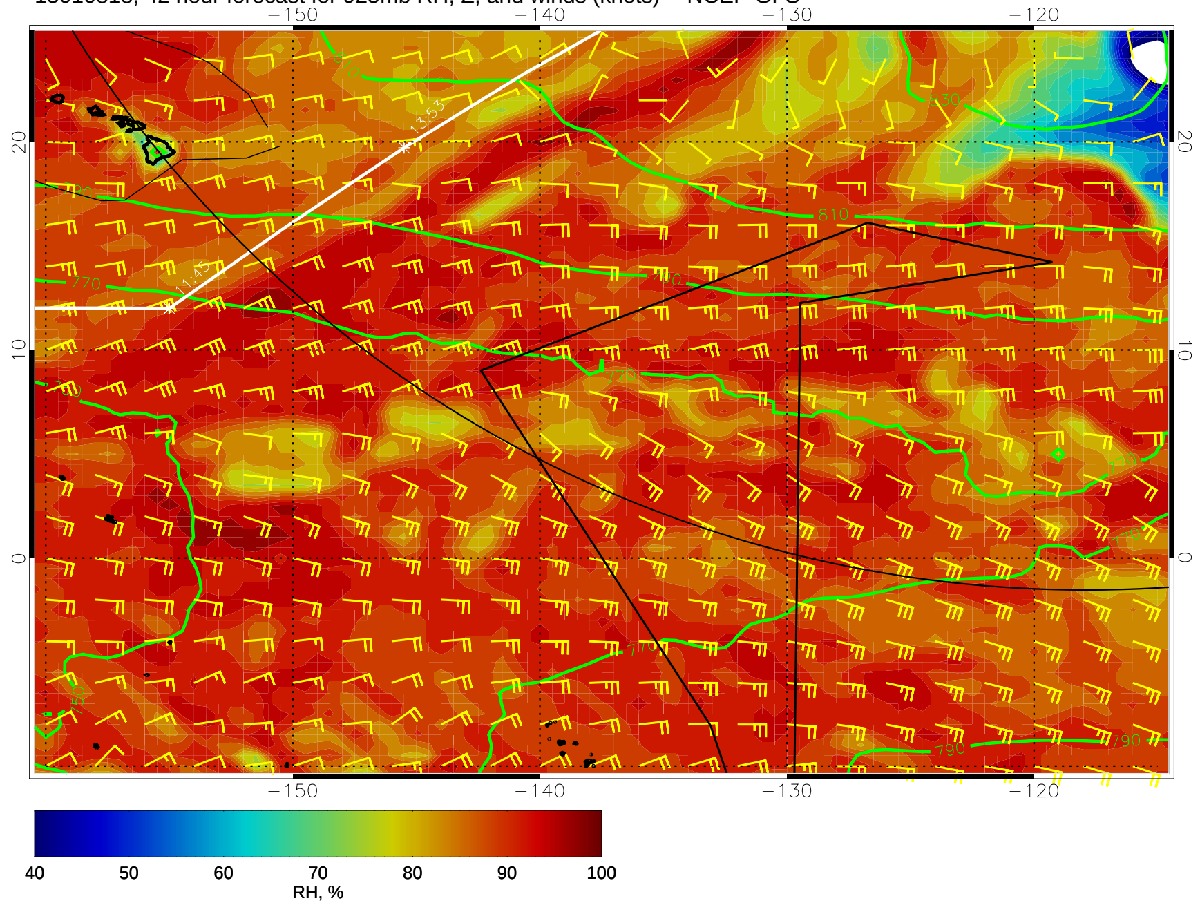
15010818, 42 hour forecast for 925mb RH, Z, and winds (knots) -- NCEP GFS
