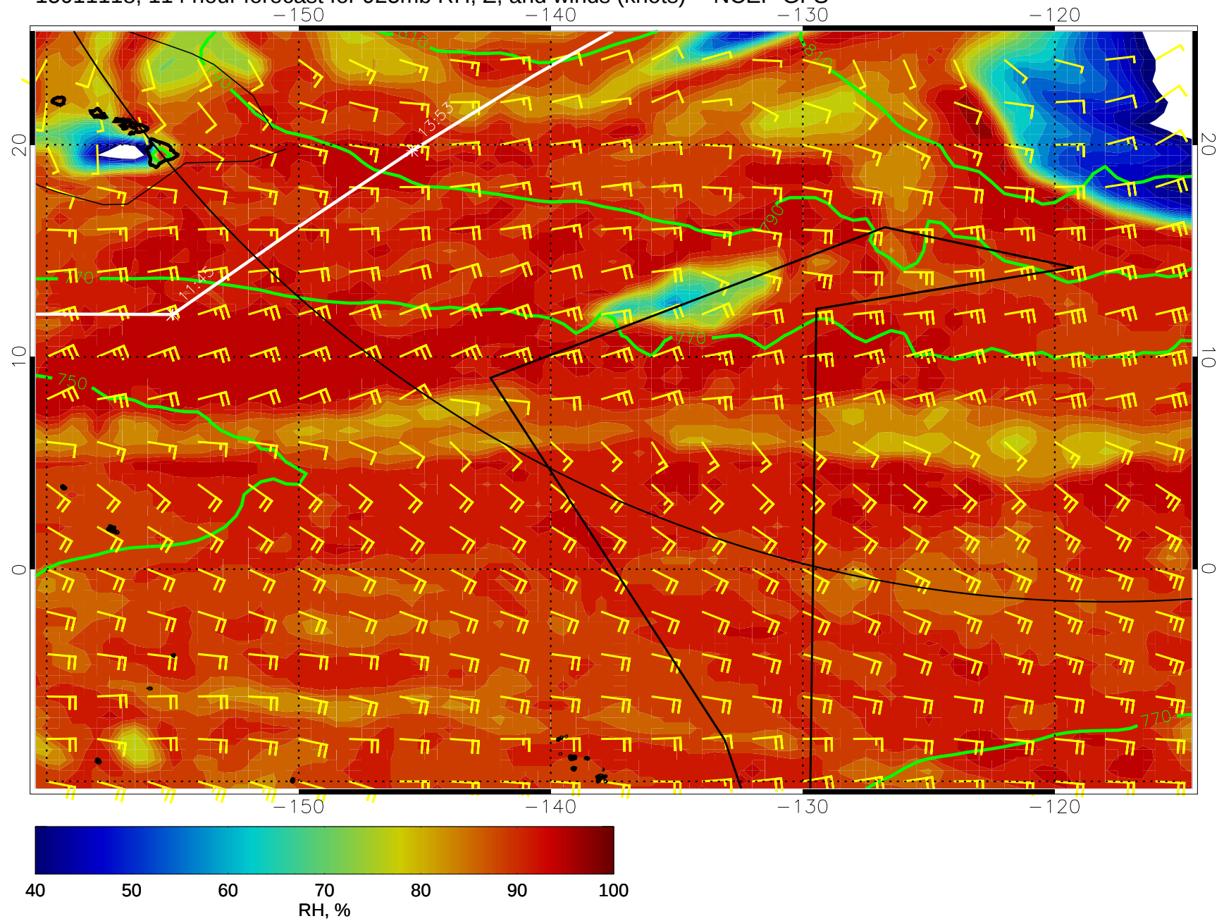
15011118, 114 hour forecast for 925mb RH, Z, and winds (knots) -- NCEP GFS
