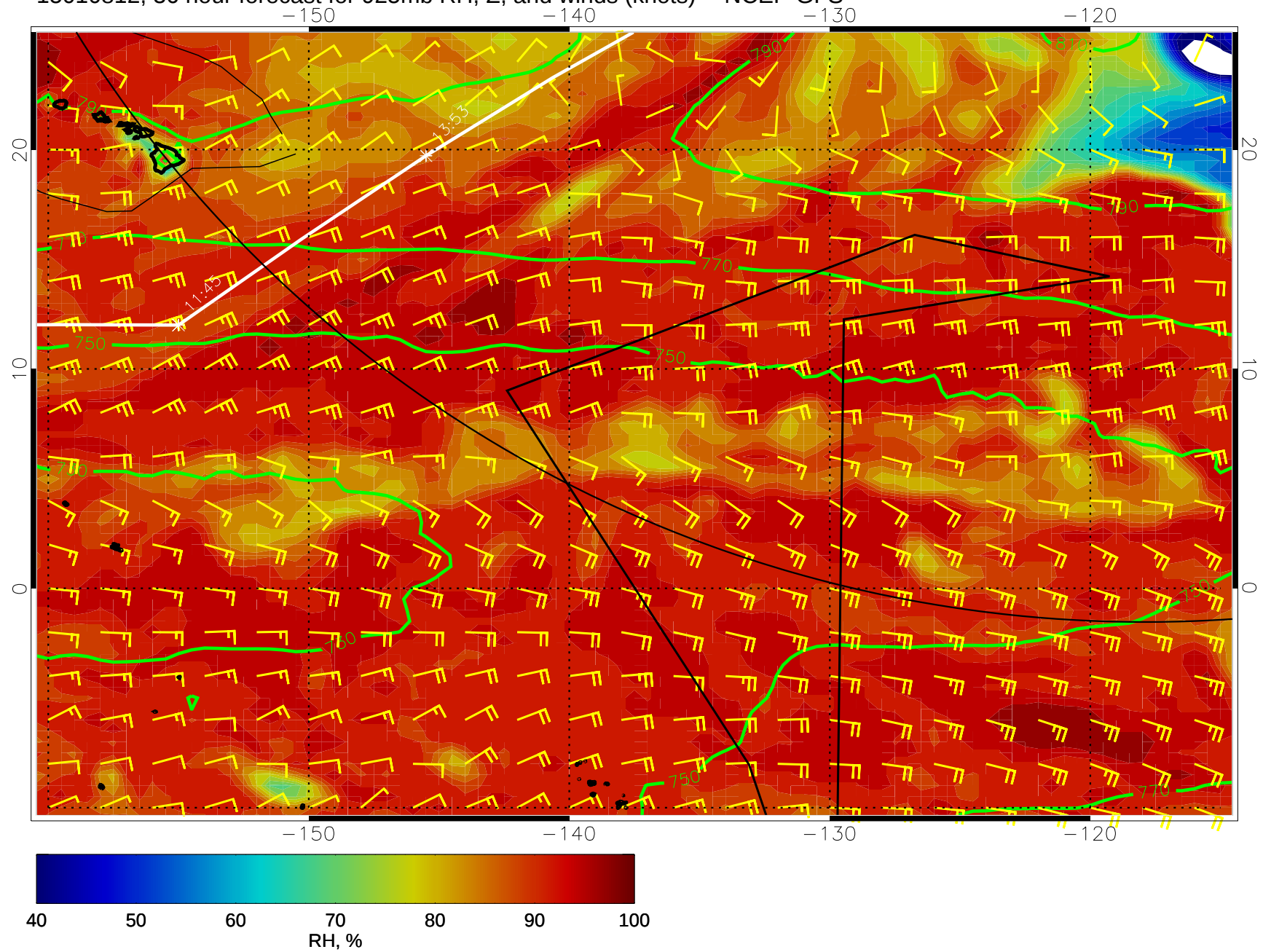
15010812, 36 hour forecast for 925mb RH, Z, and winds (knots) -- NCEP GFS
