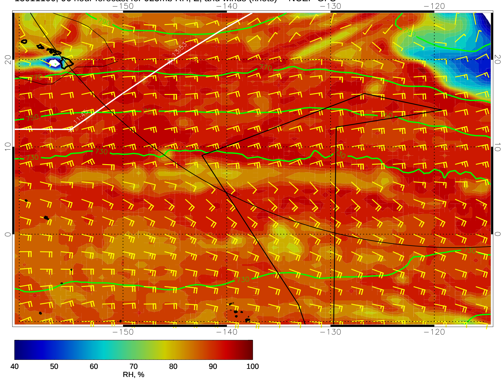
15011100, 96 hour forecast for 925mb RH, Z, and winds (knots) -- NCEP GFS
