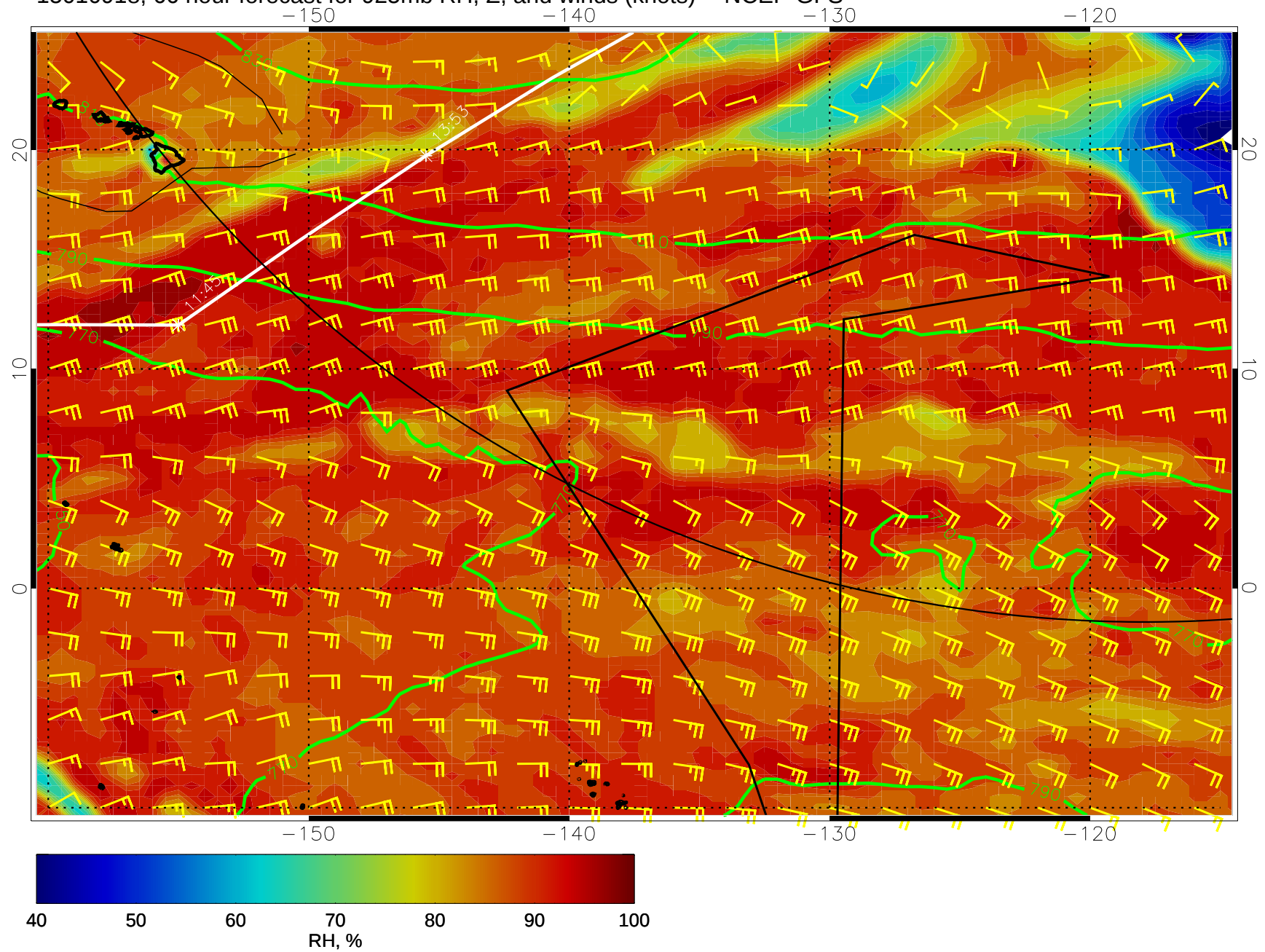
15010918, 66 hour forecast for 925mb RH, Z, and winds (knots) -- NCEP GFS
