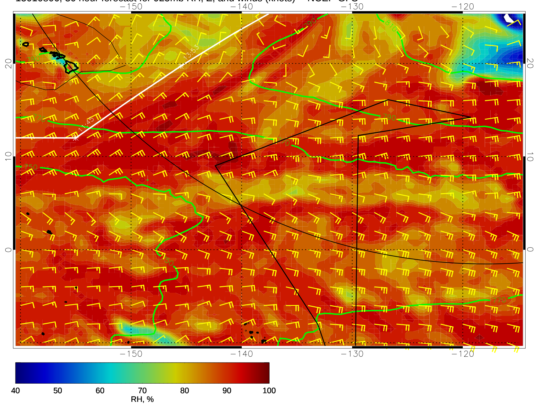
15010806, 30 hour forecast for 925mb RH, Z, and winds (knots) -- NCEP GFS
