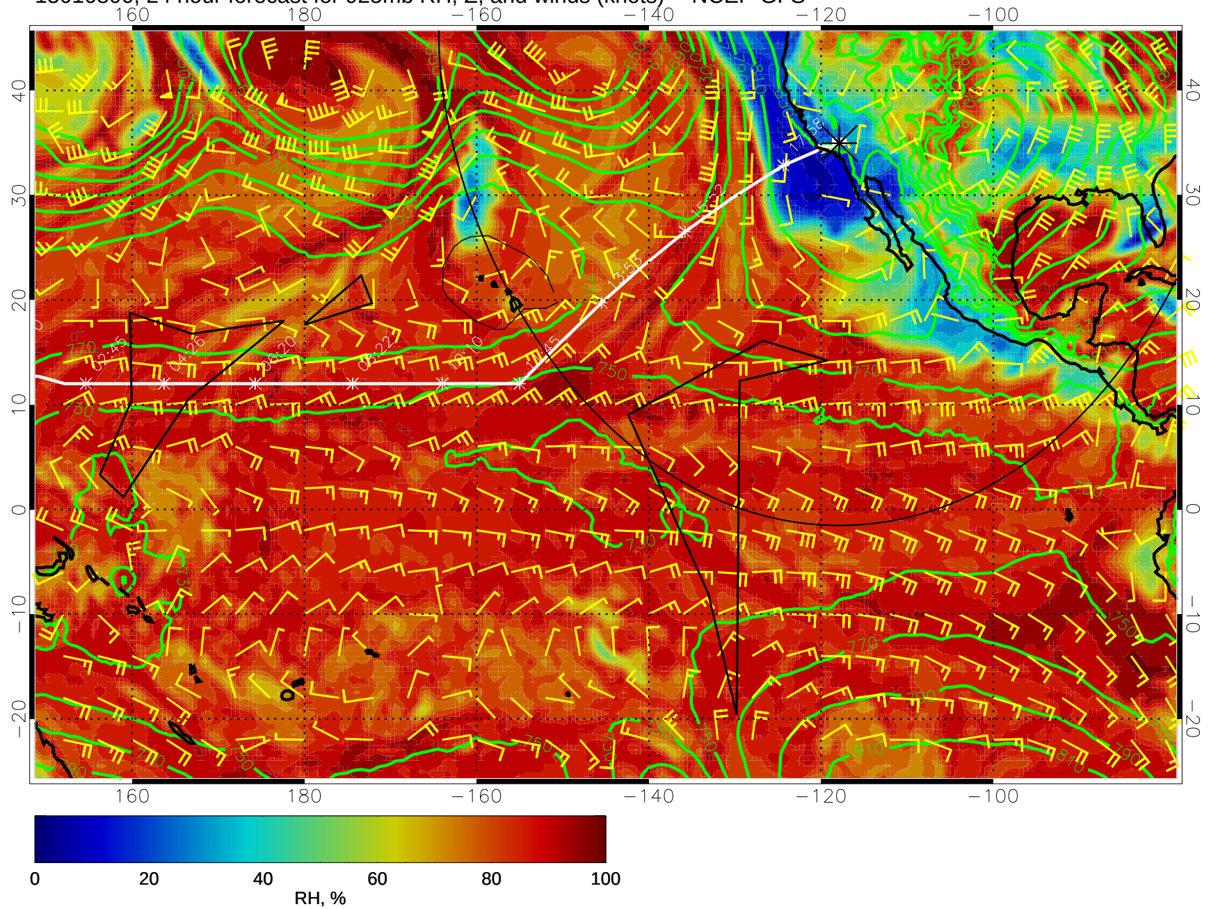
15010800, 24 hour forecast for 925mb RH, Z, and winds (knots) -- NCEP GFS
