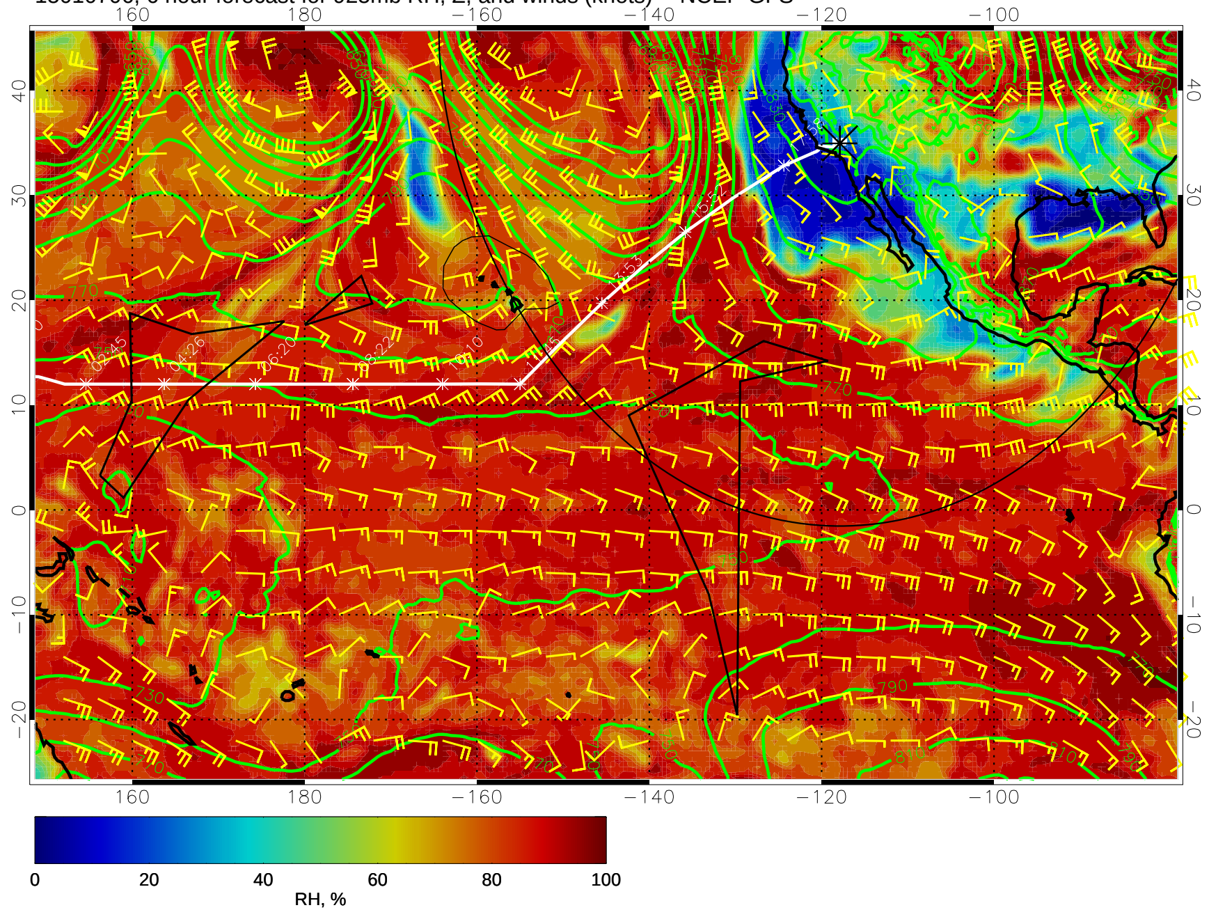
15010706, 6 hour forecast for 925mb RH, Z, and winds (knots) -- NCEP GFS
