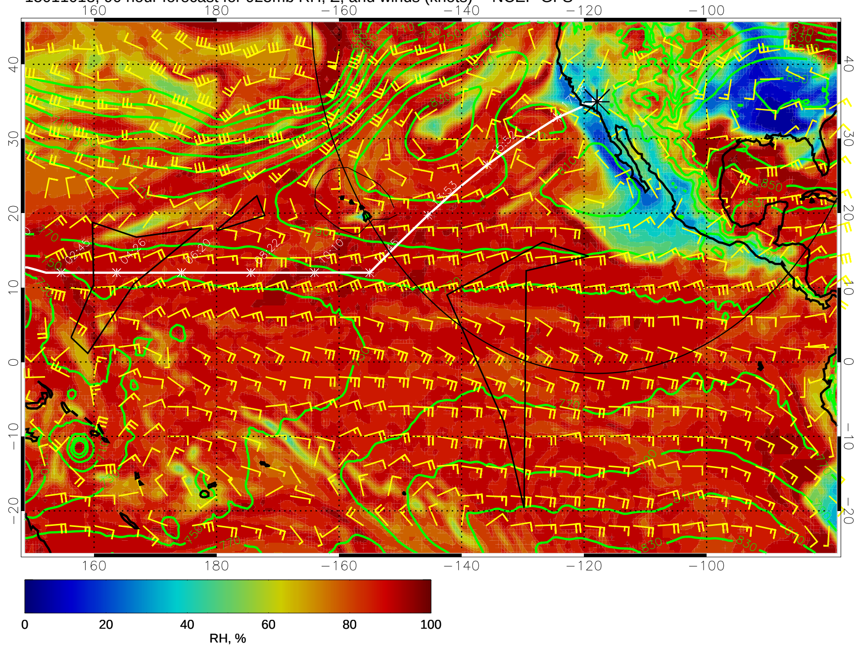
15011018, 90 hour forecast for 925mb RH, Z, and winds (knots) -- NCEP GFS
