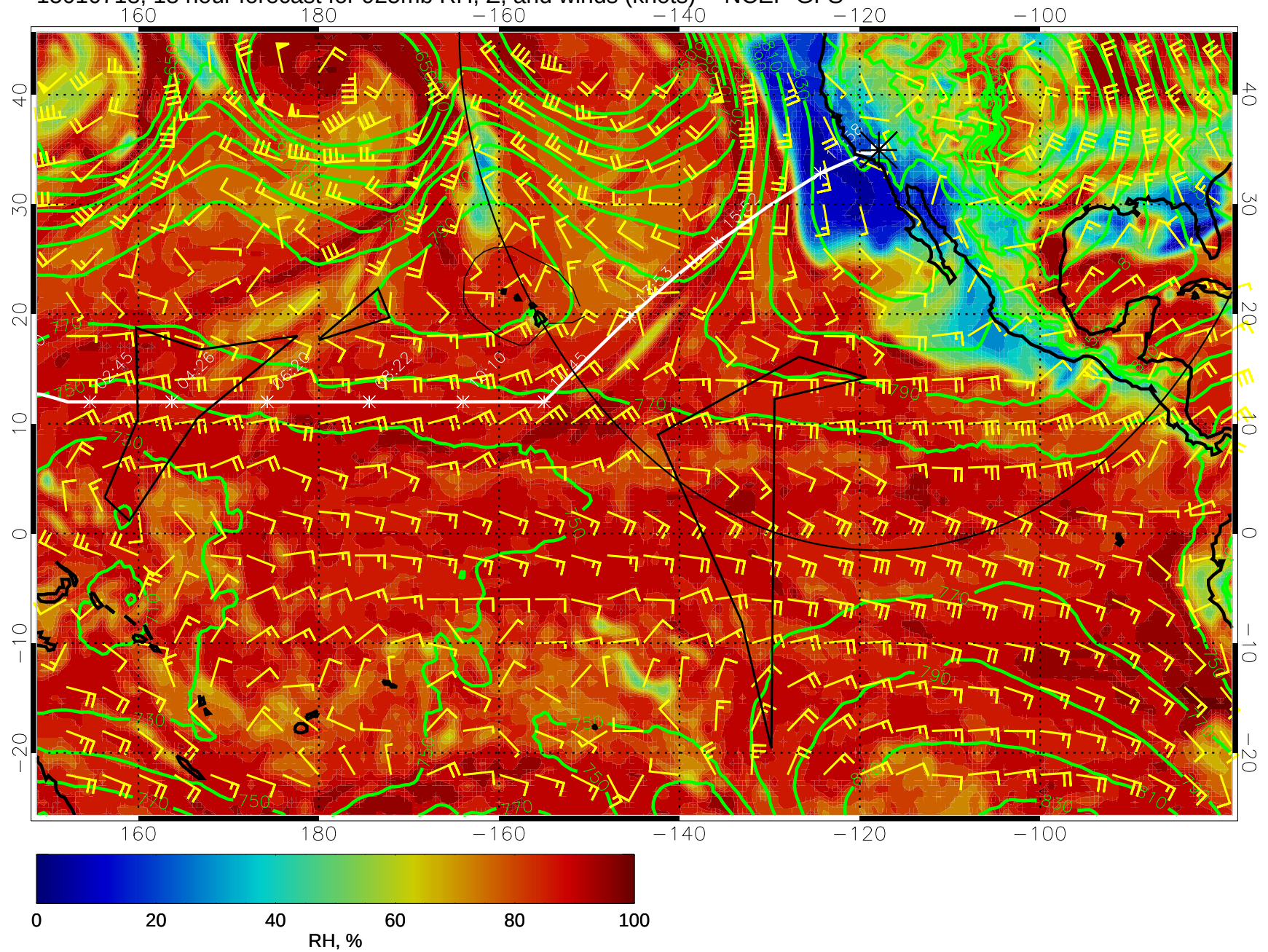
15010718, 18 hour forecast for 925mb RH, Z, and winds (knots) -- NCEP GFS
