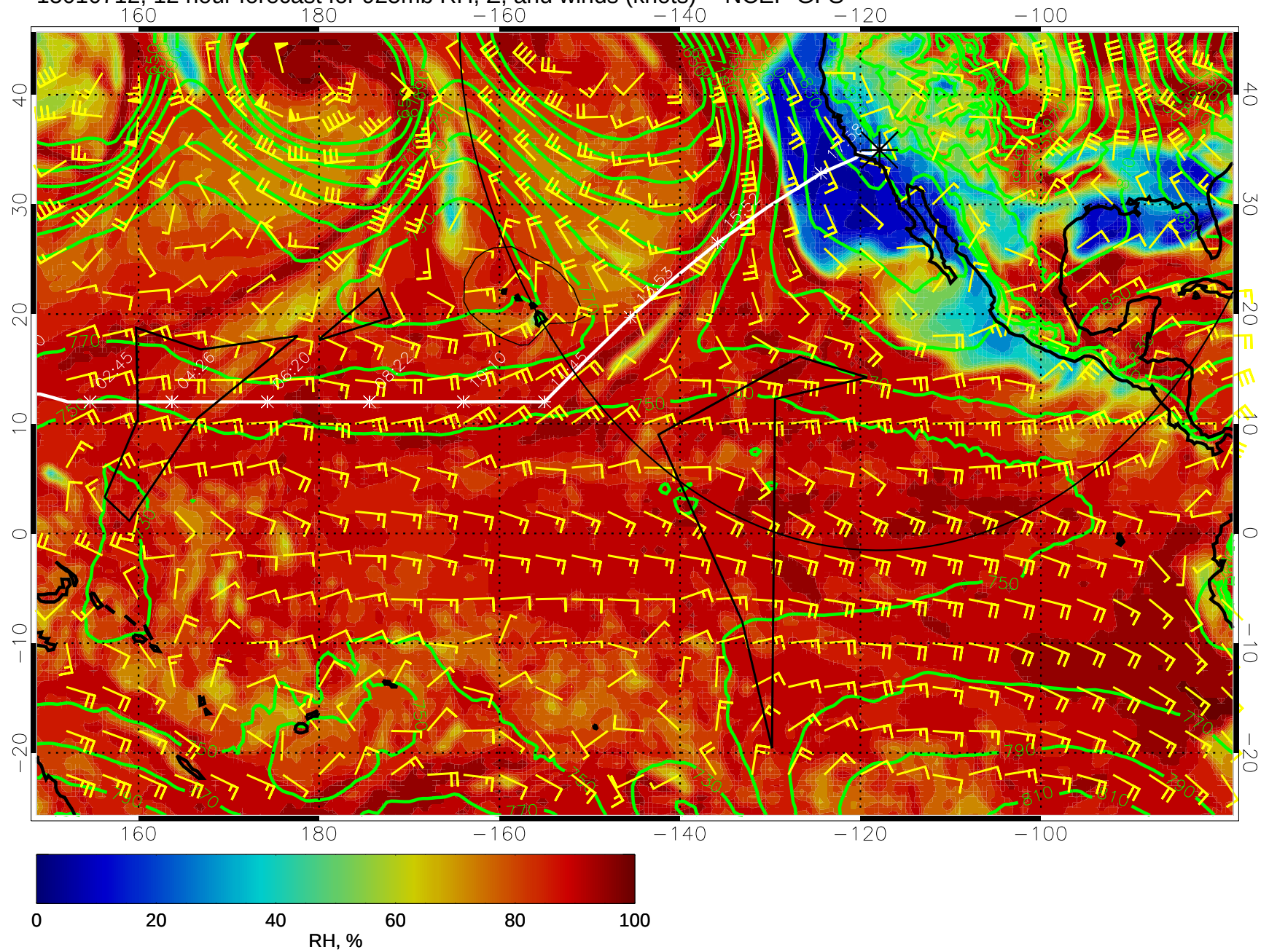
15010712, 12 hour forecast for 925mb RH, Z, and winds (knots) -- NCEP GFS
