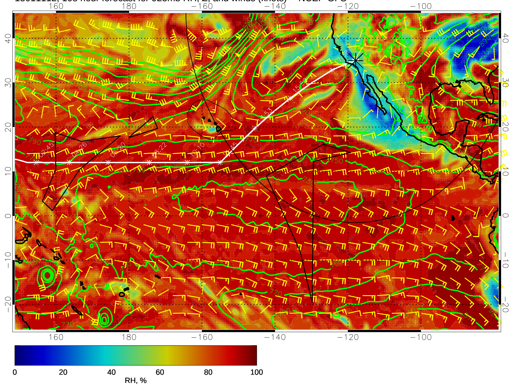
15011112, 108 hour forecast for 925mb RH, Z, and winds (knots) -- NCEP GFS
