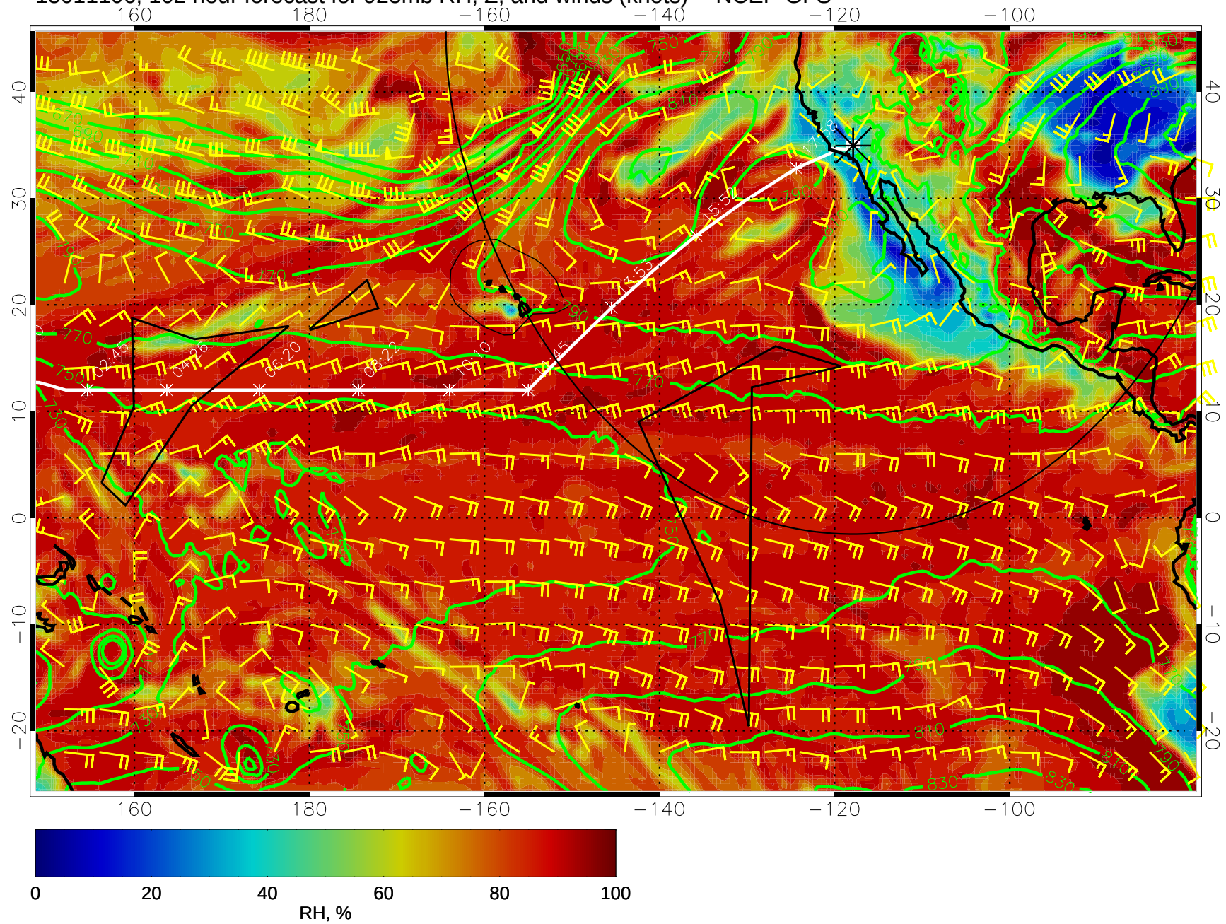
15011106, 102 hour forecast for 925mb RH, Z, and winds (knots) -- NCEP GFS
