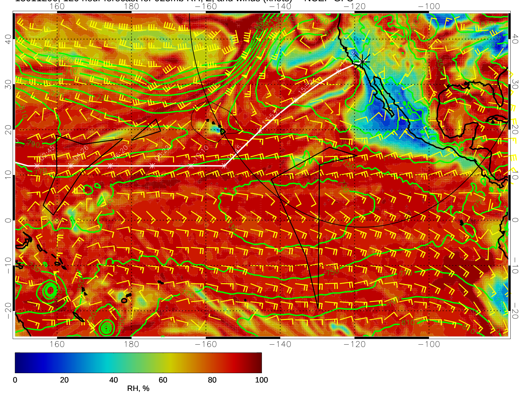
15011200, 120 hour forecast for 925mb RH, Z, and winds (knots) -- NCEP GFS
