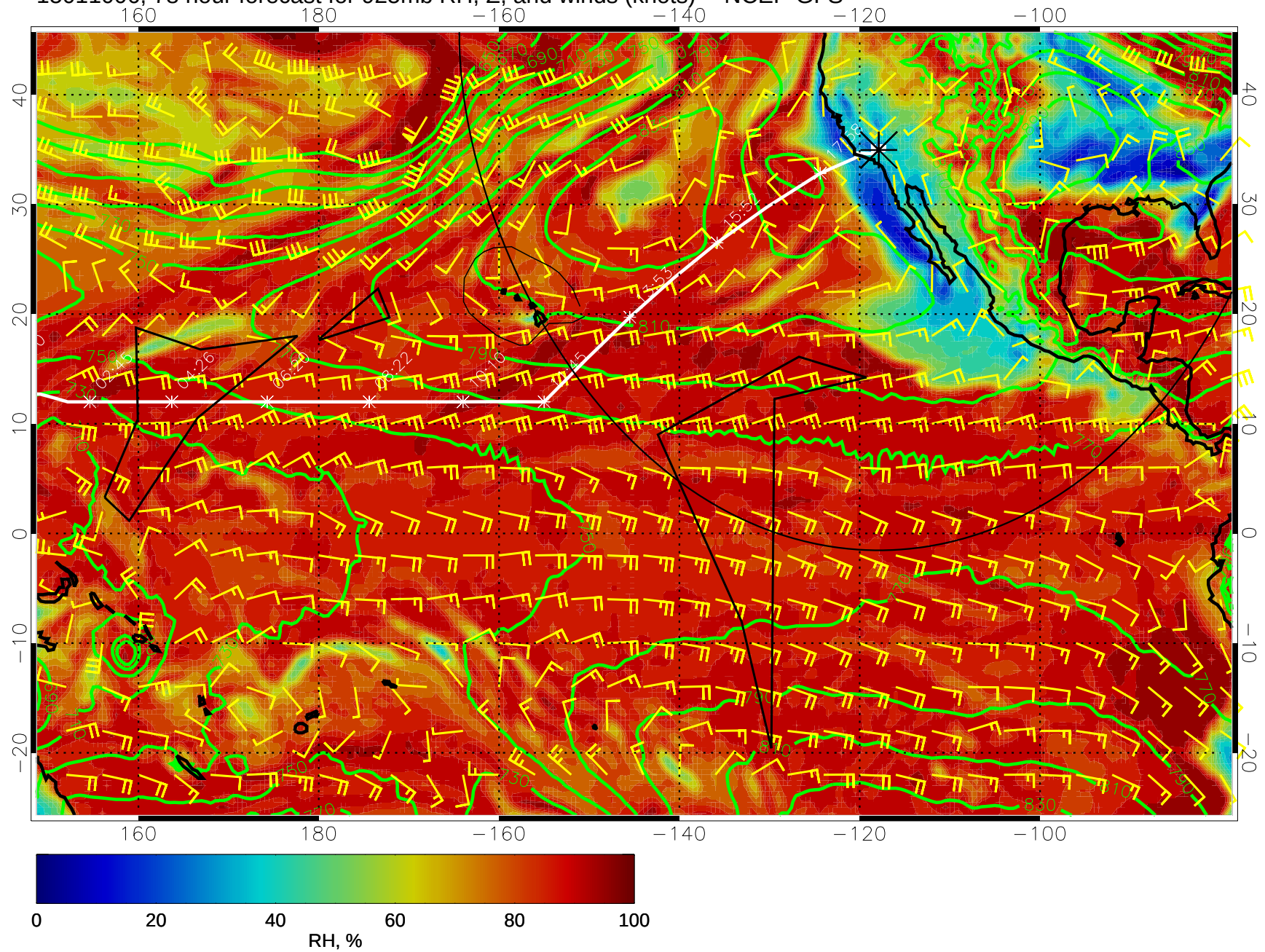
15011006, 78 hour forecast for 925mb RH, Z, and winds (knots) -- NCEP GFS
