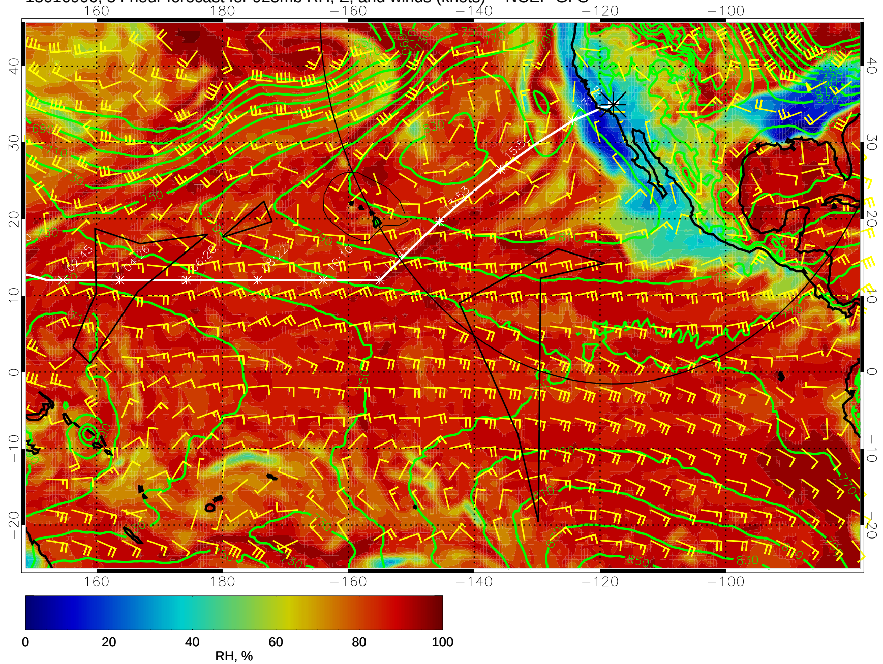
15010906, 54 hour forecast for 925mb RH, Z, and winds (knots) -- NCEP GFS
