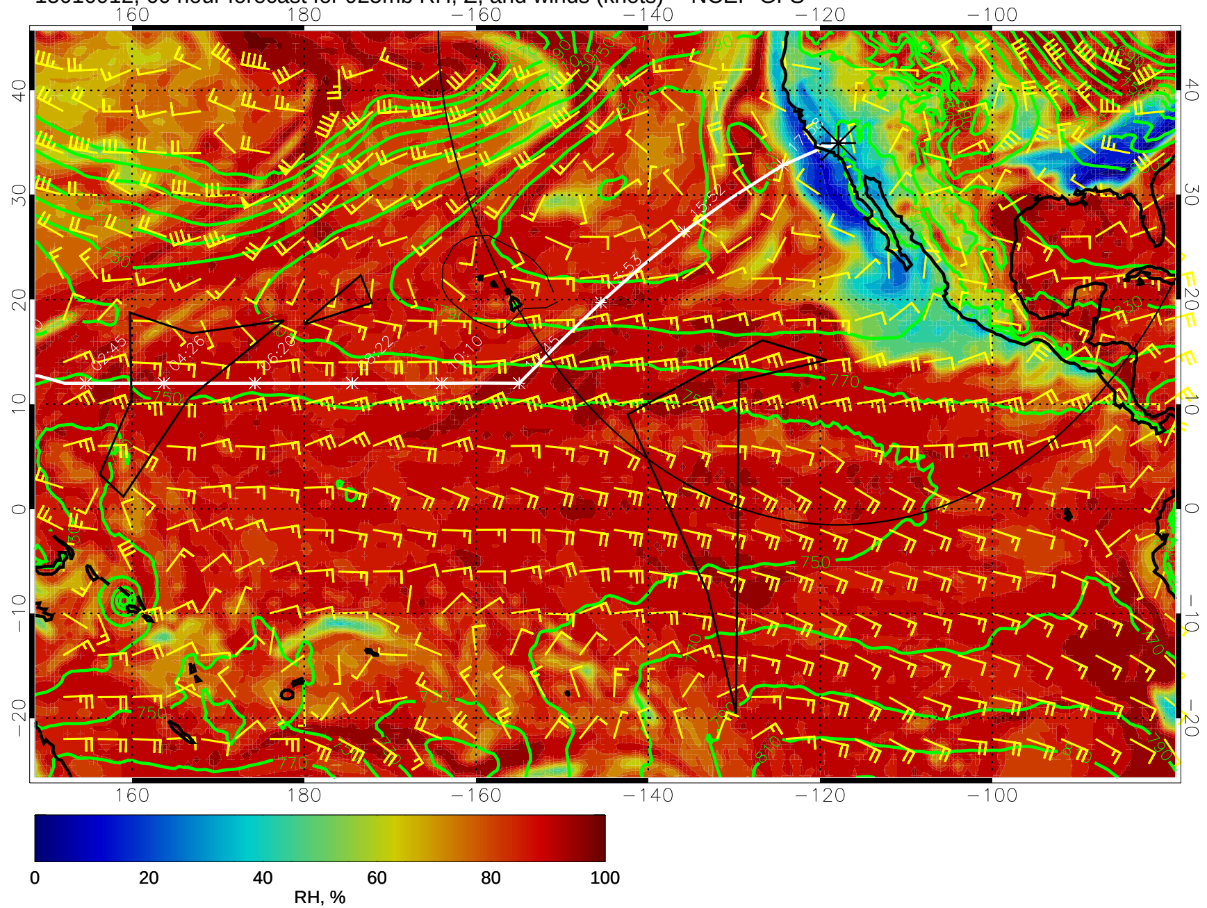
15010912, 60 hour forecast for 925mb RH, Z, and winds (knots) -- NCEP GFS
