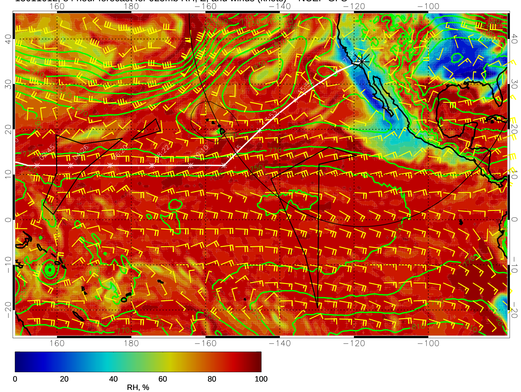
15011012, 84 hour forecast for 925mb RH, Z, and winds (knots) -- NCEP GFS
