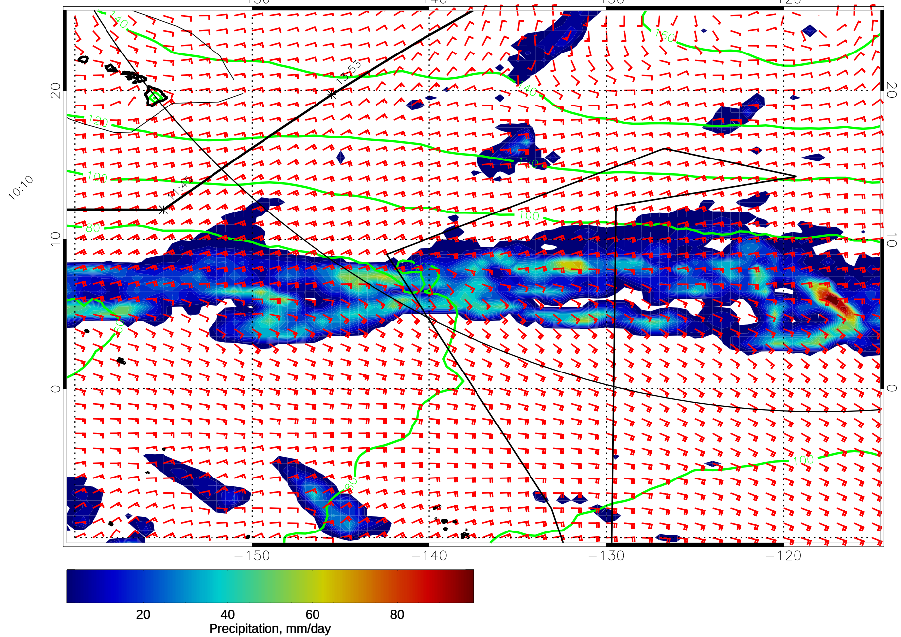
15010818, 42 hour forecast for precip, 1000mb Z, and winds (knots) -- NCEP GFS
