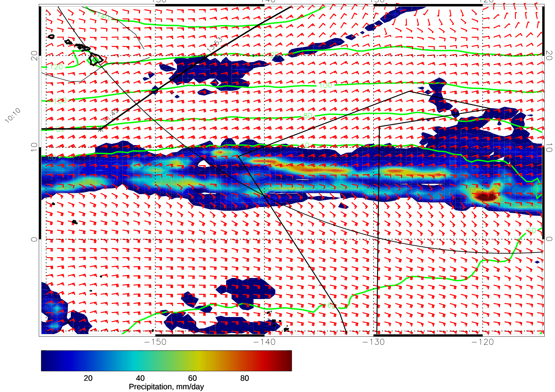
15011012, 84 hour forecast for precip, 1000mb Z, and winds (knots) -- NCEP GFS
