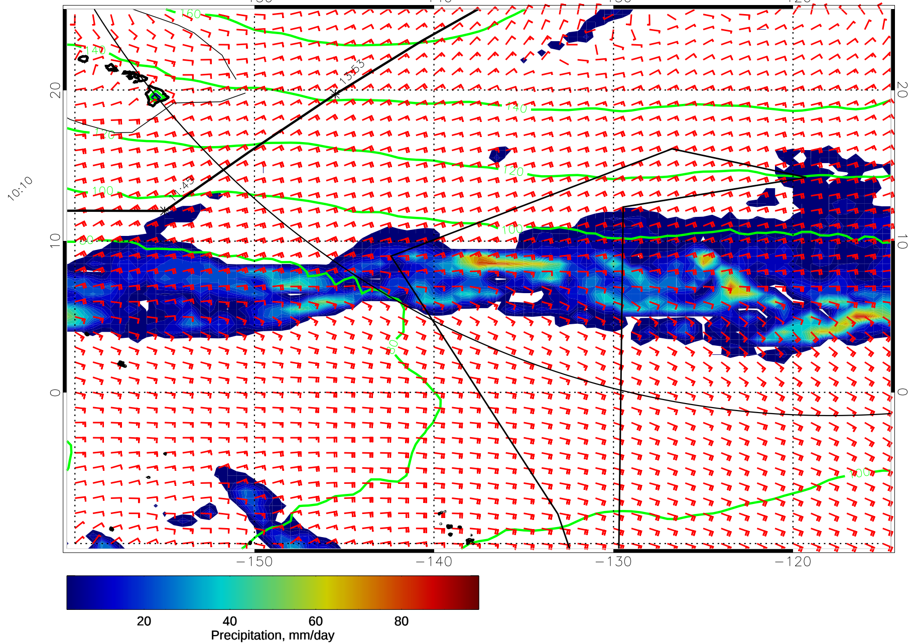
15010906, 54 hour forecast for precip, 1000mb Z, and winds (knots) -- NCEP GFS
