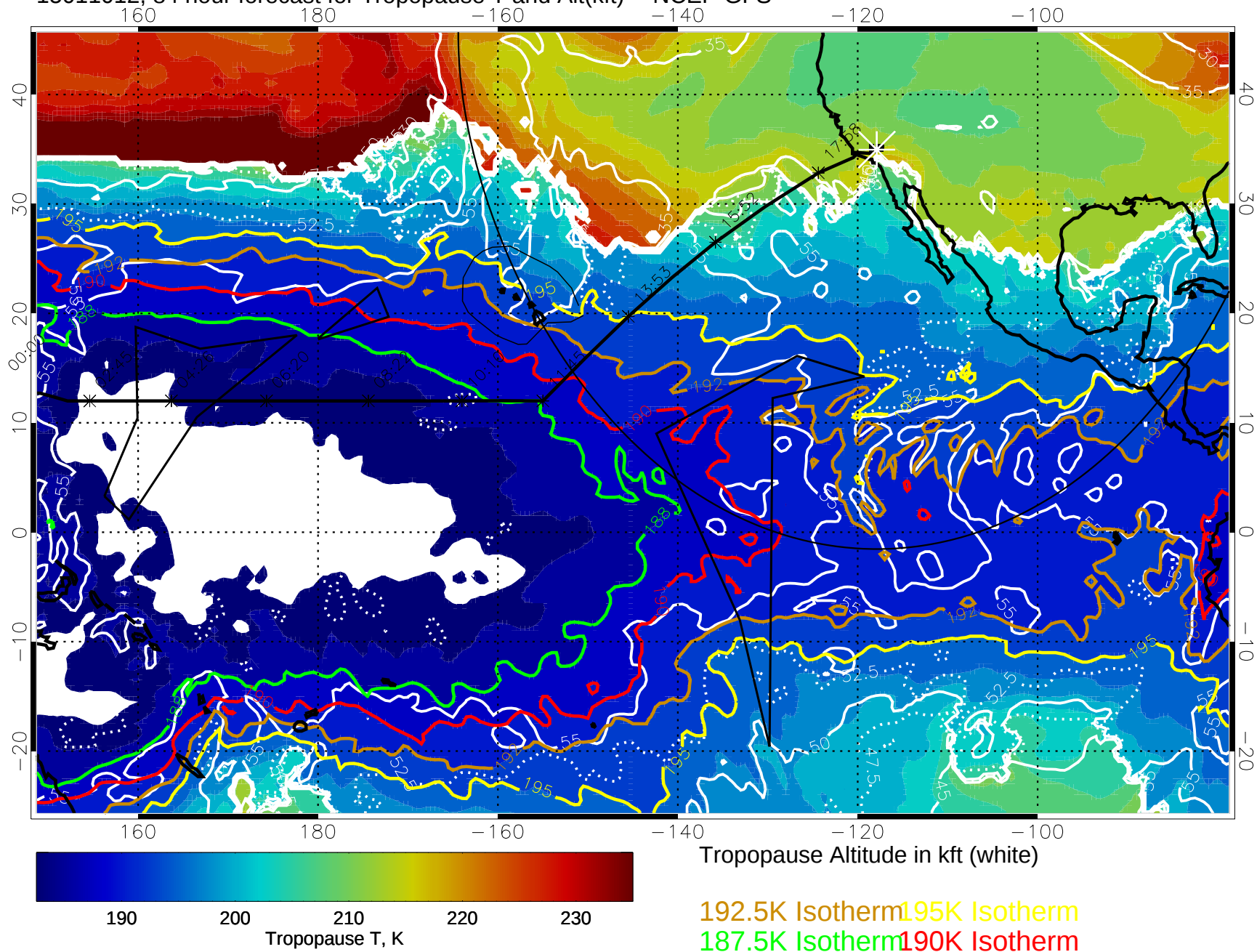
15011012, 84 hour forecast for Tropopause T and Alt(kft) -- NCEP GFS
