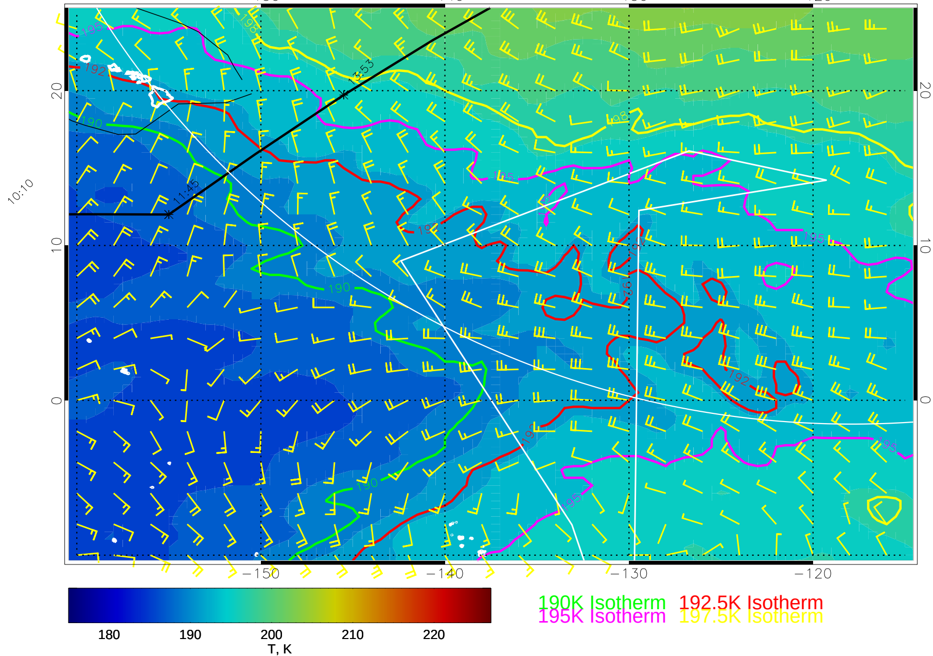
15011118, 114 hour forecast for 70mb T and winds (knots) -- NCEP GFS
