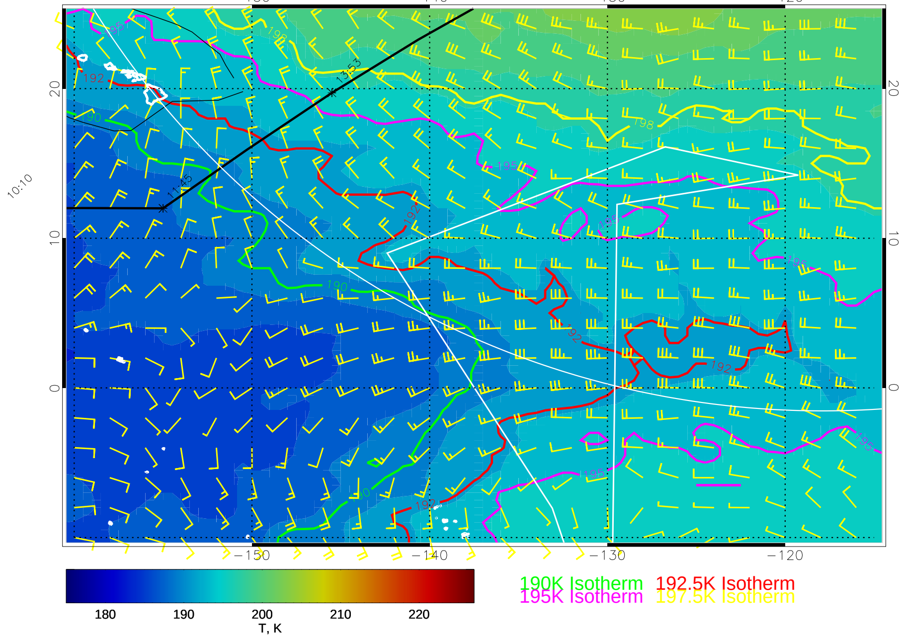
15011112, 108 hour forecast for 70mb T and winds (knots) -- NCEP GFS
