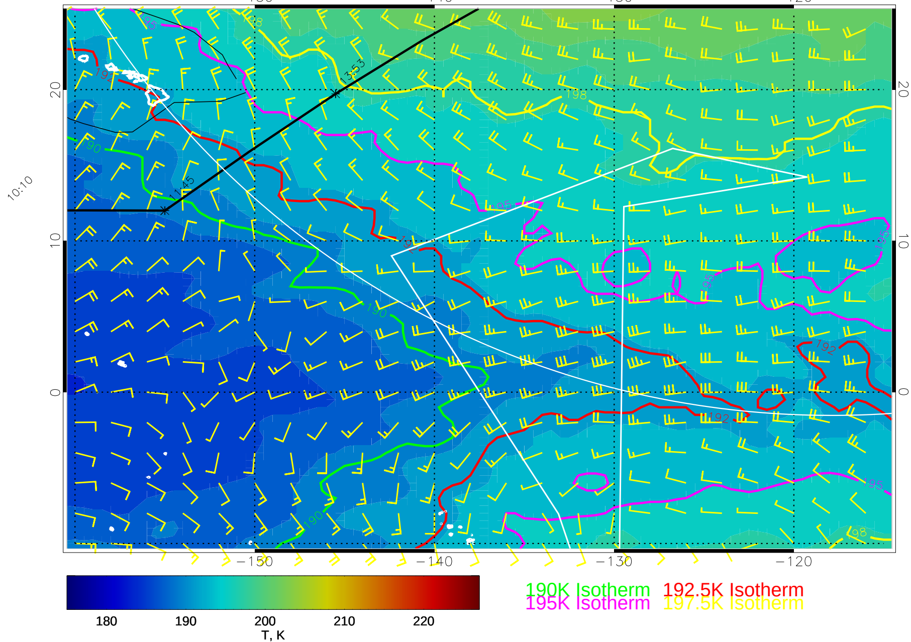
15011106, 102 hour forecast for 70mb T and winds (knots) -- NCEP GFS
