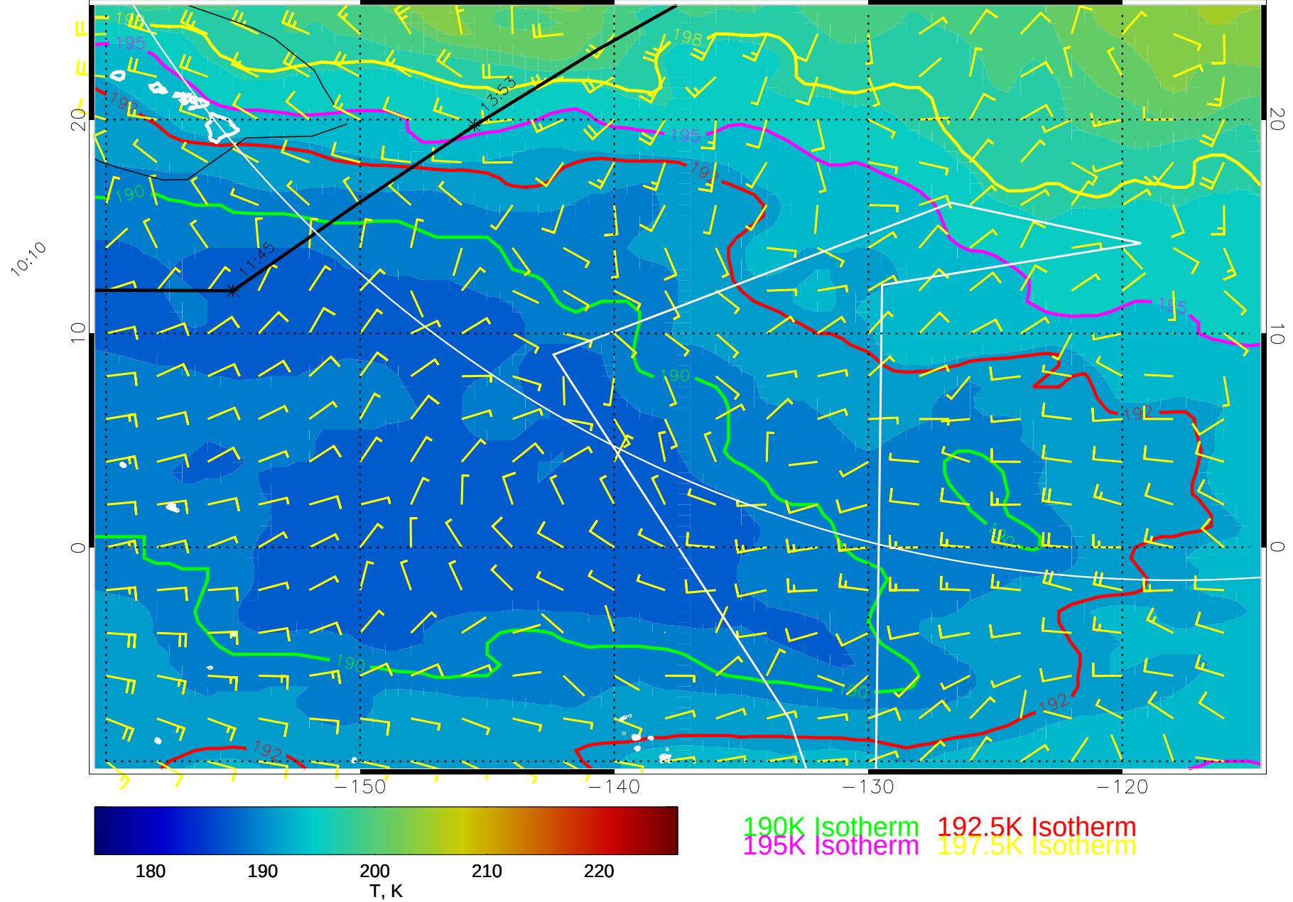
15010706, 6 hour forecast for 70mb T and winds (knots) -- NCEP GFS
