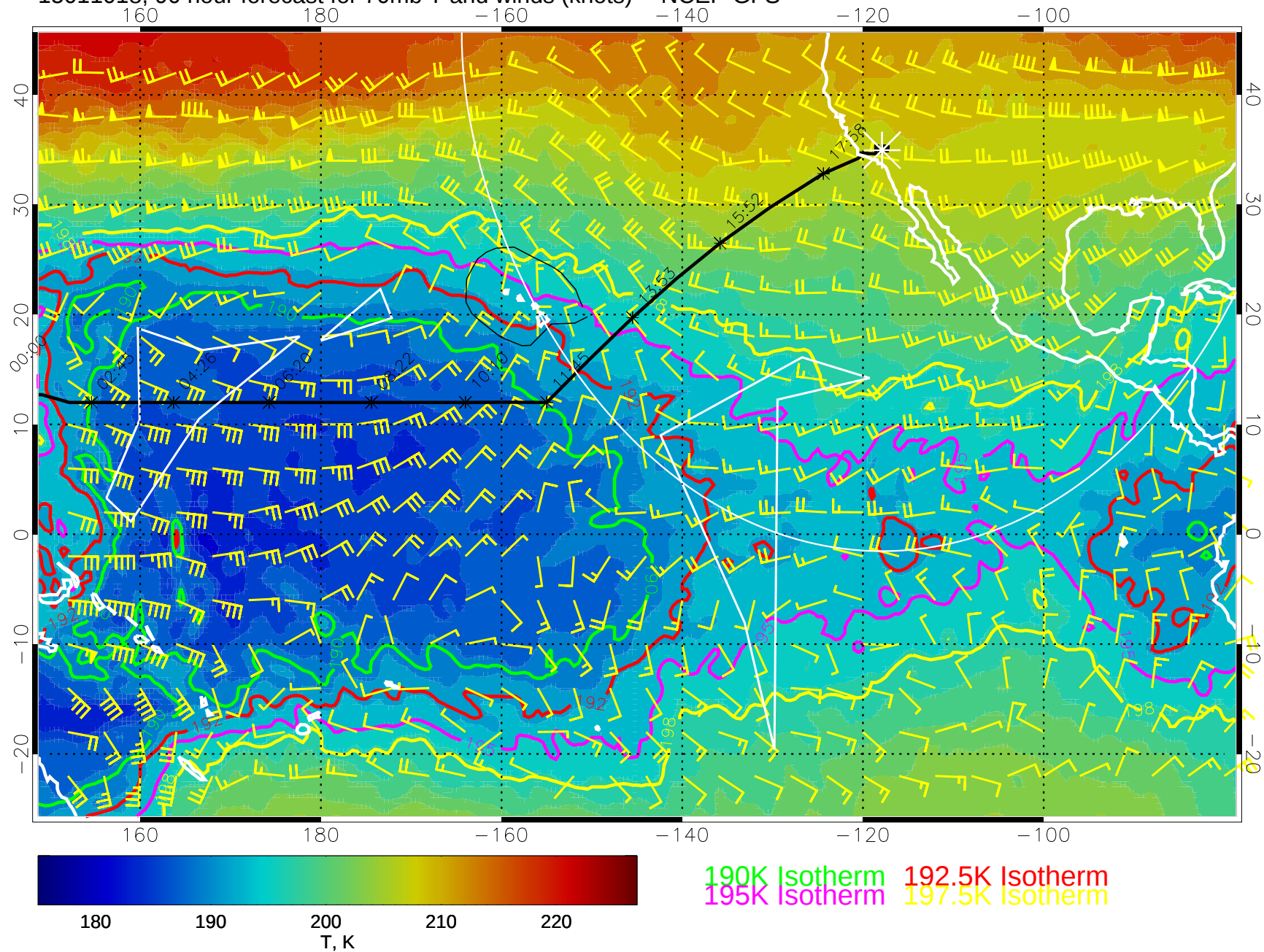
15011018, 90 hour forecast for 70mb T and winds (knots) -- NCEP GFS
