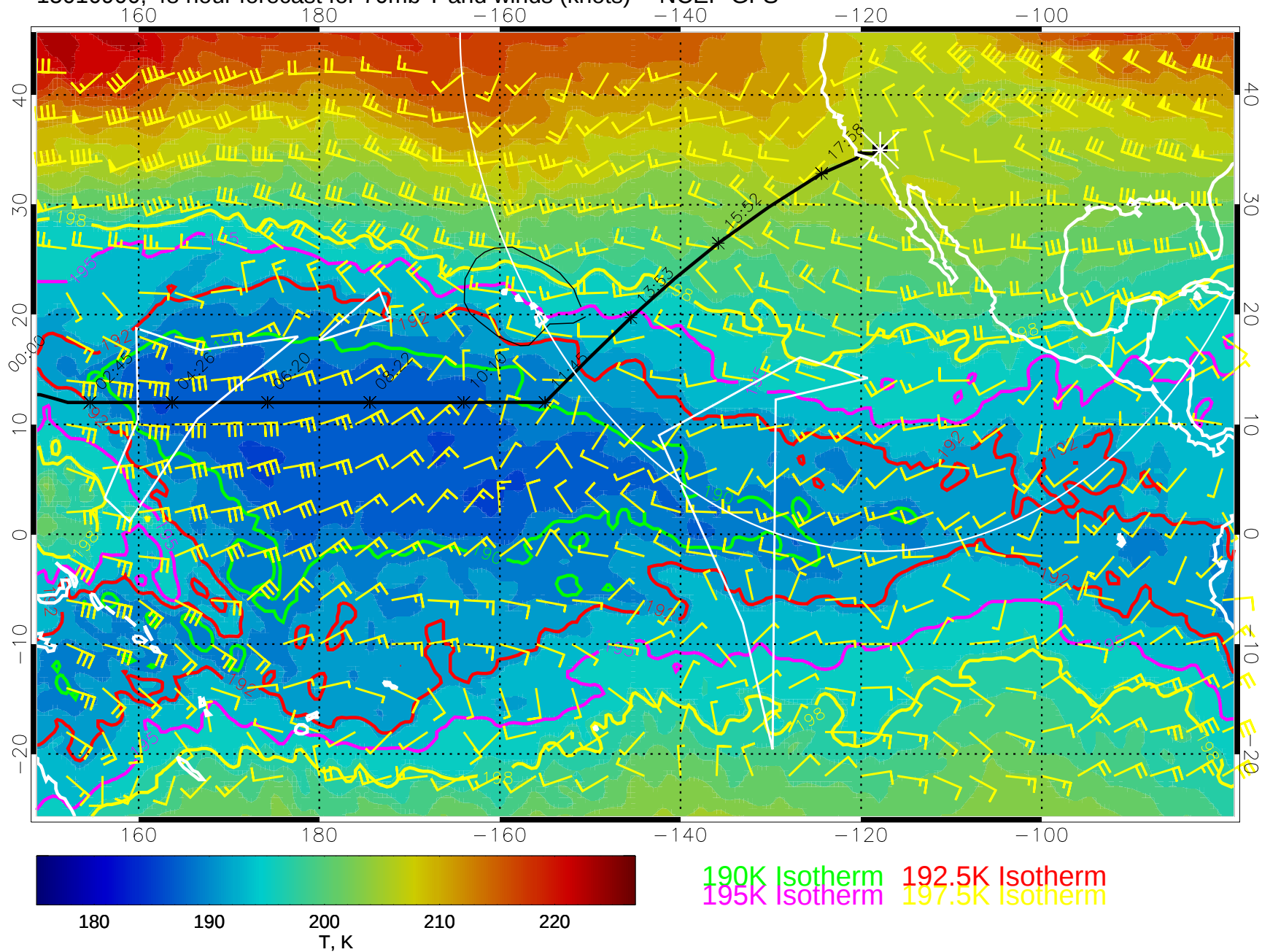
15010900, 48 hour forecast for 70mb T and winds (knots) -- NCEP GFS
