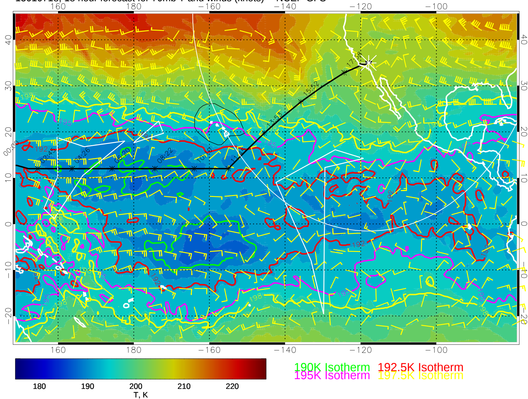
15010718, 18 hour forecast for 70mb T and winds (knots) -- NCEP GFS
