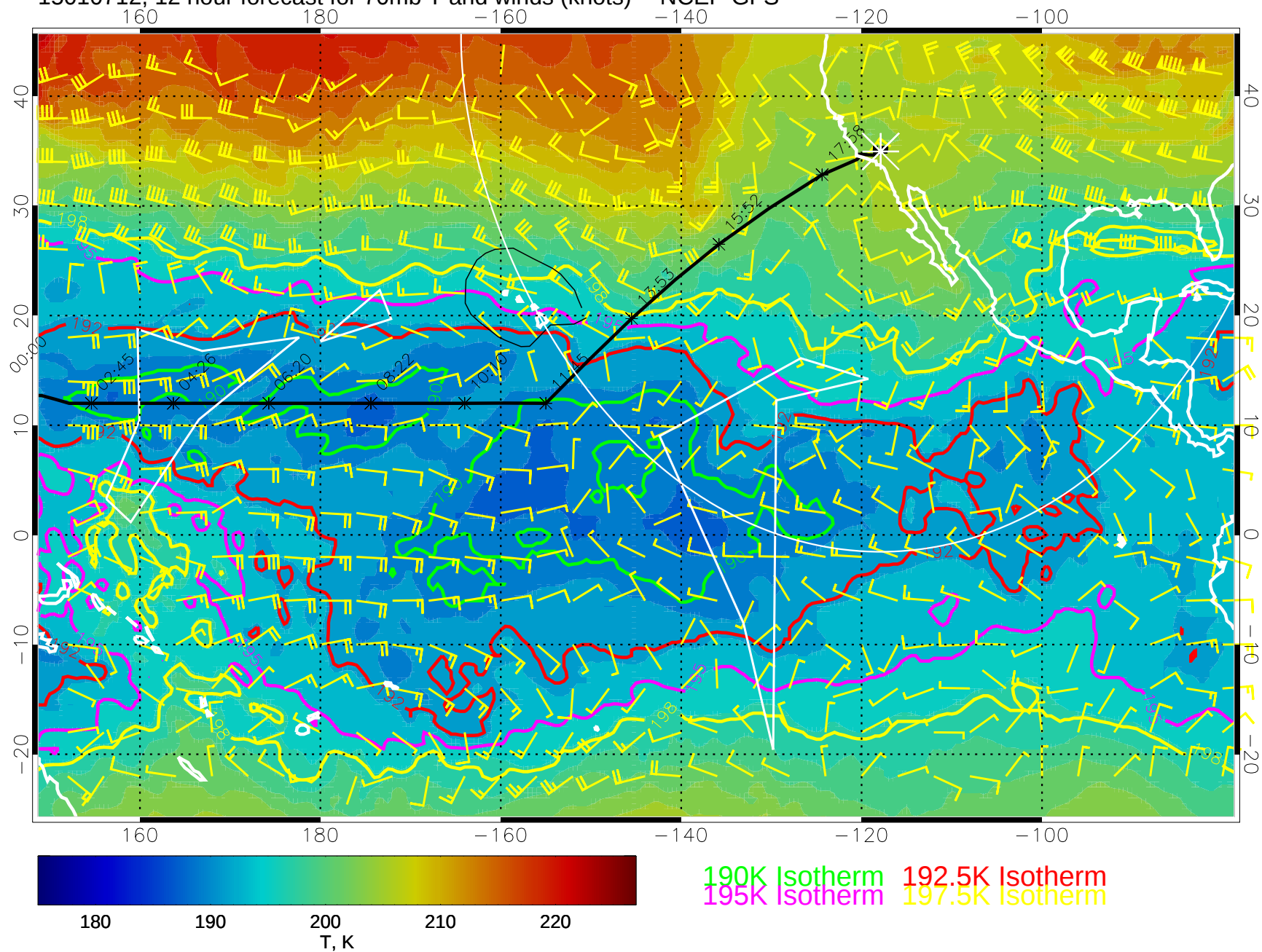
15010712, 12 hour forecast for 70mb T and winds (knots) -- NCEP GFS
