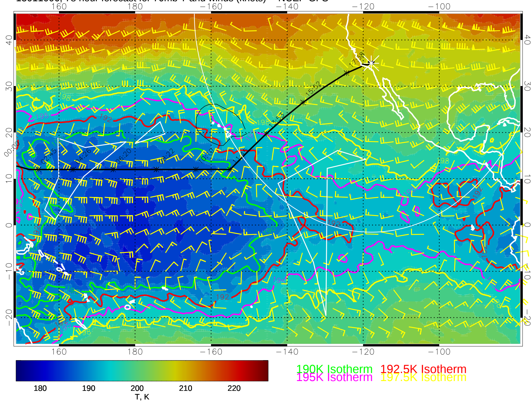
15011006, 78 hour forecast for 70mb T and winds (knots) -- NCEP GFS
