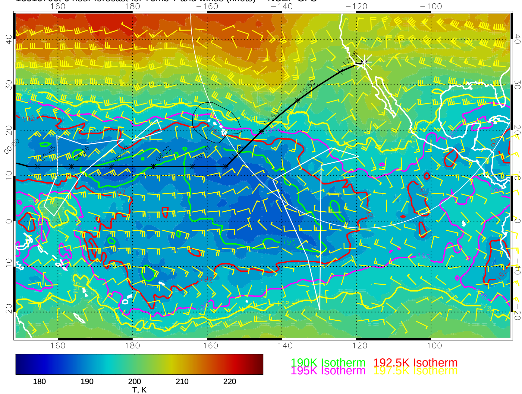
15010706, 6 hour forecast for 70mb T and winds (knots) -- NCEP GFS
