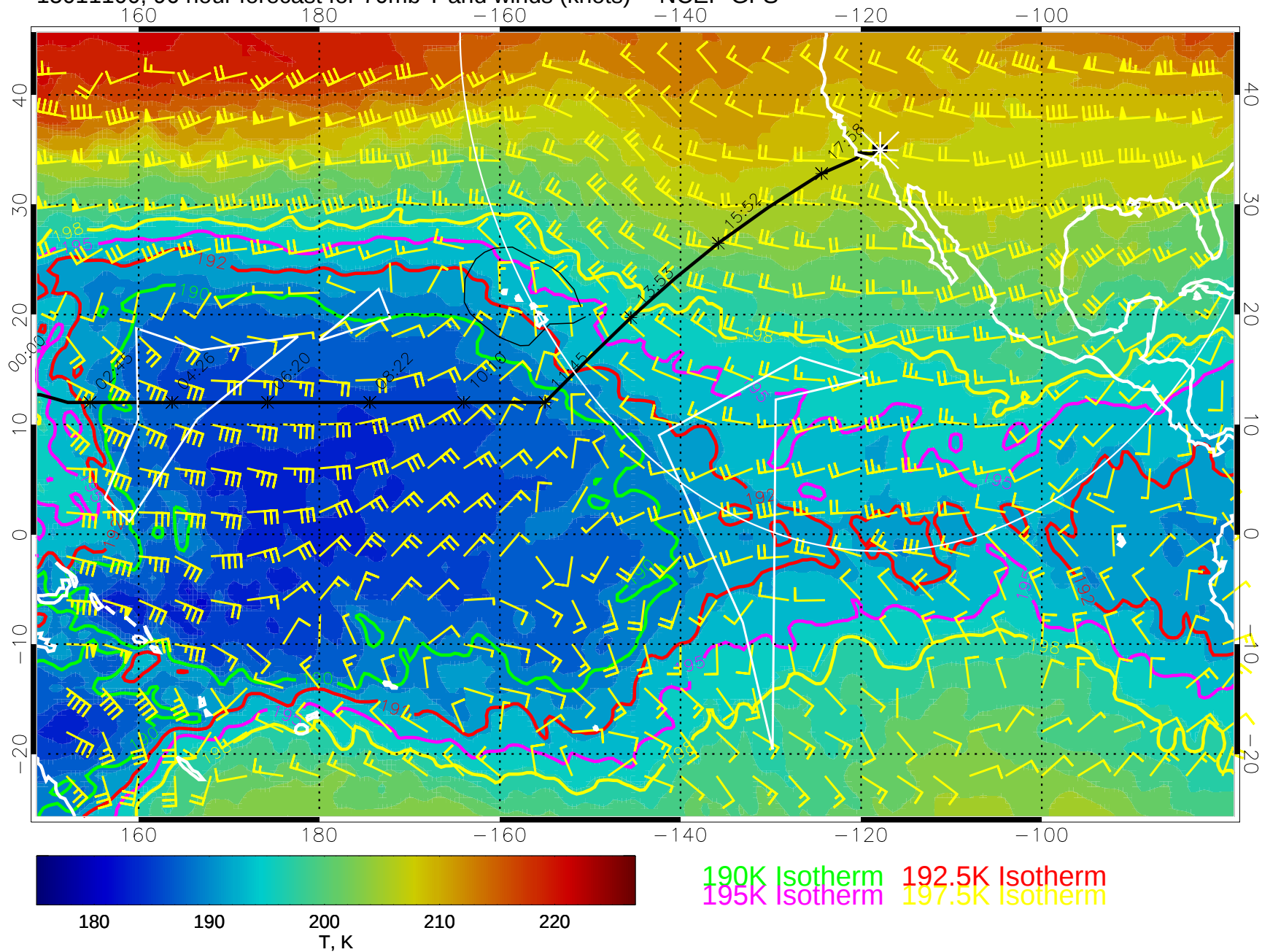
15011100, 96 hour forecast for 70mb T and winds (knots) -- NCEP GFS
