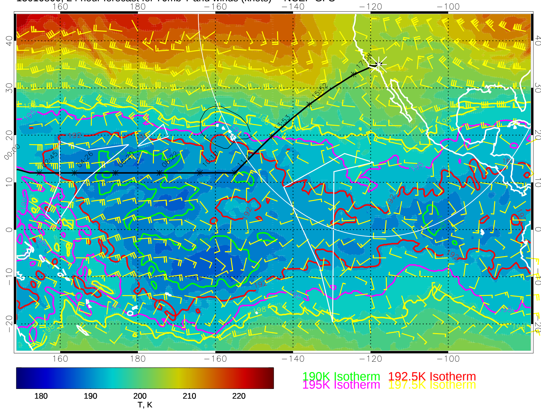
15010800, 24 hour forecast for 70mb T and winds (knots) -- NCEP GFS
