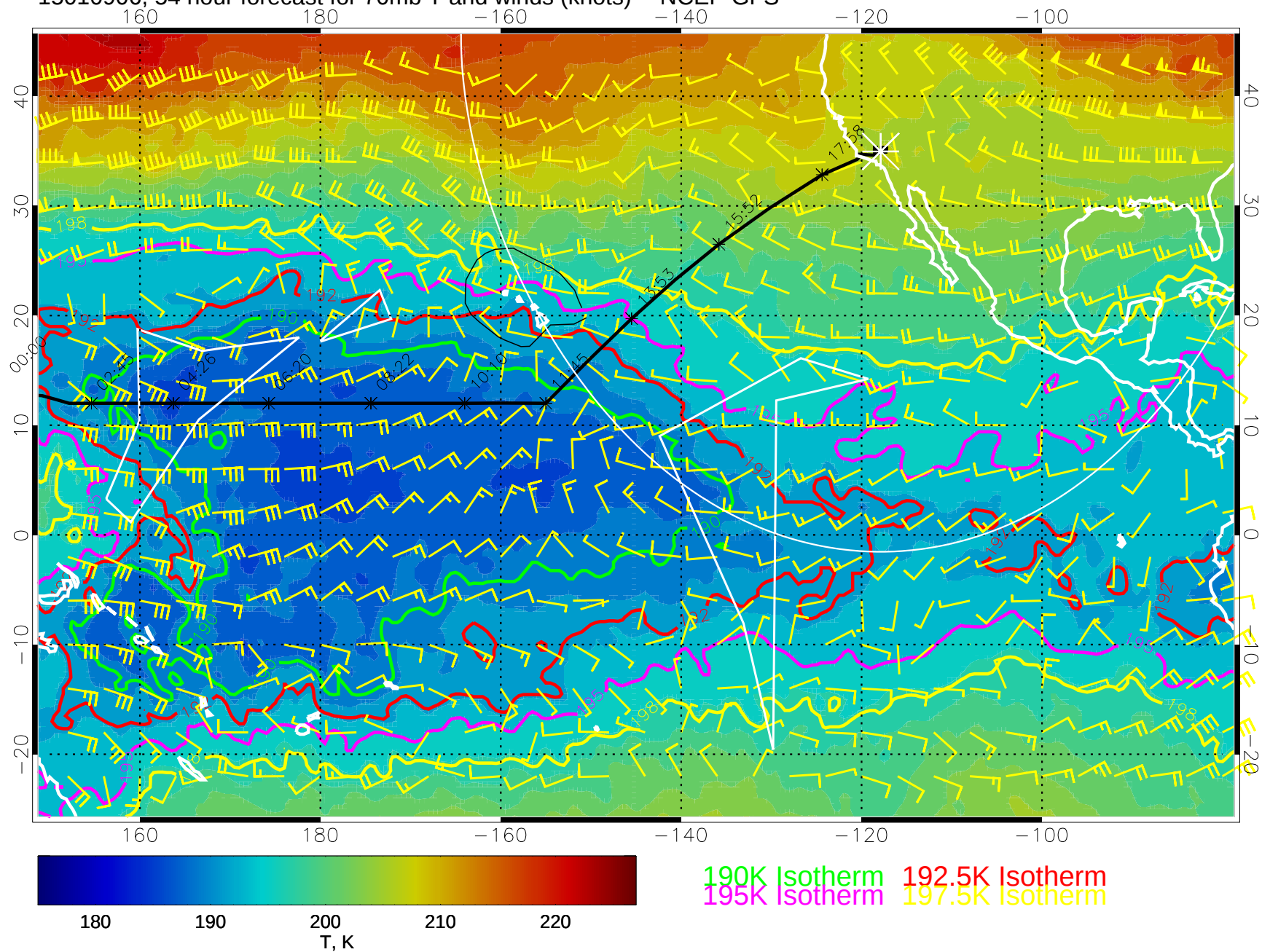
15010906, 54 hour forecast for 70mb T and winds (knots) -- NCEP GFS
