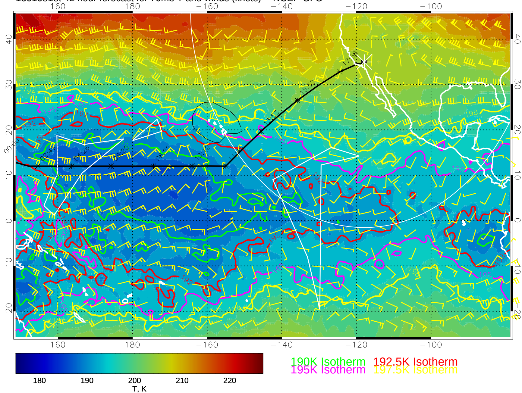
15010818, 42 hour forecast for 70mb T and winds (knots) -- NCEP GFS
