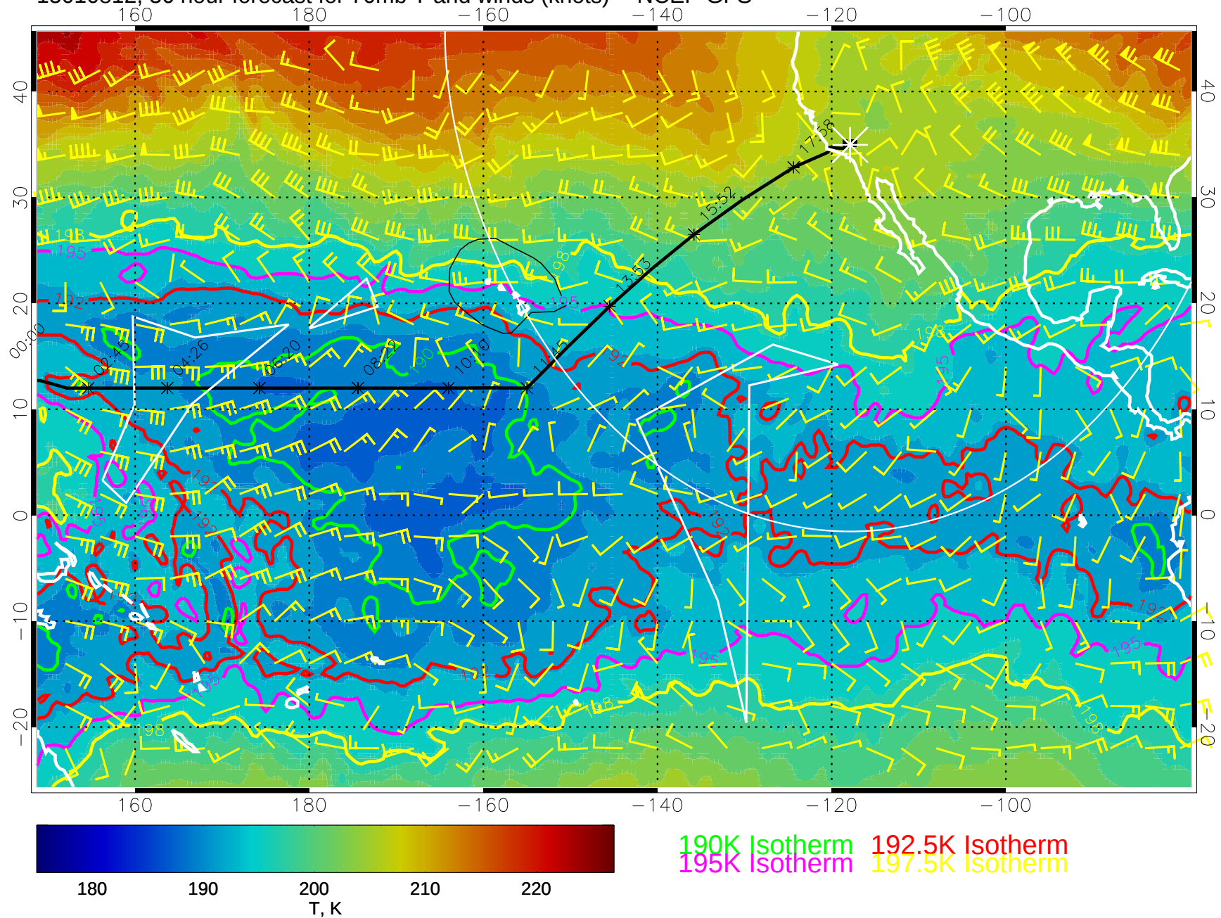
15010812, 36 hour forecast for 70mb T and winds (knots) -- NCEP GFS
