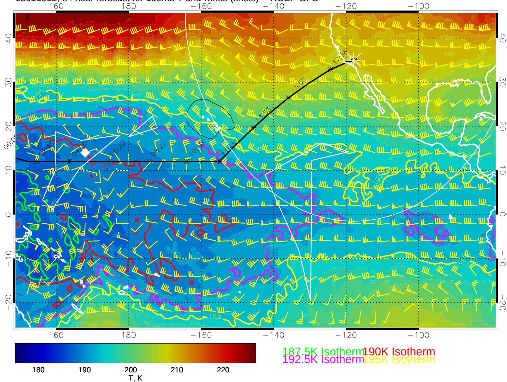
15011012, 84 hour forecast for 100mb T and winds (knots) -- NCEP GFS
