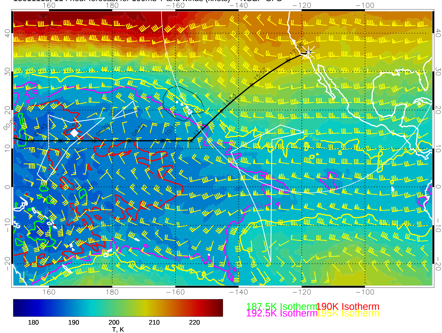
15011118, 114 hour forecast for 100mb T and winds (knots) -- NCEP GFS
