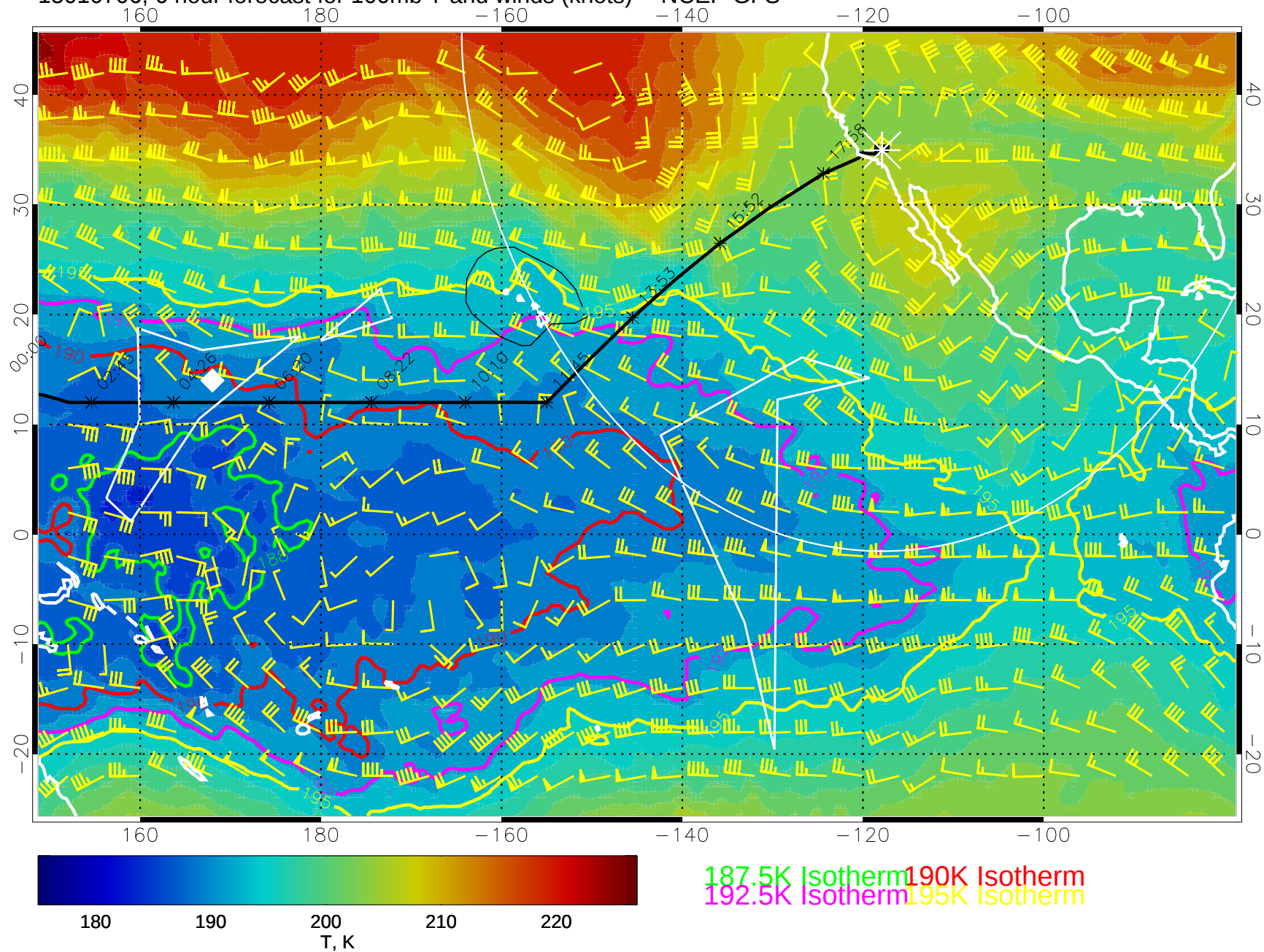
15010706, 6 hour forecast for 100mb T and winds (knots) -- NCEP GFS
