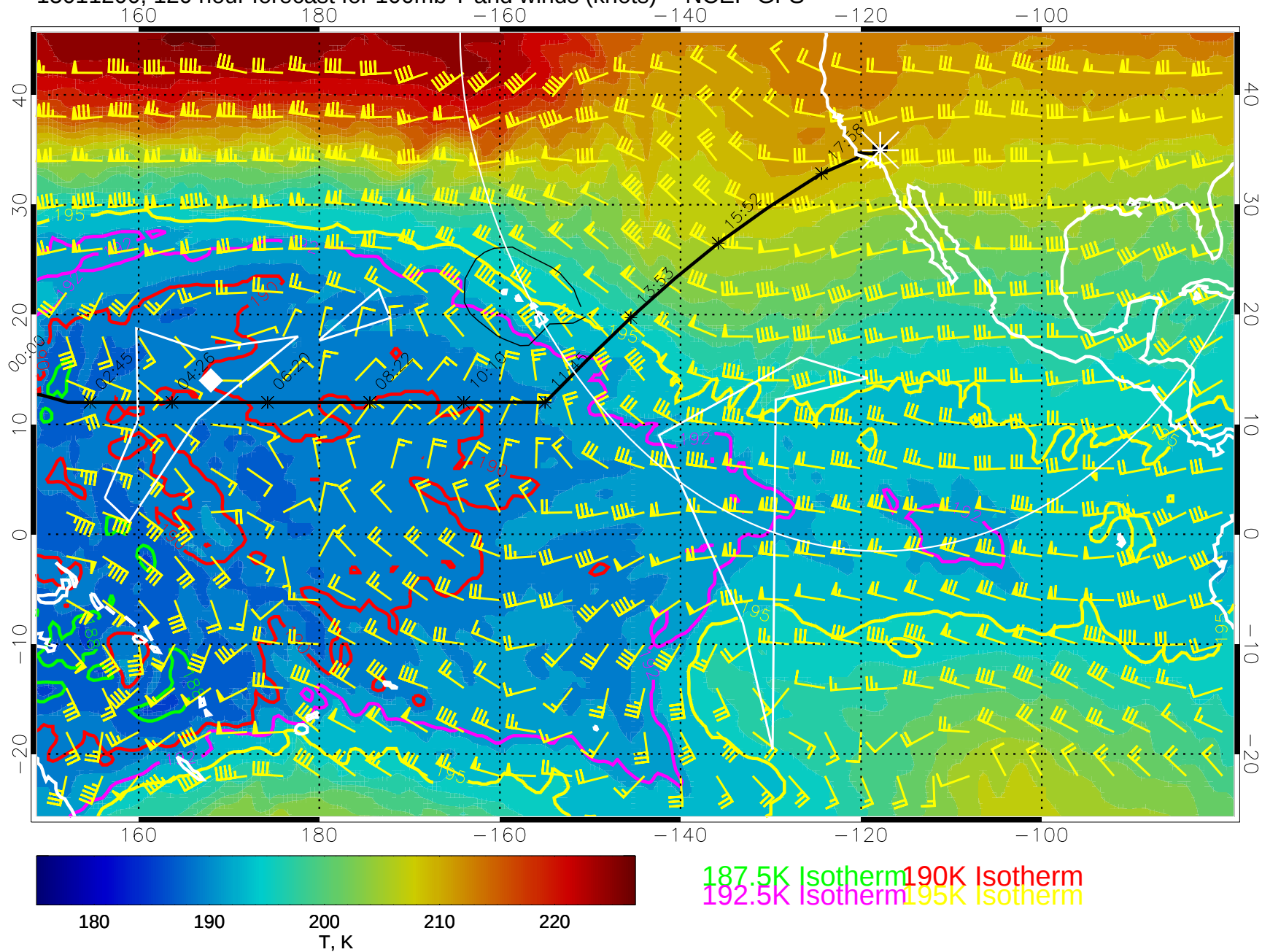
15011200, 120 hour forecast for 100mb T and winds (knots) -- NCEP GFS
