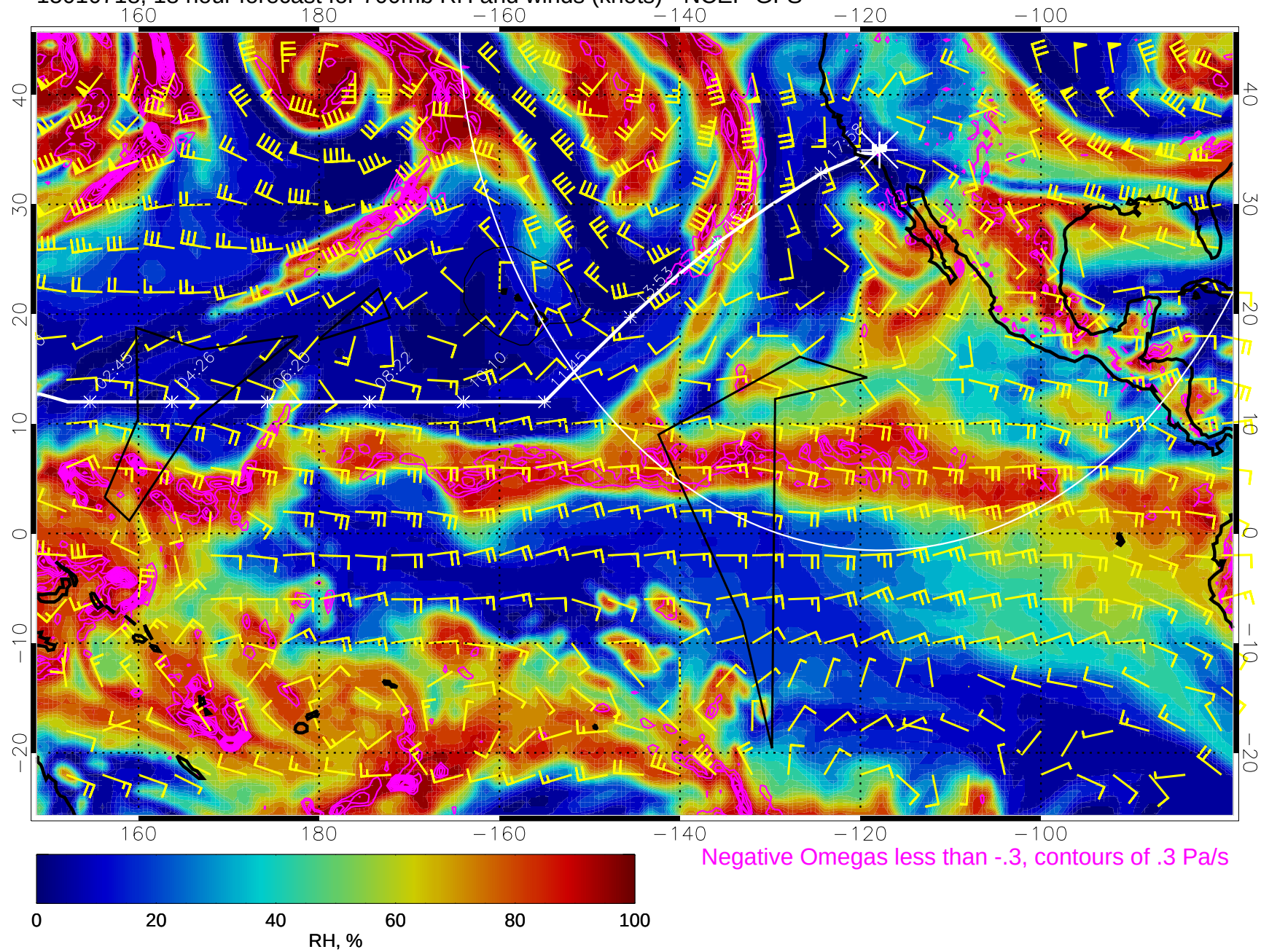
15010718, 18 hour forecast for 700mb RH and winds (knots) - NCEP GFS
