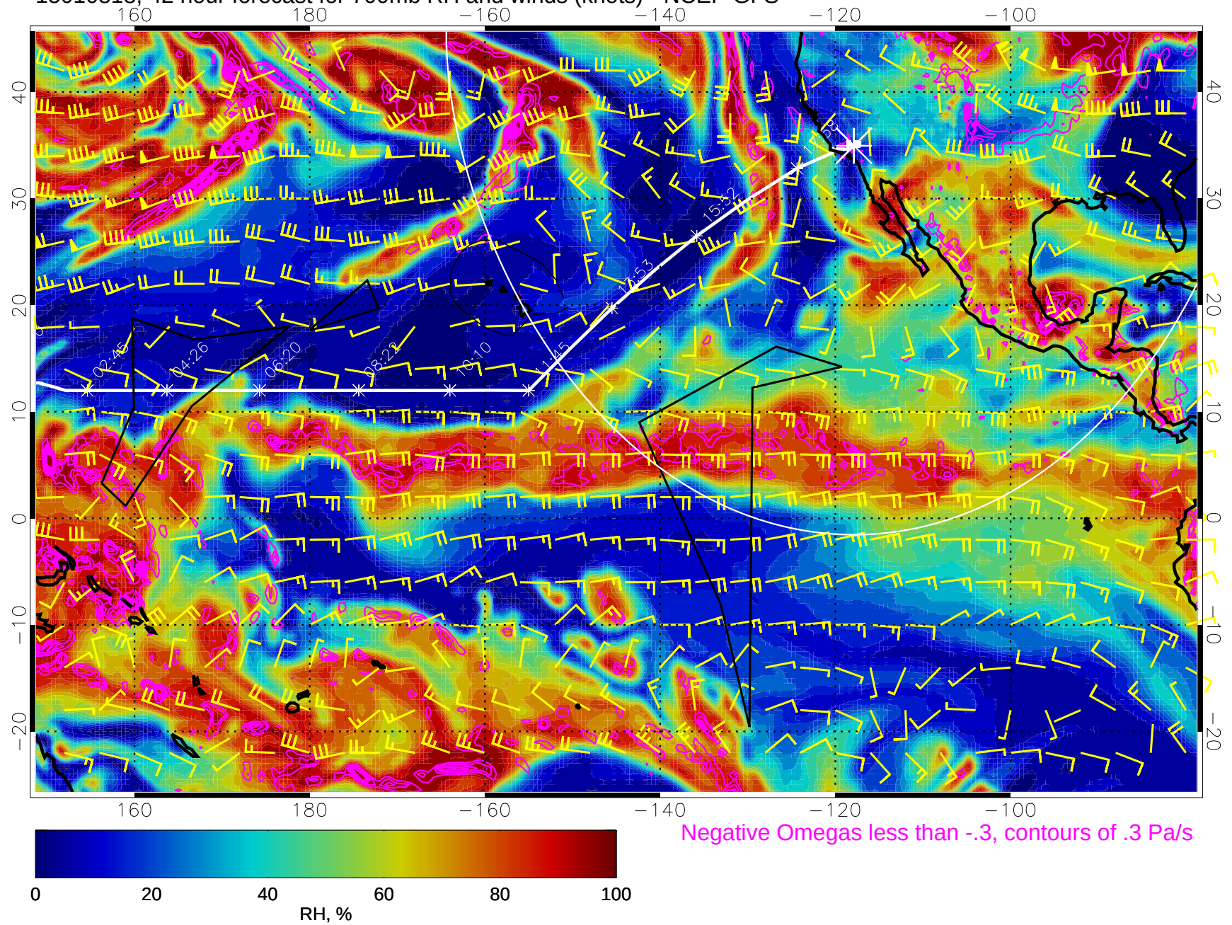
15010818, 42 hour forecast for 700mb RH and winds (knots) - NCEP GFS
