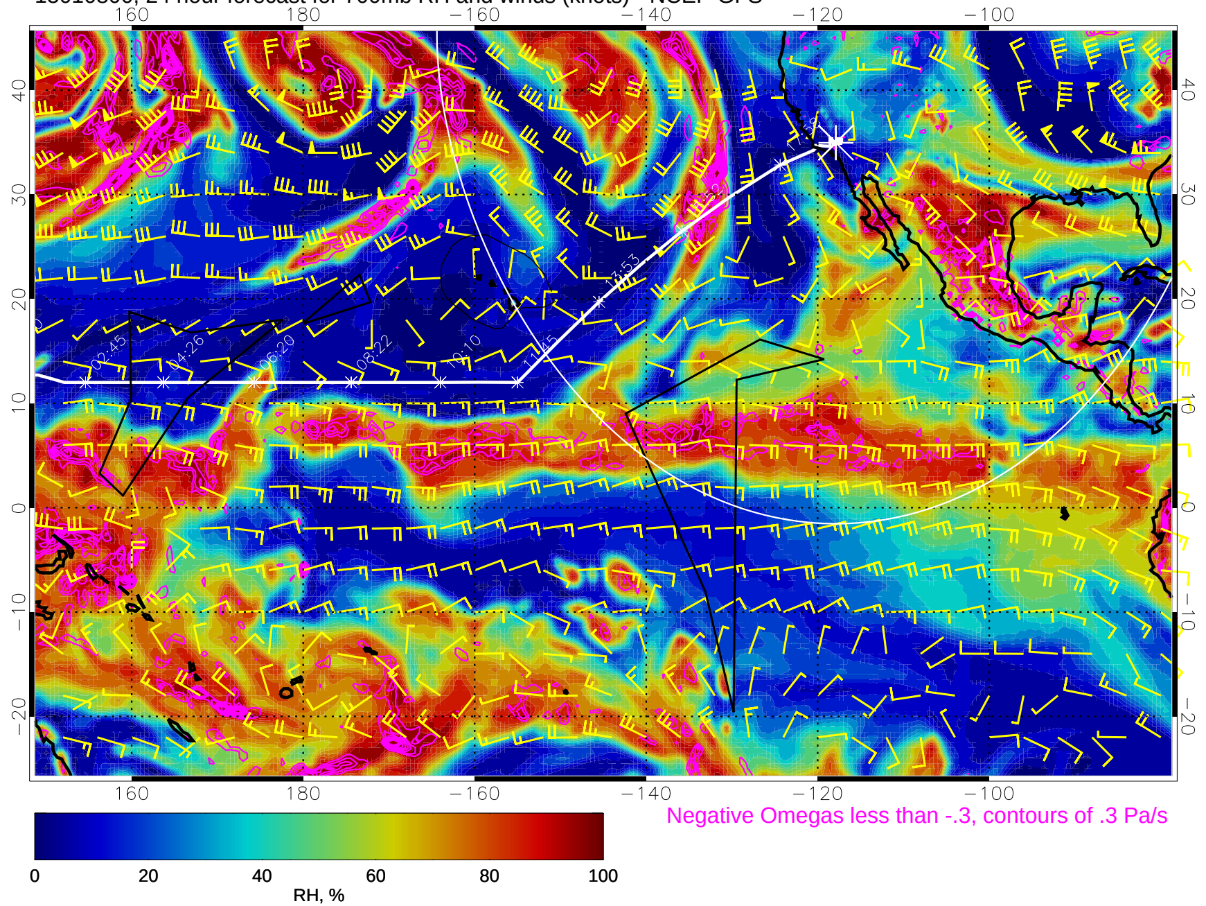
15010800, 24 hour forecast for 700mb RH and winds (knots) - NCEP GFS
