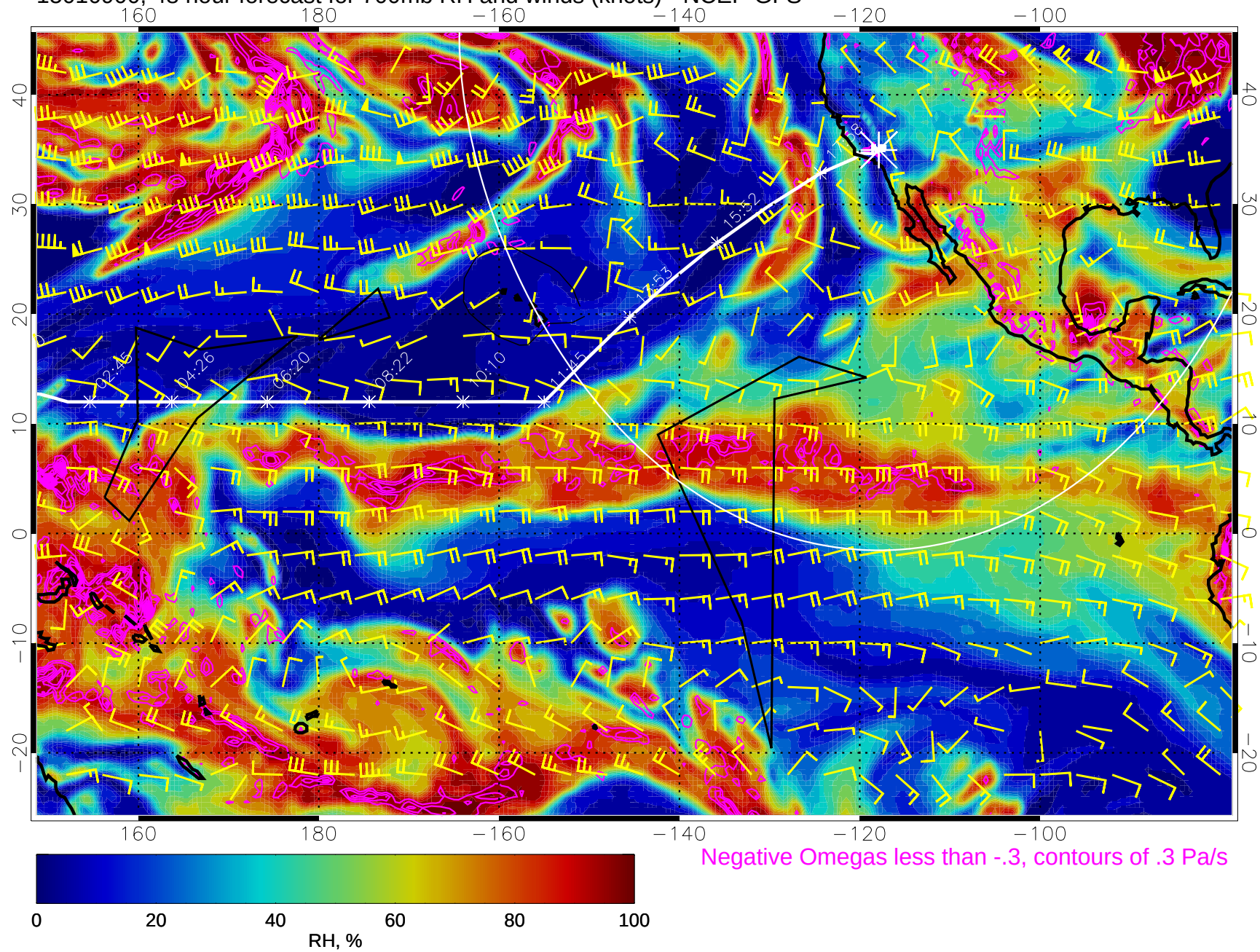
15010900, 48 hour forecast for 700mb RH and winds (knots) - NCEP GFS
