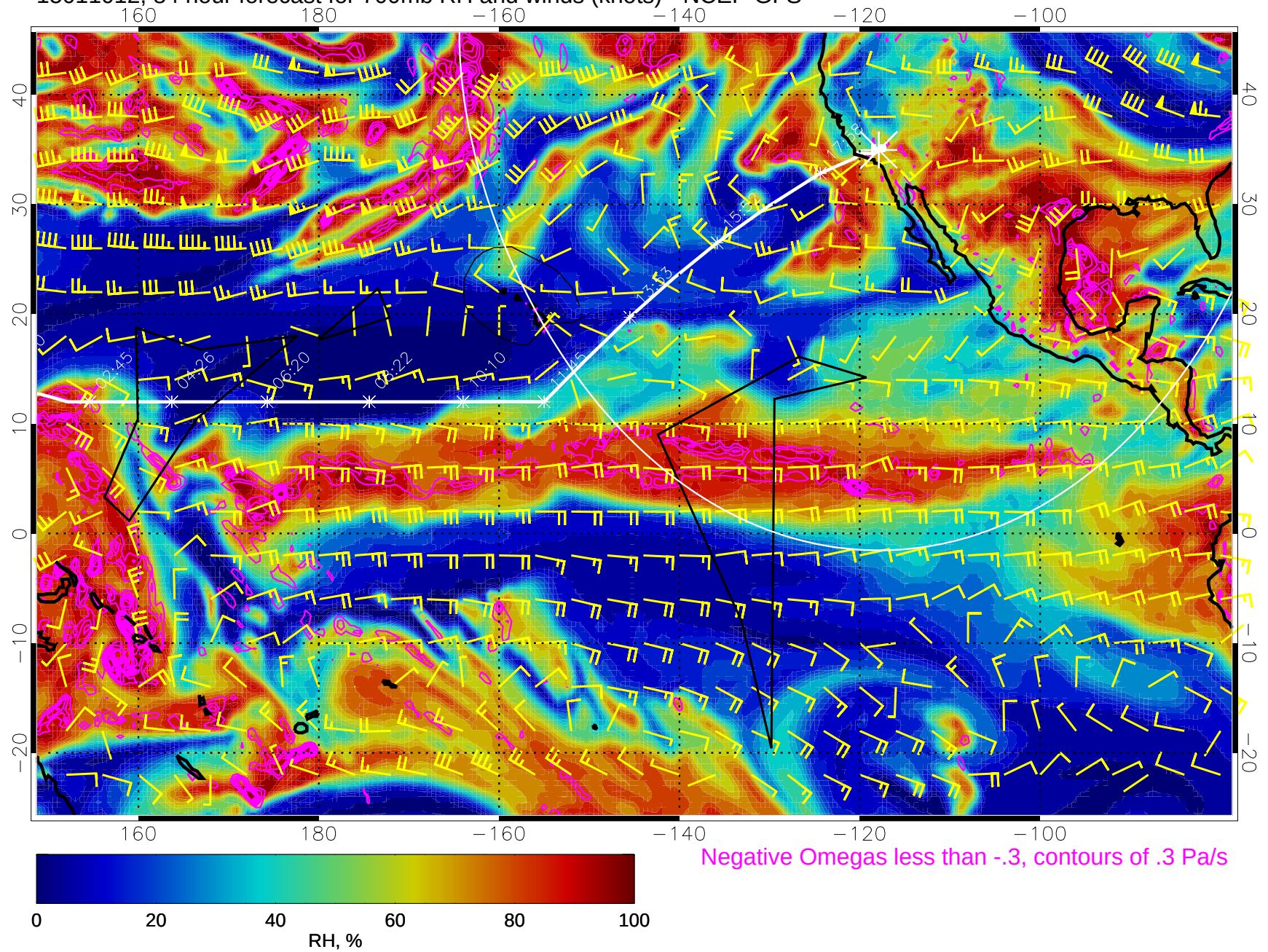
15011012, 84 hour forecast for 700mb RH and winds (knots) - NCEP GFS
