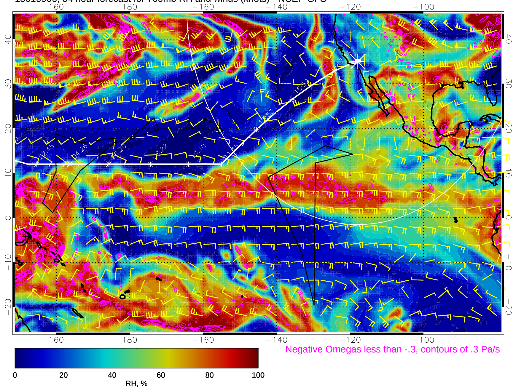
15010906, 54 hour forecast for 700mb RH and winds (knots) - NCEP GFS
