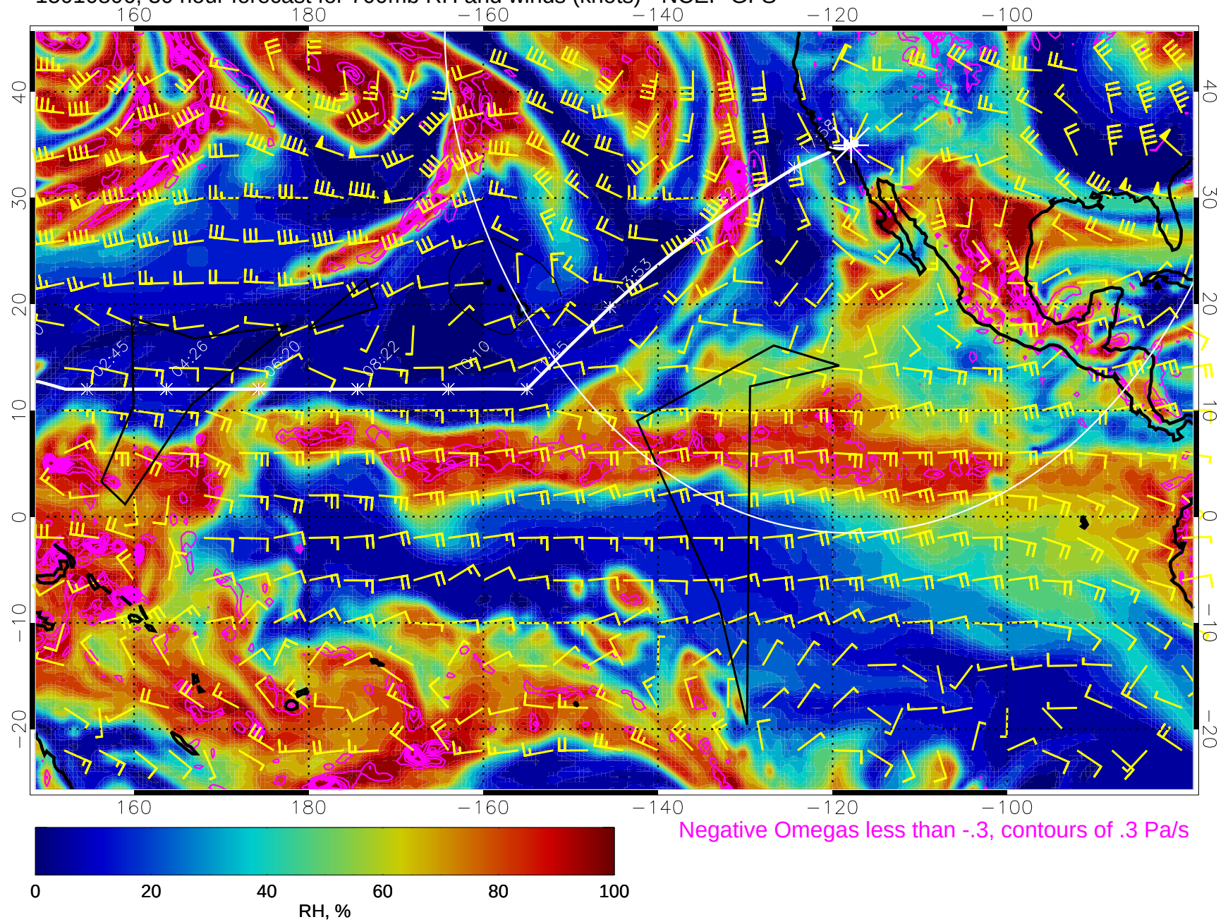
15010806, 30 hour forecast for 700mb RH and winds (knots) - NCEP GFS
