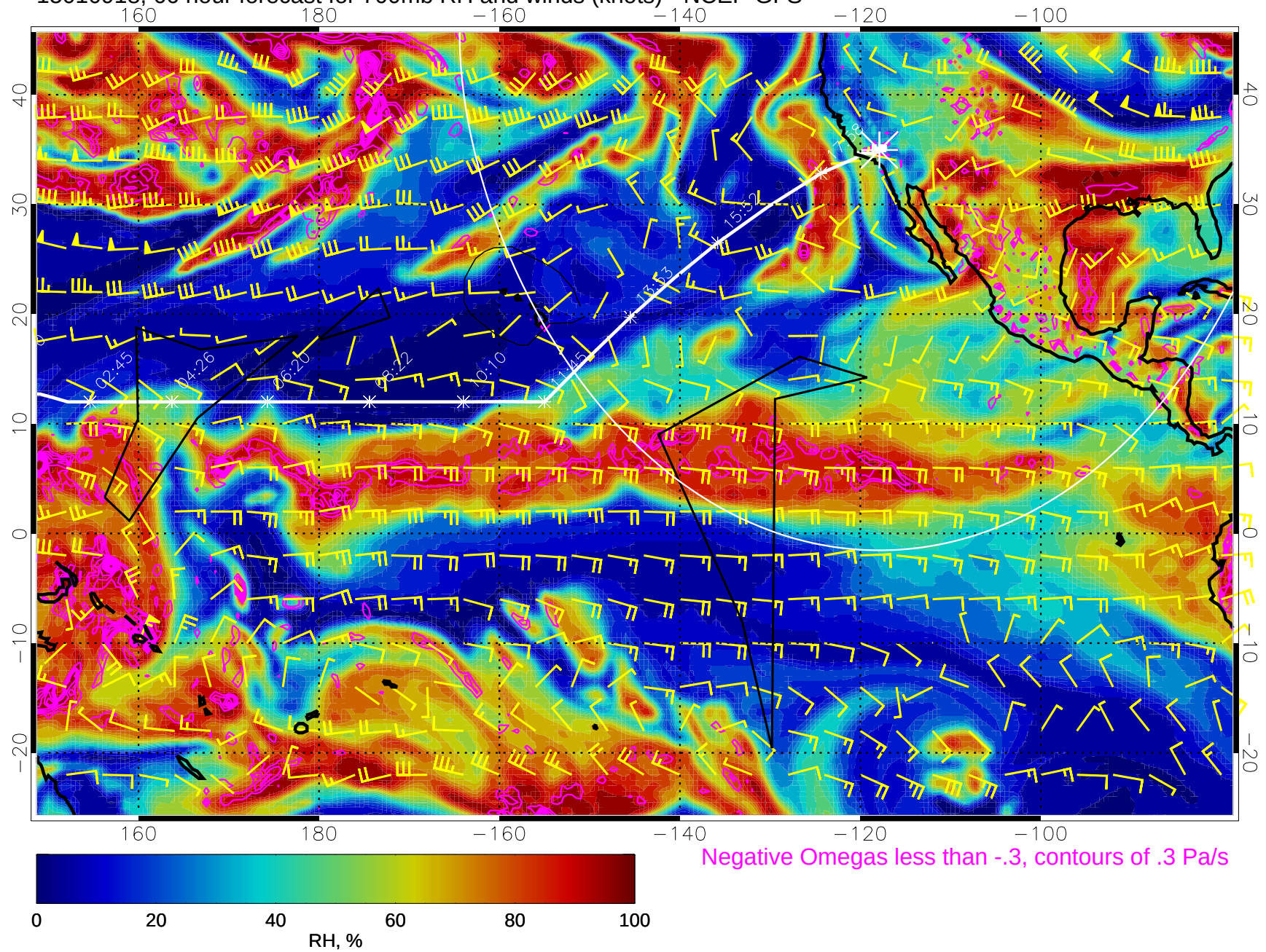
15010918, 66 hour forecast for 700mb RH and winds (knots) - NCEP GFS
