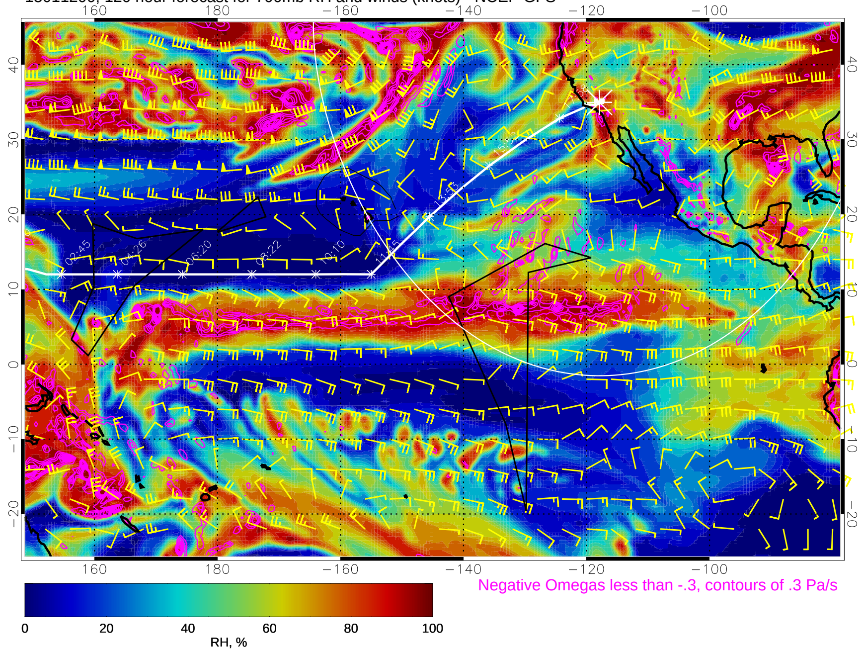
15011200, 120 hour forecast for 700mb RH and winds (knots) - NCEP GFS
