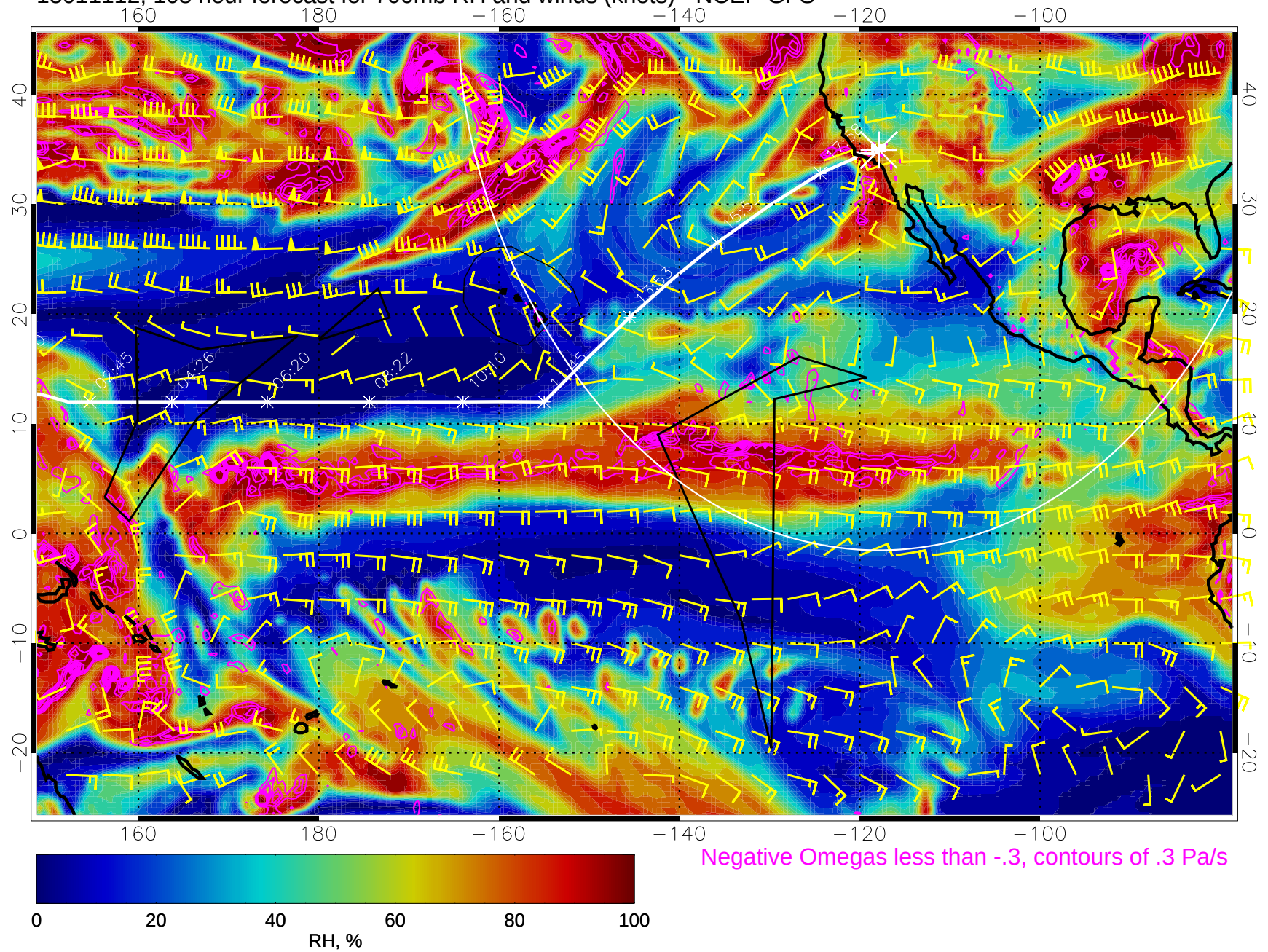
15011112, 108 hour forecast for 700mb RH and winds (knots) - NCEP GFS
