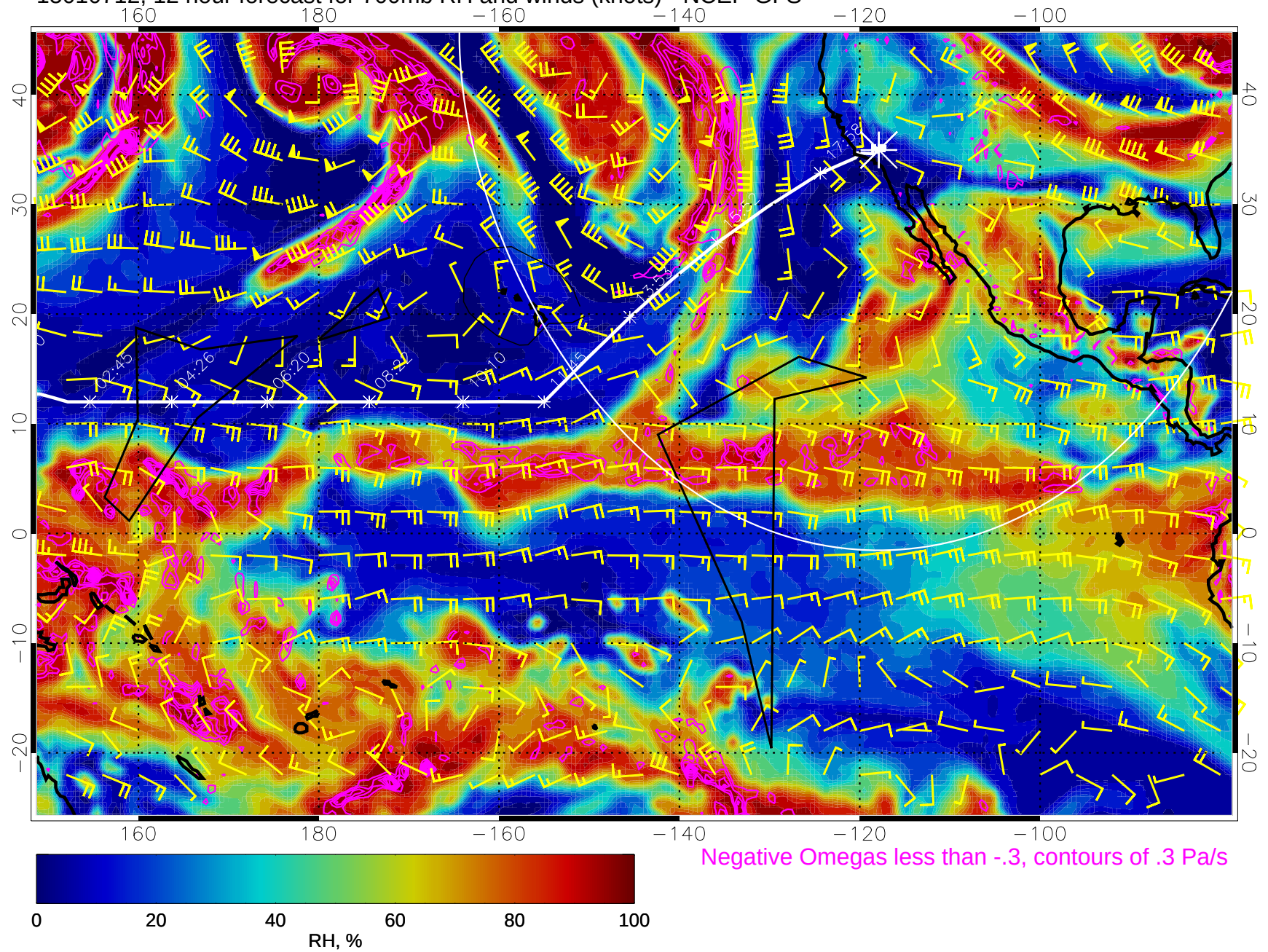
15010712, 12 hour forecast for 700mb RH and winds (knots) - NCEP GFS
