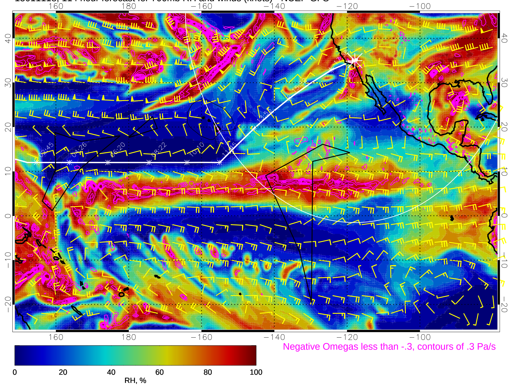
15011118, 114 hour forecast for 700mb RH and winds (knots) - NCEP GFS
