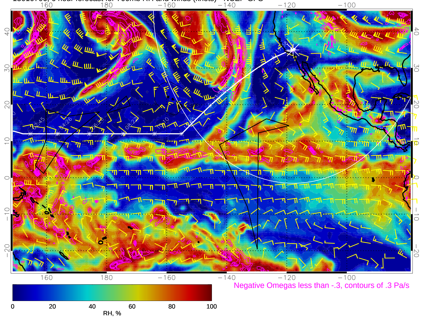
15010706, 6 hour forecast for 700mb RH and winds (knots) - NCEP GFS
