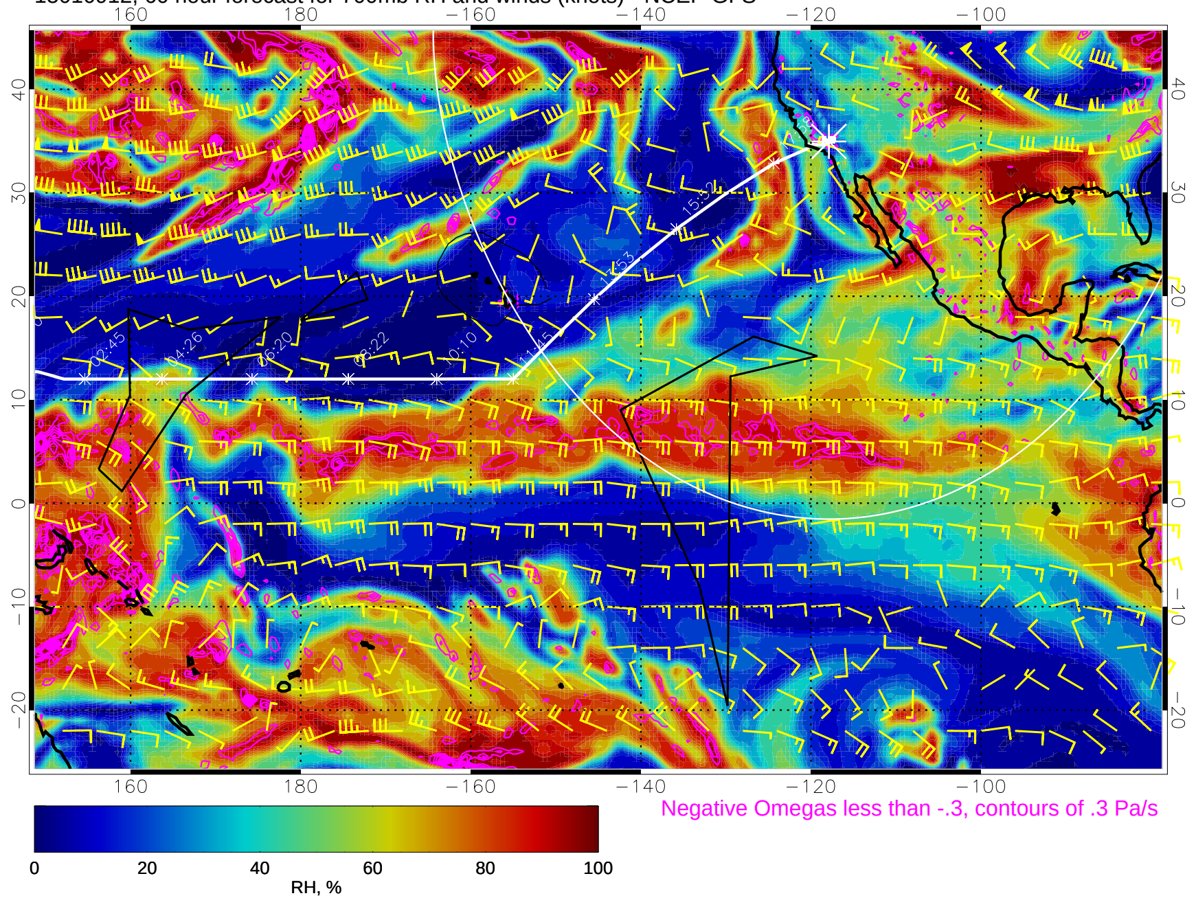
15010912, 60 hour forecast for 700mb RH and winds (knots) - NCEP GFS
