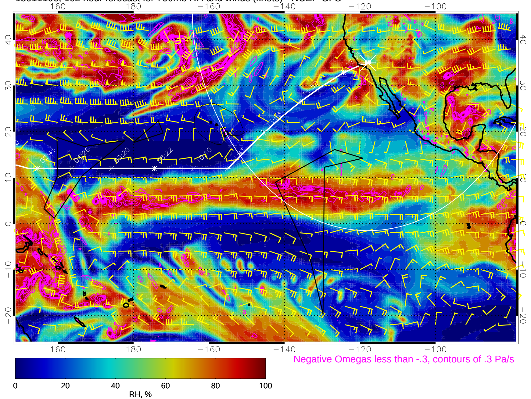
15011106, 102 hour forecast for 700mb RH and winds (knots) - NCEP GFS
