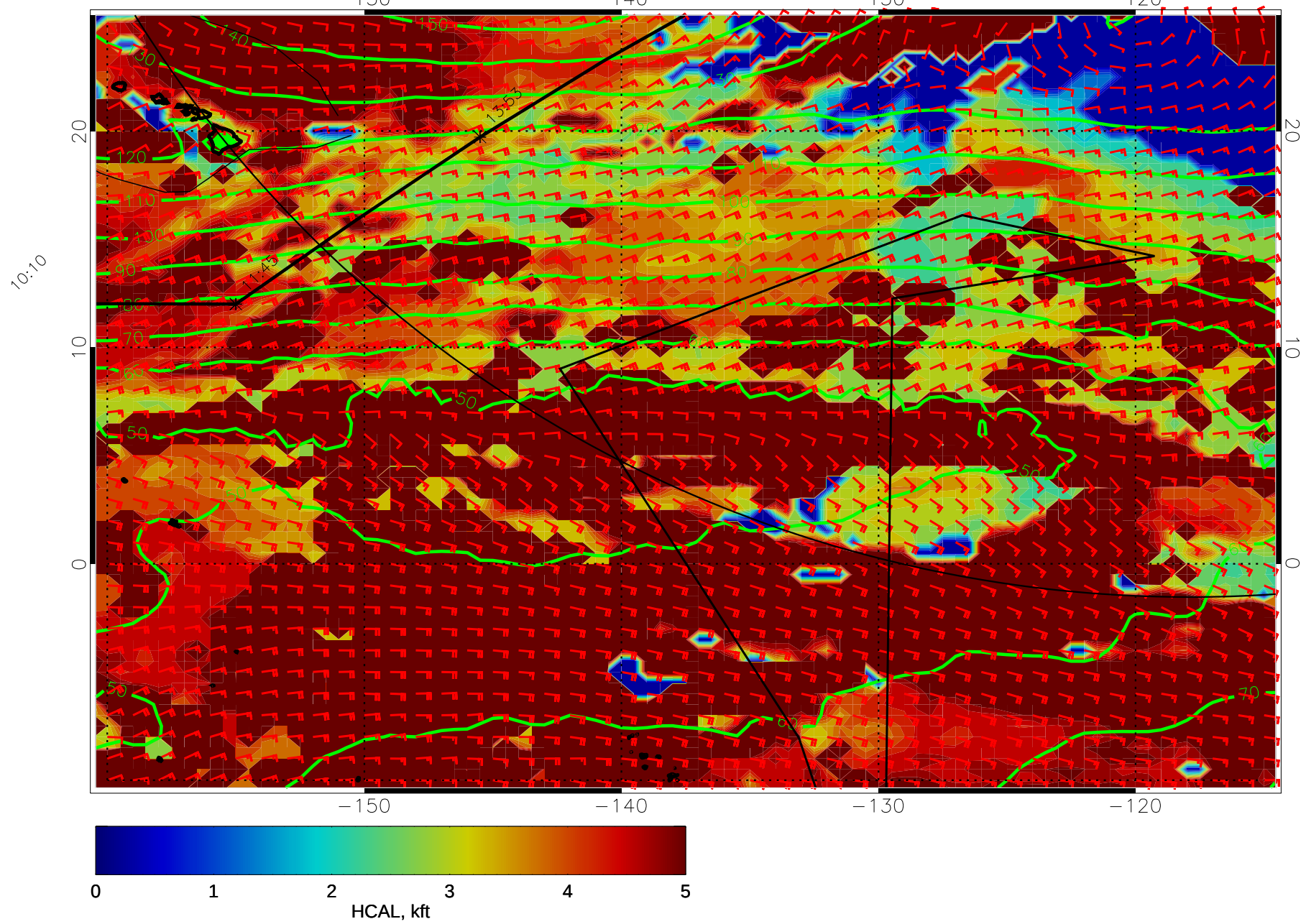
15011012, 84 hour forecast for HCAL, 1000mb Z, and winds (knots) -- NCEP GFS
