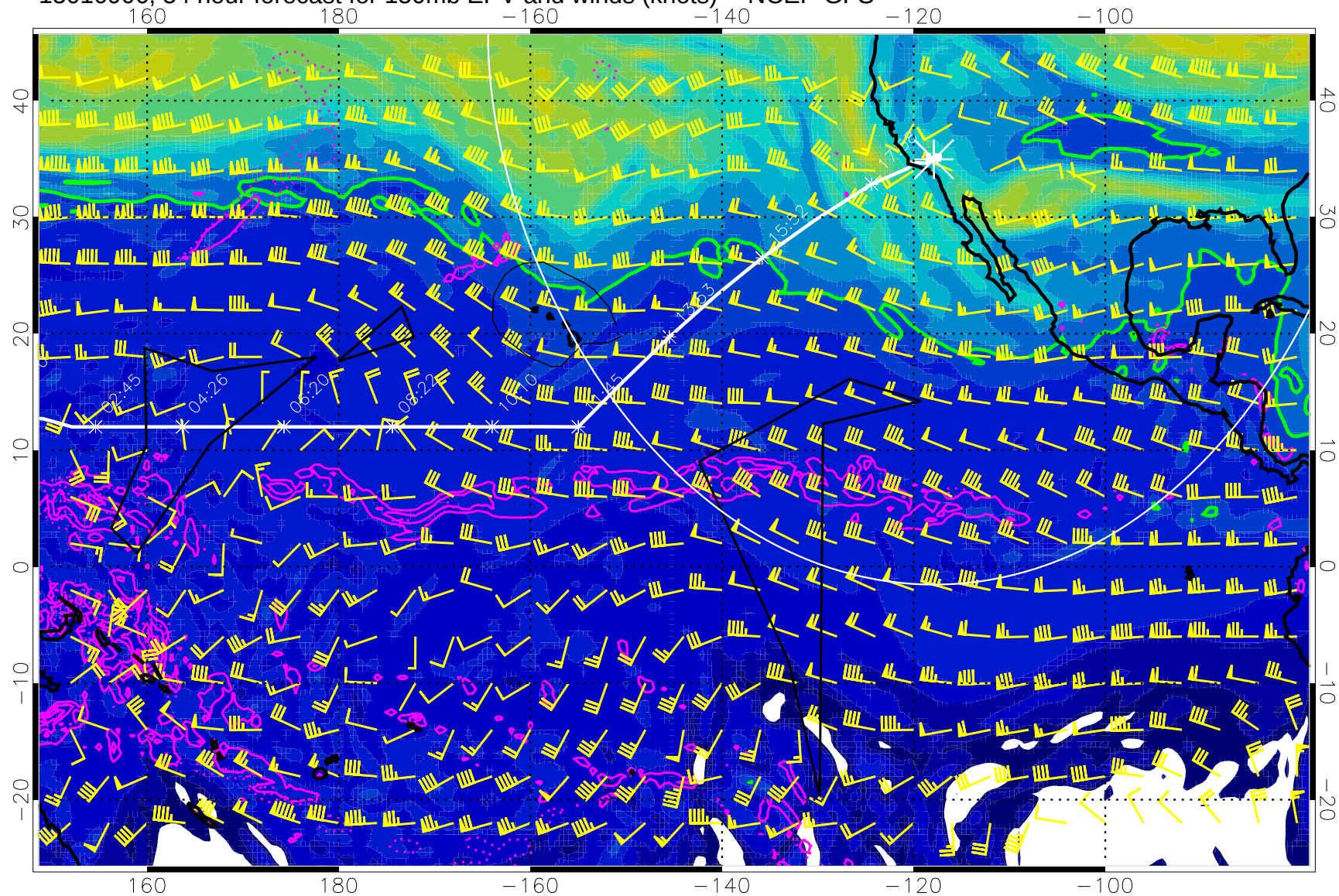
15010906, 54 hour forecast for 150mb EPV and winds (knots) -- NCEP GFS
