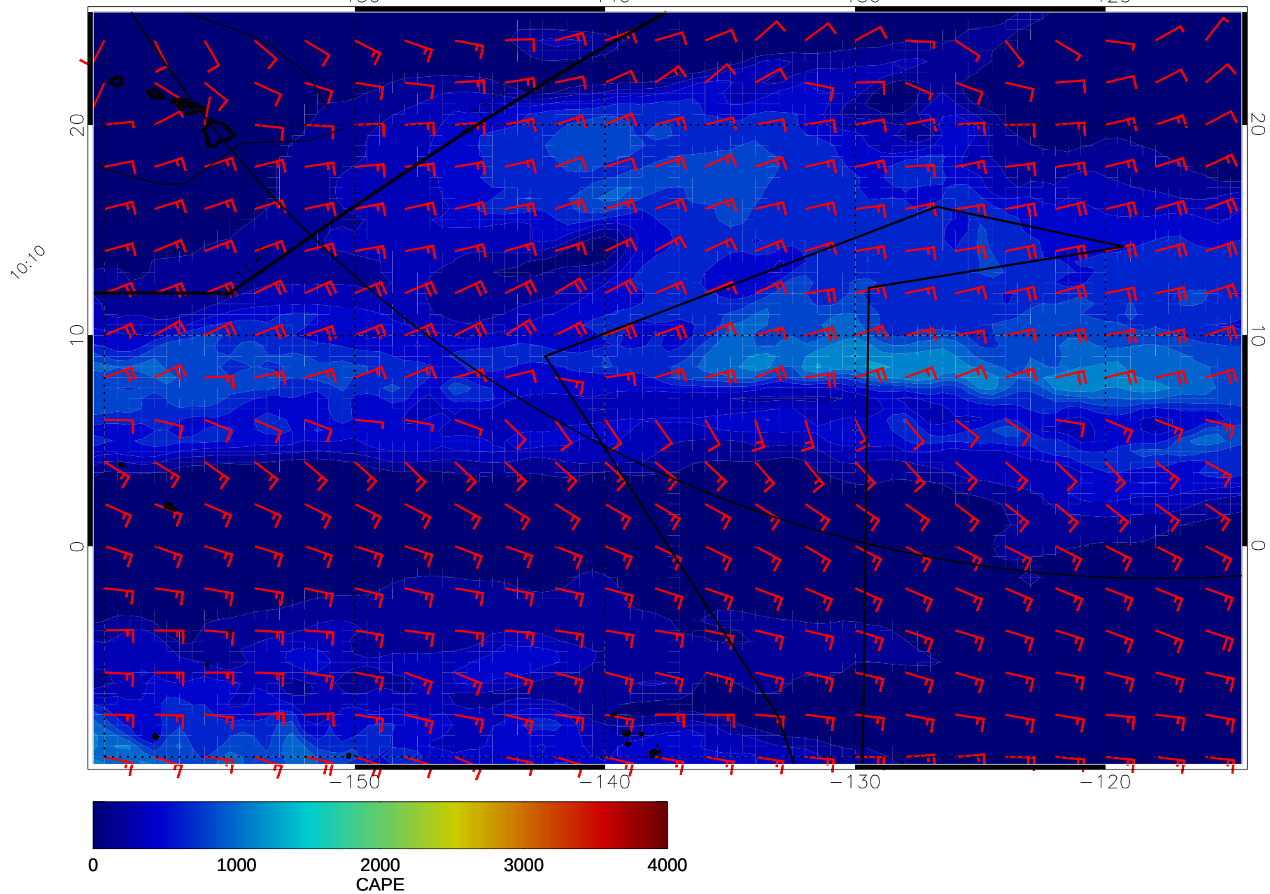
15011112, 108 hour forecast for CAPE and surface winds (knots) -- NCEP GFS
