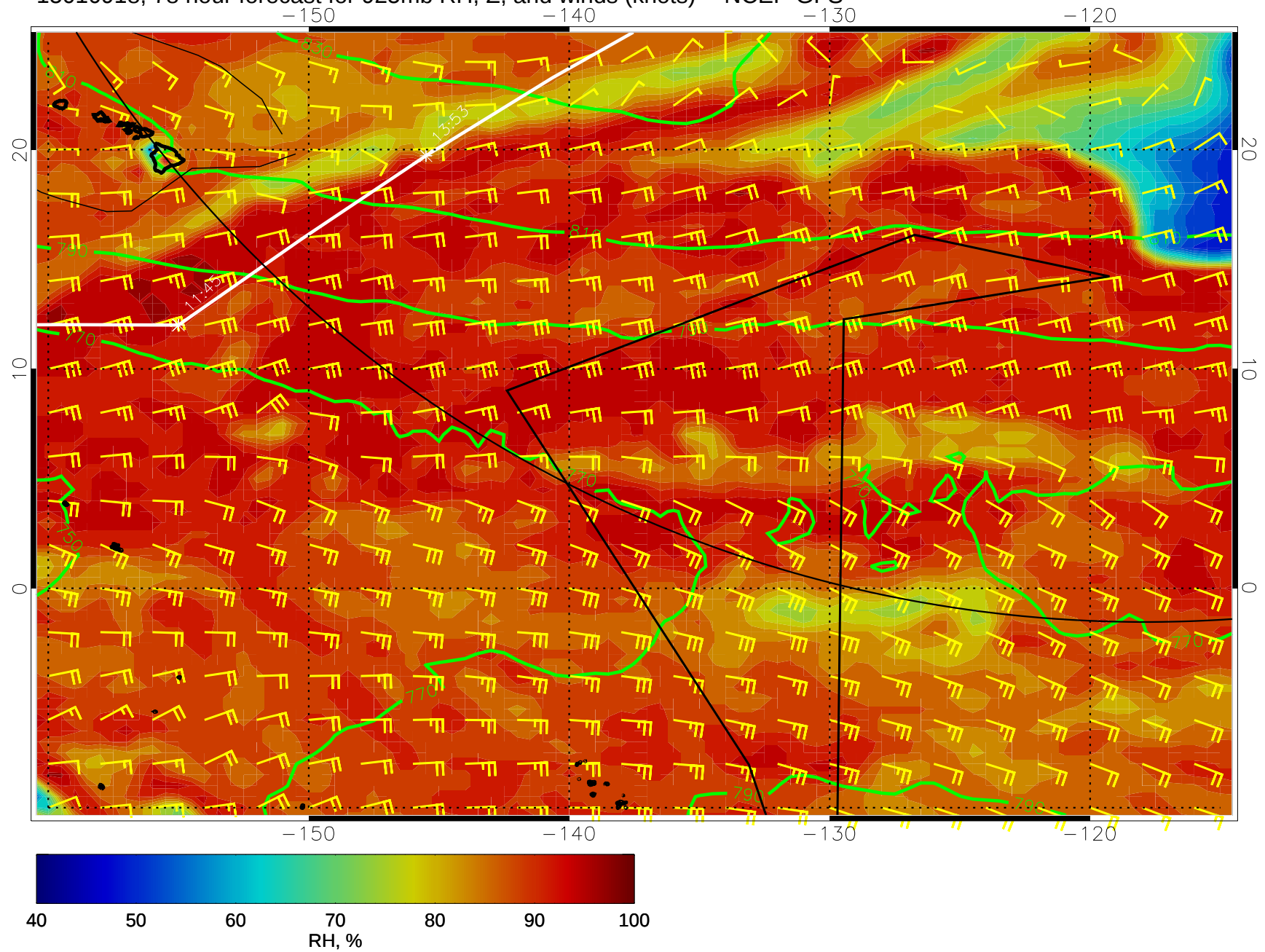
15010918, 78 hour forecast for 925mb RH, Z, and winds (knots) -- NCEP GFS
