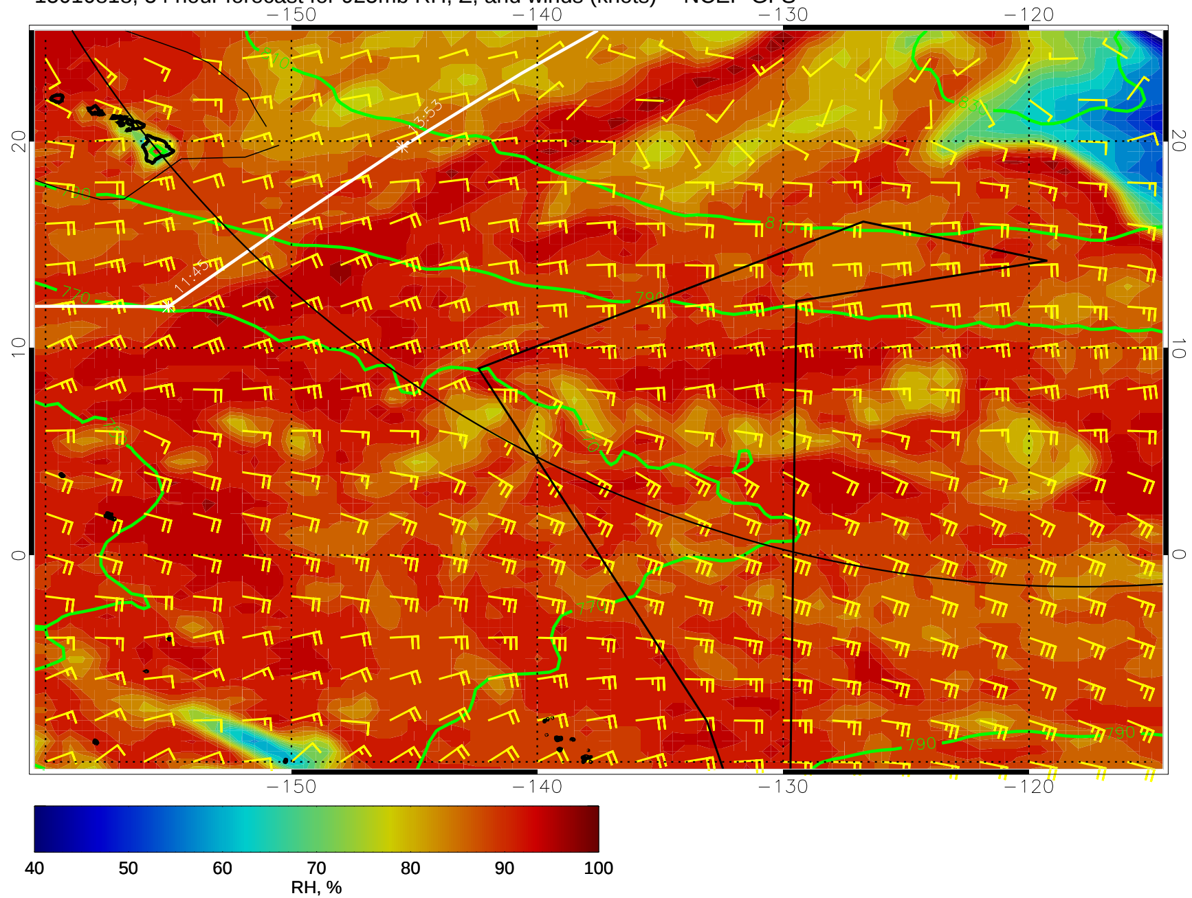
15010818, 54 hour forecast for 925mb RH, Z, and winds (knots) -- NCEP GFS
