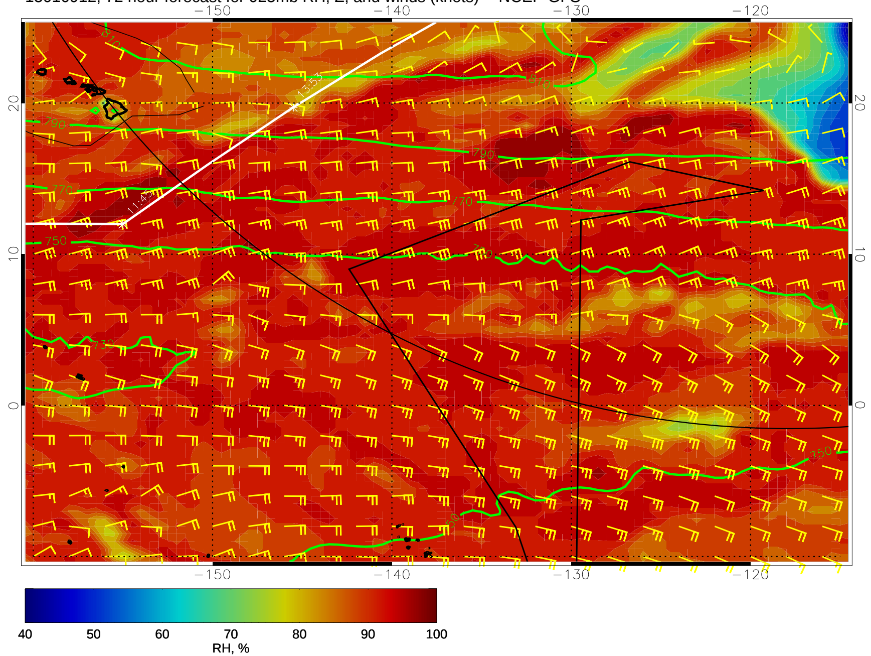
15010912, 72 hour forecast for 925mb RH, Z, and winds (knots) -- NCEP GFS
