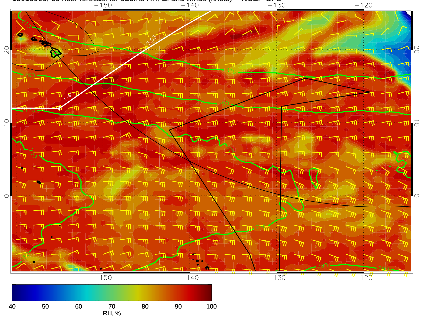
15010906, 66 hour forecast for 925mb RH, Z, and winds (knots) -- NCEP GFS
