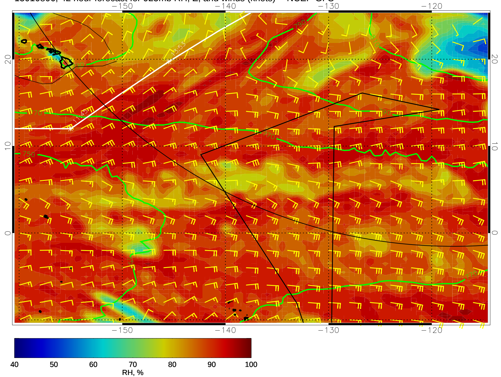
15010806, 42 hour forecast for 925mb RH, Z, and winds (knots) -- NCEP GFS
