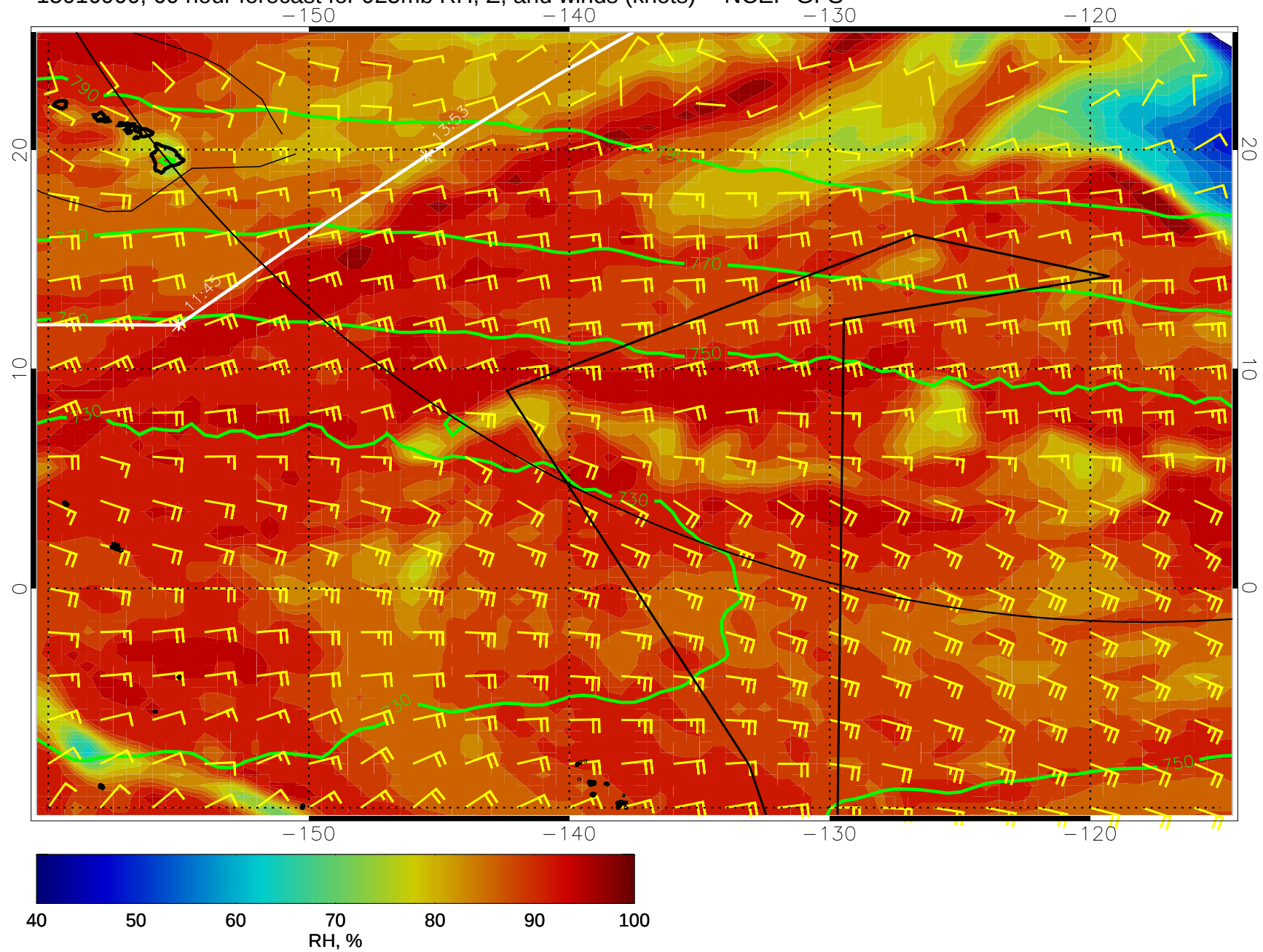
15010900, 60 hour forecast for 925mb RH, Z, and winds (knots) -- NCEP GFS
