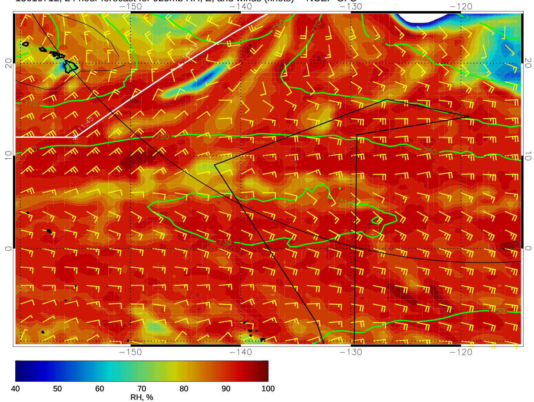
15010712, 24 hour forecast for 925mb RH, Z, and winds (knots) -- NCEP GFS
