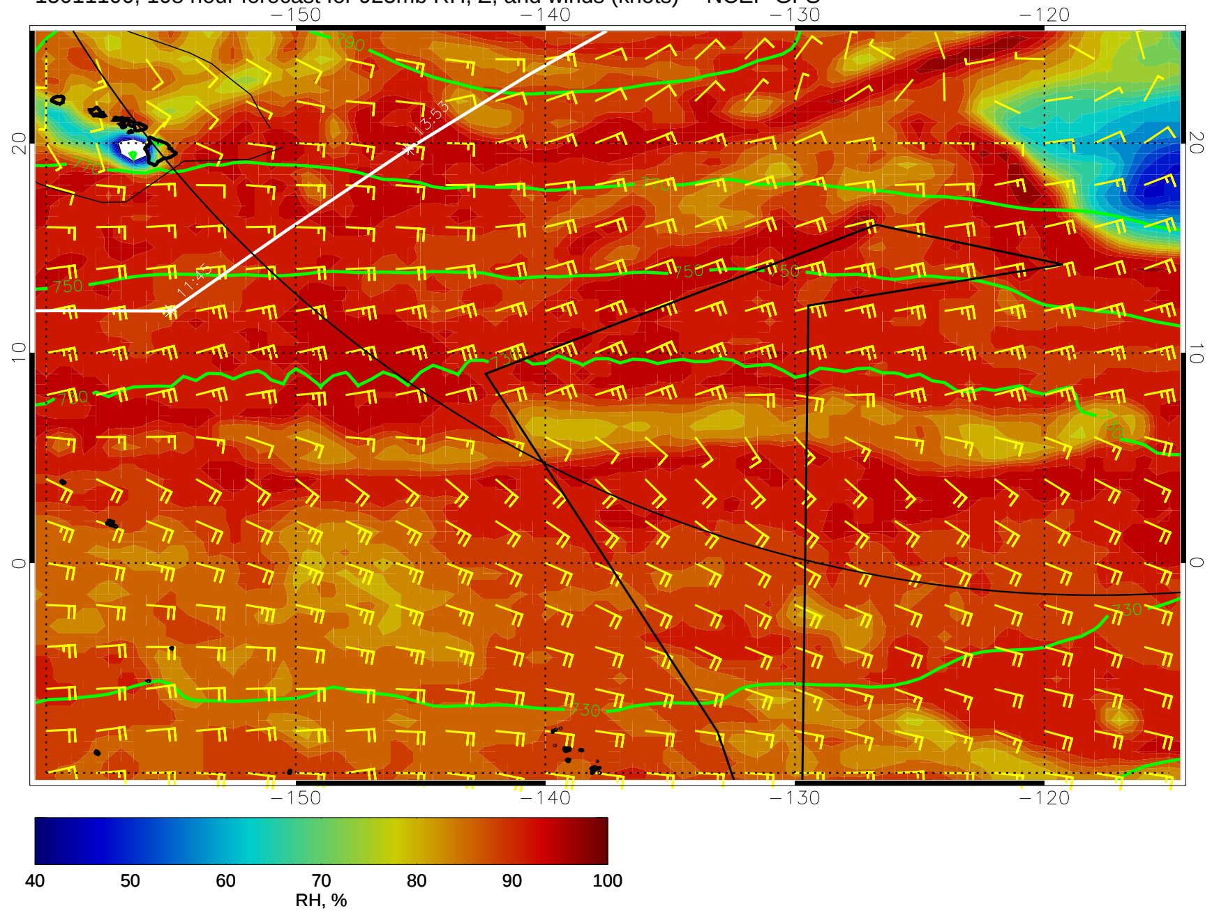
15011100, 108 hour forecast for 925mb RH, Z, and winds (knots) -- NCEP GFS
