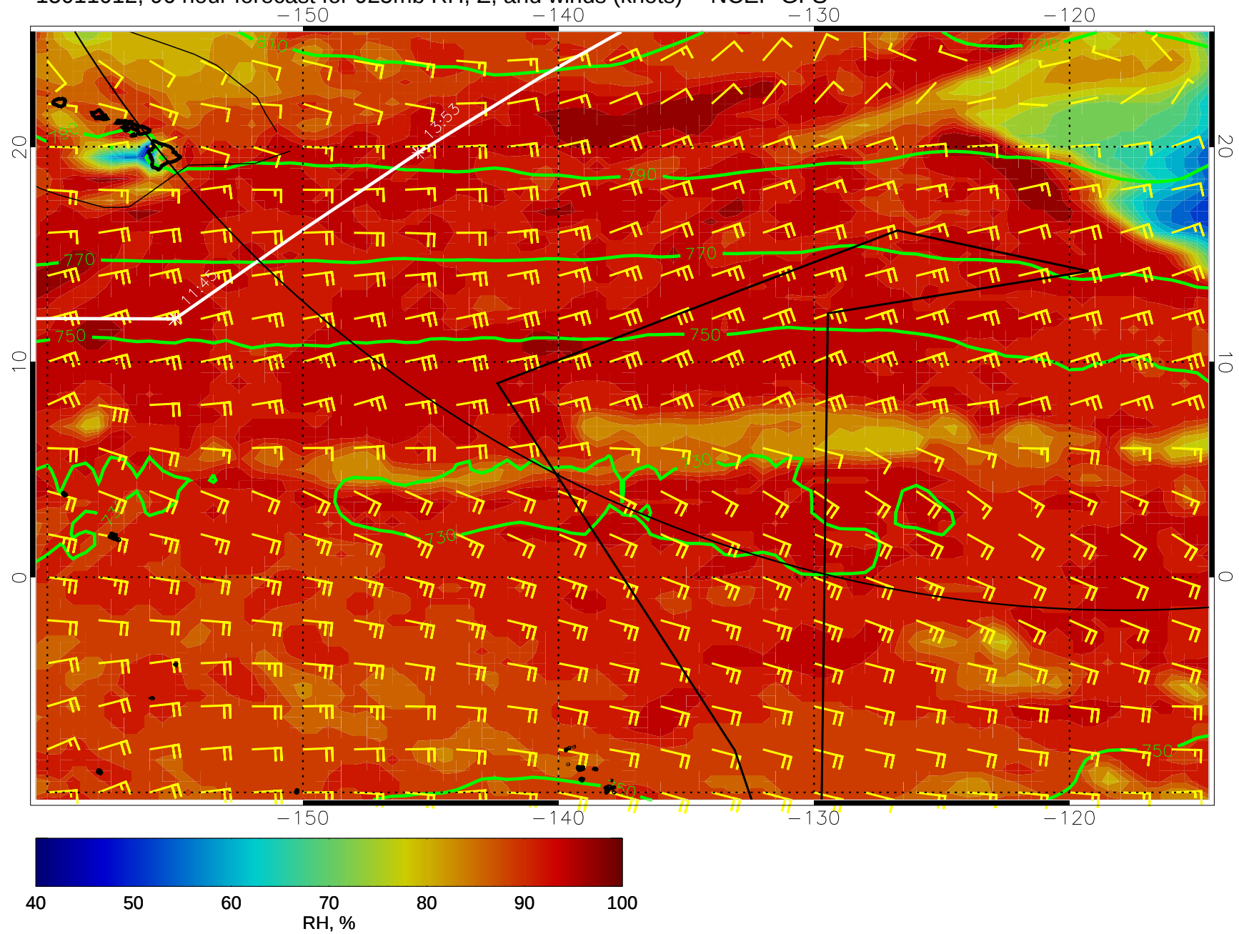
15011012, 96 hour forecast for 925mb RH, Z, and winds (knots) -- NCEP GFS
