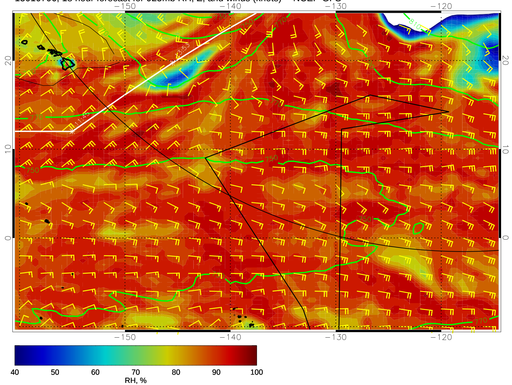
15010706, 18 hour forecast for 925mb RH, Z, and winds (knots) -- NCEP GFS
