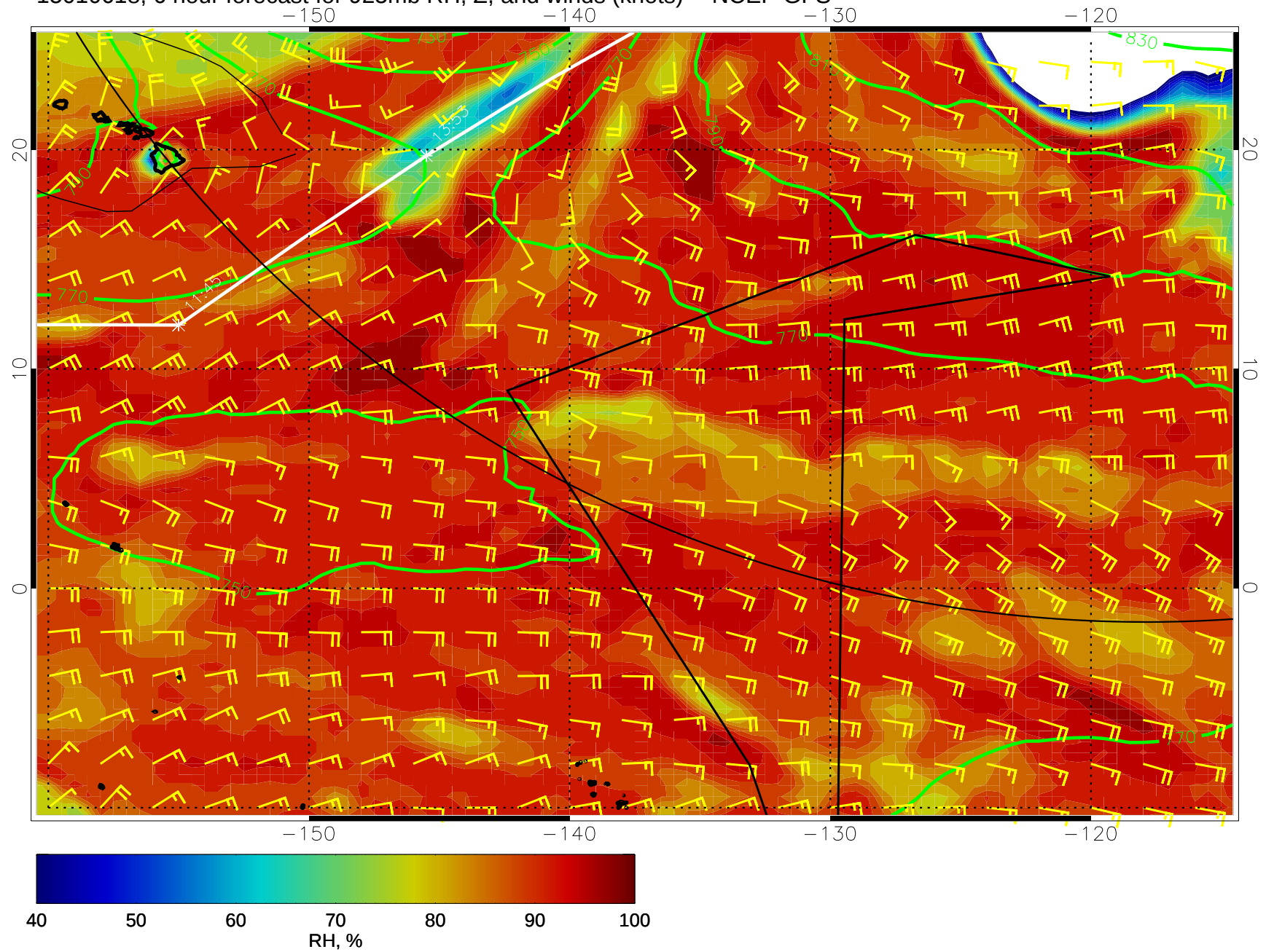
15010618, 6 hour forecast for 925mb RH, Z, and winds (knots) -- NCEP GFS
