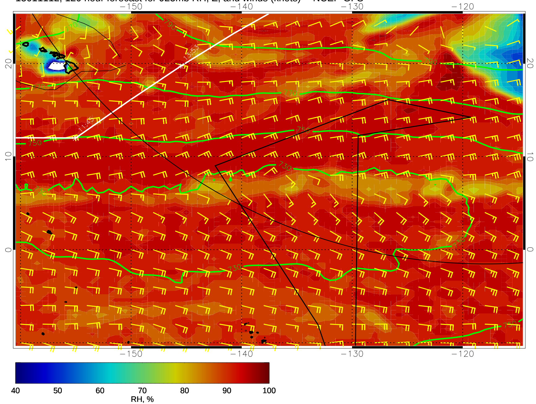
15011112, 120 hour forecast for 925mb RH, Z, and winds (knots) -- NCEP GFS
