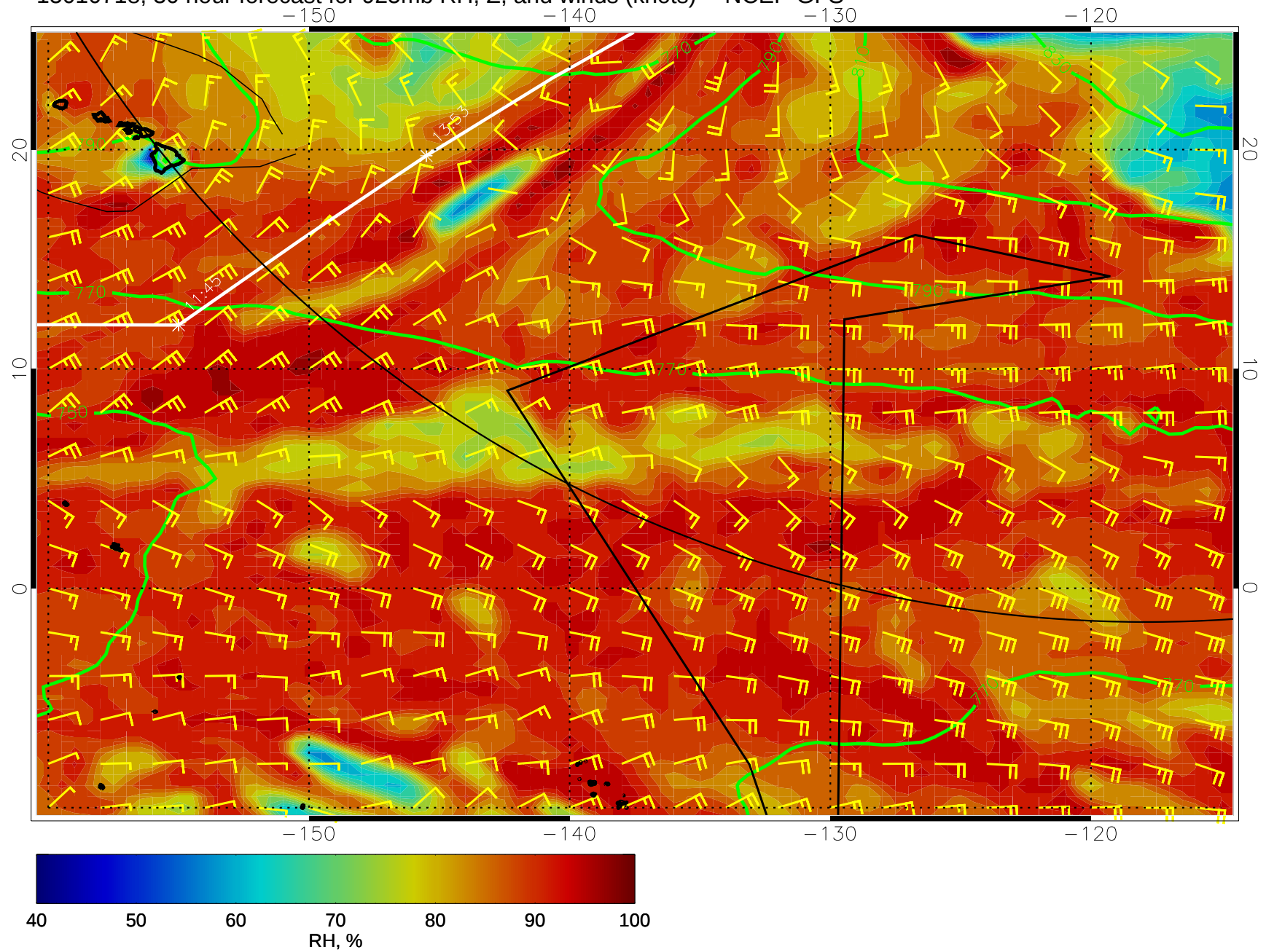
15010718, 30 hour forecast for 925mb RH, Z, and winds (knots) -- NCEP GFS
