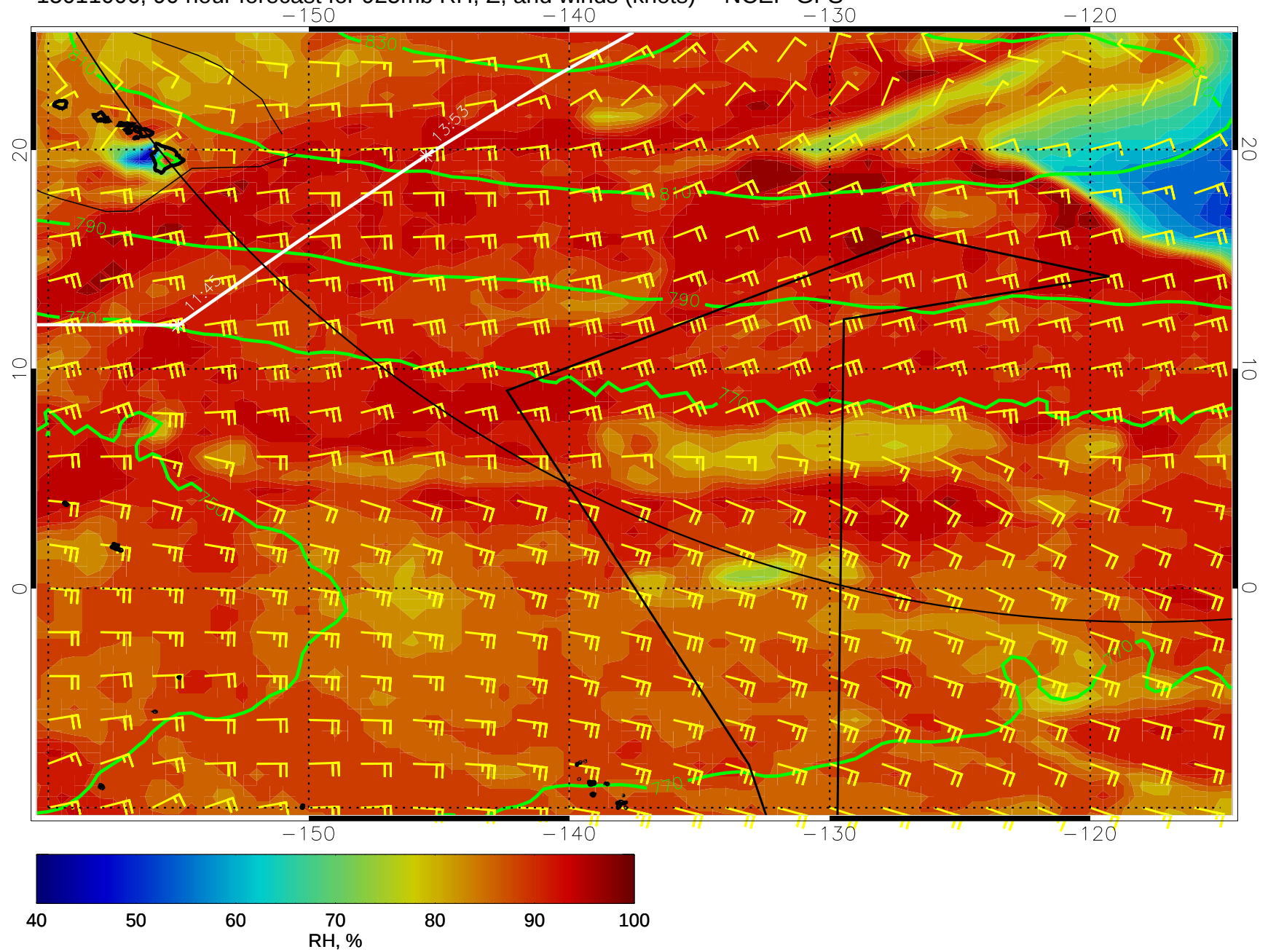
15011006, 90 hour forecast for 925mb RH, Z, and winds (knots) -- NCEP GFS
