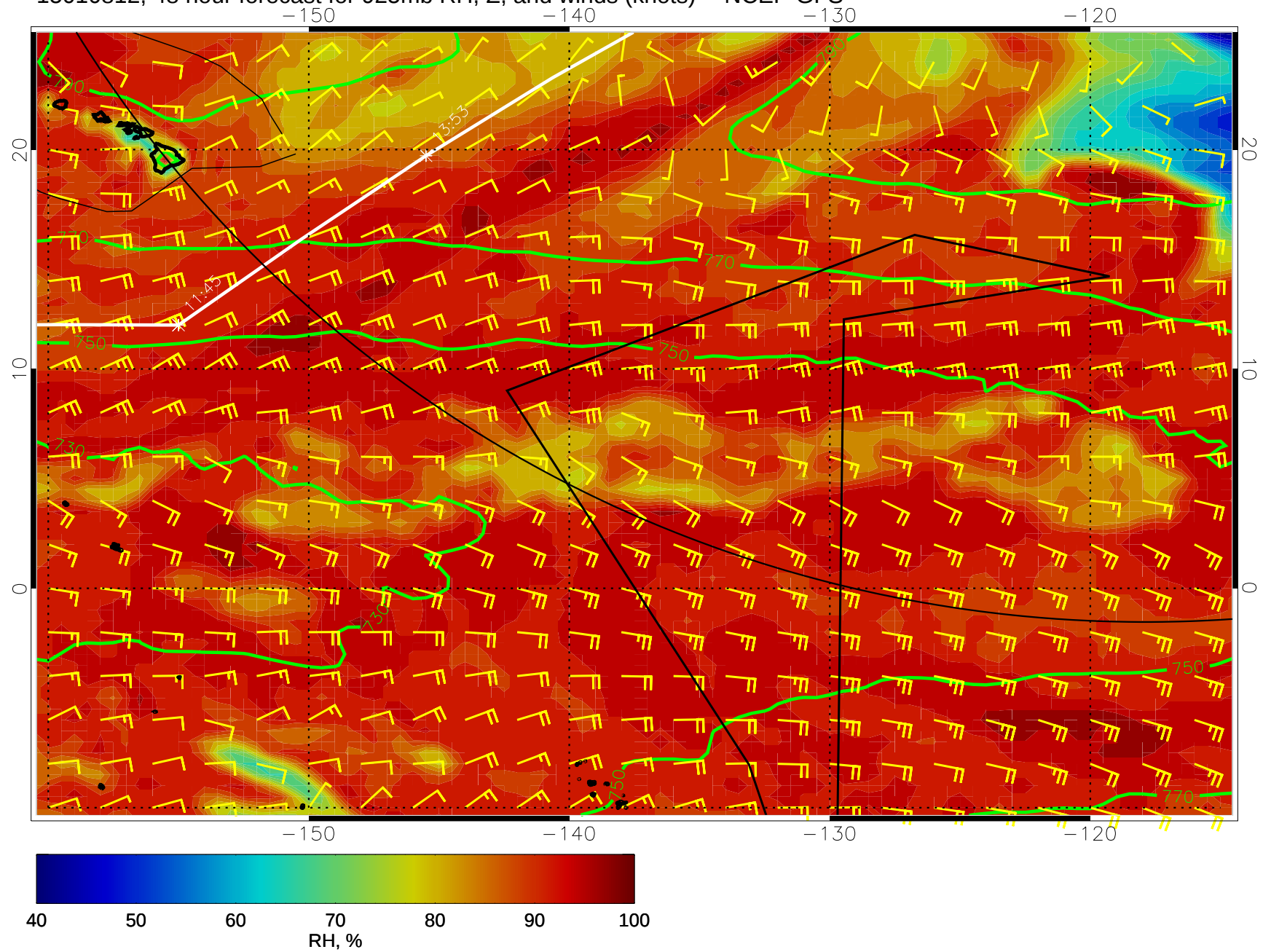
15010812, 48 hour forecast for 925mb RH, Z, and winds (knots) -- NCEP GFS
