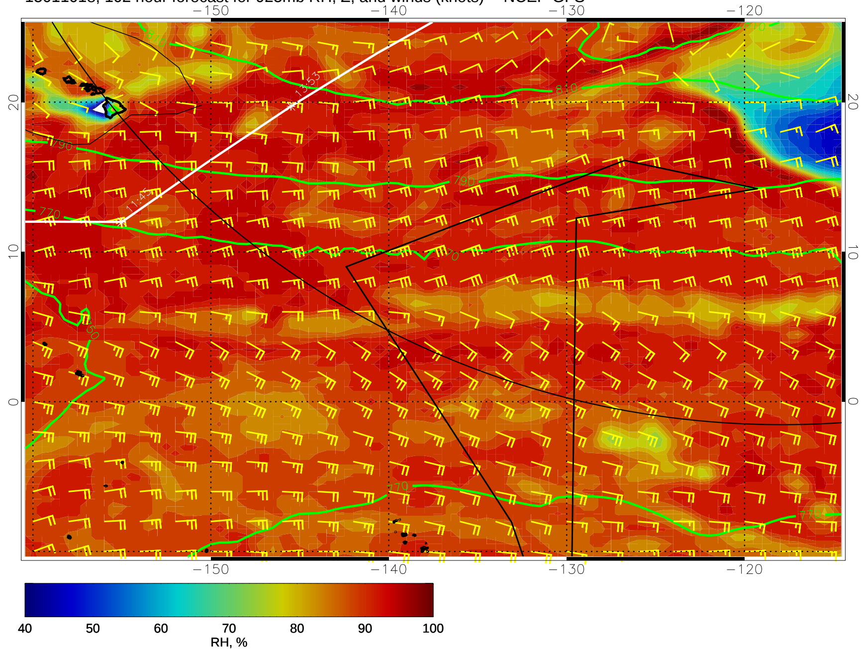
15011018, 102 hour forecast for 925mb RH, Z, and winds (knots) -- NCEP GFS
