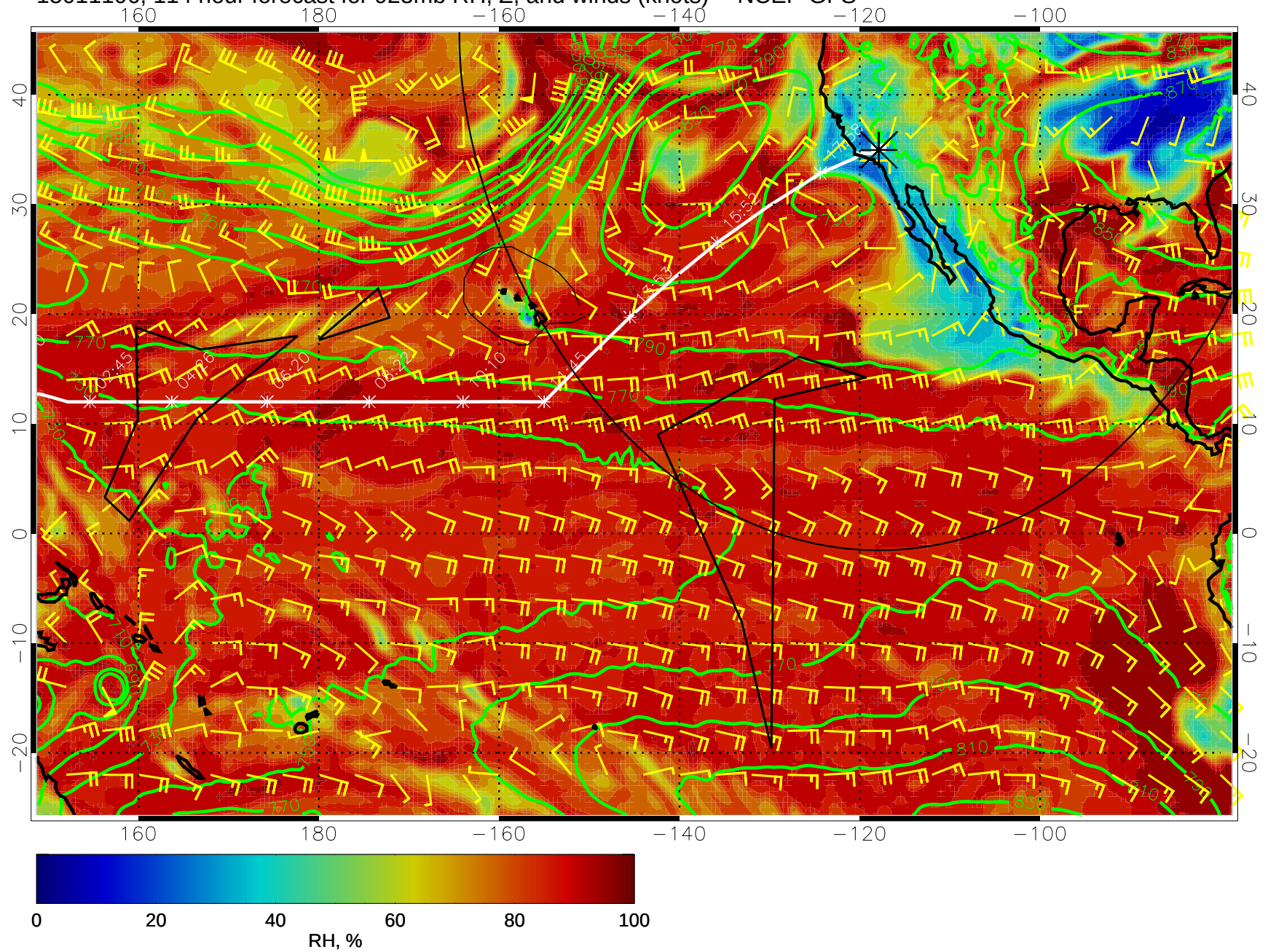
15011106, 114 hour forecast for 925mb RH, Z, and winds (knots) -- NCEP GFS
