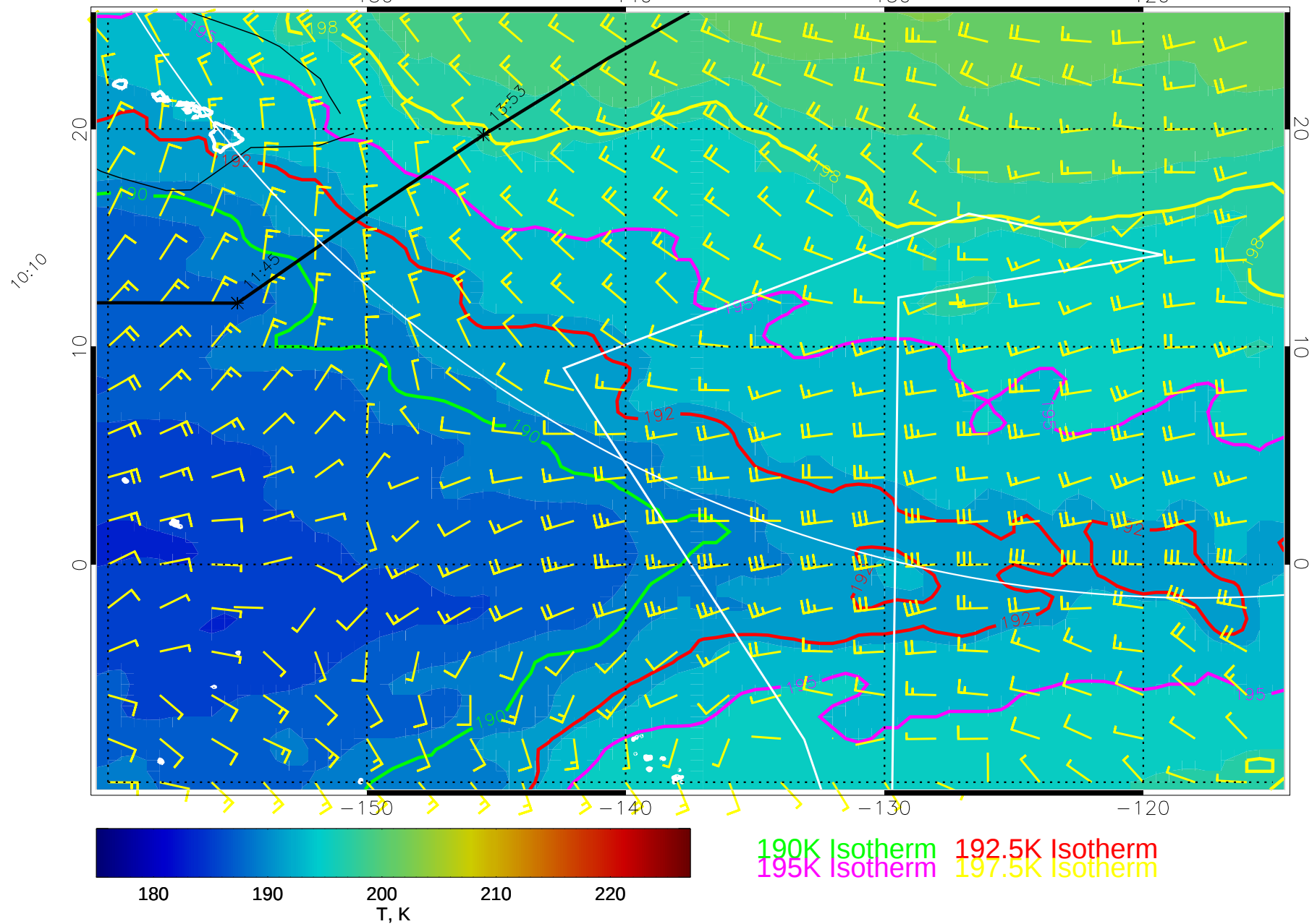
15011106, 114 hour forecast for 70mb T and winds (knots) -- NCEP GFS
