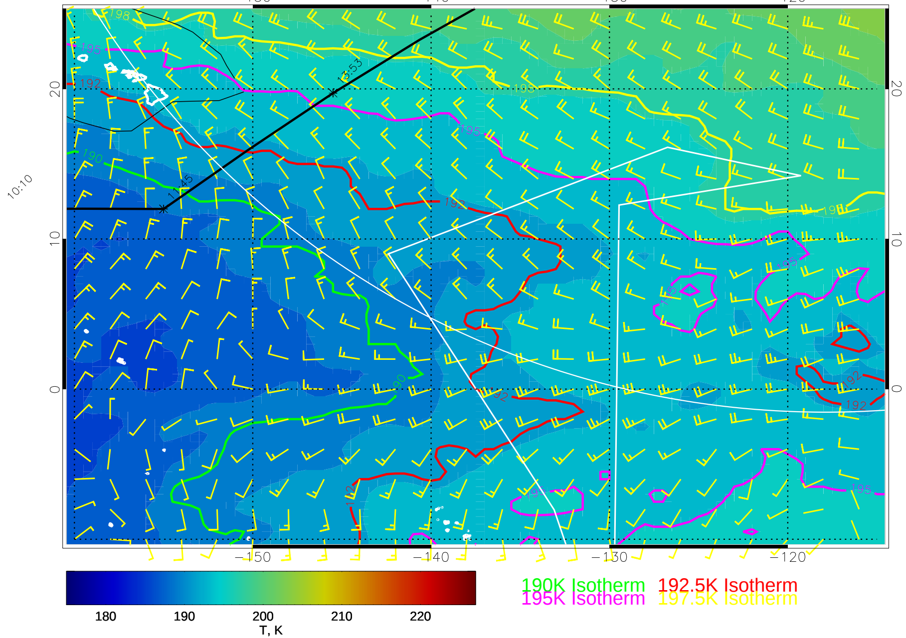
15011012, 96 hour forecast for 70mb T and winds (knots) -- NCEP GFS
