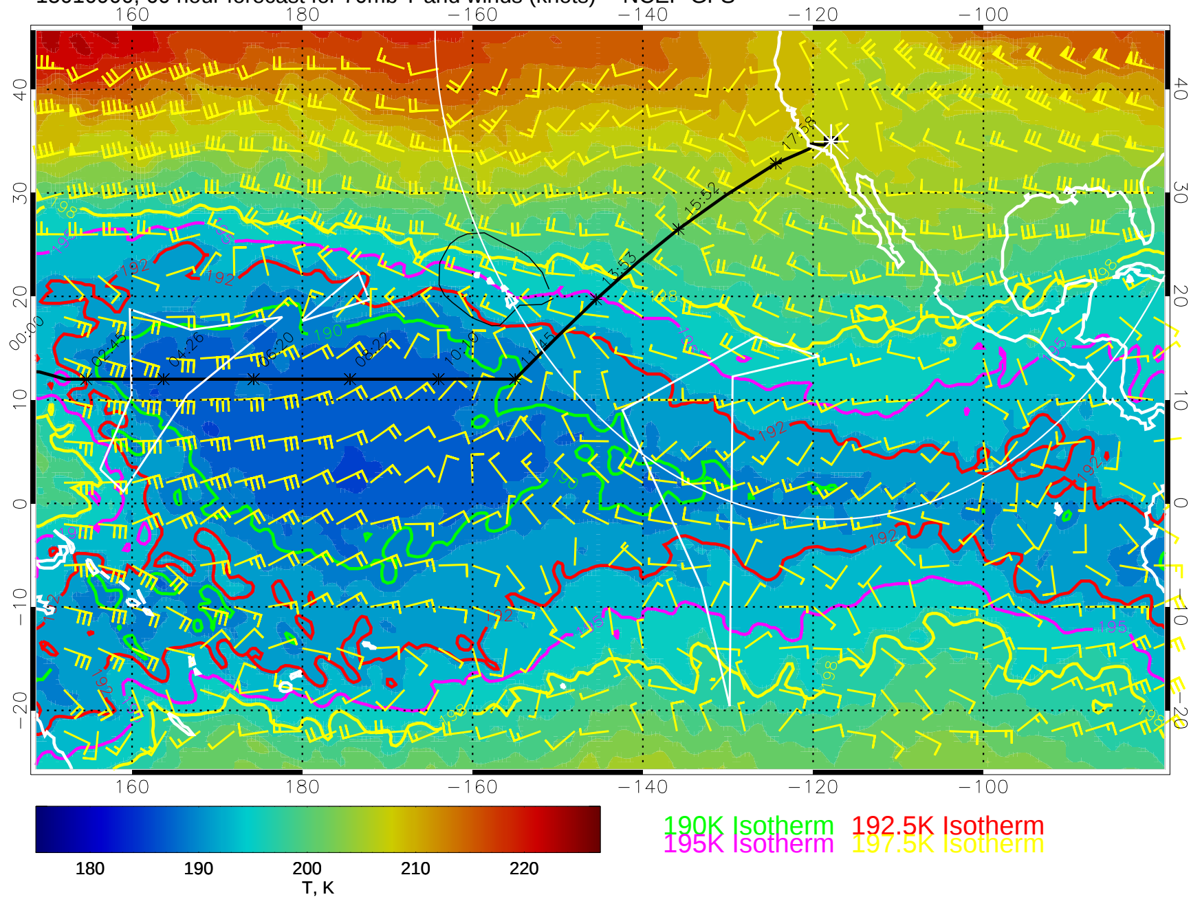
15010900, 60 hour forecast for 70mb T and winds (knots) -- NCEP GFS
