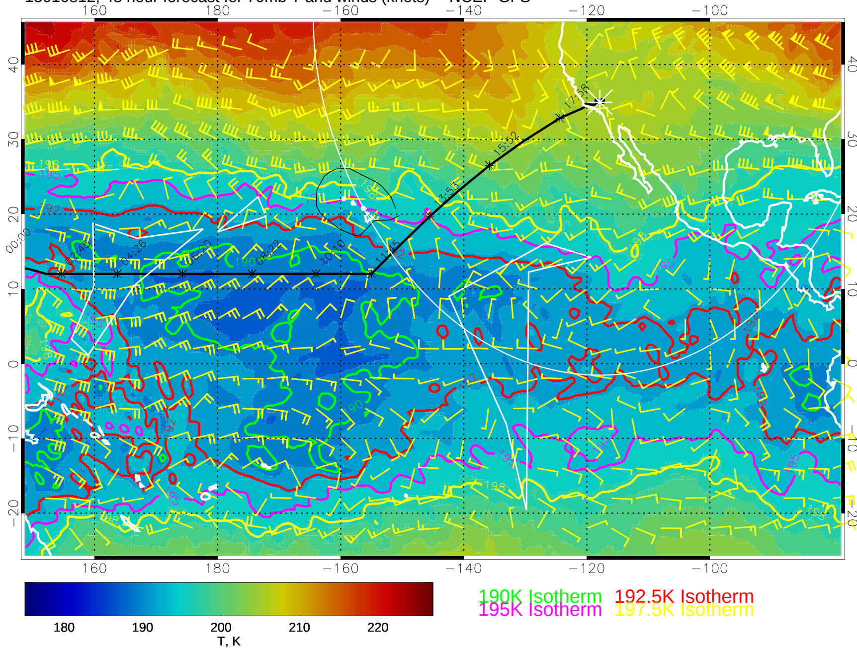
15010812, 48 hour forecast for 70mb T and winds (knots) -- NCEP GFS
