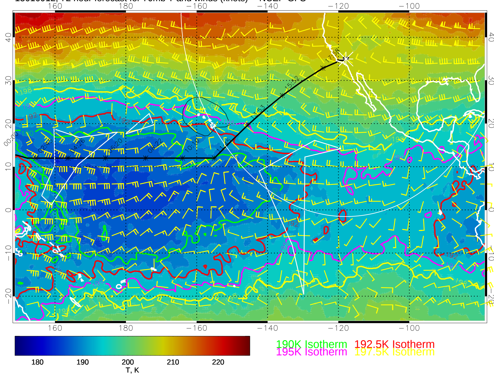
15010912, 72 hour forecast for 70mb T and winds (knots) -- NCEP GFS
