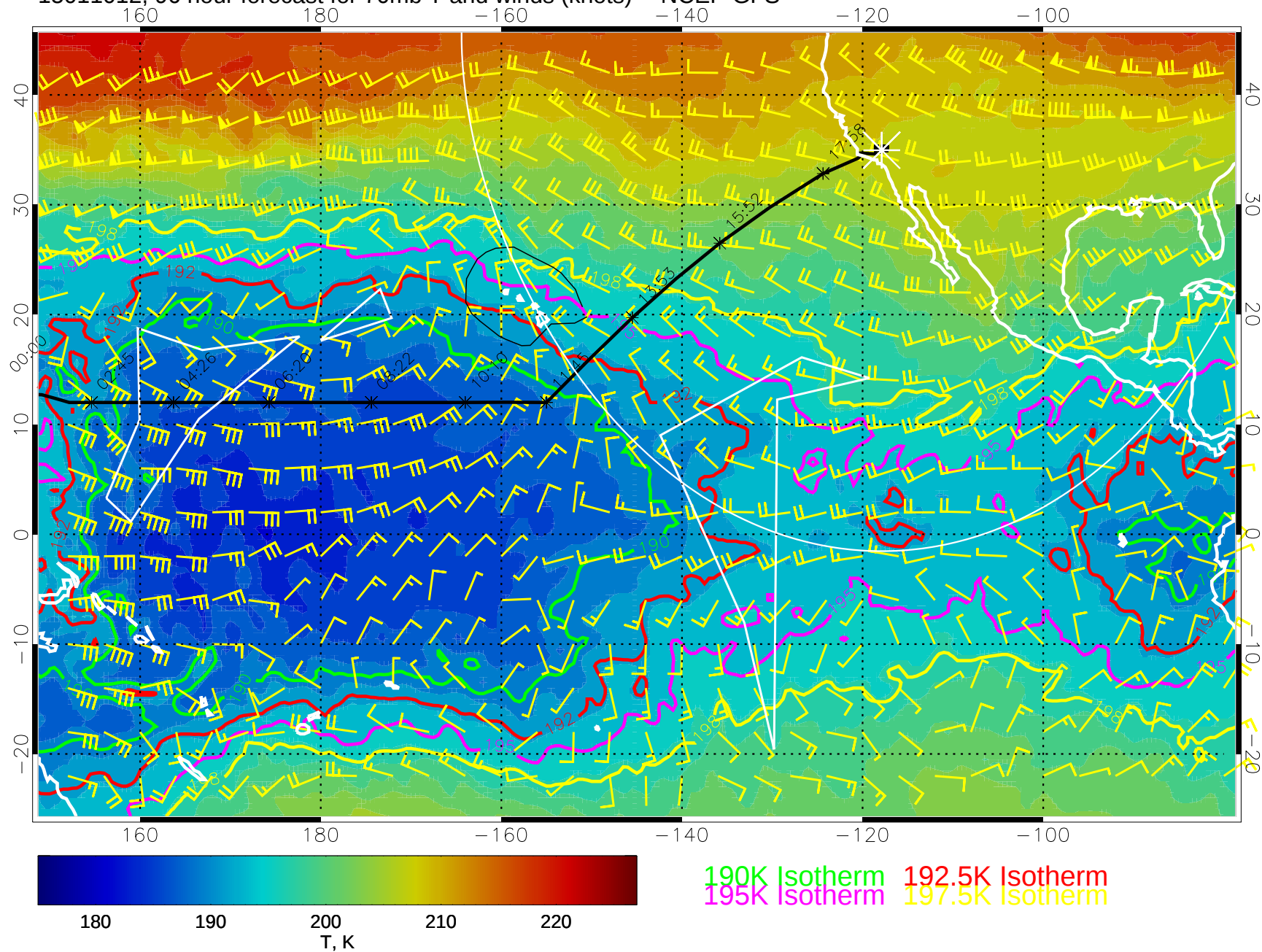
15011012, 96 hour forecast for 70mb T and winds (knots) -- NCEP GFS
