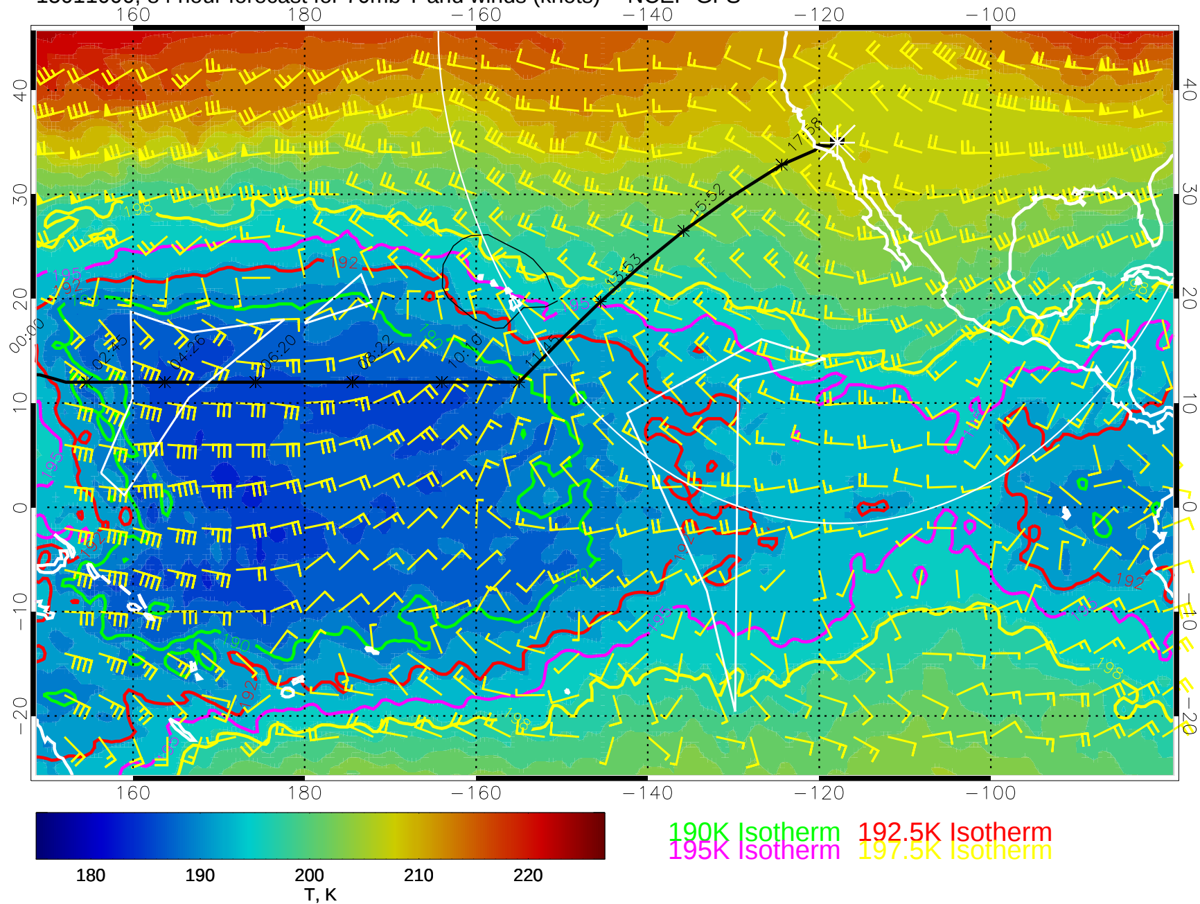
15011000, 84 hour forecast for 70mb T and winds (knots) -- NCEP GFS
