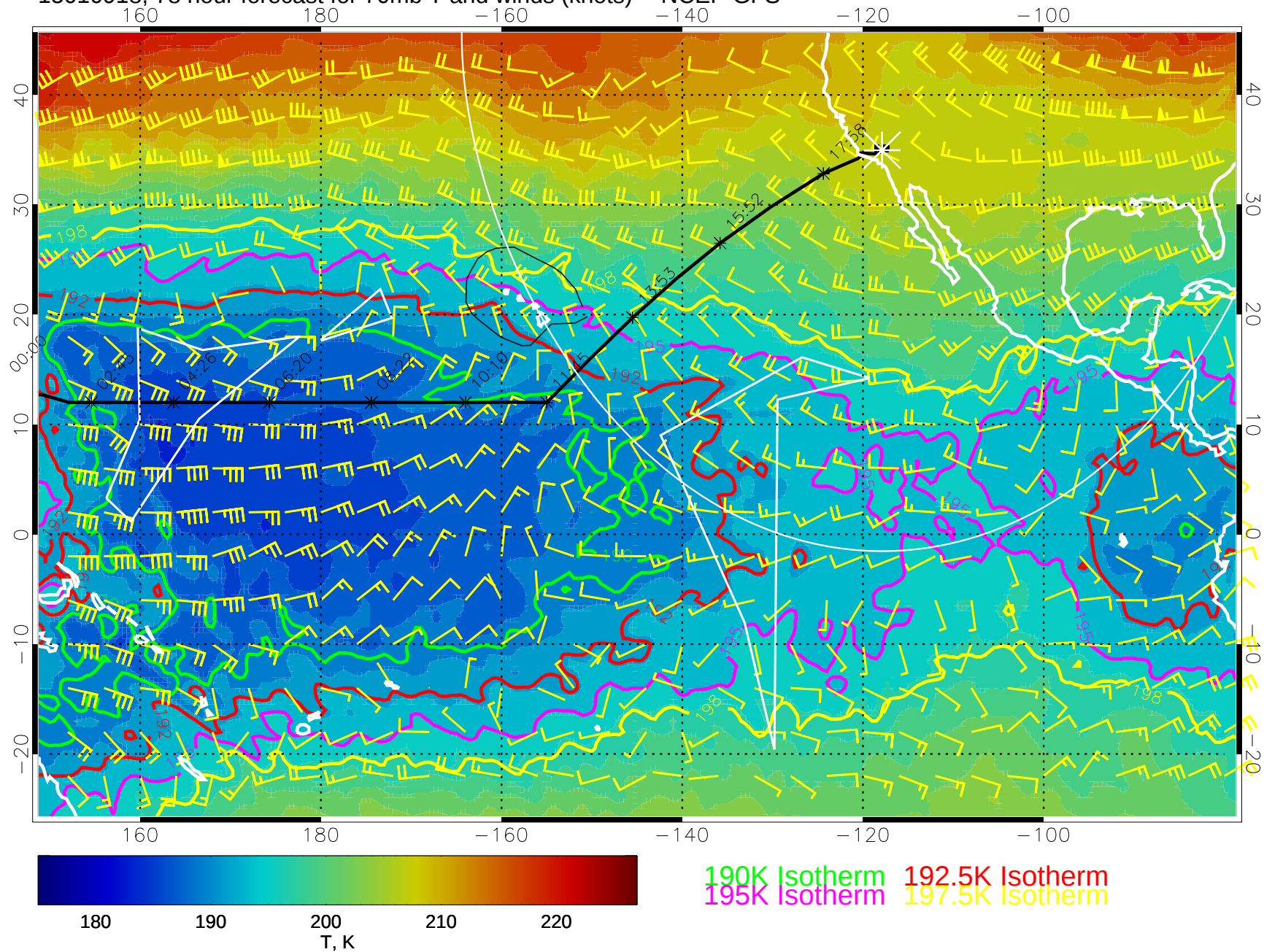
15010918, 78 hour forecast for 70mb T and winds (knots) -- NCEP GFS
