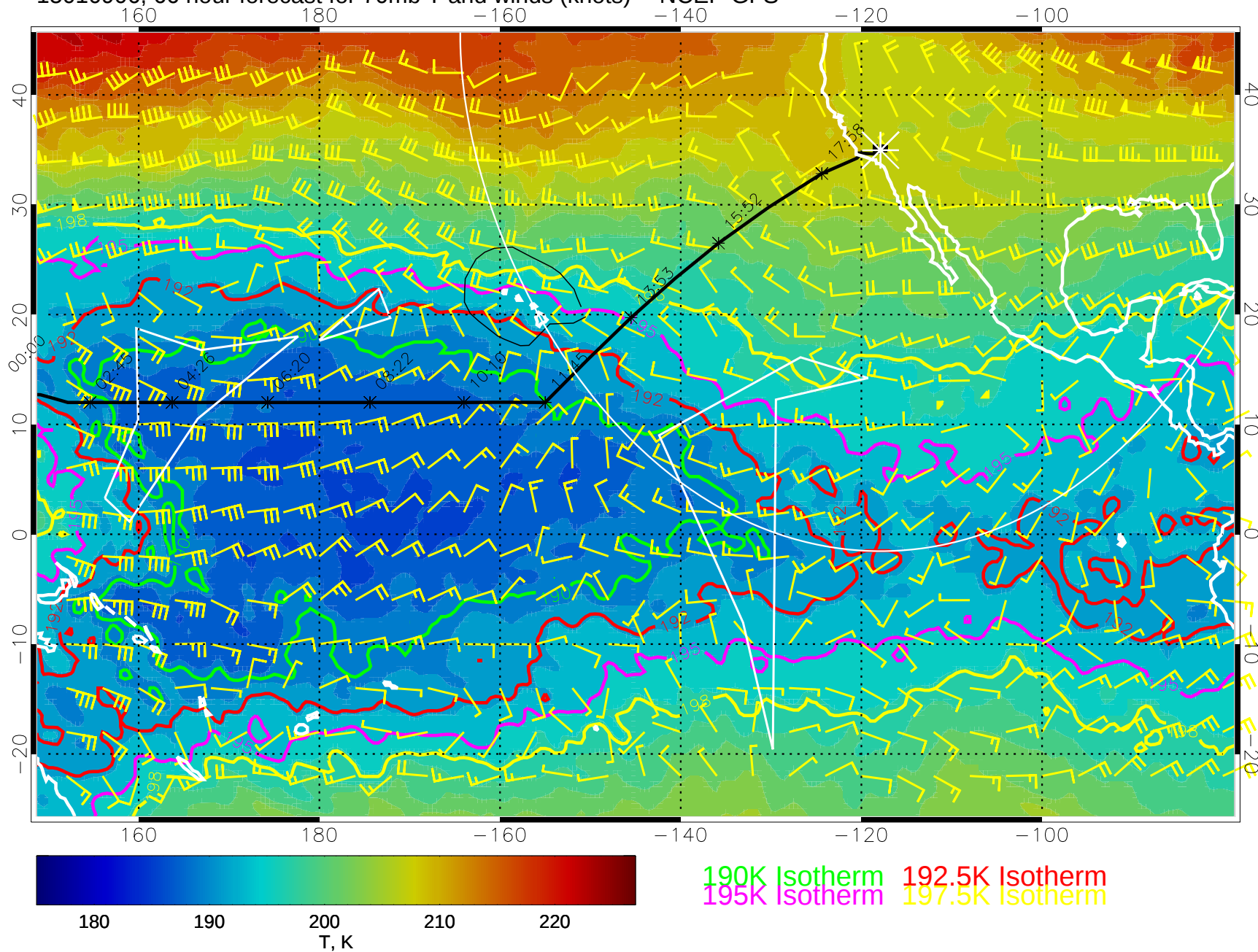
15010906, 66 hour forecast for 70mb T and winds (knots) -- NCEP GFS
