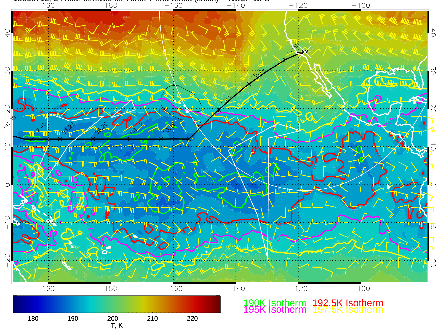
15010712, 24 hour forecast for 70mb T and winds (knots) -- NCEP GFS
