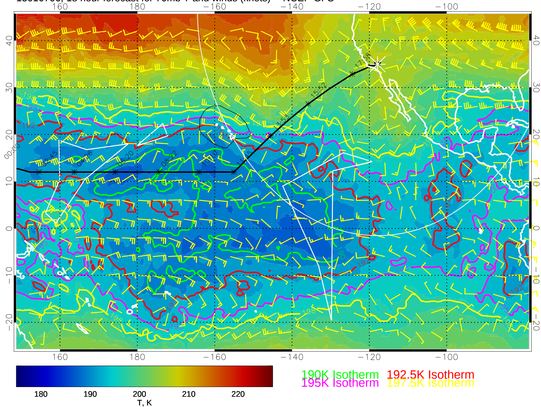
15010706, 18 hour forecast for 70mb T and winds (knots) -- NCEP GFS
