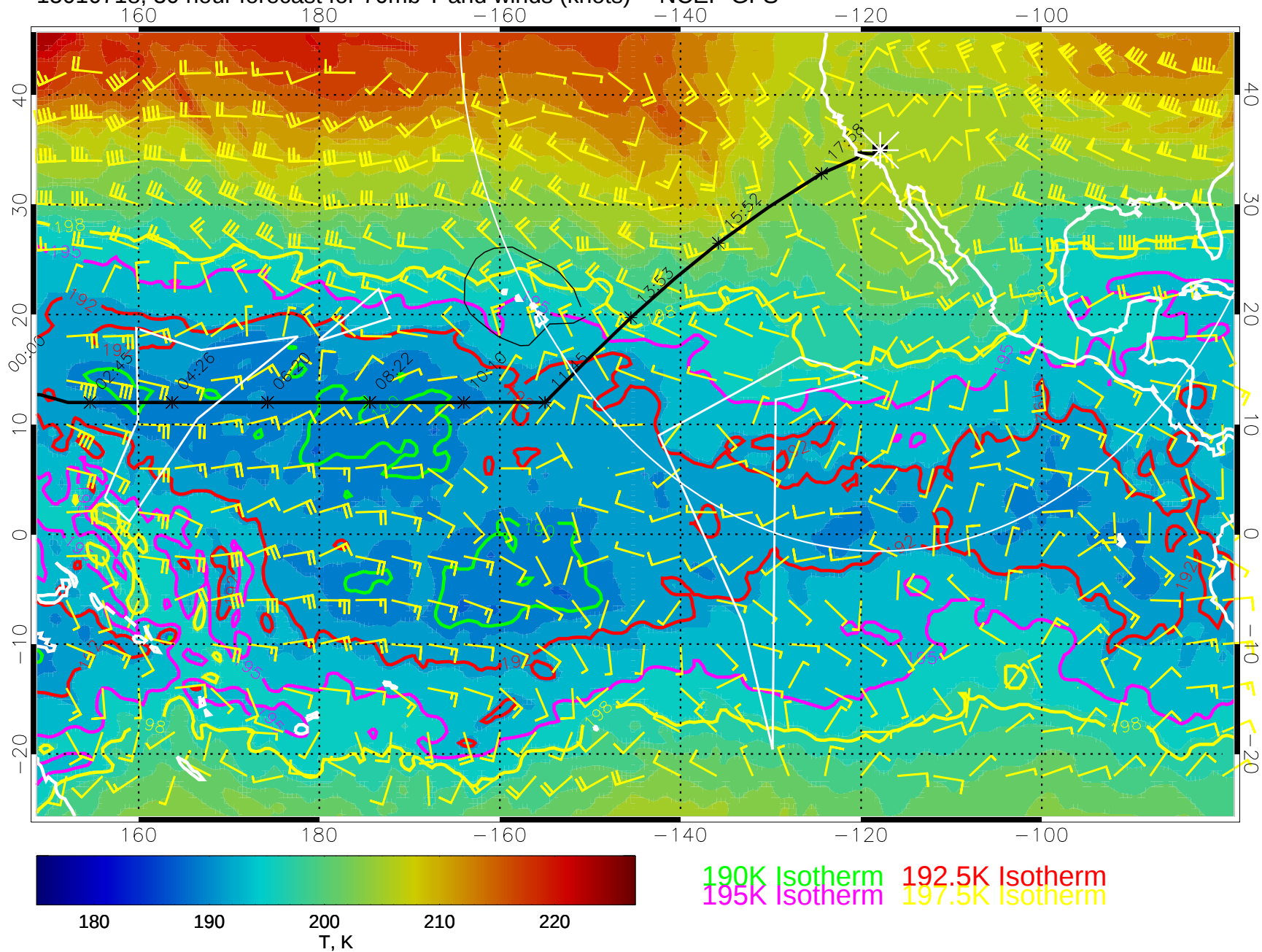
15010718, 30 hour forecast for 70mb T and winds (knots) -- NCEP GFS
