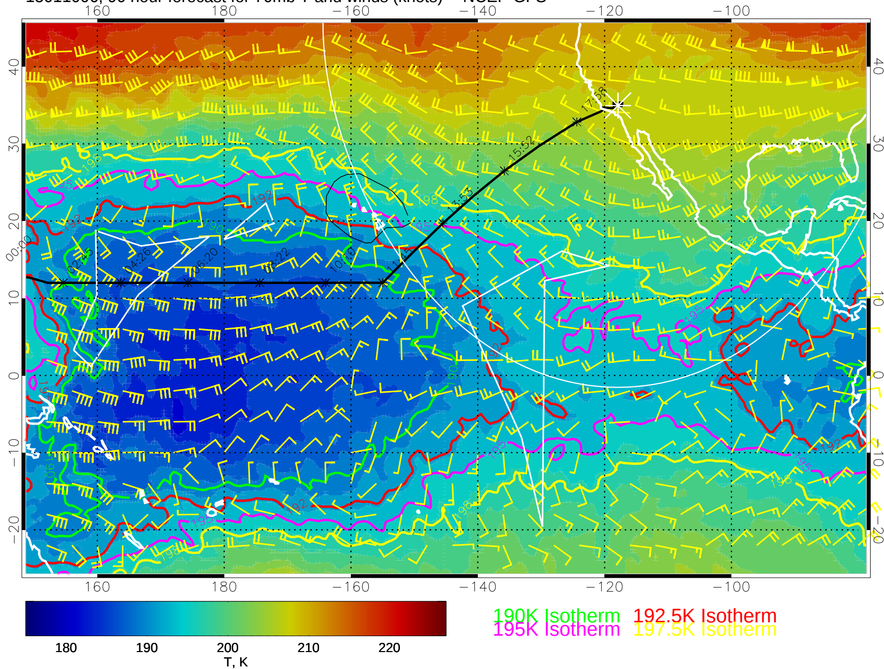
15011006, 90 hour forecast for 70mb T and winds (knots) -- NCEP GFS
