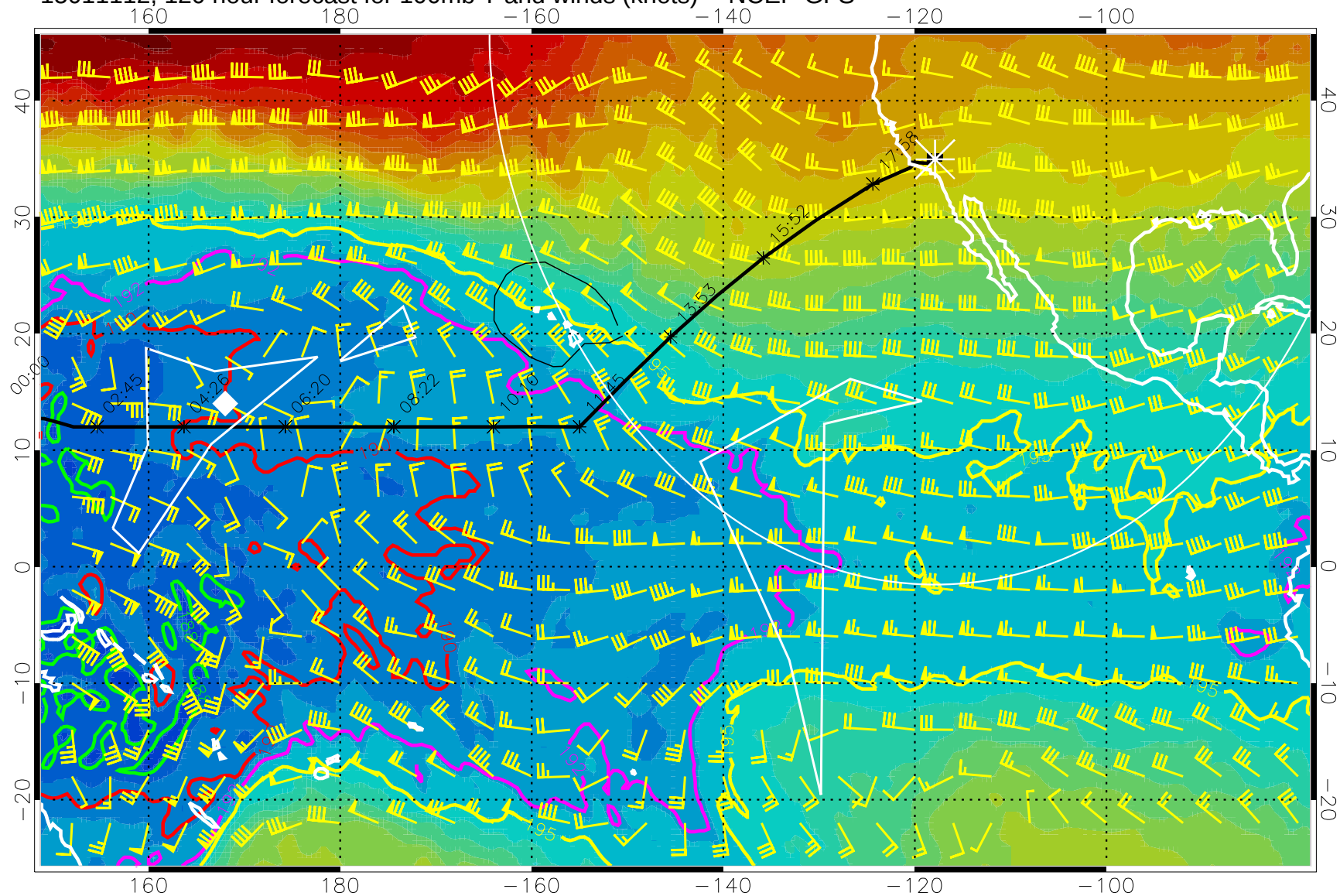
15011112, 120 hour forecast for 100mb T and winds (knots) -- NCEP GFS
