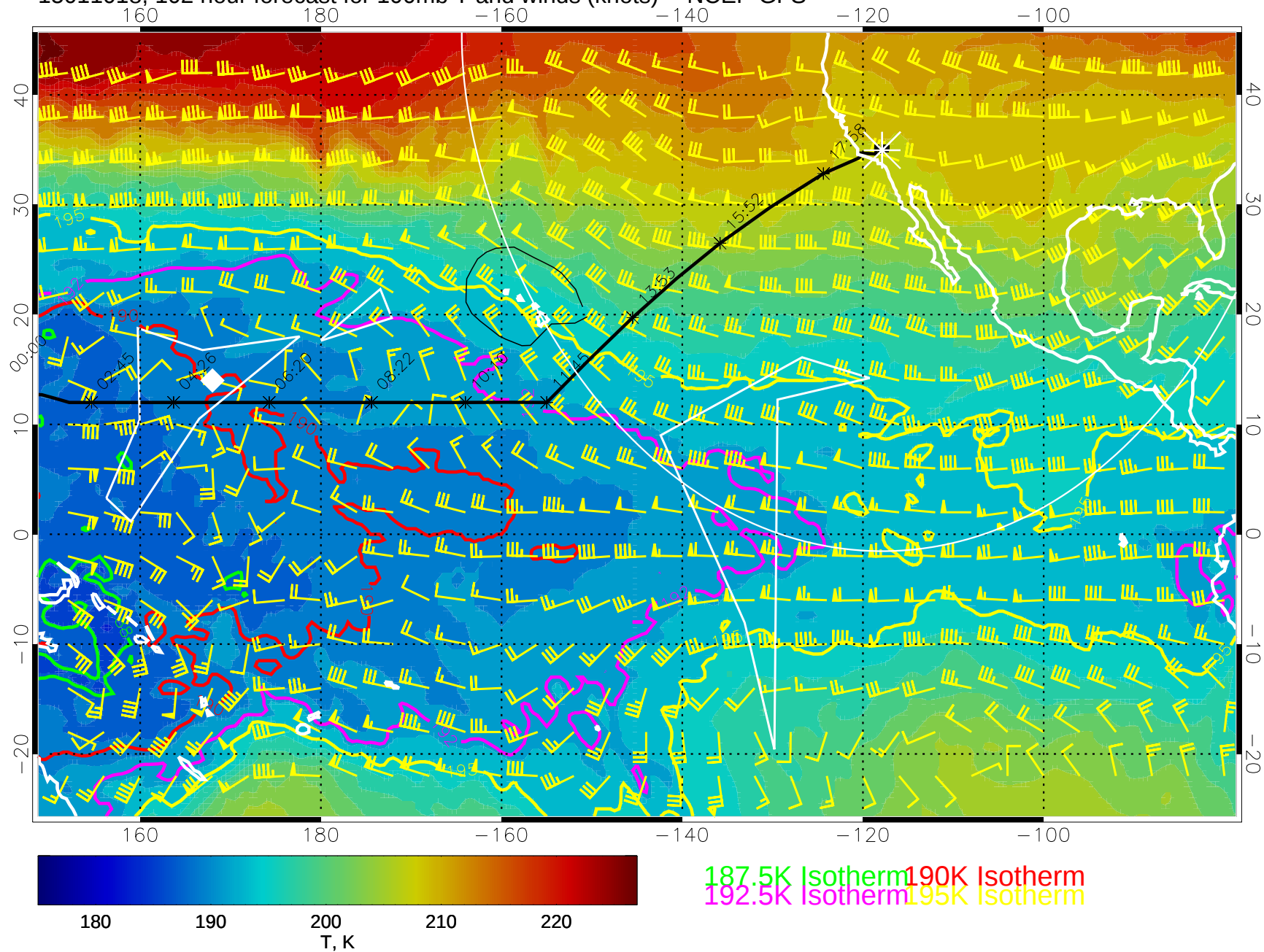
15011018, 102 hour forecast for 100mb T and winds (knots) -- NCEP GFS
