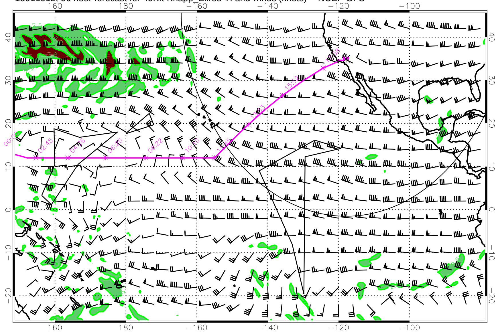
15011012, 96 hour forecast for 49Kft Knapp_Ellrod TI and winds (knots) -- NCEP GFS
