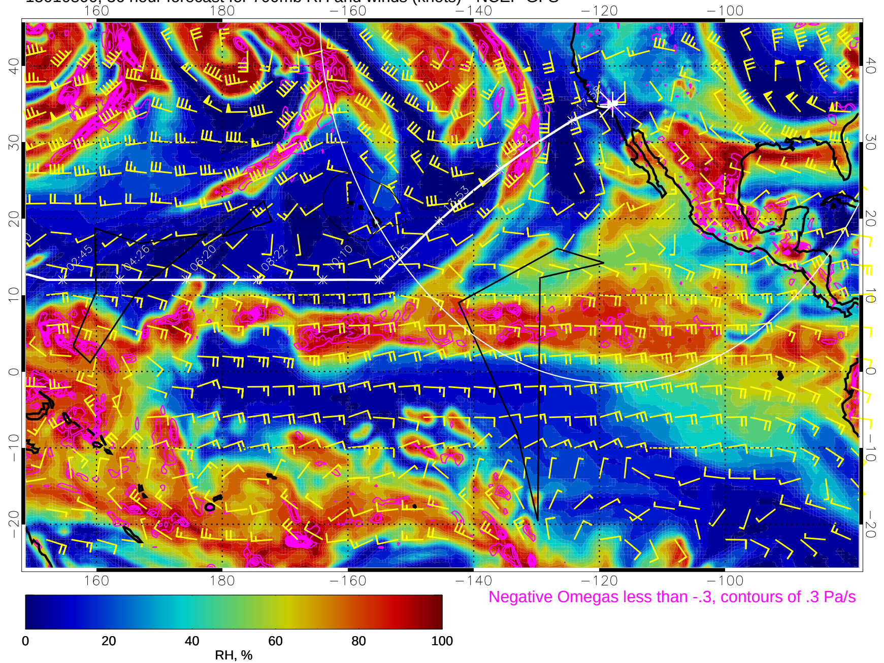
15010800, 36 hour forecast for 700mb RH and winds (knots) - NCEP GFS
