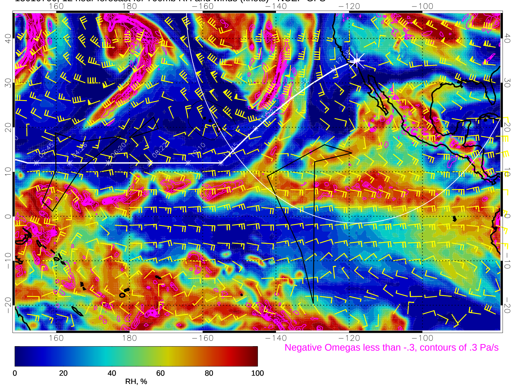
15010700, 12 hour forecast for 700mb RH and winds (knots) - NCEP GFS
