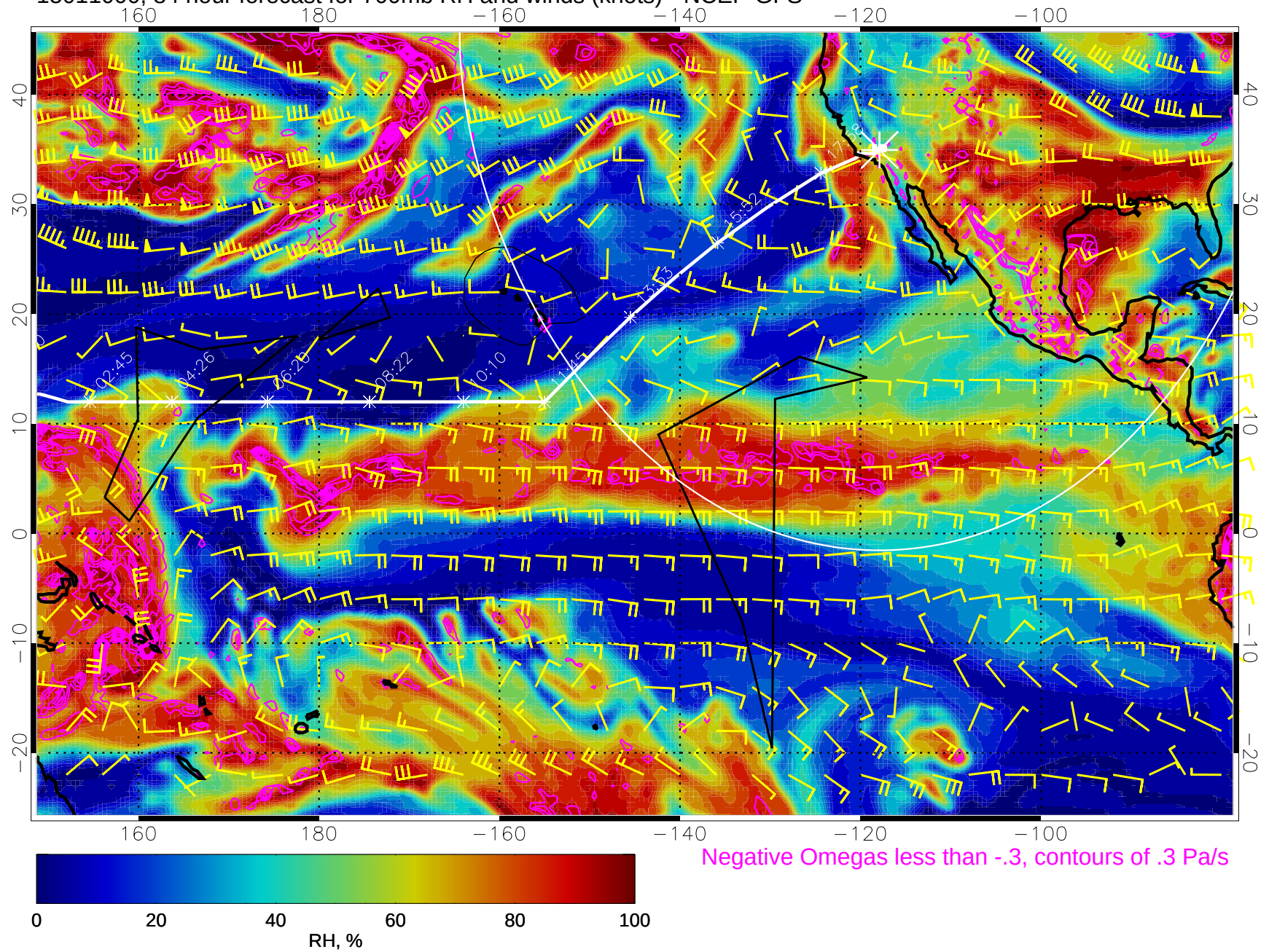
15011000, 84 hour forecast for 700mb RH and winds (knots) - NCEP GFS
