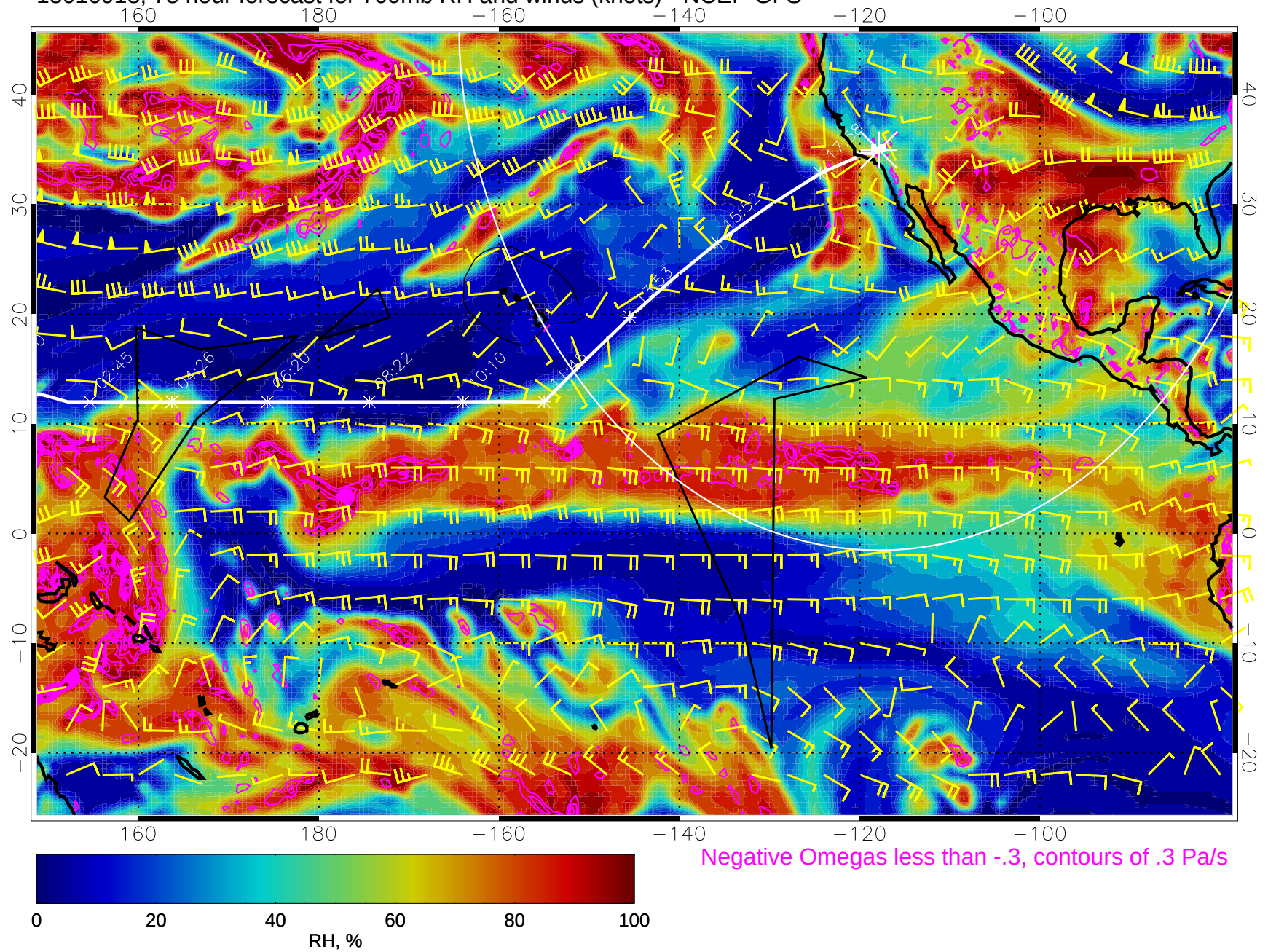
15010918, 78 hour forecast for 700mb RH and winds (knots) - NCEP GFS
