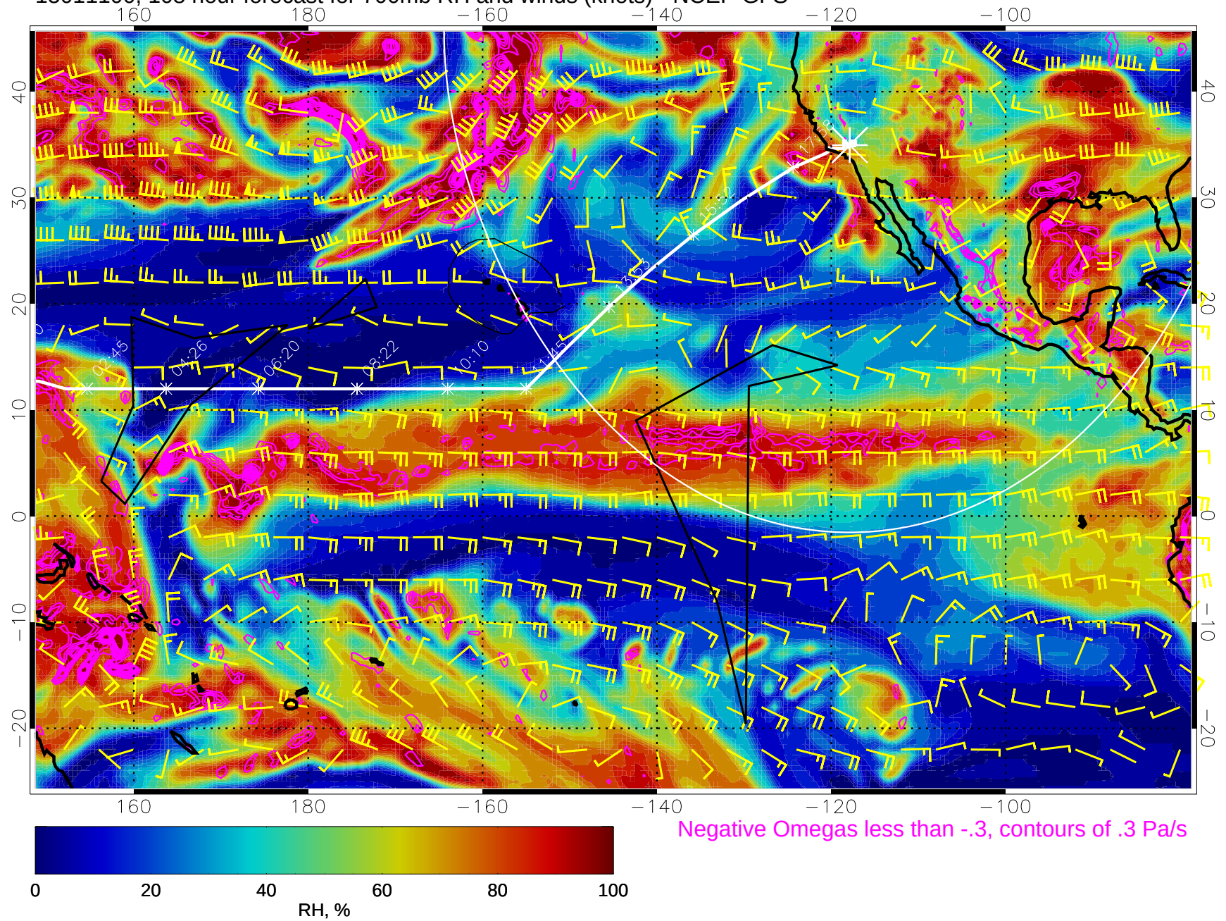
15011100, 108 hour forecast for 700mb RH and winds (knots) - NCEP GFS
