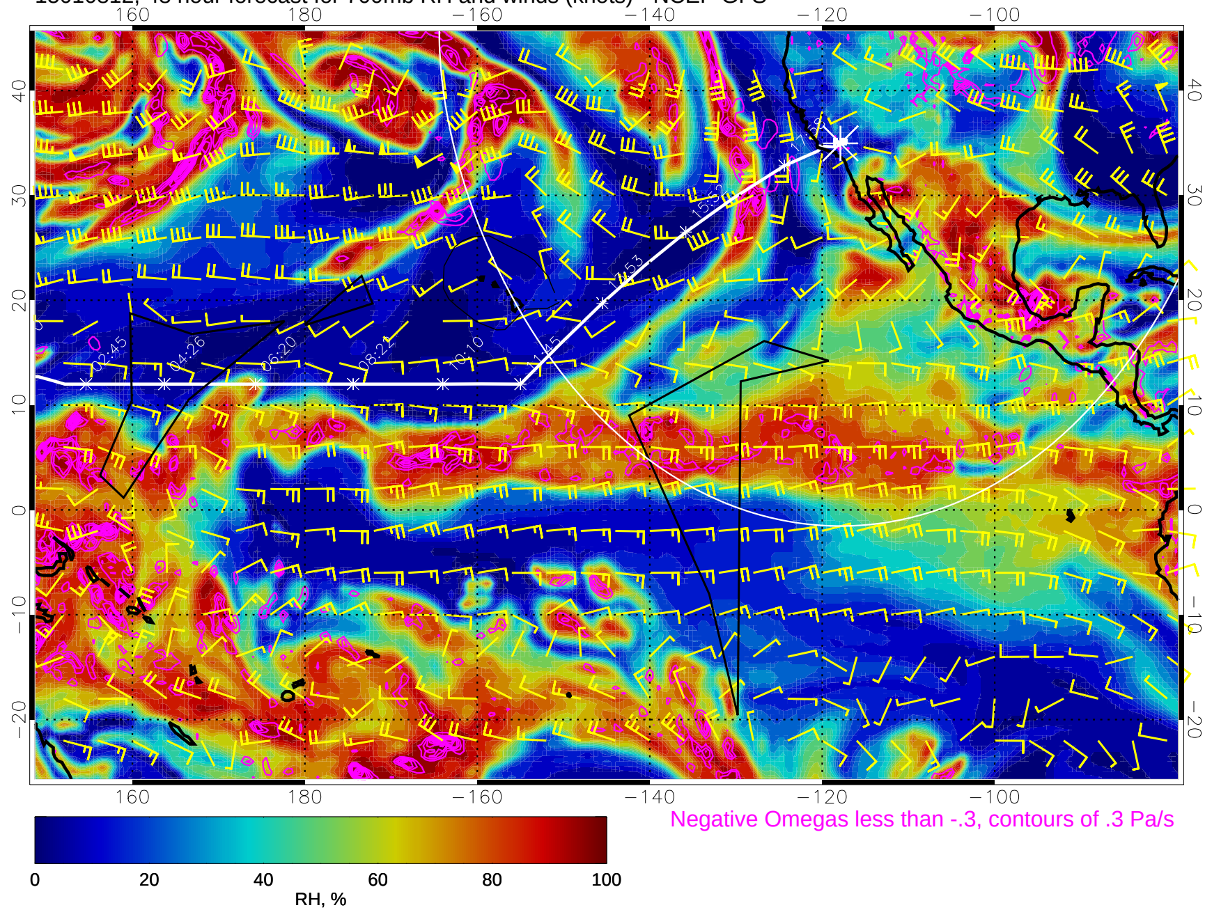
15010812, 48 hour forecast for 700mb RH and winds (knots) - NCEP GFS
