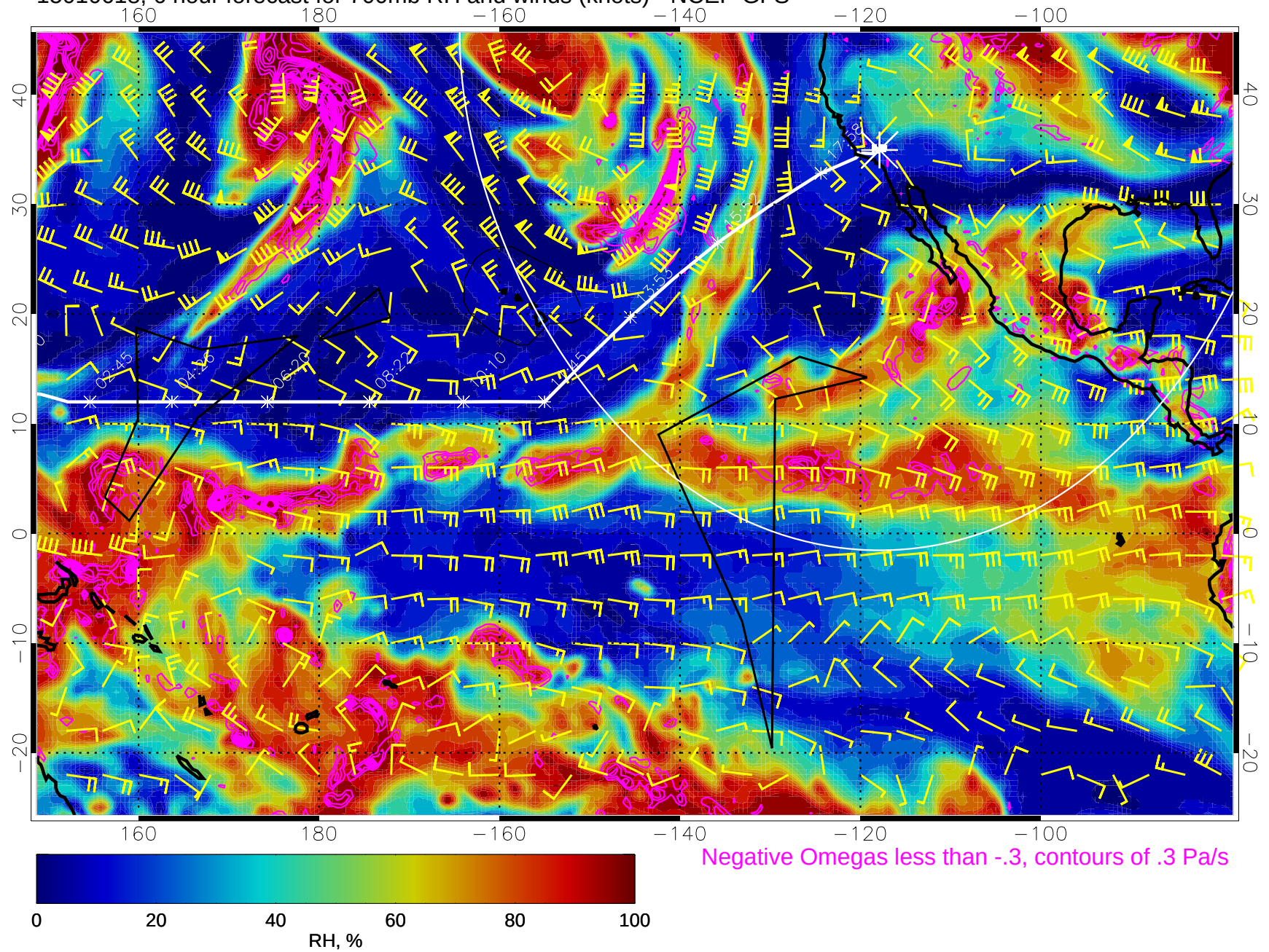
15010618, 6 hour forecast for 700mb RH and winds (knots) - NCEP GFS
