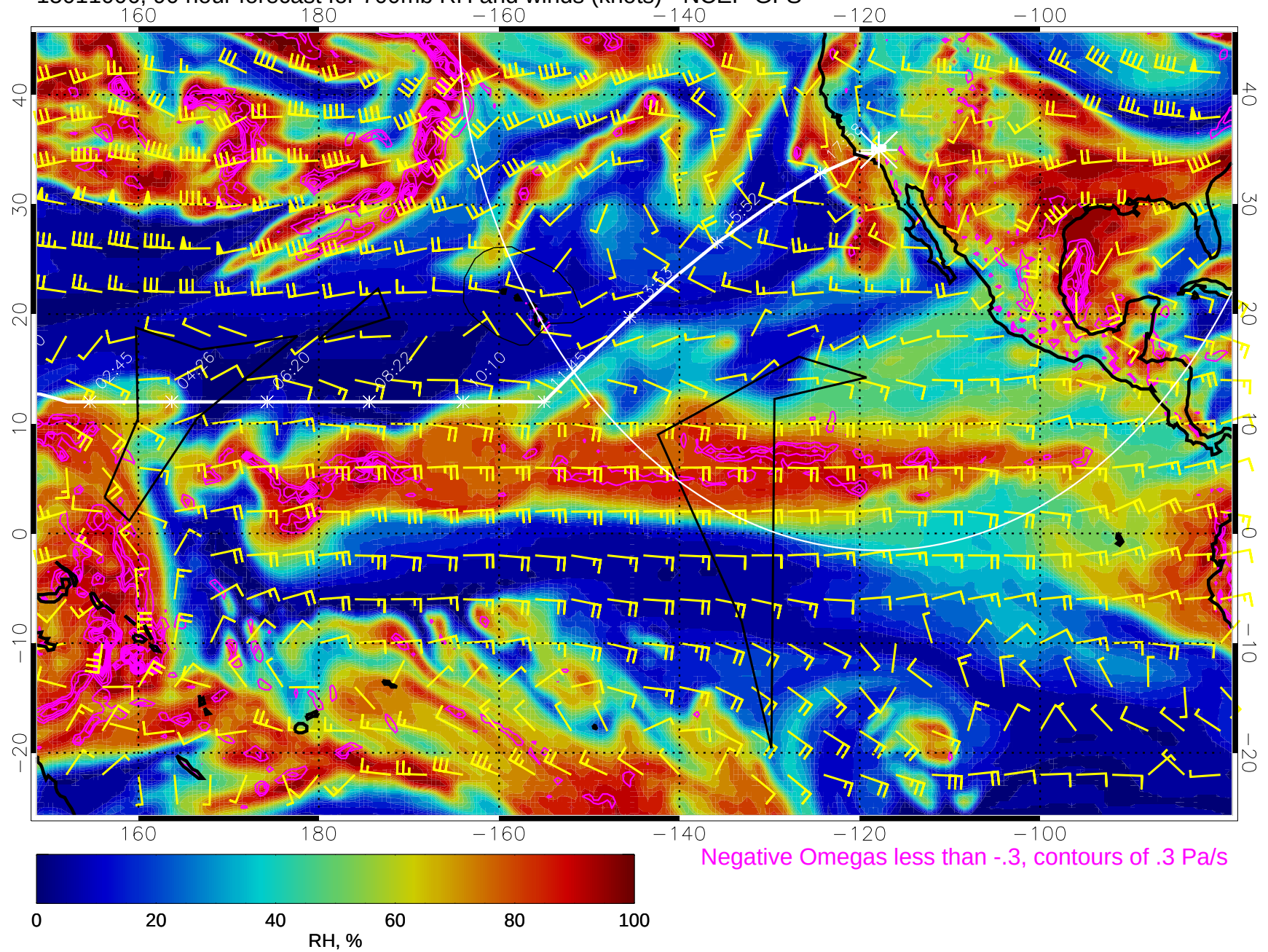
15011006, 90 hour forecast for 700mb RH and winds (knots) - NCEP GFS
