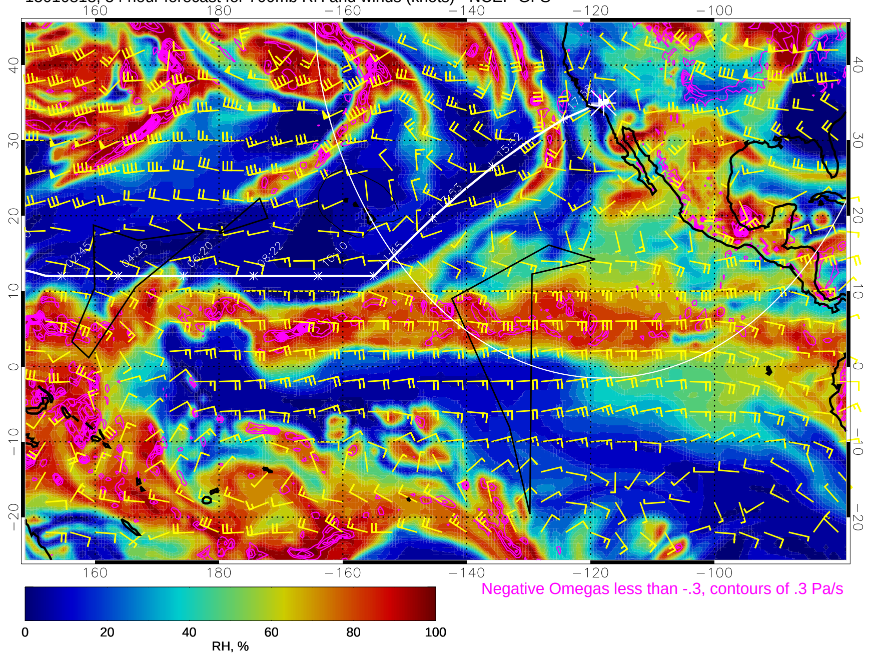
15010818, 54 hour forecast for 700mb RH and winds (knots) - NCEP GFS
