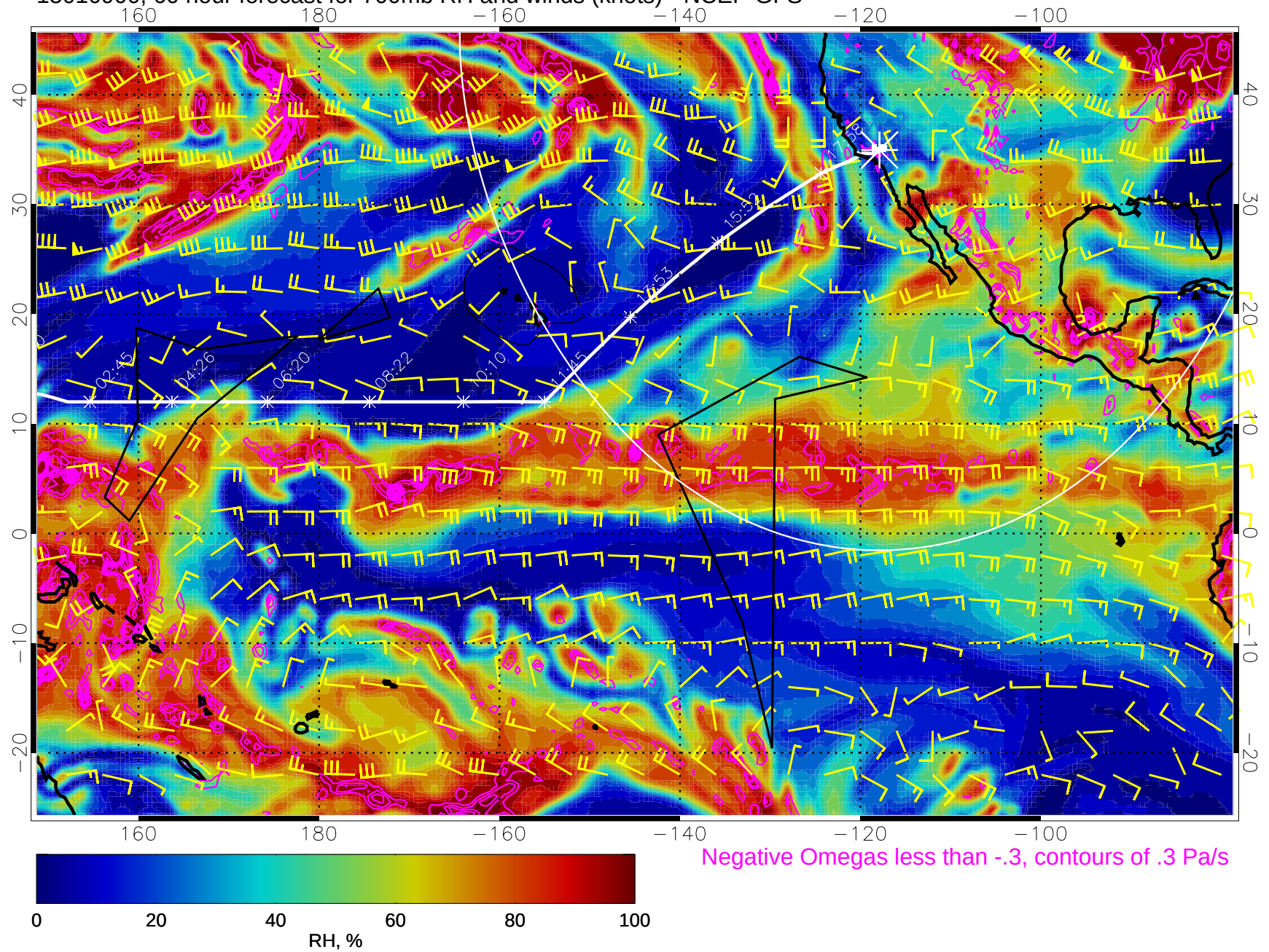
15010900, 60 hour forecast for 700mb RH and winds (knots) - NCEP GFS
