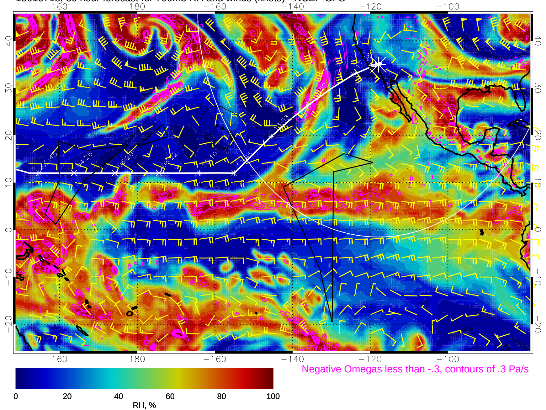
15010718, 30 hour forecast for 700mb RH and winds (knots) - NCEP GFS
