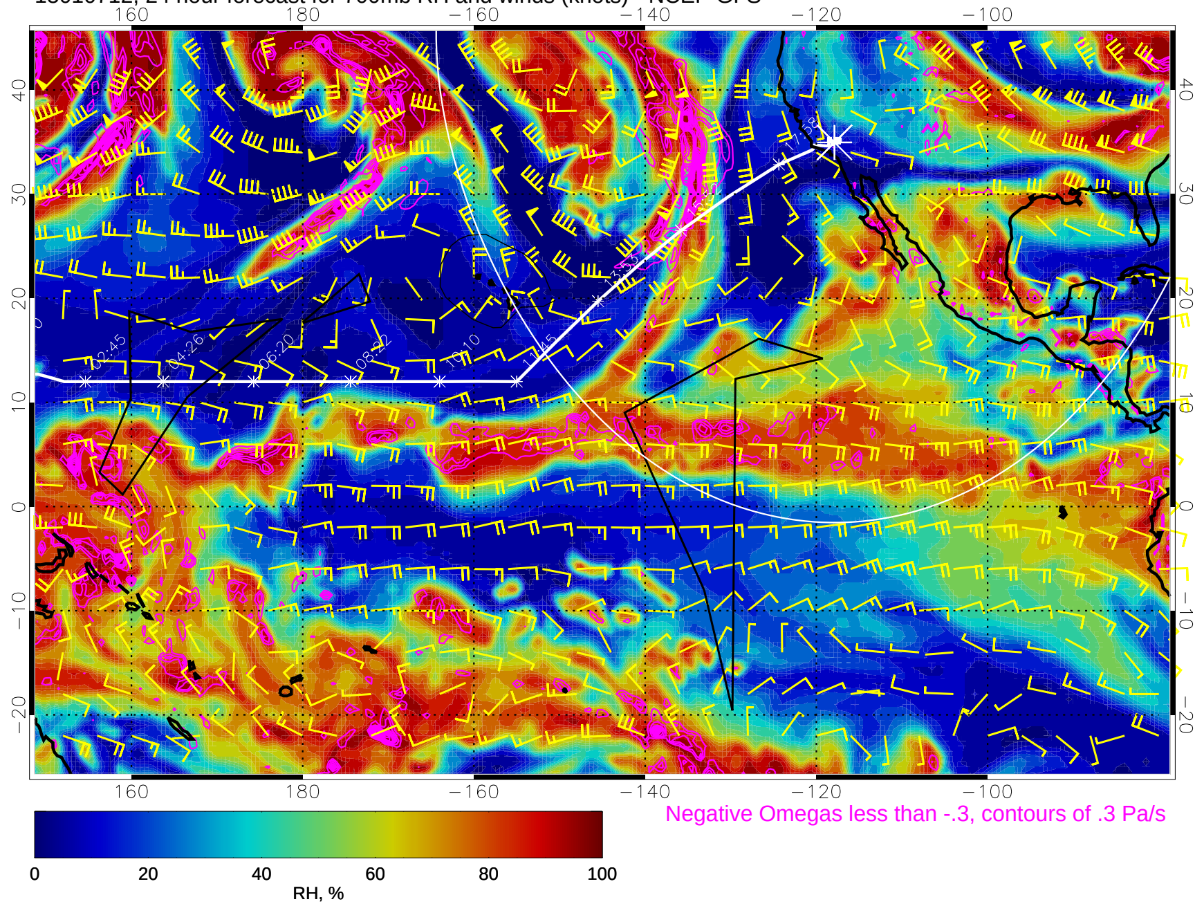
15010712, 24 hour forecast for 700mb RH and winds (knots) - NCEP GFS
