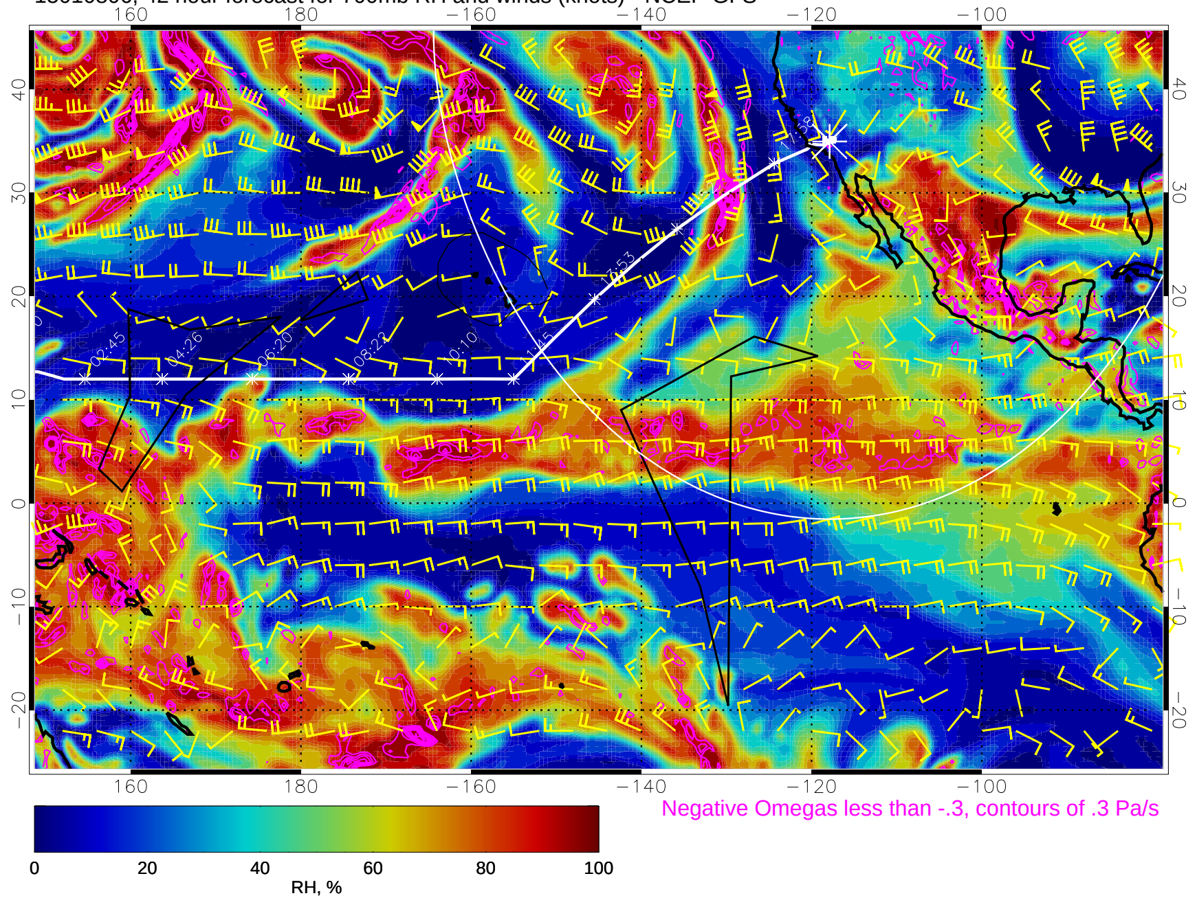
15010806, 42 hour forecast for 700mb RH and winds (knots) - NCEP GFS
