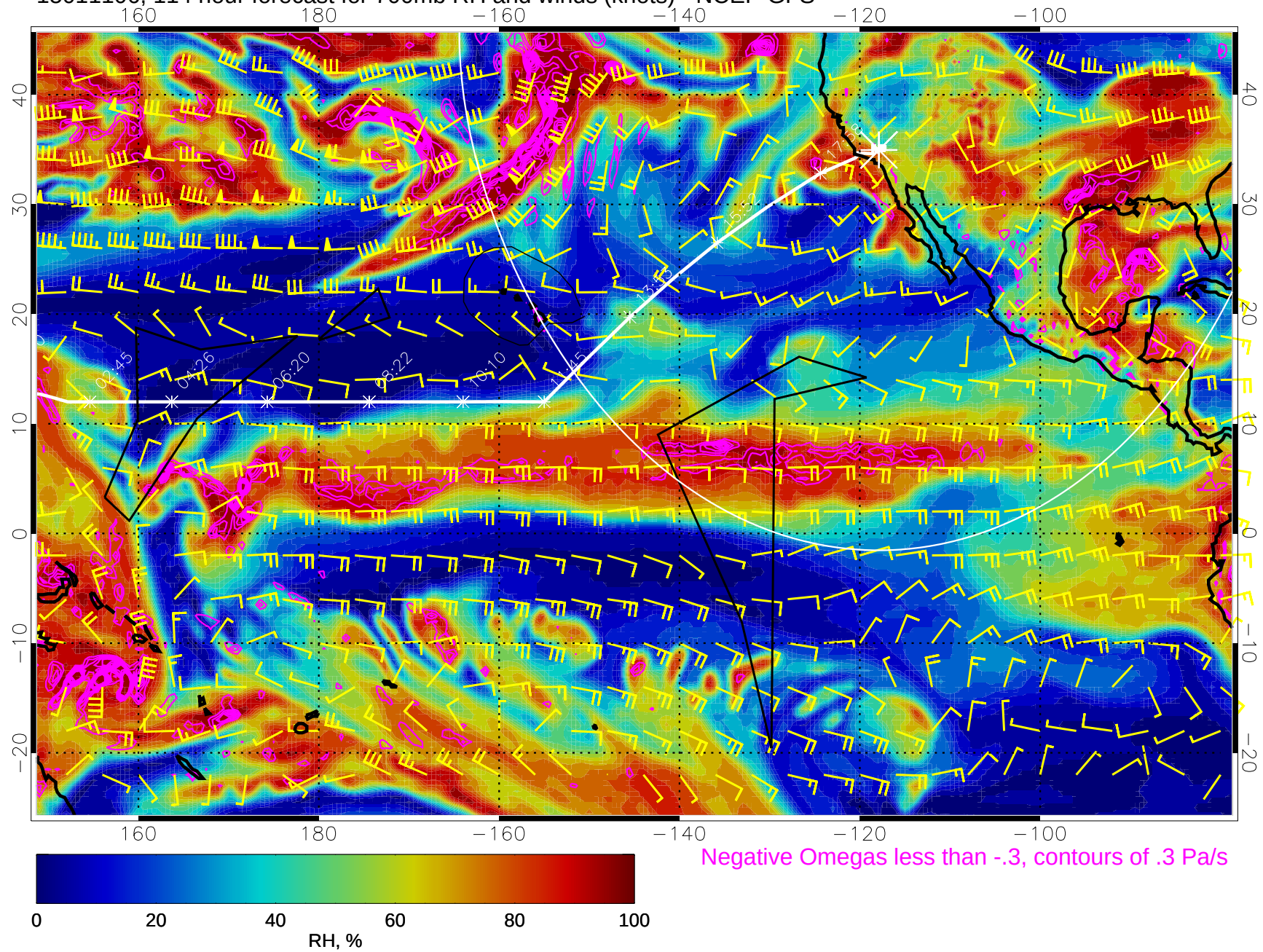
15011106, 114 hour forecast for 700mb RH and winds (knots) - NCEP GFS
