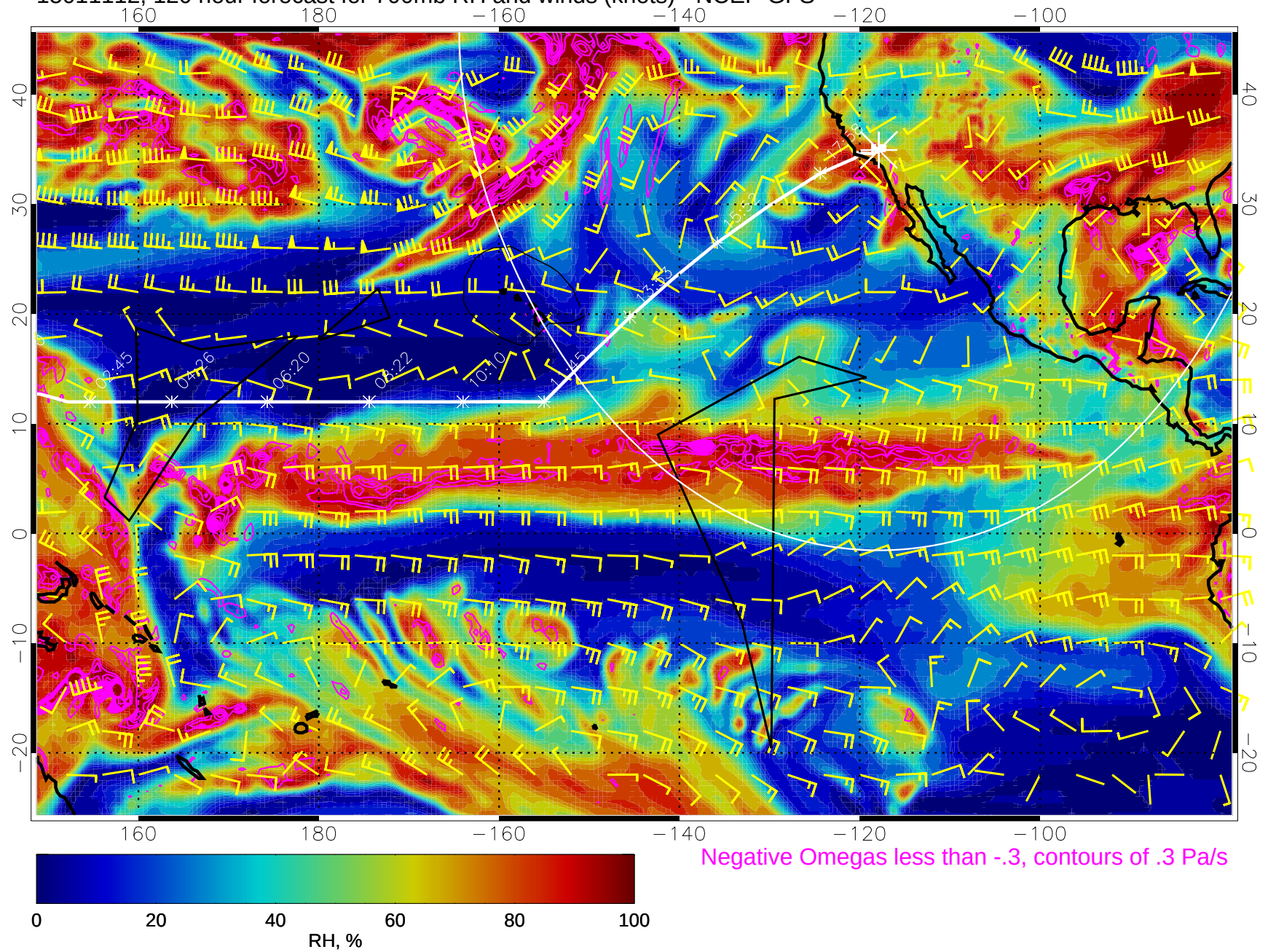
15011112, 120 hour forecast for 700mb RH and winds (knots) - NCEP GFS
