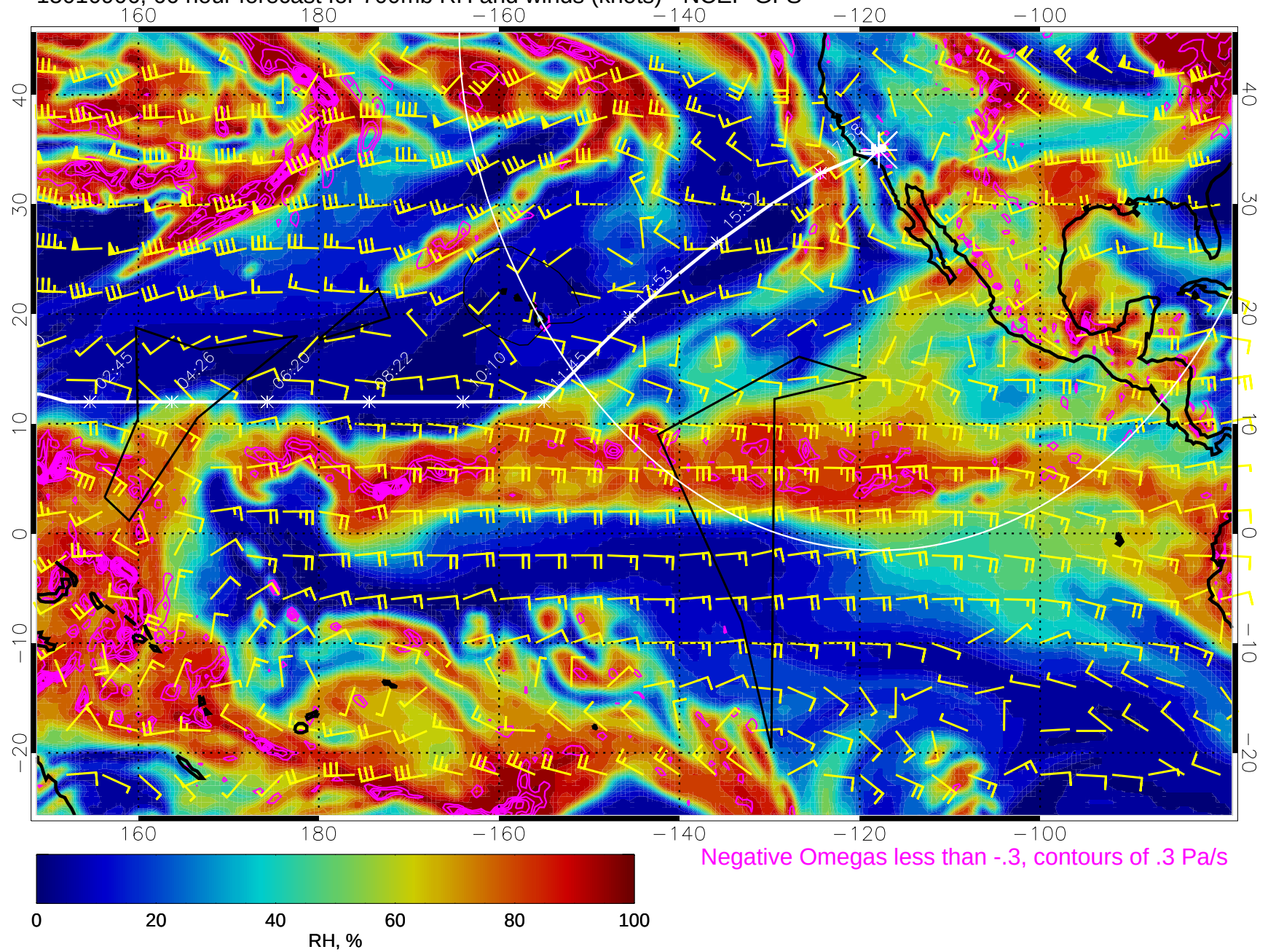
15010906, 66 hour forecast for 700mb RH and winds (knots) - NCEP GFS
