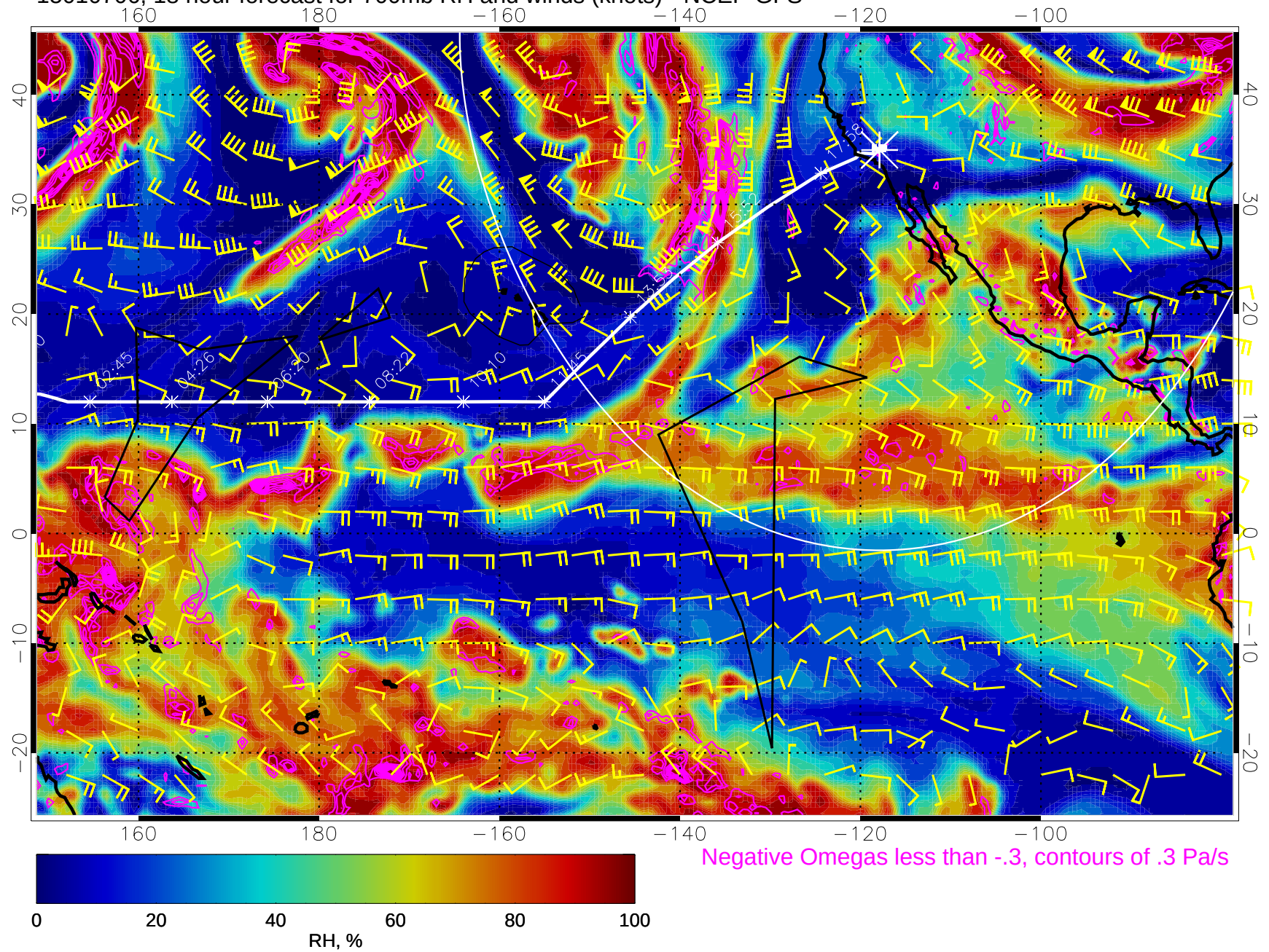
15010706, 18 hour forecast for 700mb RH and winds (knots) - NCEP GFS
