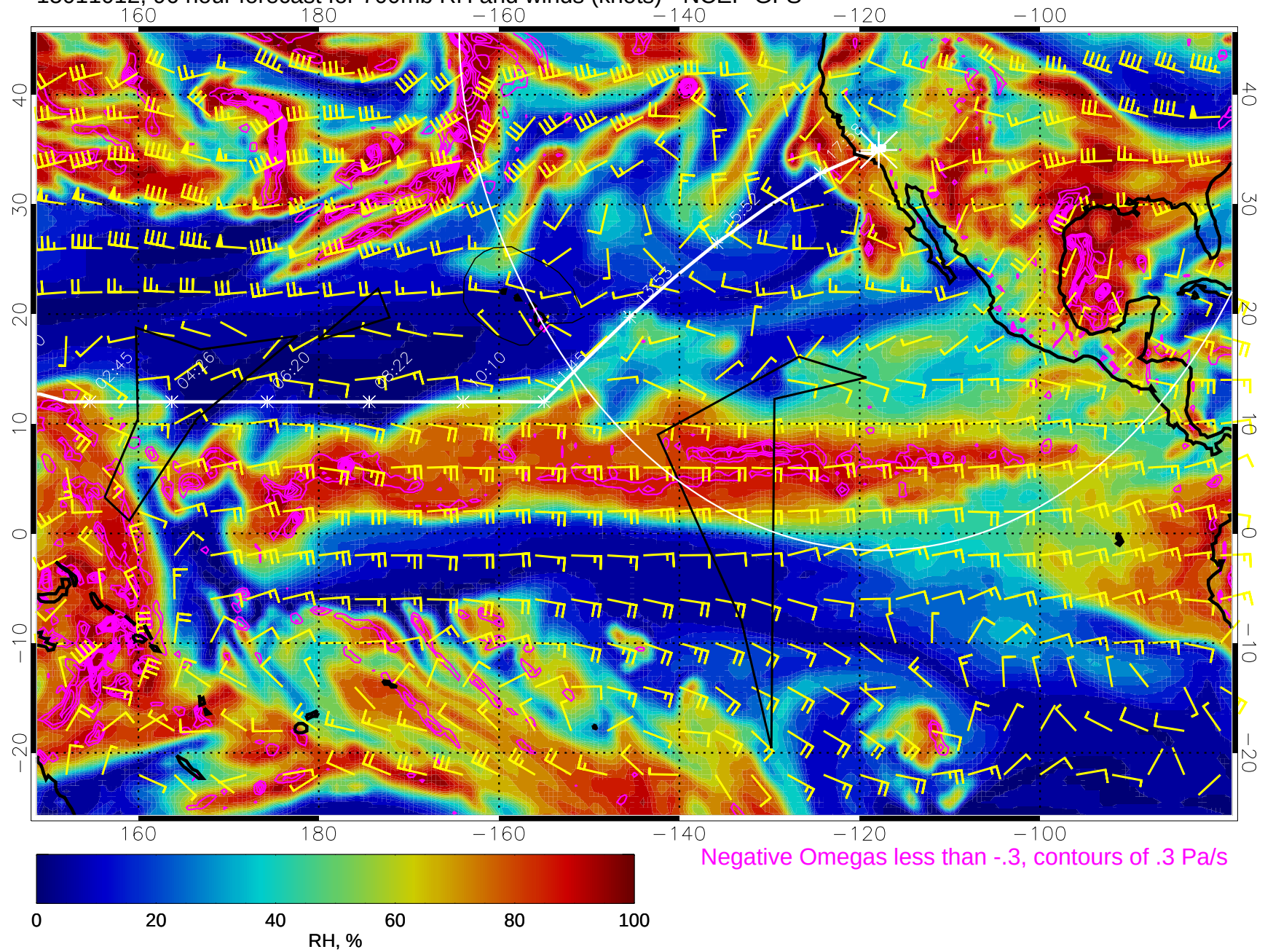
15011012, 96 hour forecast for 700mb RH and winds (knots) - NCEP GFS
