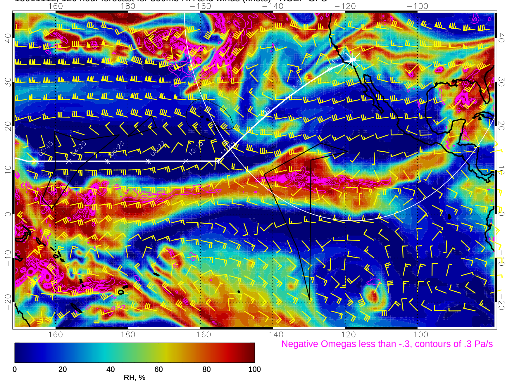
15011112, 120 hour forecast for 500mb RH and winds (knots) - NCEP GFS
