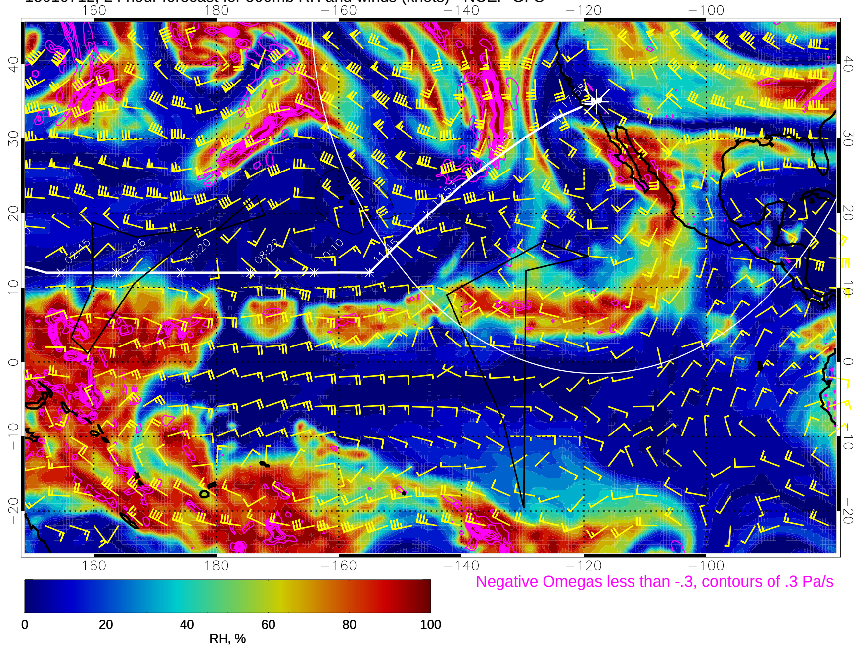
15010712, 24 hour forecast for 500mb RH and winds (knots) - NCEP GFS
