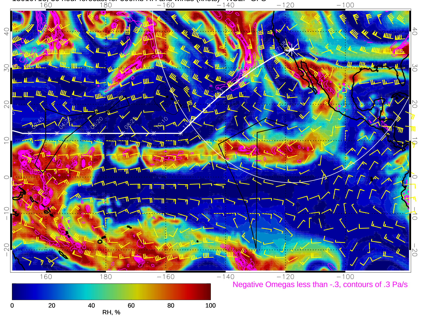
15010718, 30 hour forecast for 500mb RH and winds (knots) - NCEP GFS
