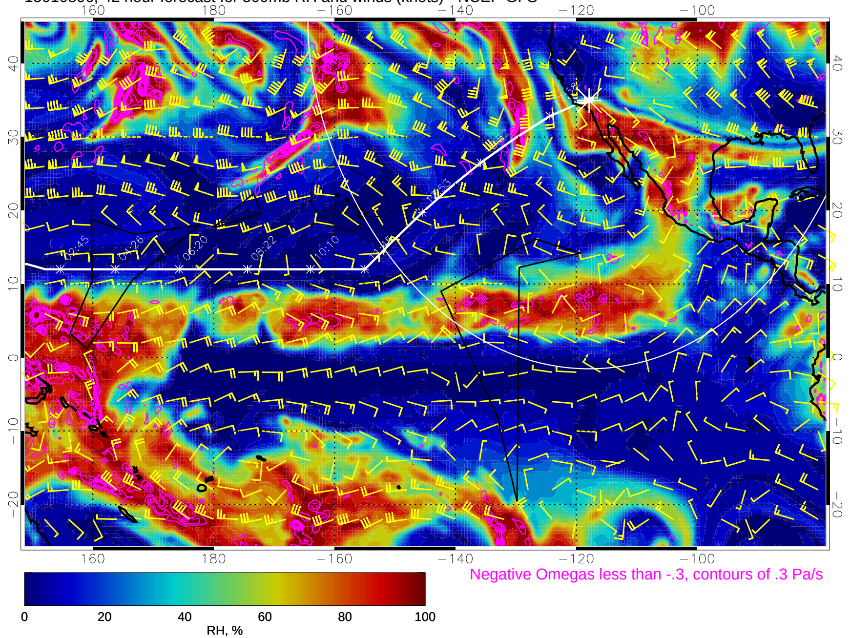
15010806, 42 hour forecast for 500mb RH and winds (knots) - NCEP GFS
