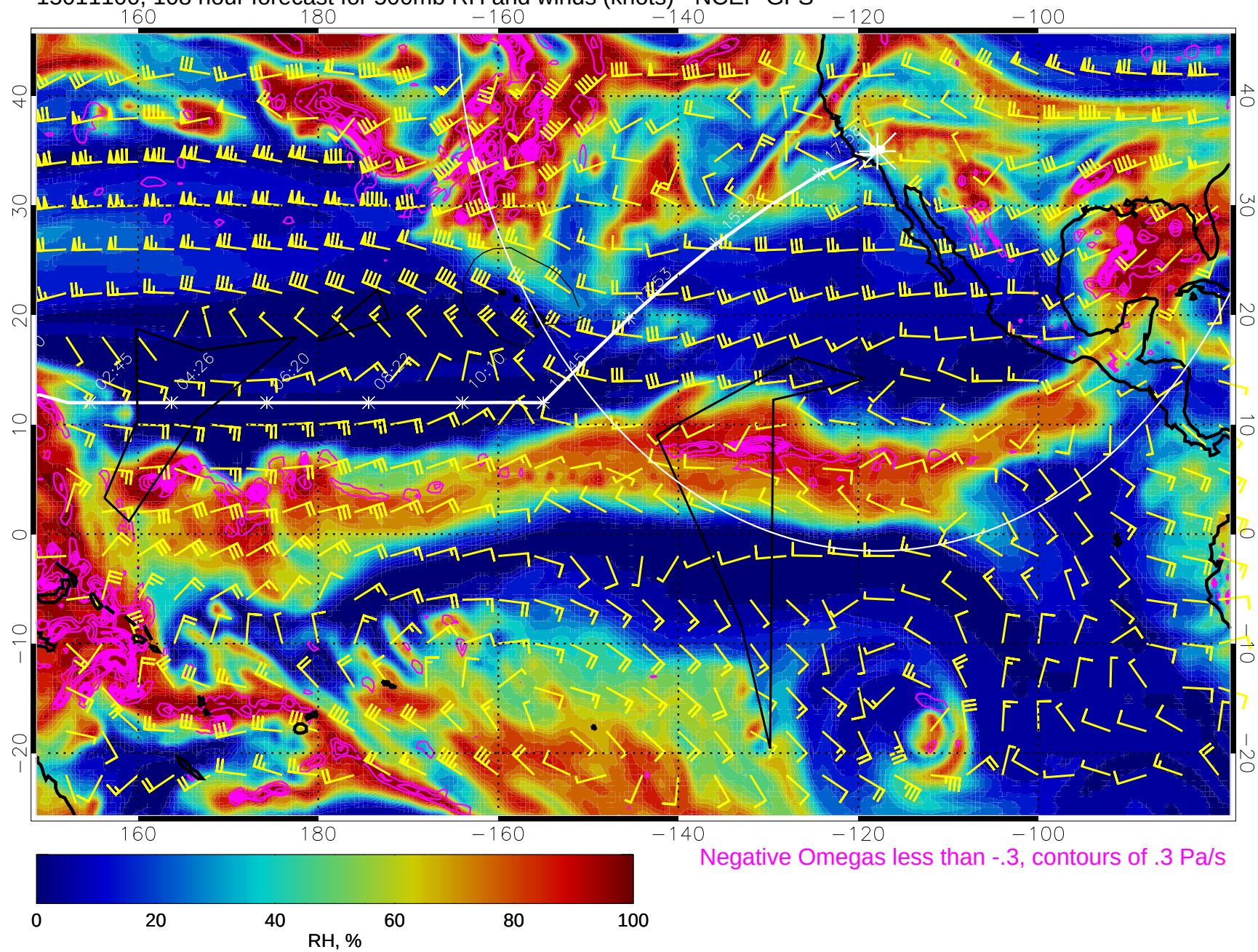
15011100, 108 hour forecast for 500mb RH and winds (knots) - NCEP GFS
