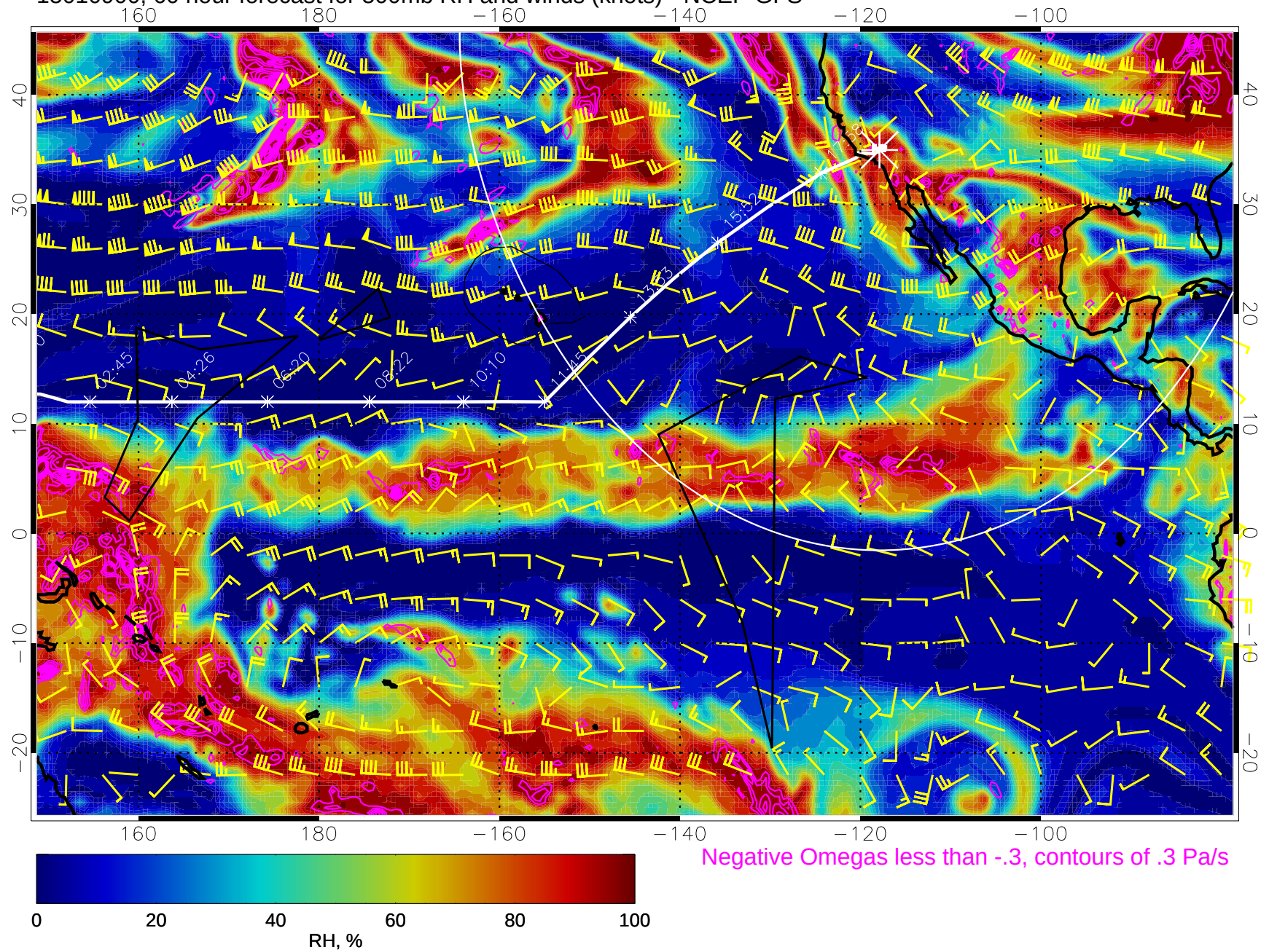
15010900, 60 hour forecast for 500mb RH and winds (knots) - NCEP GFS
