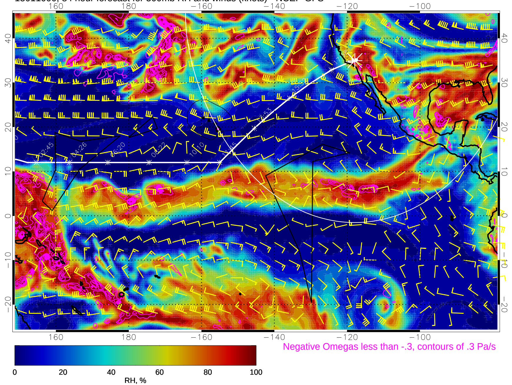
15011000, 84 hour forecast for 500mb RH and winds (knots) - NCEP GFS
