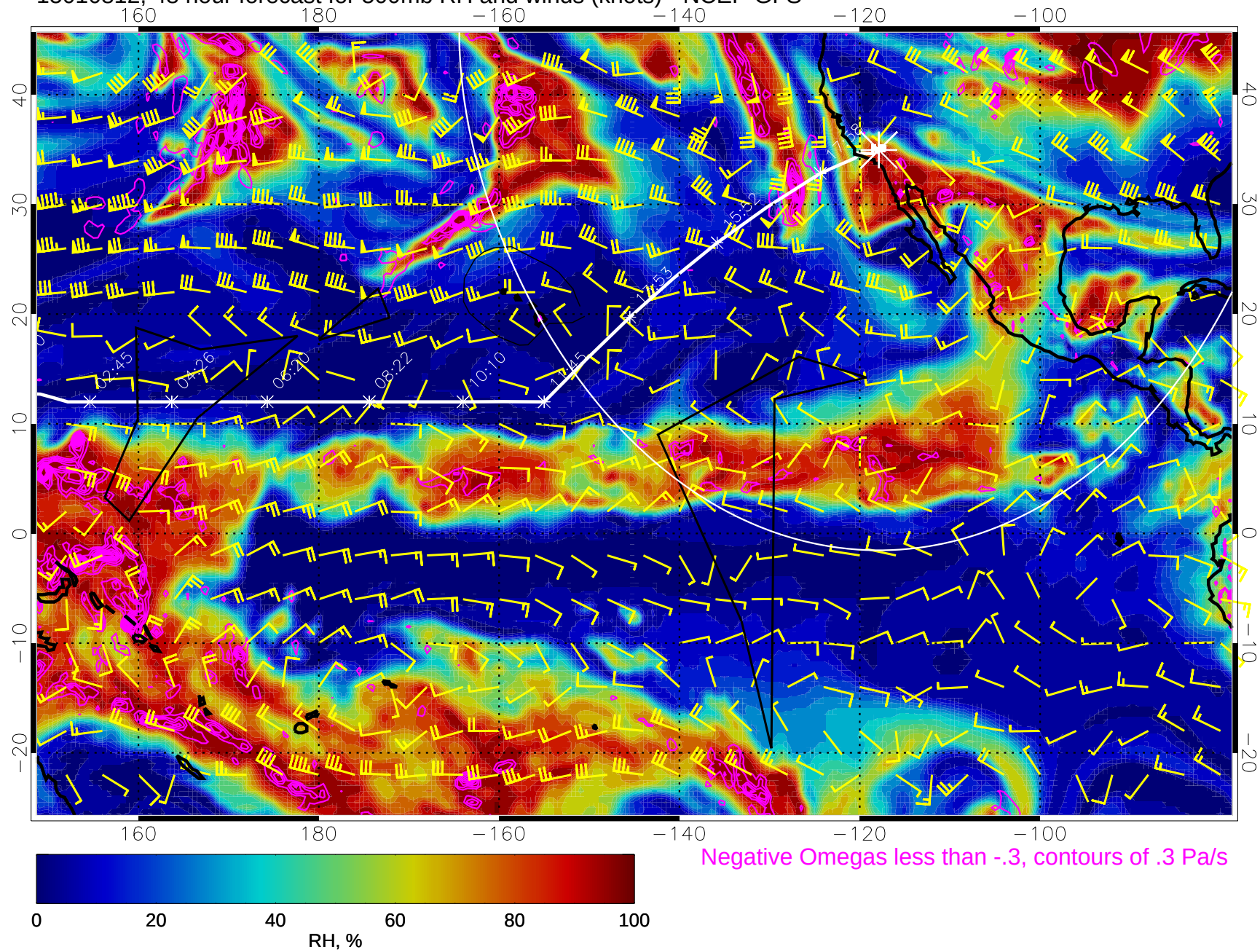
15010812, 48 hour forecast for 500mb RH and winds (knots) - NCEP GFS
