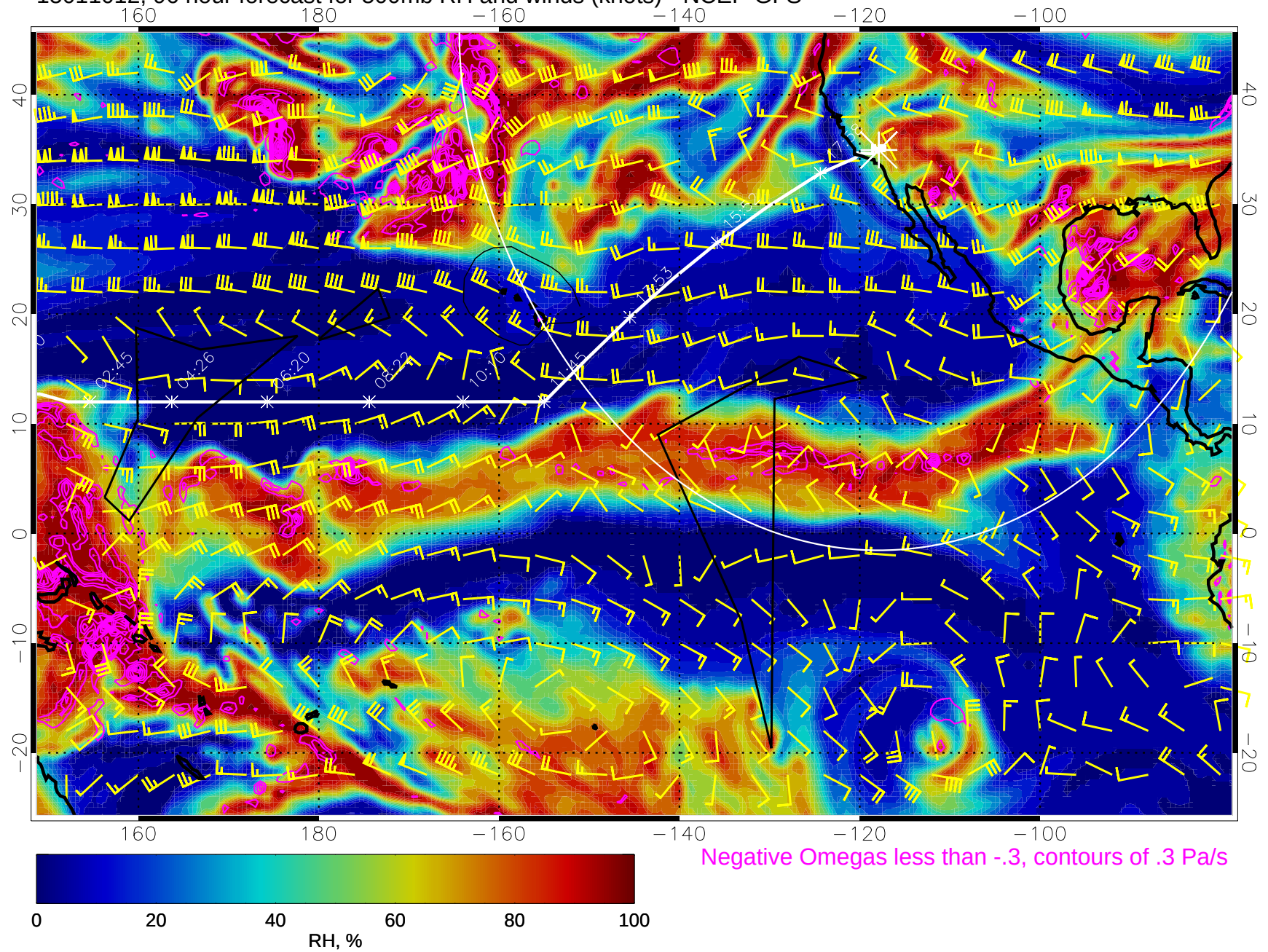
15011012, 96 hour forecast for 500mb RH and winds (knots) - NCEP GFS
