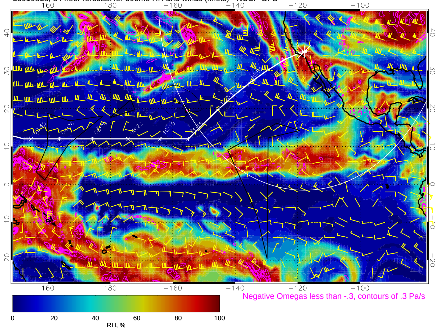
15010818, 54 hour forecast for 500mb RH and winds (knots) - NCEP GFS
