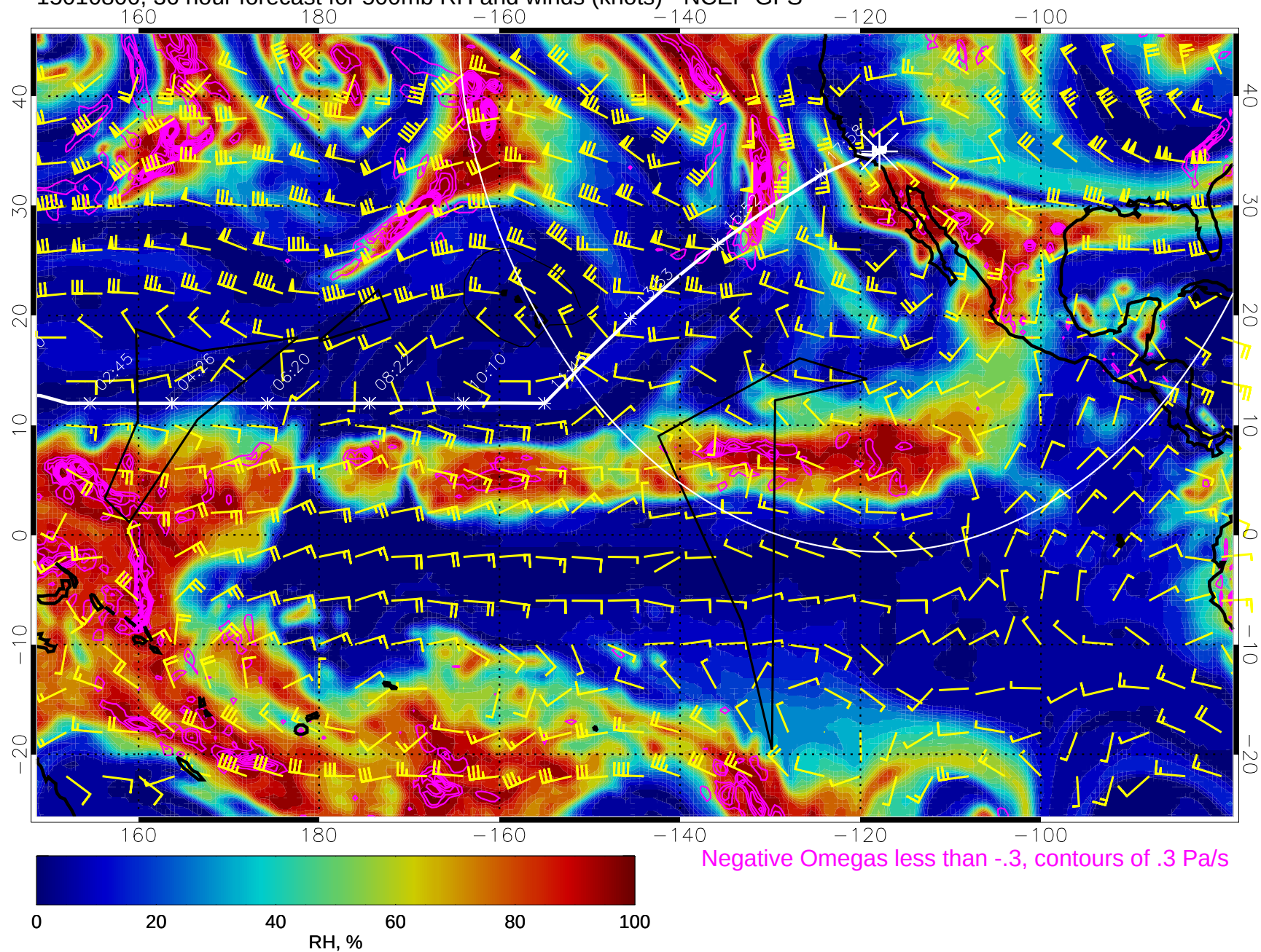
15010800, 36 hour forecast for 500mb RH and winds (knots) - NCEP GFS
