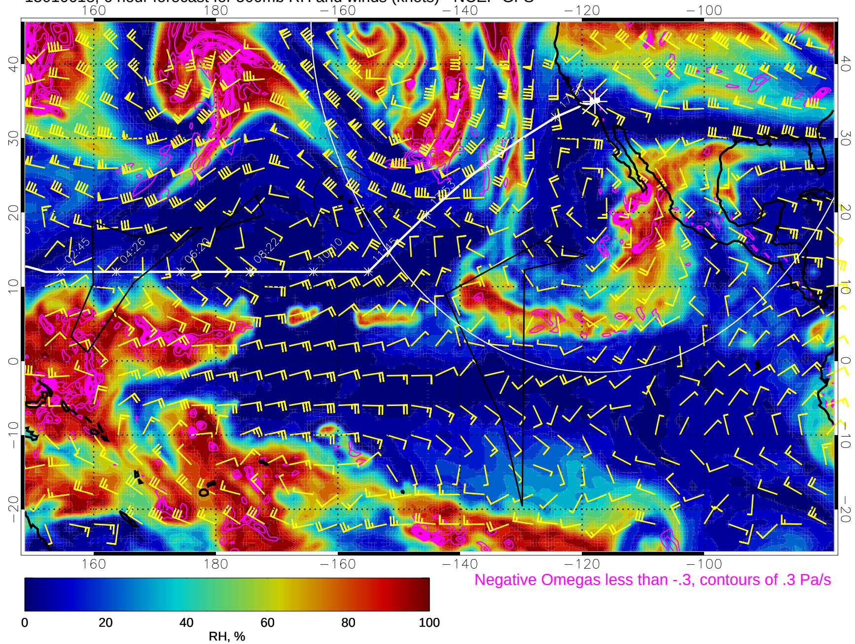
15010618, 6 hour forecast for 500mb RH and winds (knots) - NCEP GFS
