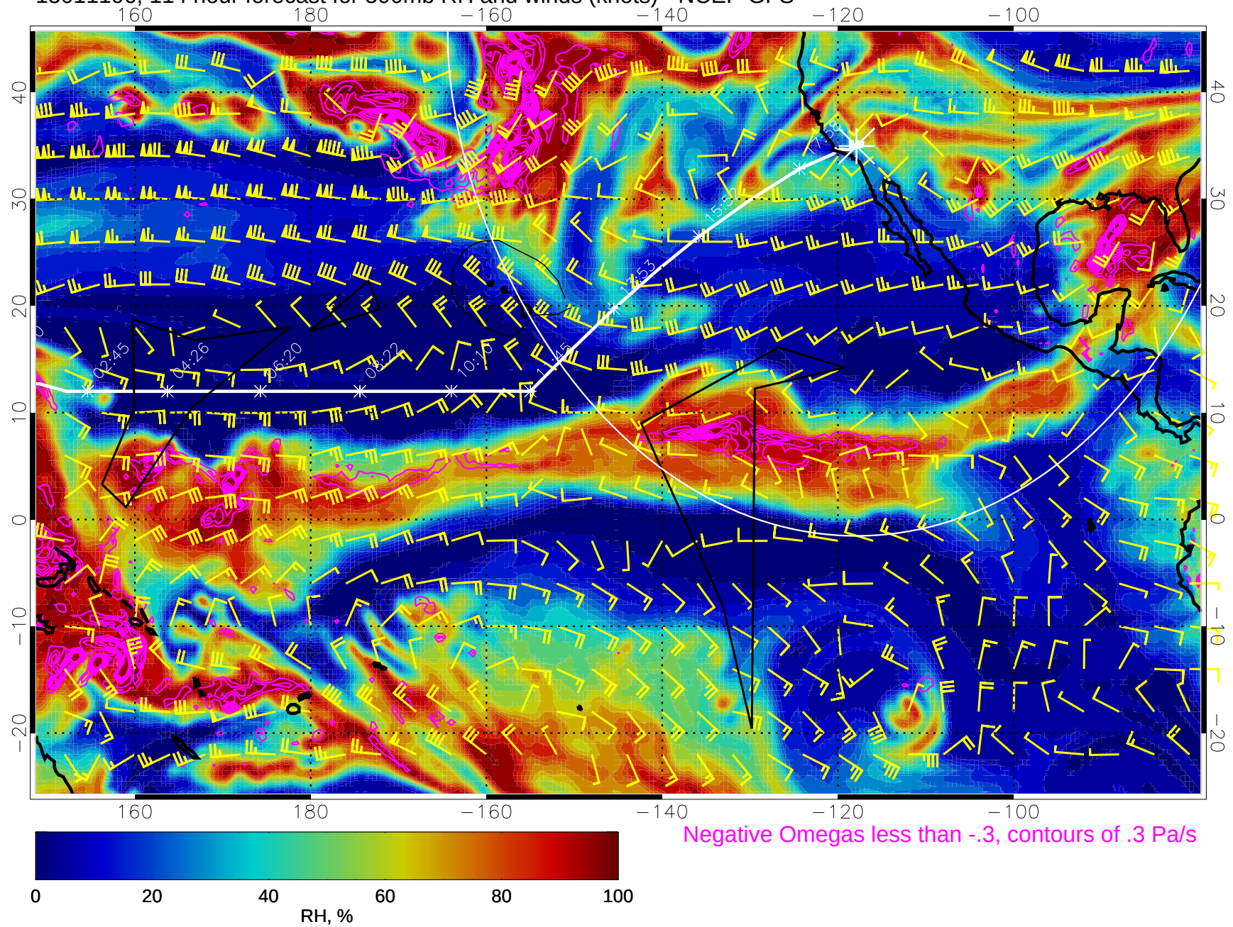
15011106, 114 hour forecast for 500mb RH and winds (knots) - NCEP GFS
