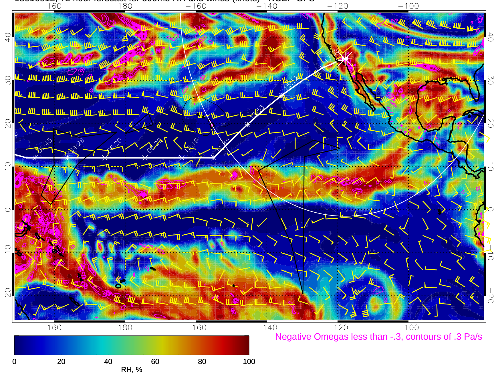
15010912, 72 hour forecast for 500mb RH and winds (knots) - NCEP GFS
