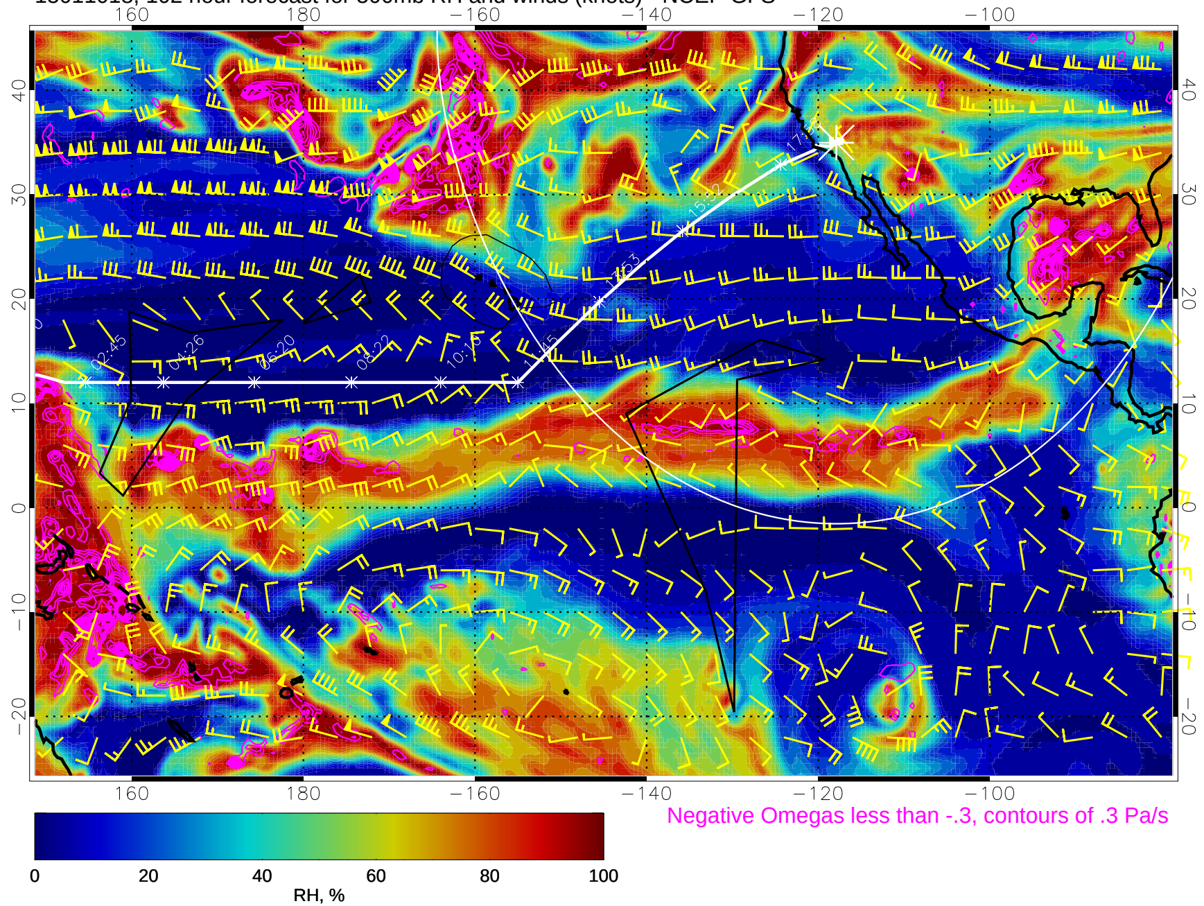
15011018, 102 hour forecast for 500mb RH and winds (knots) - NCEP GFS
