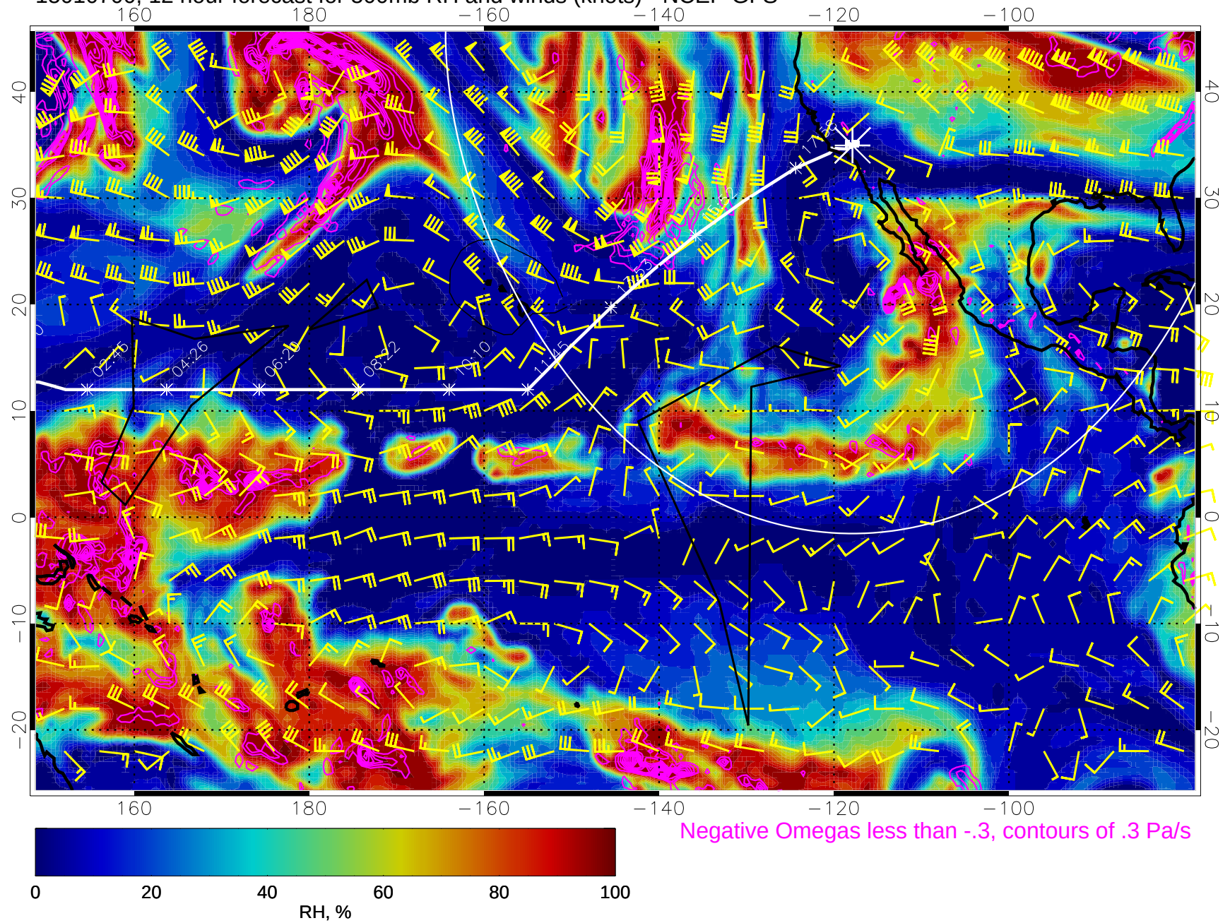
15010700, 12 hour forecast for 500mb RH and winds (knots) - NCEP GFS
