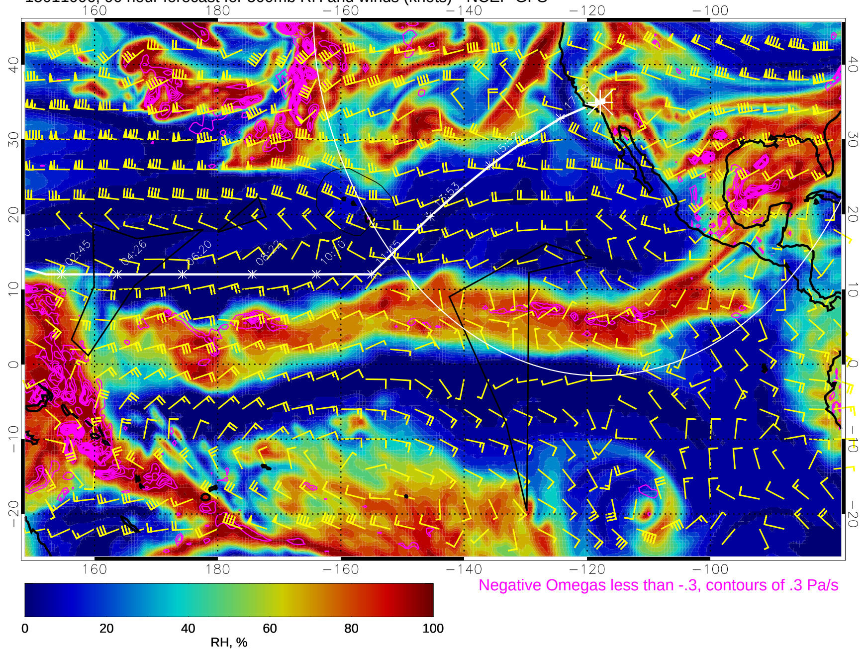
15011006, 90 hour forecast for 500mb RH and winds (knots) - NCEP GFS
