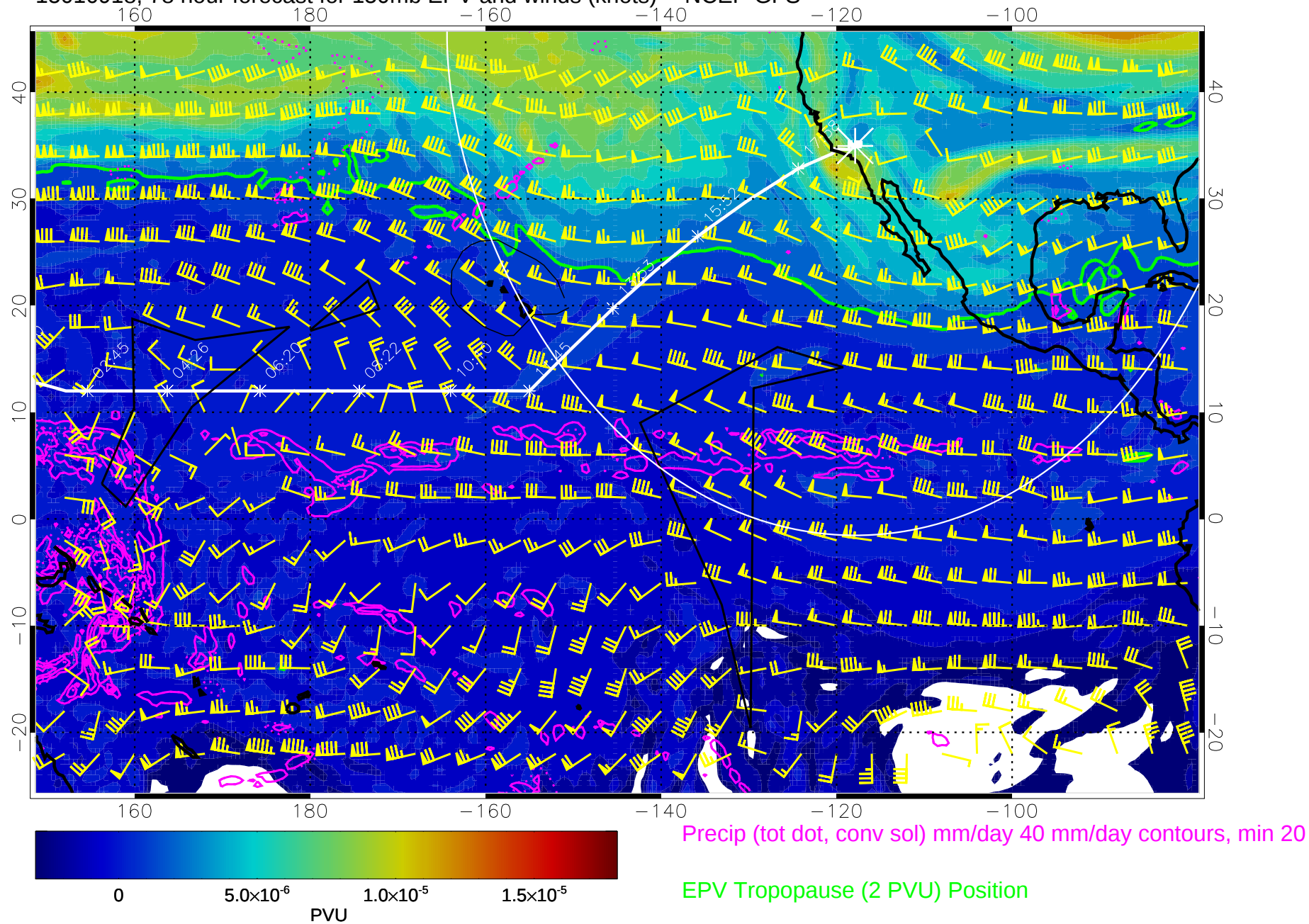
15010918, 78 hour forecast for 150mb EPV and winds (knots) -- NCEP GFS
