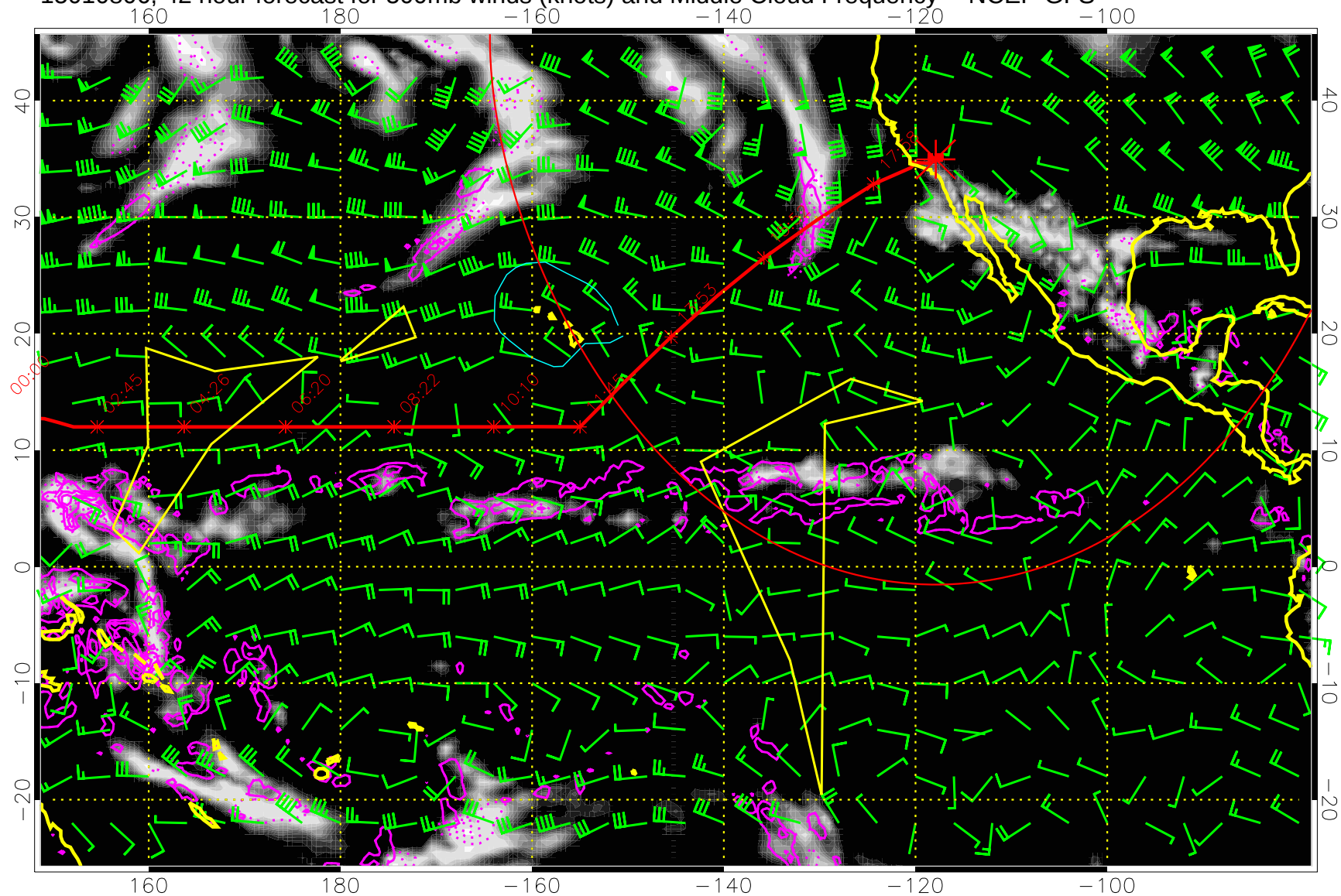
15010806, 42 hour forecast for 500mb winds (knots) and Middle Cloud Frequency -- NCEP GFS
