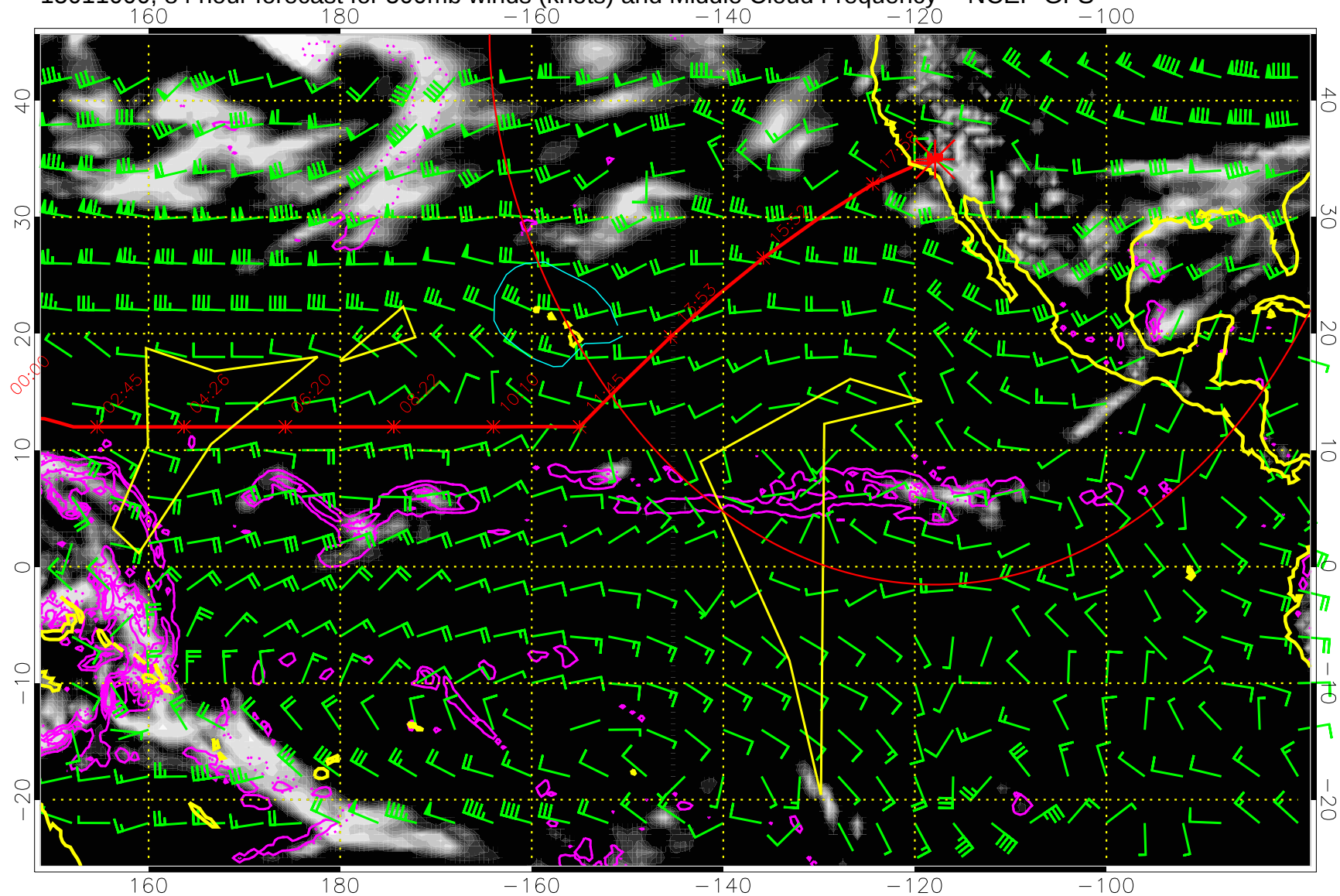
15011000, 84 hour forecast for 500mb winds (knots) and Middle Cloud Frequency -- NCEP GFS
