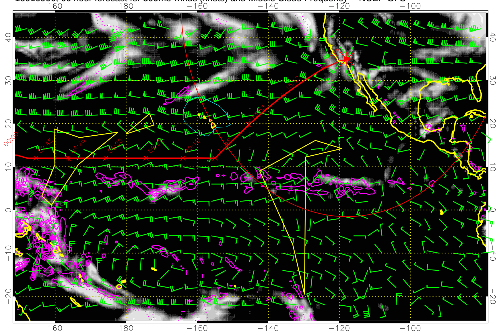
15010906, 66 hour forecast for 500mb winds (knots) and Middle Cloud Frequency -- NCEP GFS
