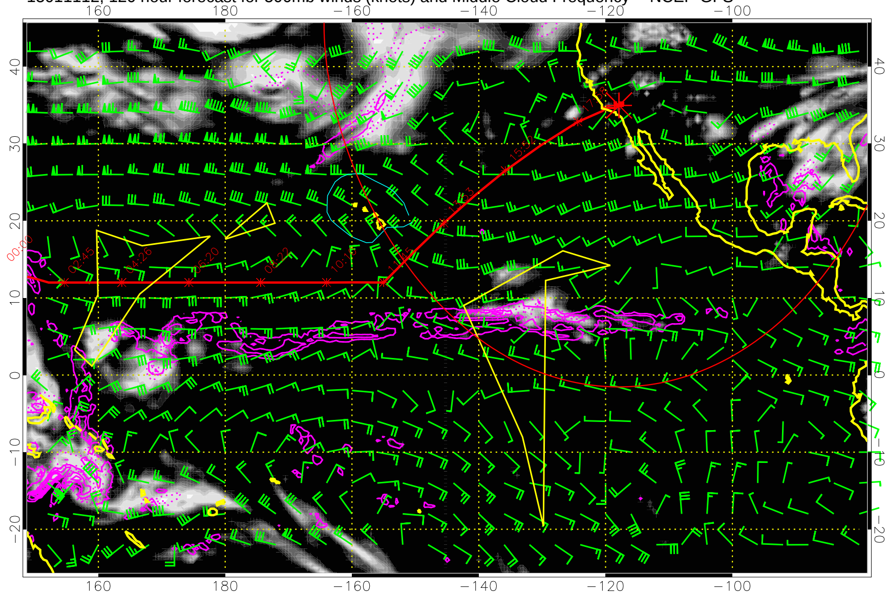
15011112, 120 hour forecast for 500mb winds (knots) and Middle Cloud Frequency -- NCEP GFS
