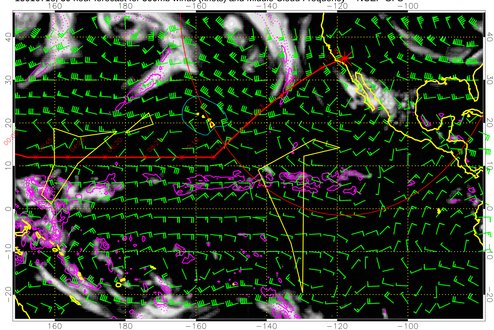
15010718, 30 hour forecast for 500mb winds (knots) and Middle Cloud Frequency -- NCEP GFS
