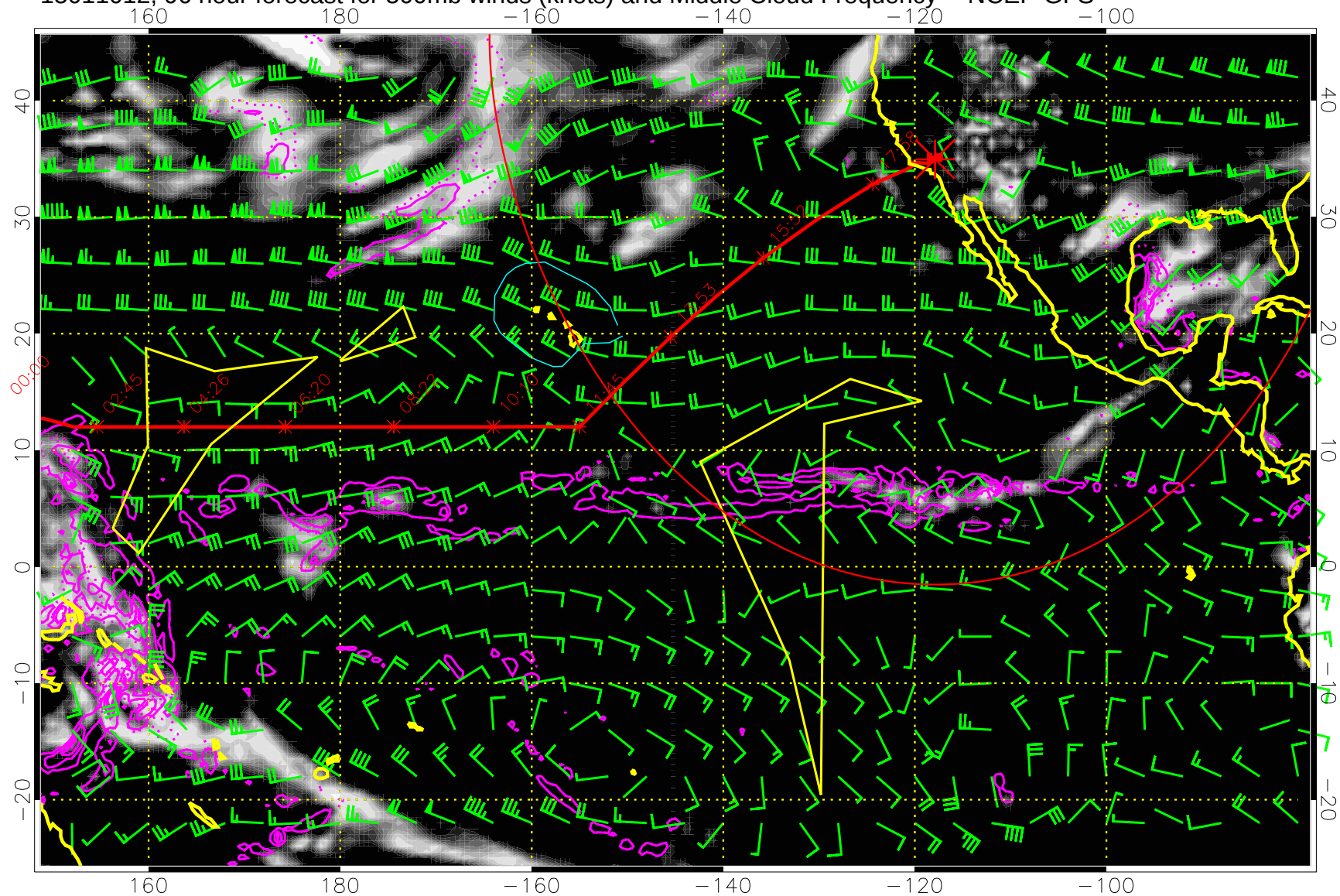
15011012, 96 hour forecast for 500mb winds (knots) and Middle Cloud Frequency -- NCEP GFS
