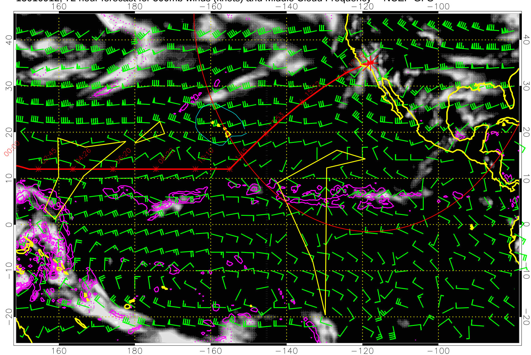
15010912, 72 hour forecast for 500mb winds (knots) and Middle Cloud Frequency -- NCEP GFS
