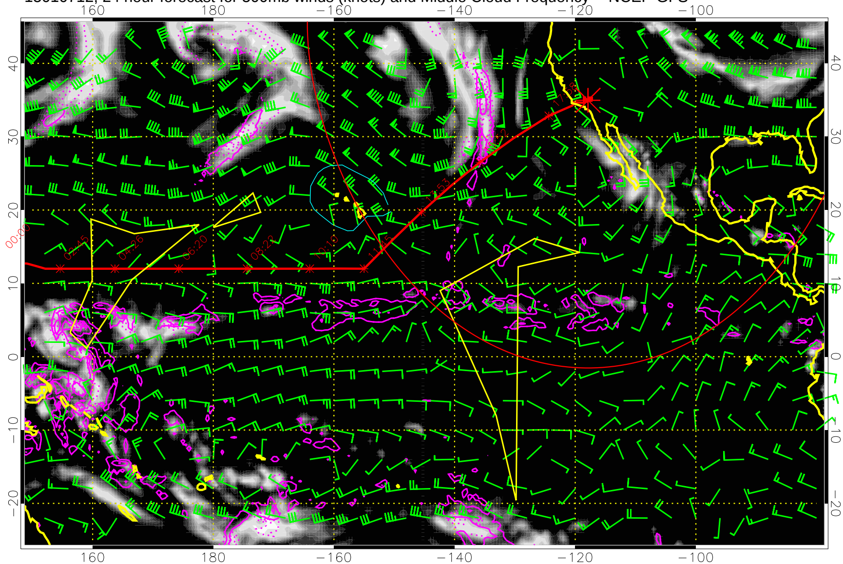
15010712, 24 hour forecast for 500mb winds (knots) and Middle Cloud Frequency -- NCEP GFS
