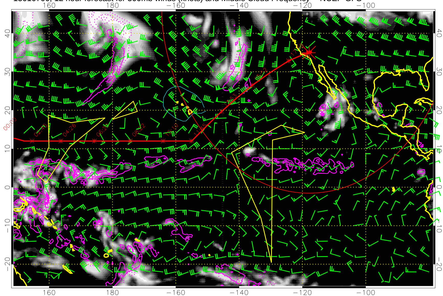
15010700, 12 hour forecast for 500mb winds (knots) and Middle Cloud Frequency -- NCEP GFS
