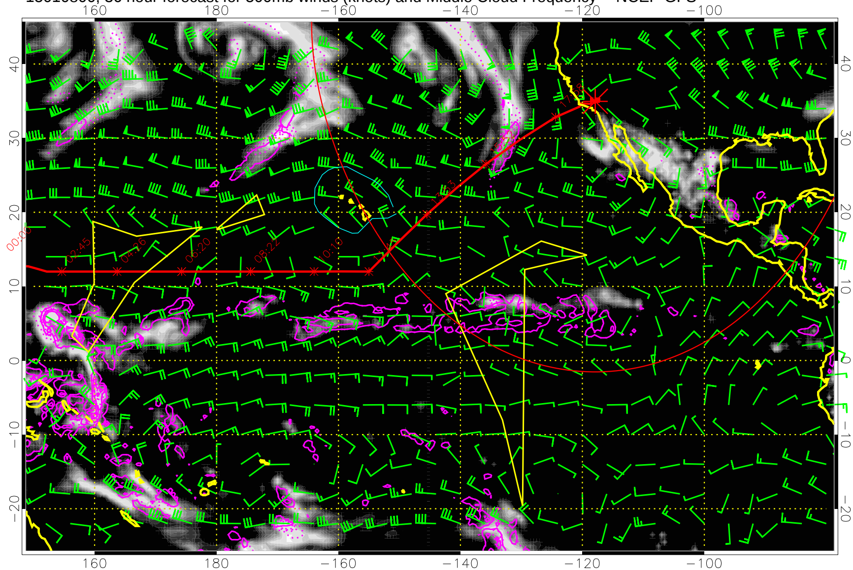
15010800, 36 hour forecast for 500mb winds (knots) and Middle Cloud Frequency -- NCEP GFS
