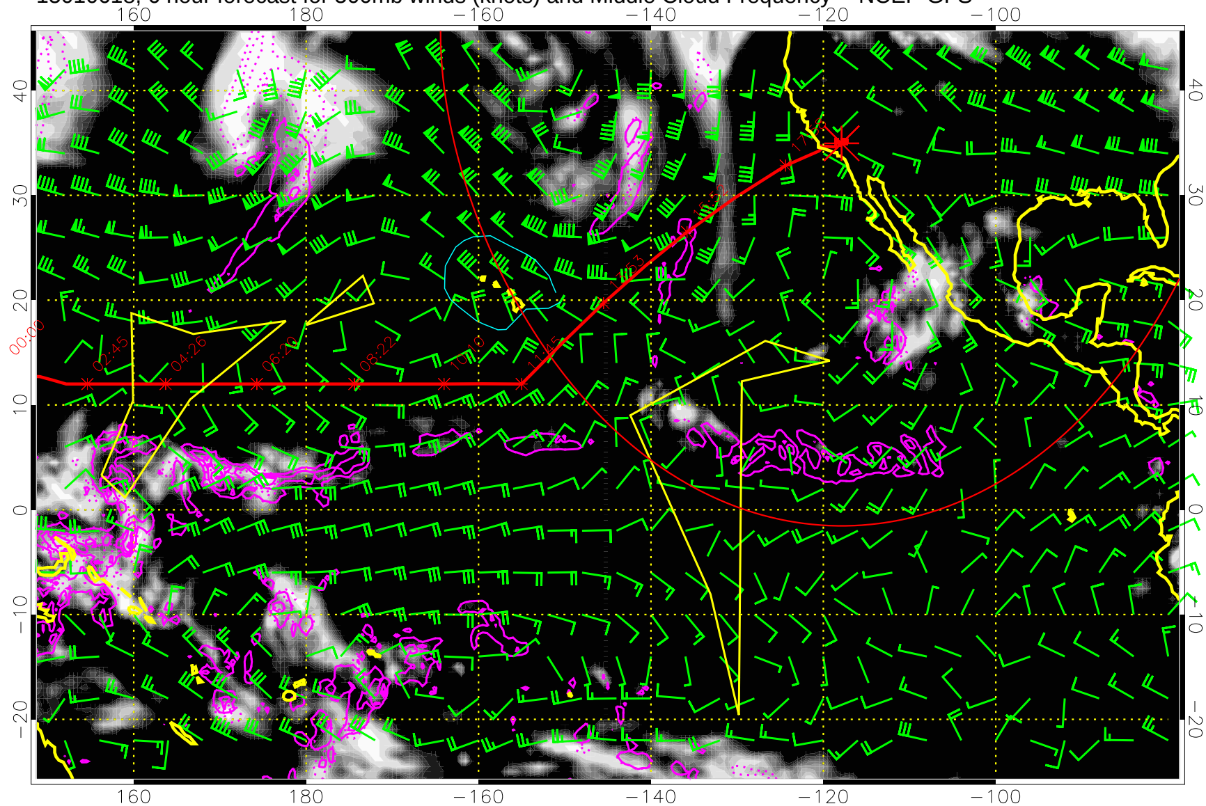
15010618, 6 hour forecast for 500mb winds (knots) and Middle Cloud Frequency -- NCEP GFS
