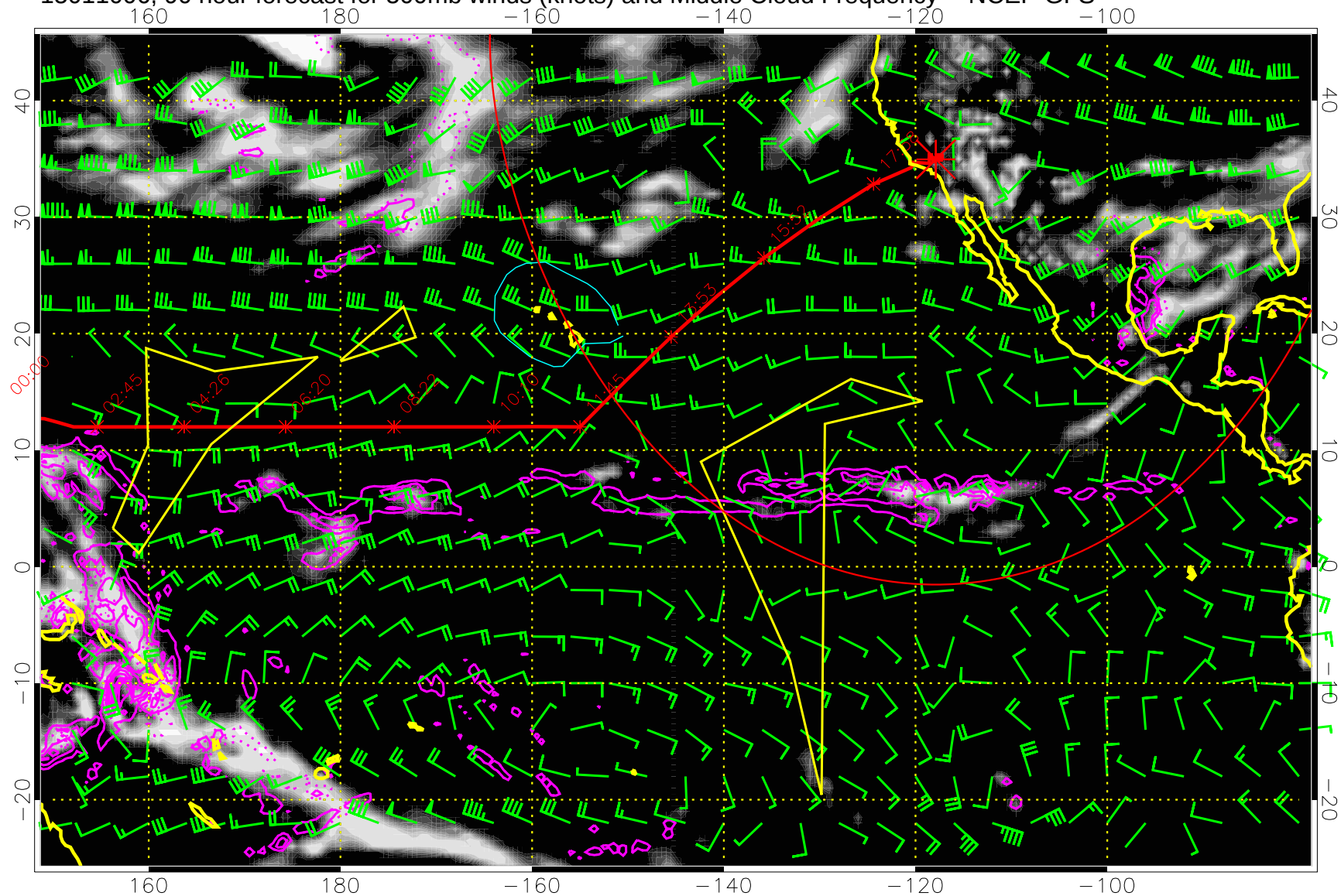
15011006, 90 hour forecast for 500mb winds (knots) and Middle Cloud Frequency -- NCEP GFS
