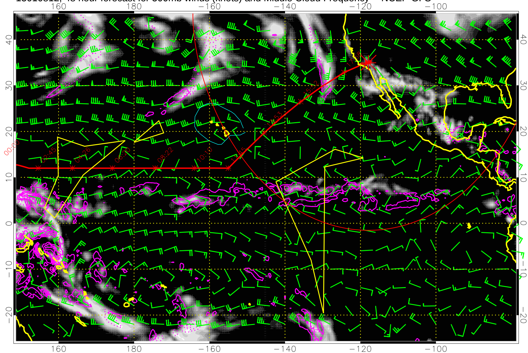
15010812, 48 hour forecast for 500mb winds (knots) and Middle Cloud Frequency -- NCEP GFS
