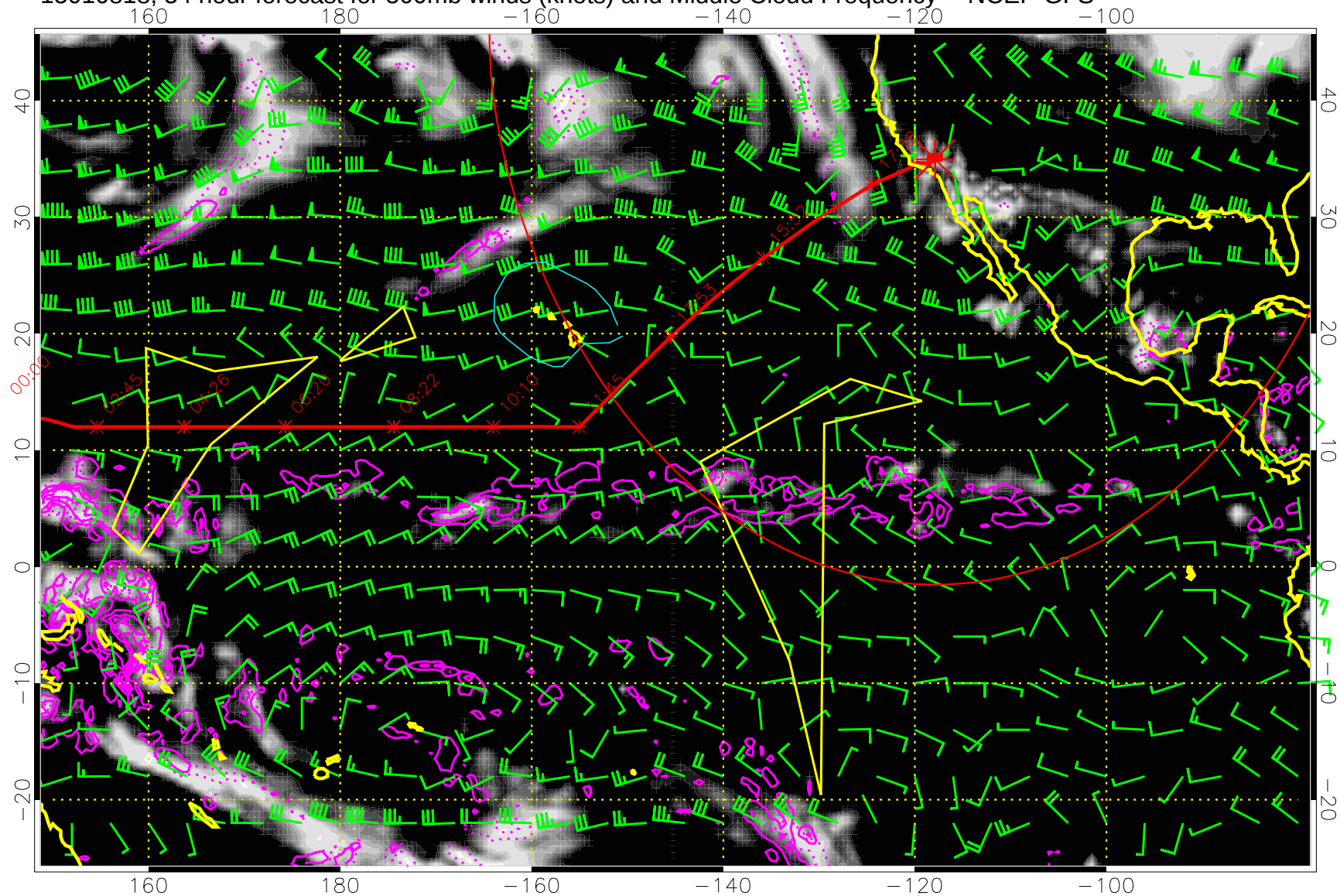
15010818, 54 hour forecast for 500mb winds (knots) and Middle Cloud Frequency -- NCEP GFS
