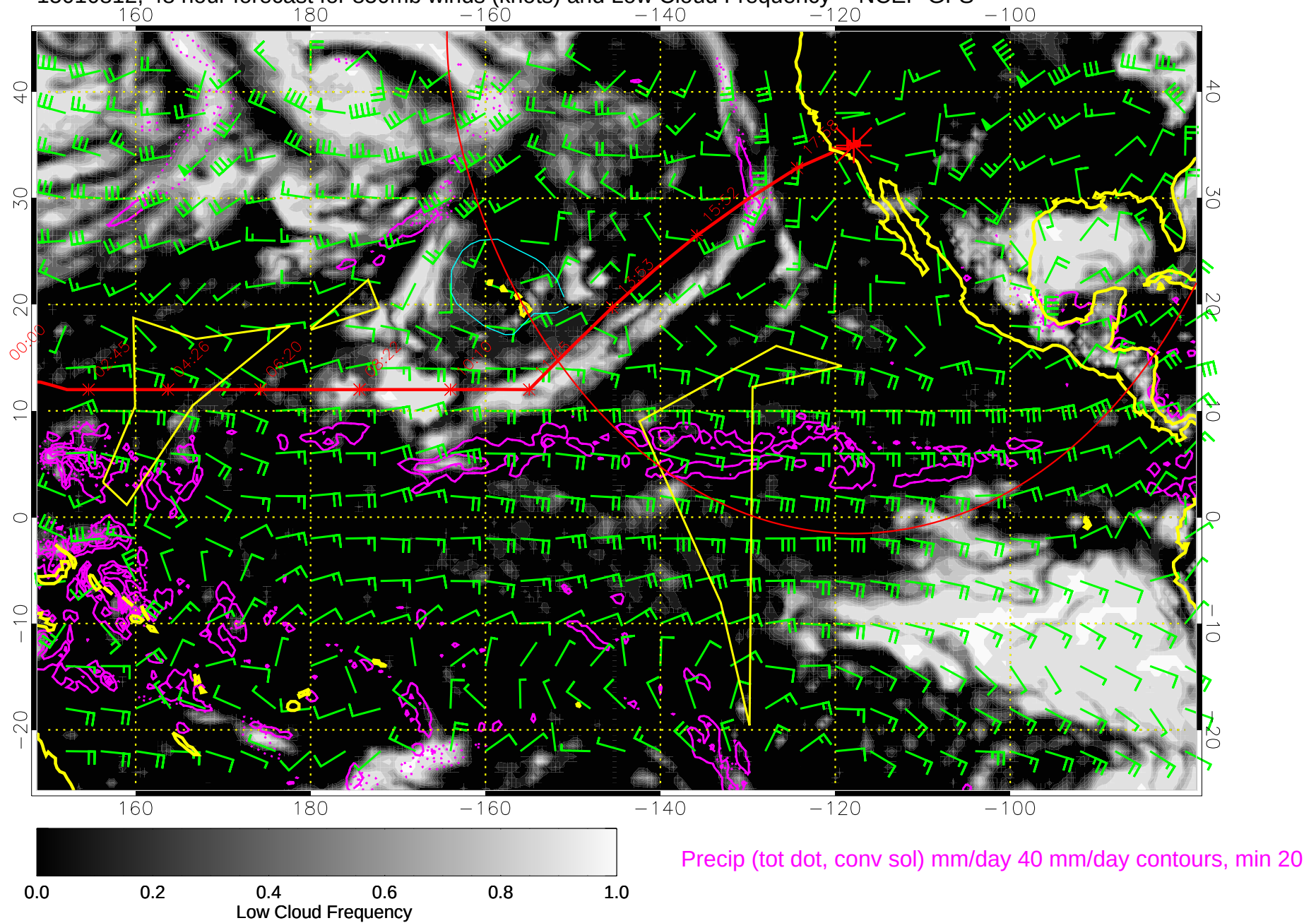
15010812, 48 hour forecast for 850mb winds (knots) and Low Cloud Frequency -- NCEP GFS
