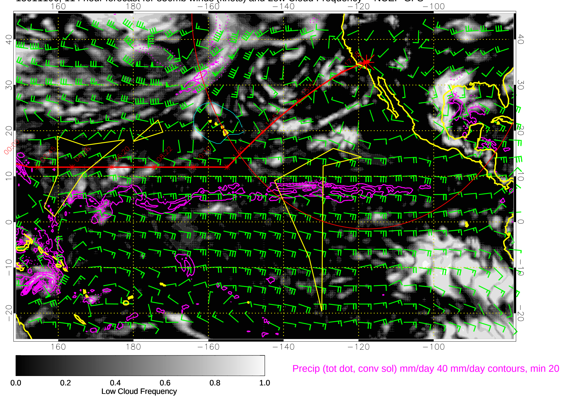
15011106, 114 hour forecast for 850mb winds (knots) and Low Cloud Frequency -- NCEP GFS
