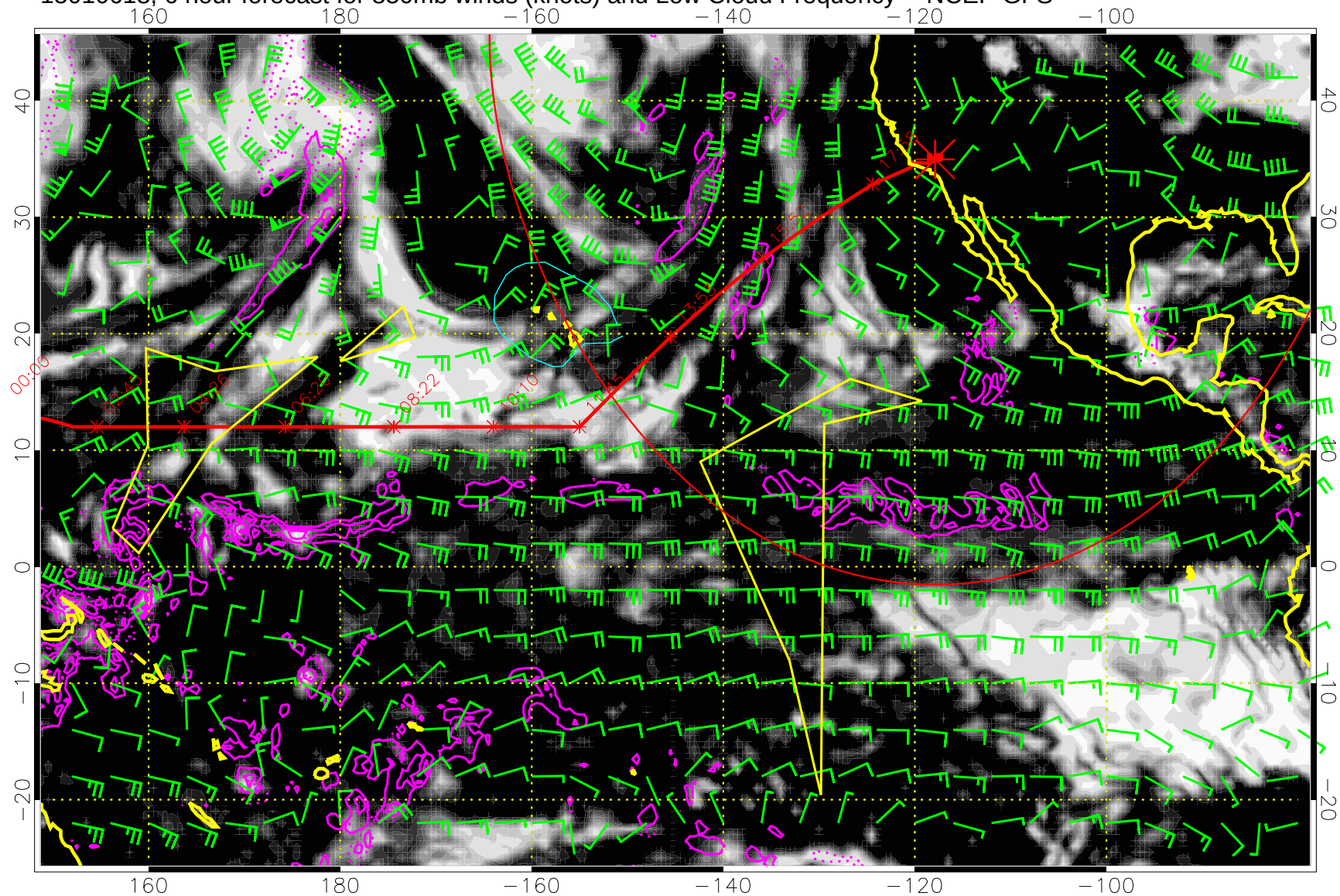
15010618, 6 hour forecast for 850mb winds (knots) and Low Cloud Frequency -- NCEP GFS
