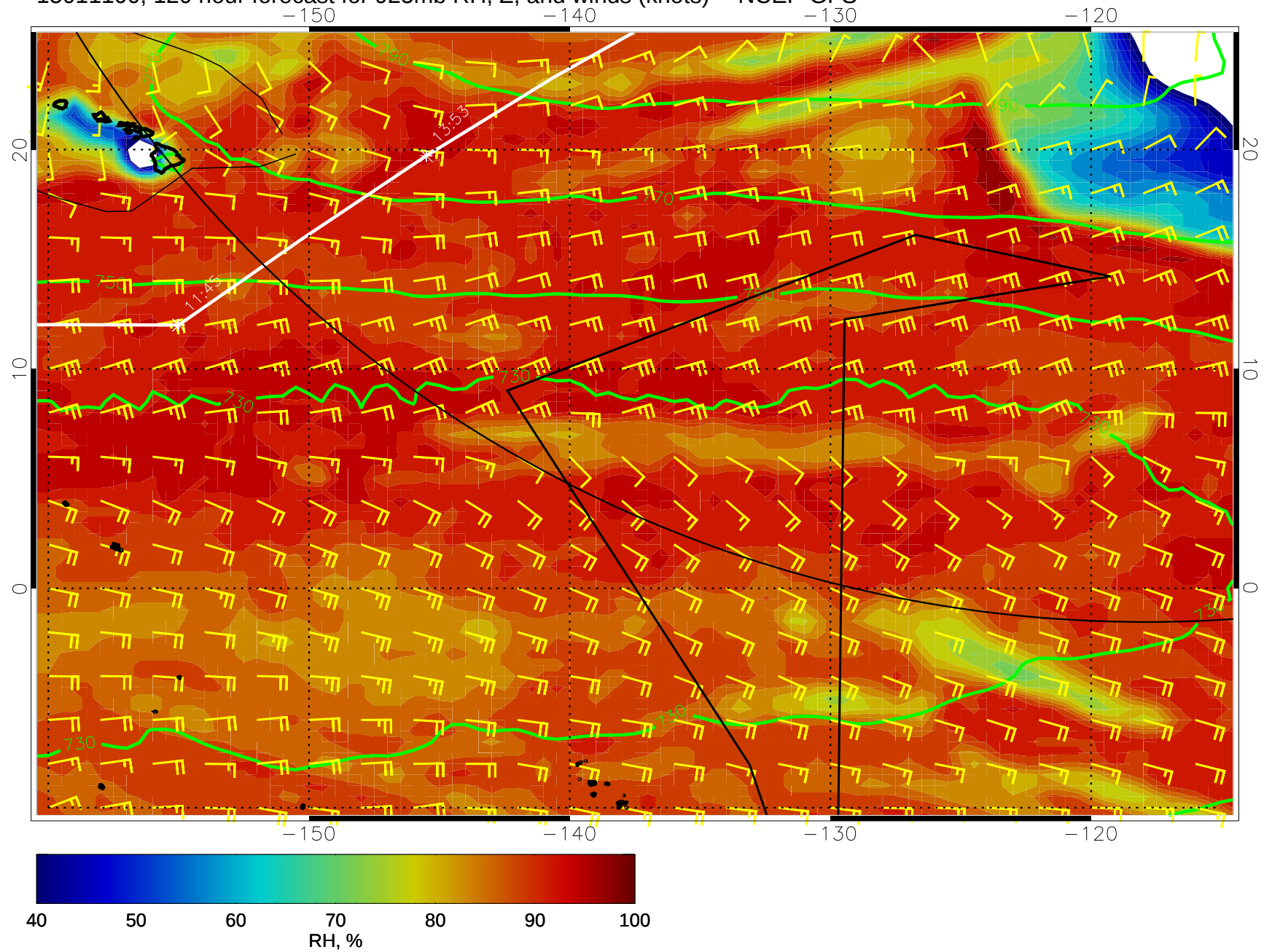
15011100, 120 hour forecast for 925mb RH, Z, and winds (knots) -- NCEP GFS
