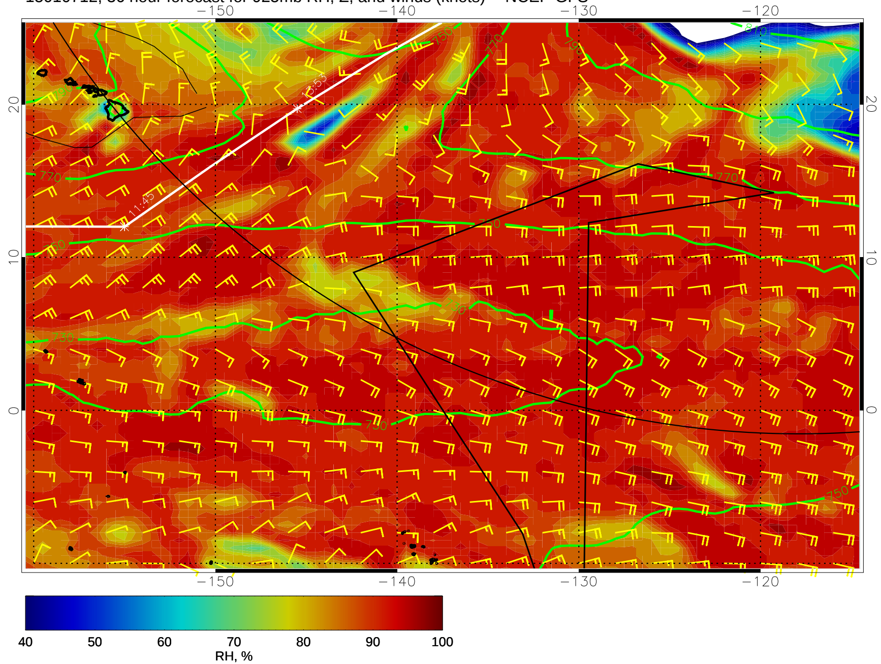
15010712, 36 hour forecast for 925mb RH, Z, and winds (knots) -- NCEP GFS
