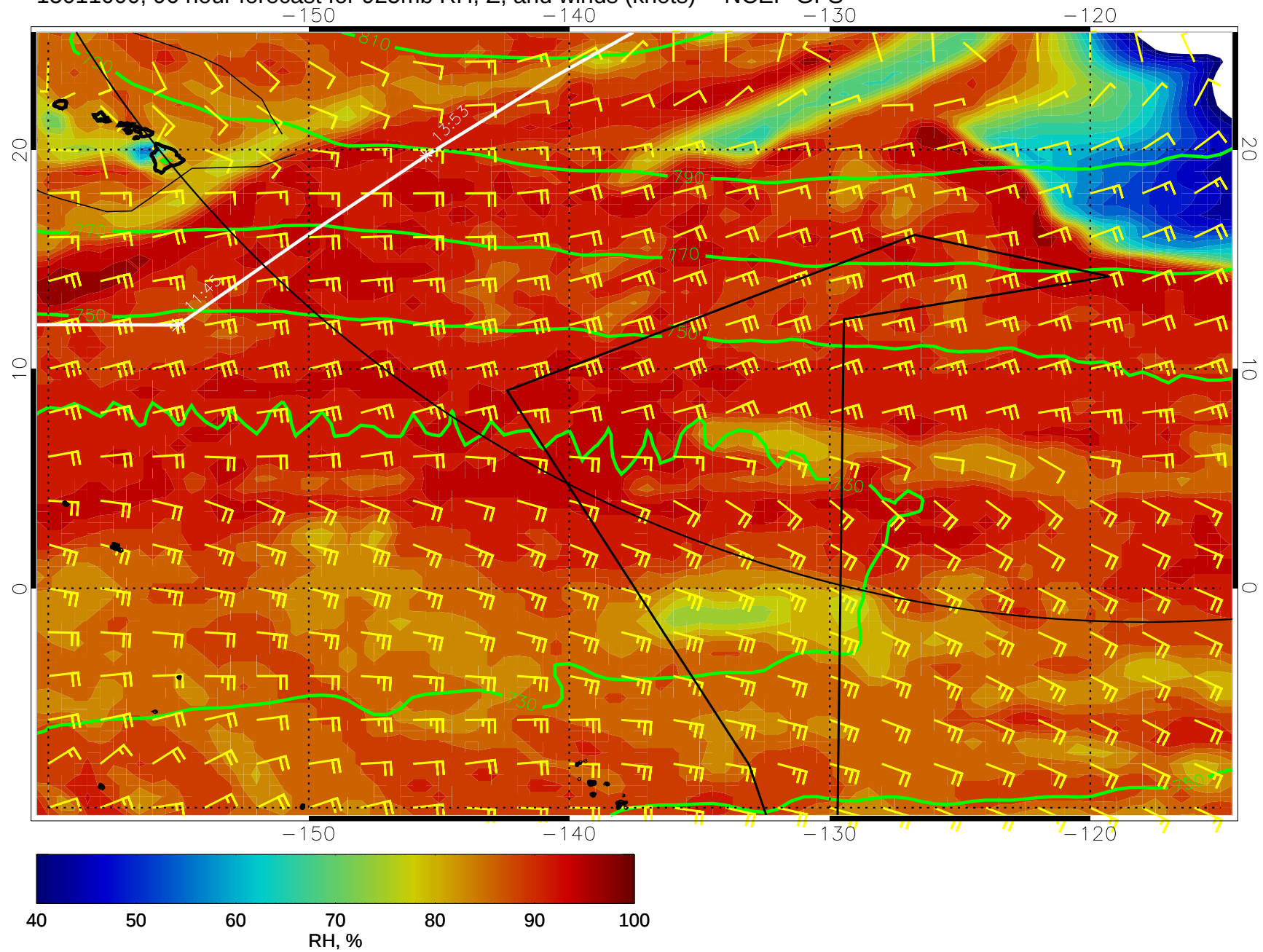
15011000, 96 hour forecast for 925mb RH, Z, and winds (knots) -- NCEP GFS
