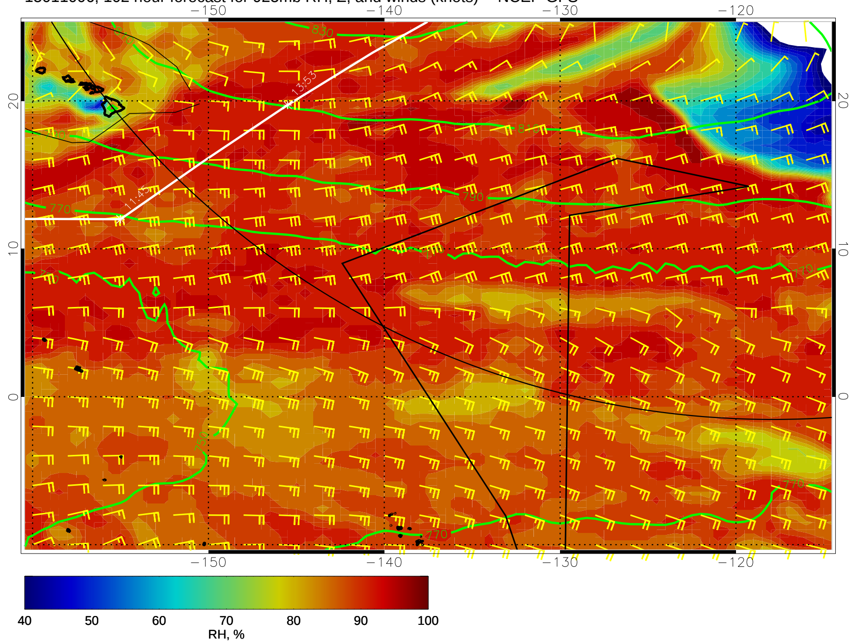
15011006, 102 hour forecast for 925mb RH, Z, and winds (knots) -- NCEP GFS
