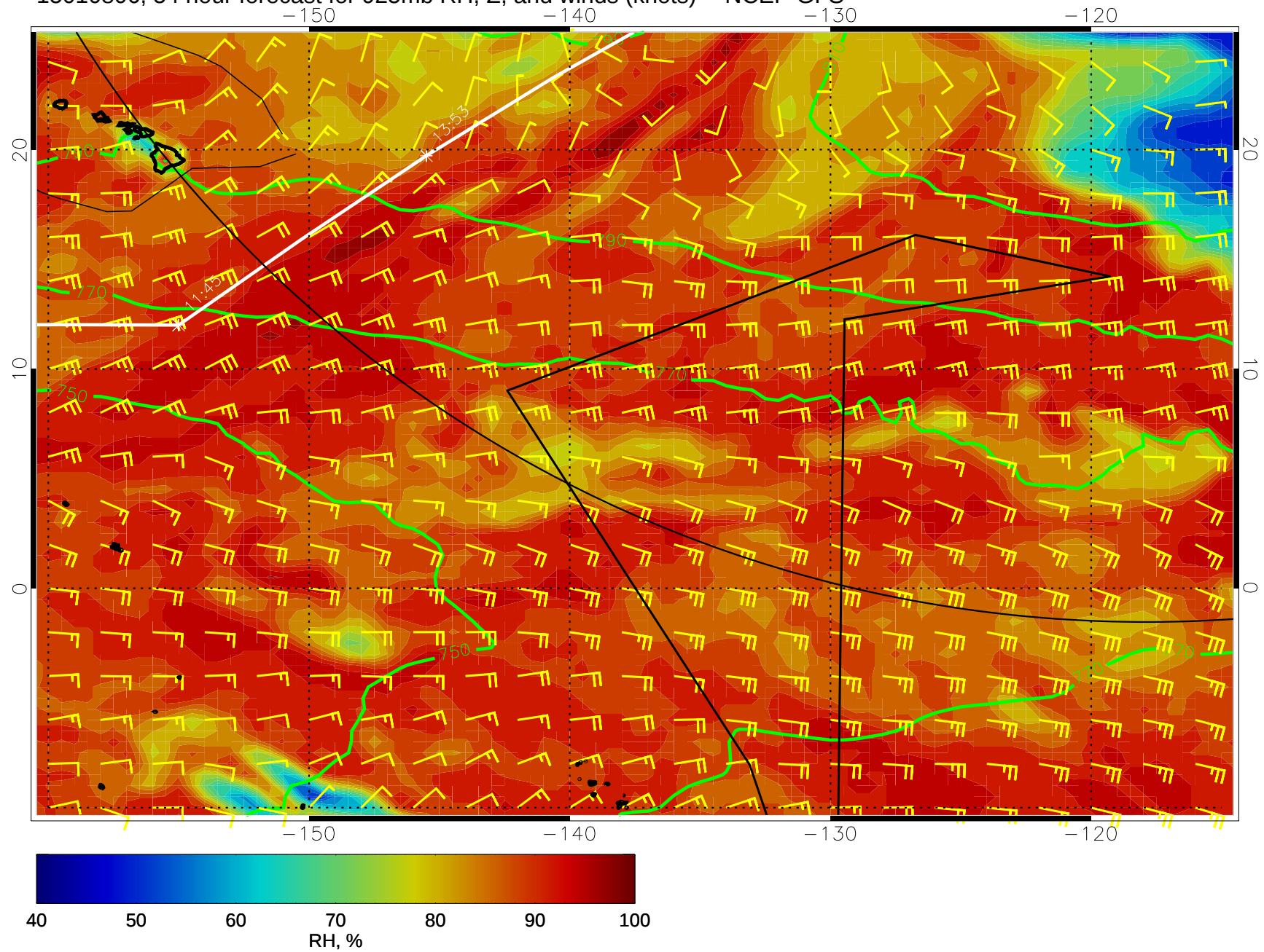
15010806, 54 hour forecast for 925mb RH, Z, and winds (knots) -- NCEP GFS
