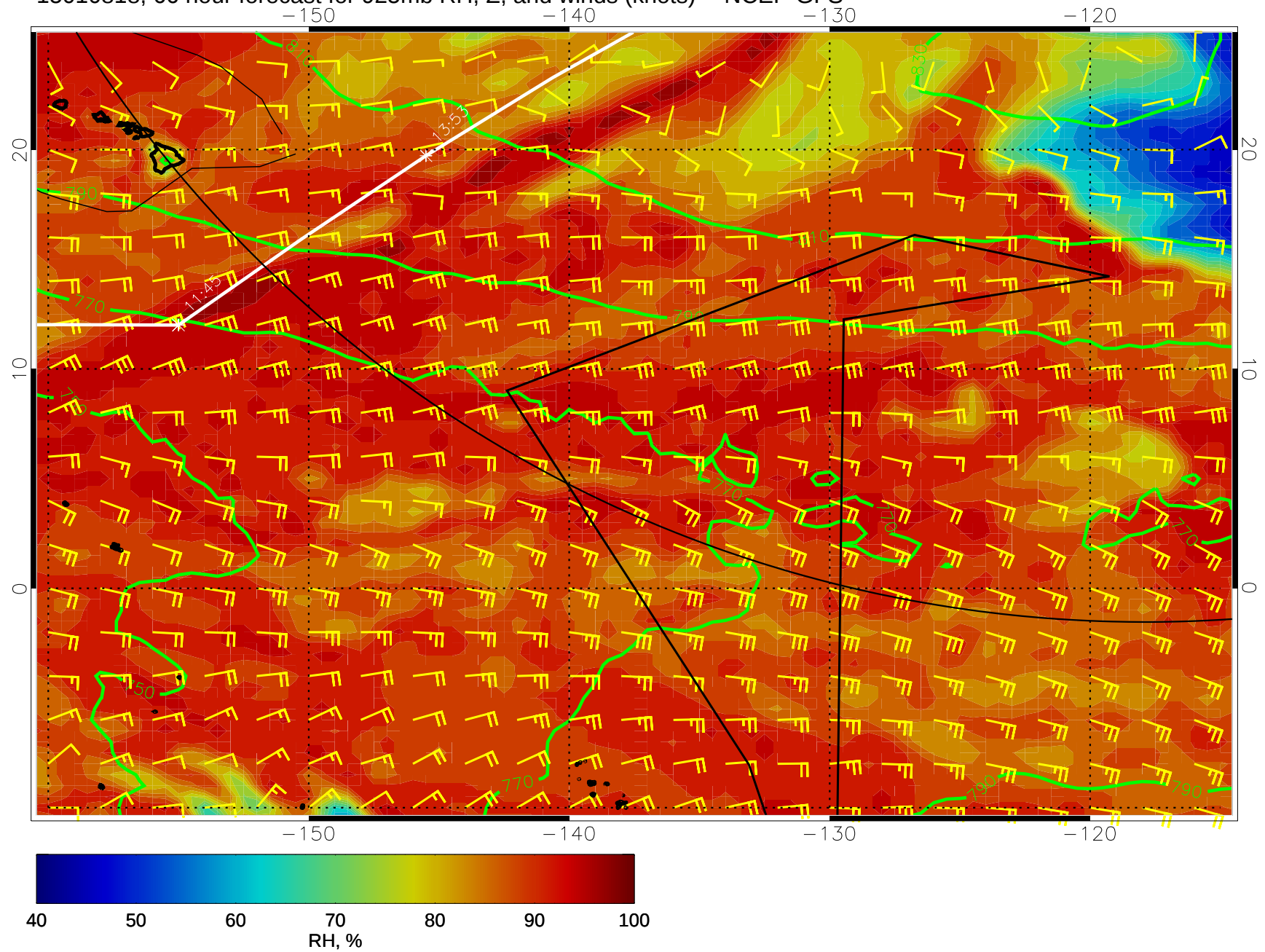
15010818, 66 hour forecast for 925mb RH, Z, and winds (knots) -- NCEP GFS
