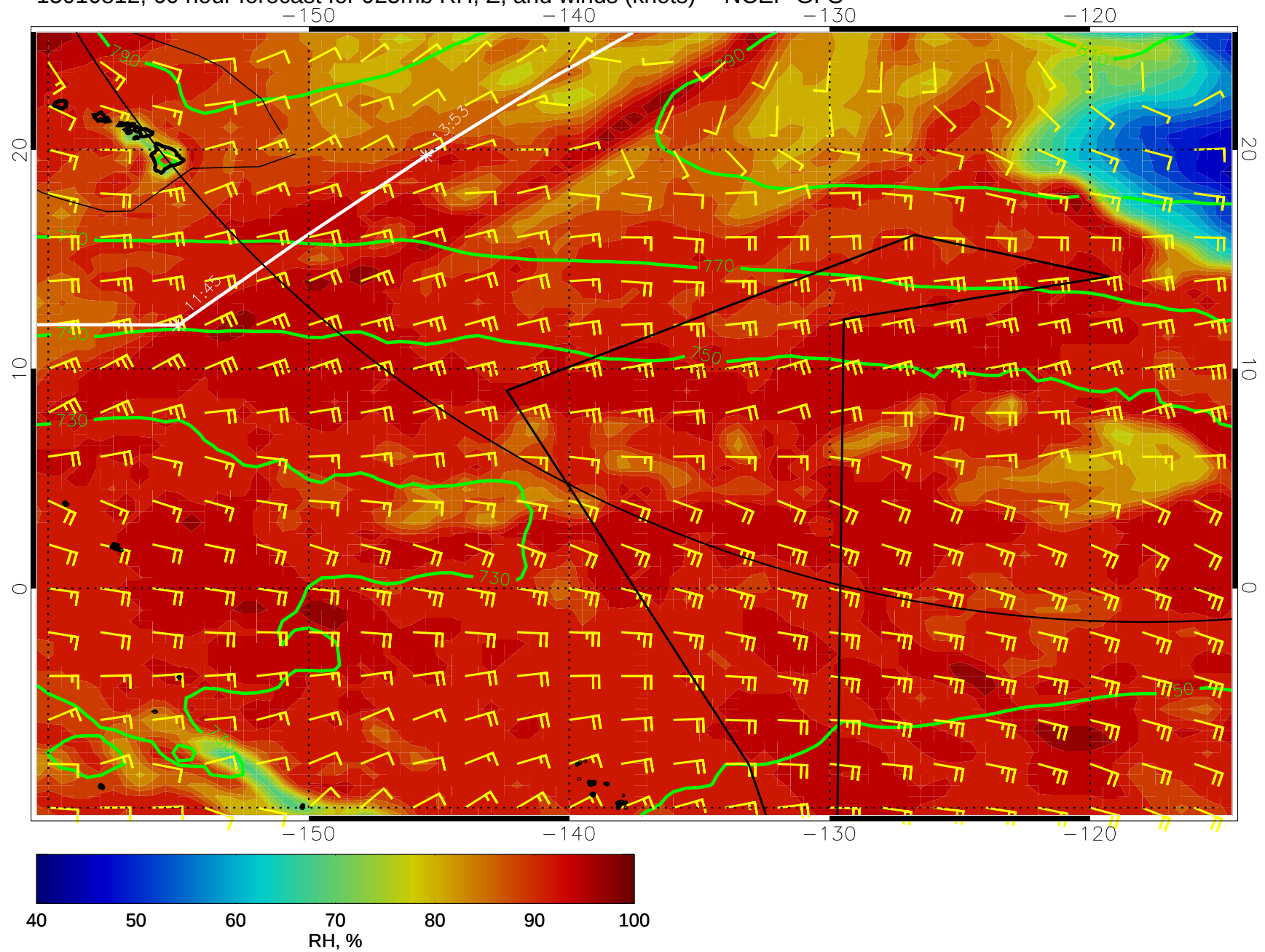
15010812, 60 hour forecast for 925mb RH, Z, and winds (knots) -- NCEP GFS
