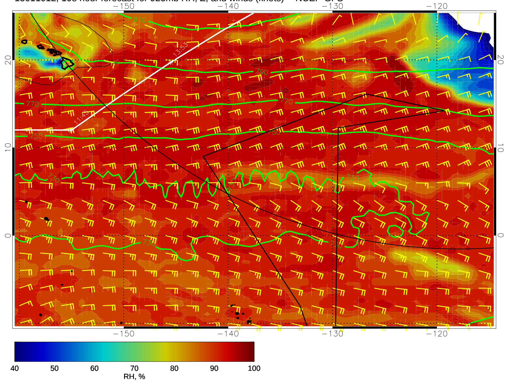
15011012, 108 hour forecast for 925mb RH, Z, and winds (knots) -- NCEP GFS
