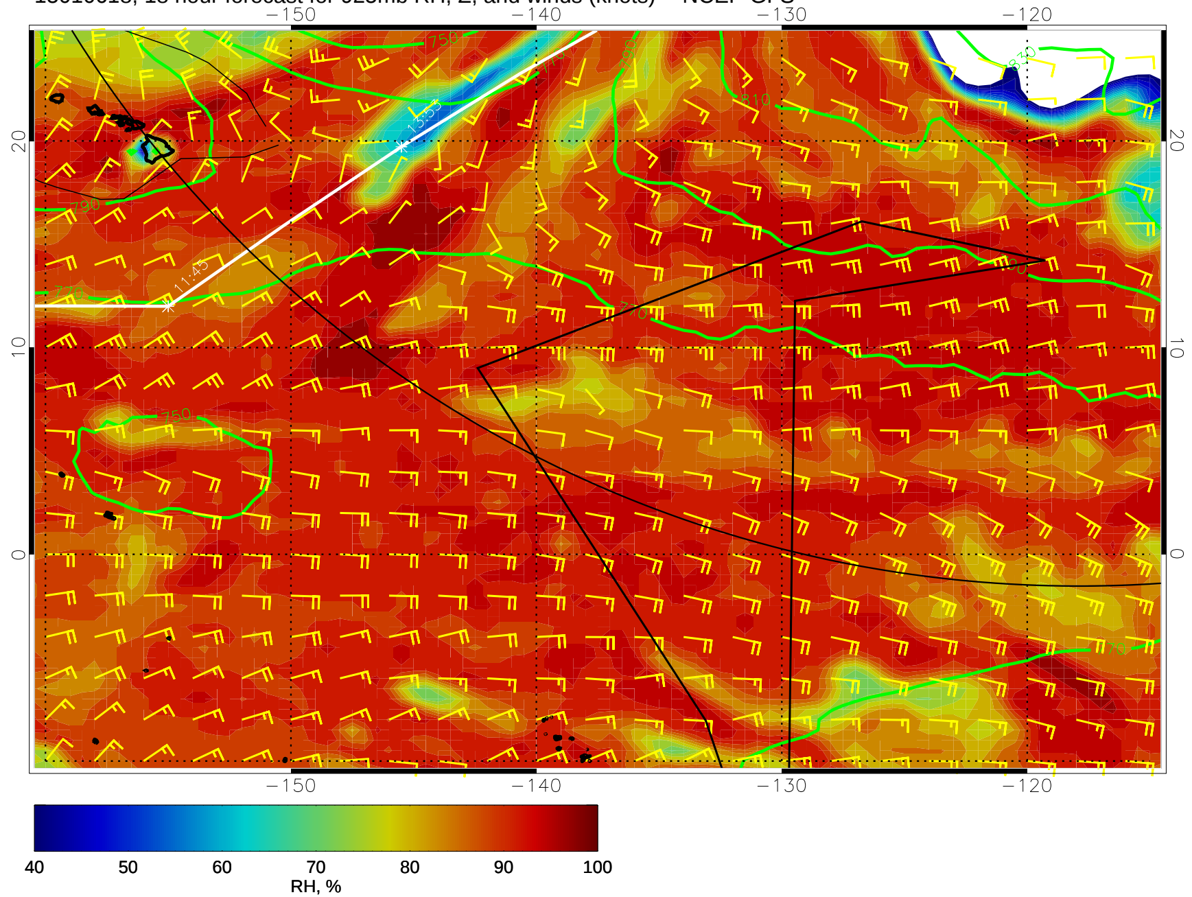
15010618, 18 hour forecast for 925mb RH, Z, and winds (knots) -- NCEP GFS
