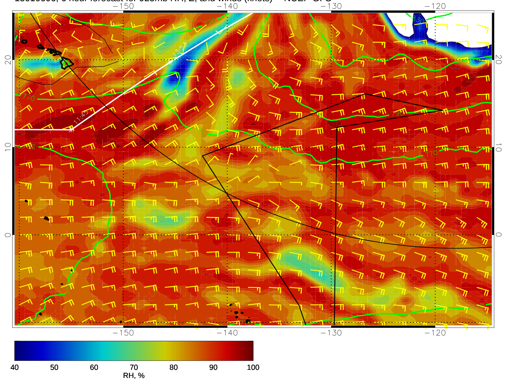
15010606, 6 hour forecast for 925mb RH, Z, and winds (knots) -- NCEP GFS
