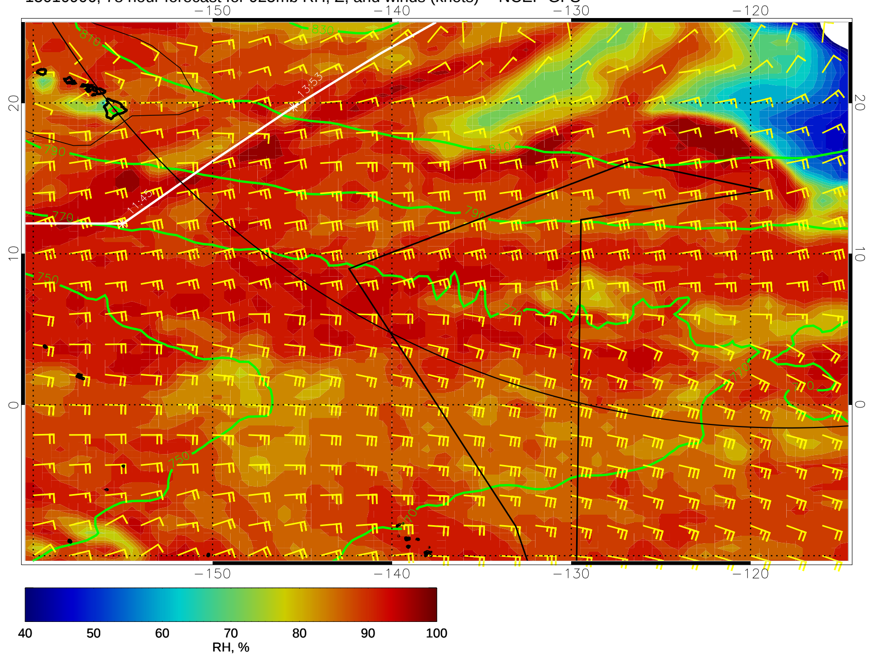
15010906, 78 hour forecast for 925mb RH, Z, and winds (knots) -- NCEP GFS
