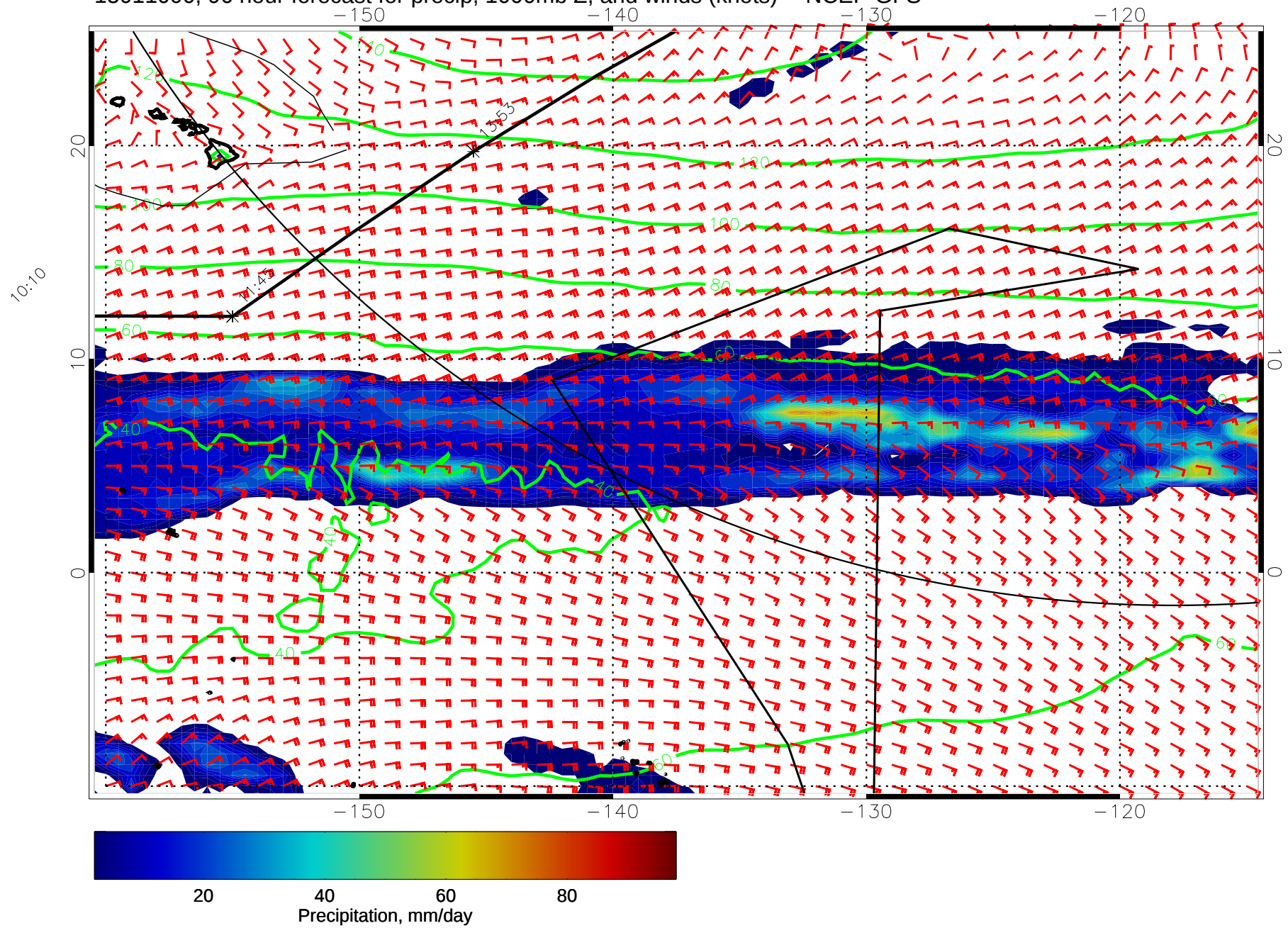
15011000, 96 hour forecast for precip, 1000mb Z, and winds (knots) -- NCEP GFS
