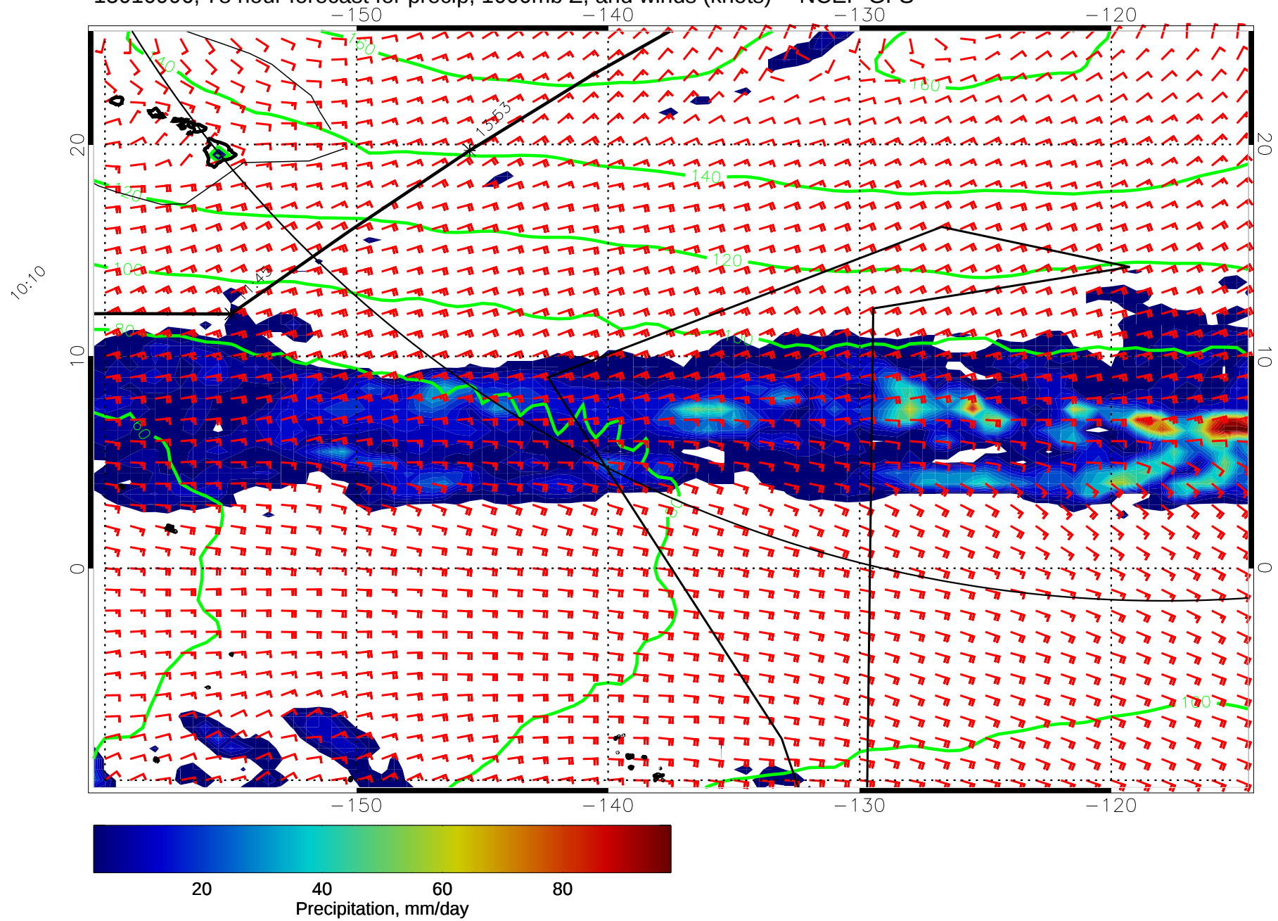
15010906, 78 hour forecast for precip, 1000mb Z, and winds (knots) -- NCEP GFS
