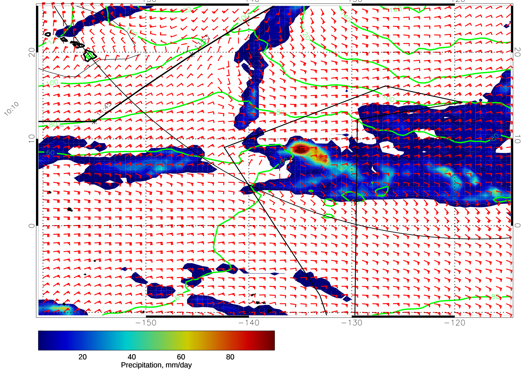
15010612, 12 hour forecast for precip, 1000mb Z, and winds (knots) -- NCEP GFS
