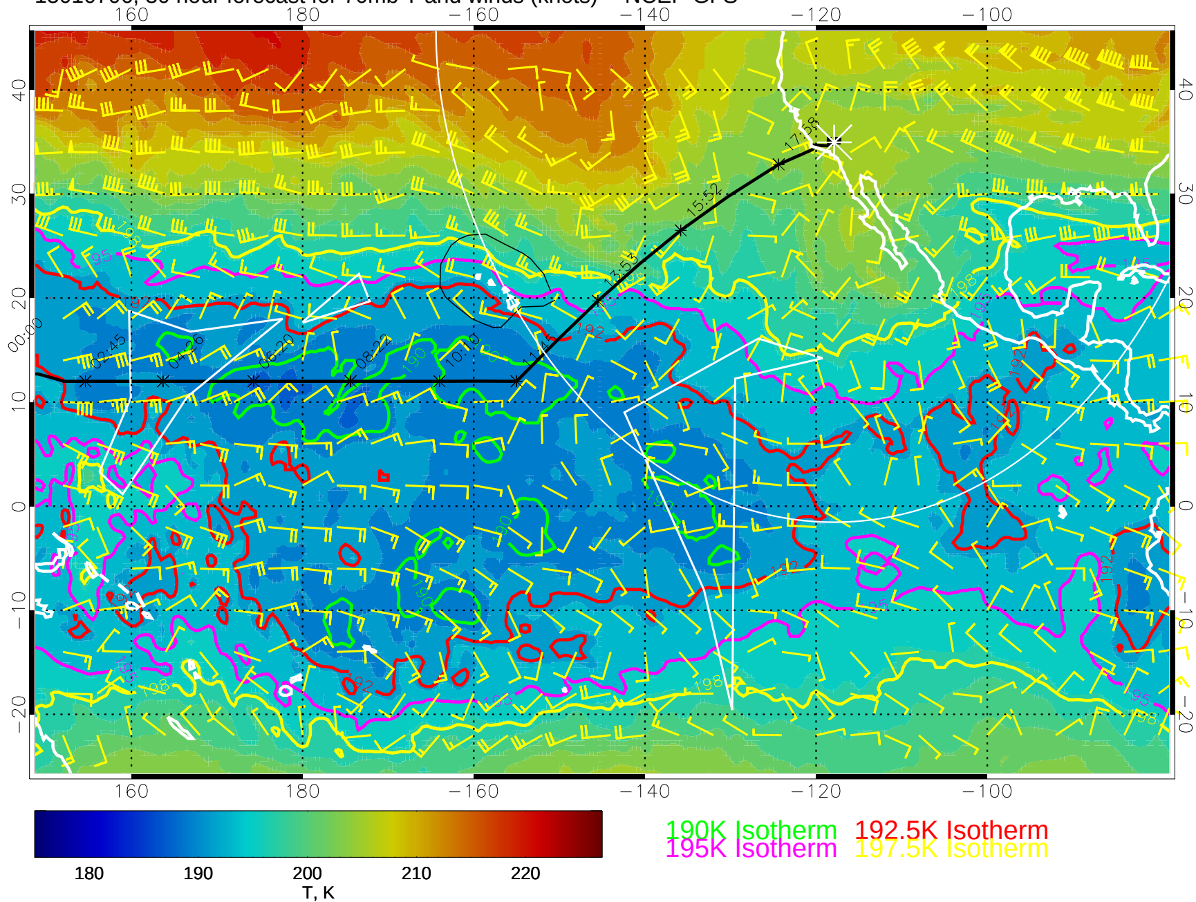
15010706, 30 hour forecast for 70mb T and winds (knots) -- NCEP GFS
