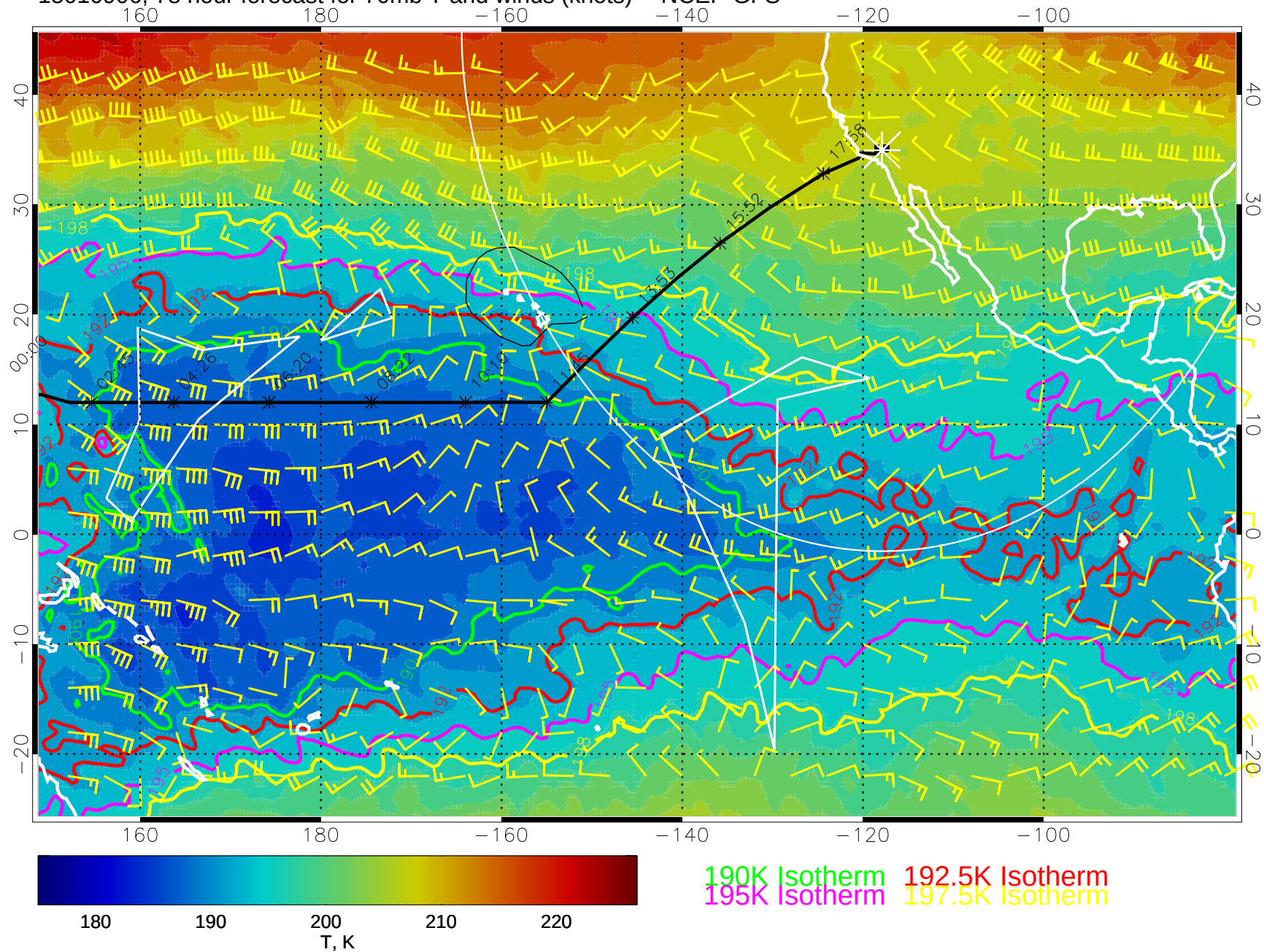
15010906, 78 hour forecast for 70mb T and winds (knots) -- NCEP GFS
