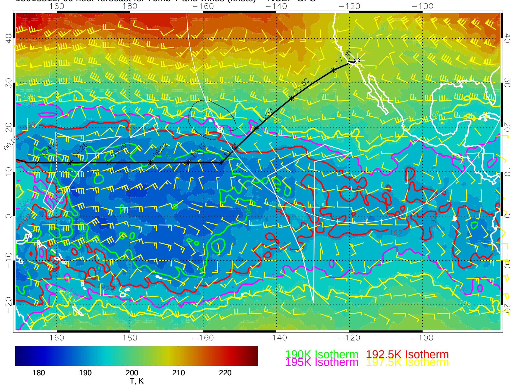
15010812, 60 hour forecast for 70mb T and winds (knots) -- NCEP GFS
