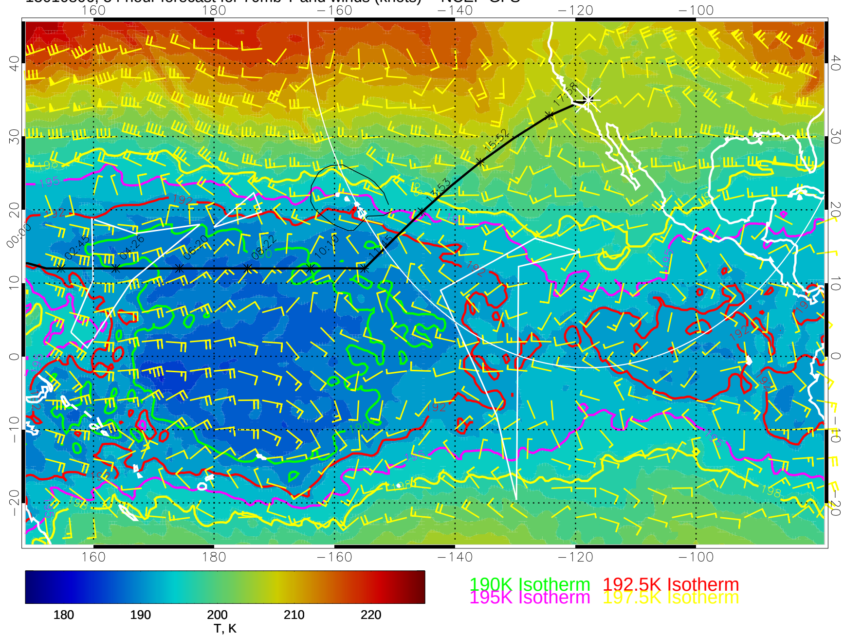
15010806, 54 hour forecast for 70mb T and winds (knots) -- NCEP GFS
