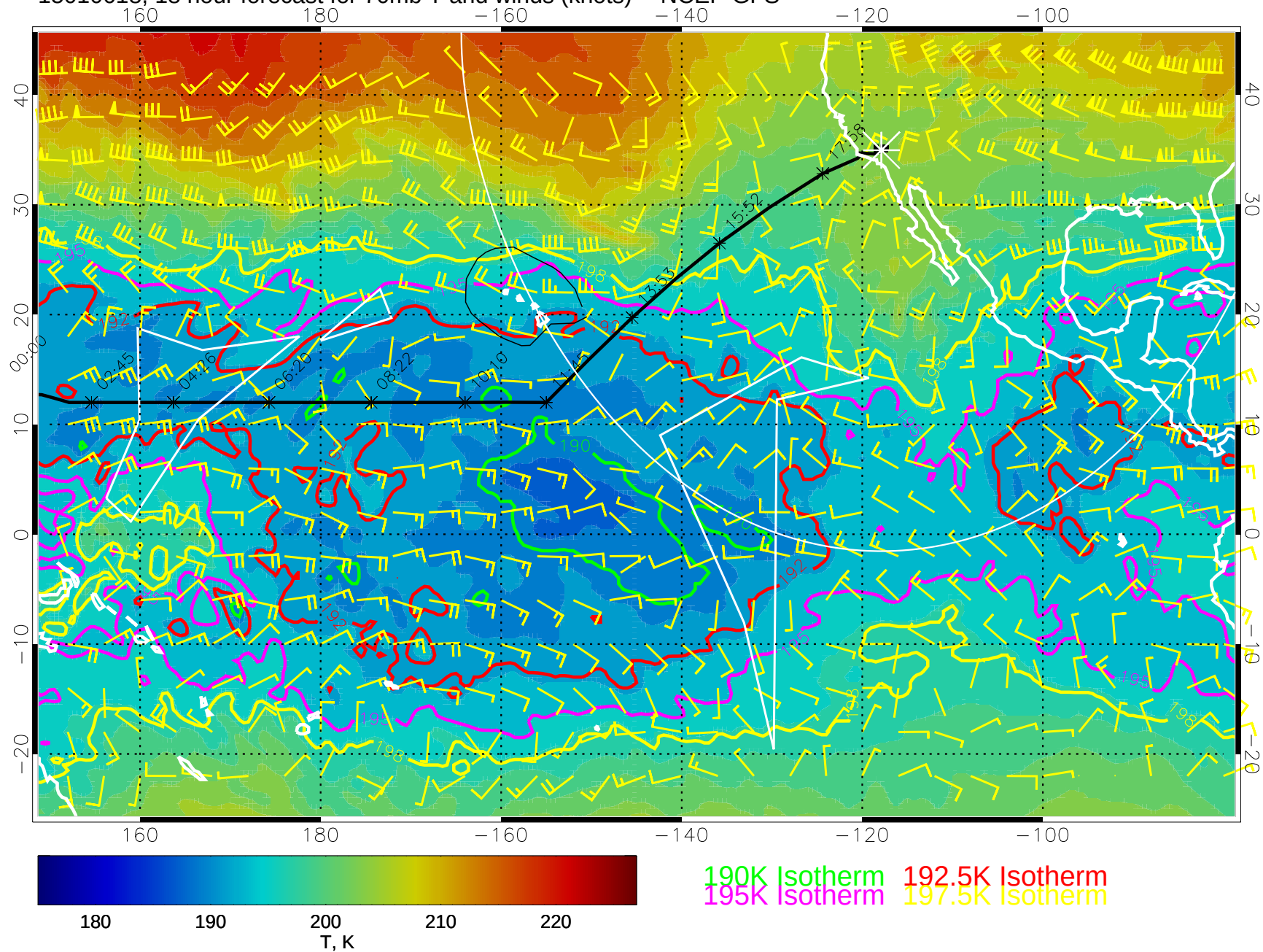
15010618, 18 hour forecast for 70mb T and winds (knots) -- NCEP GFS
