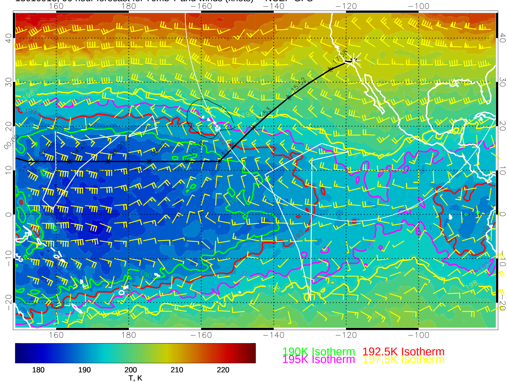
15010918, 90 hour forecast for 70mb T and winds (knots) -- NCEP GFS
