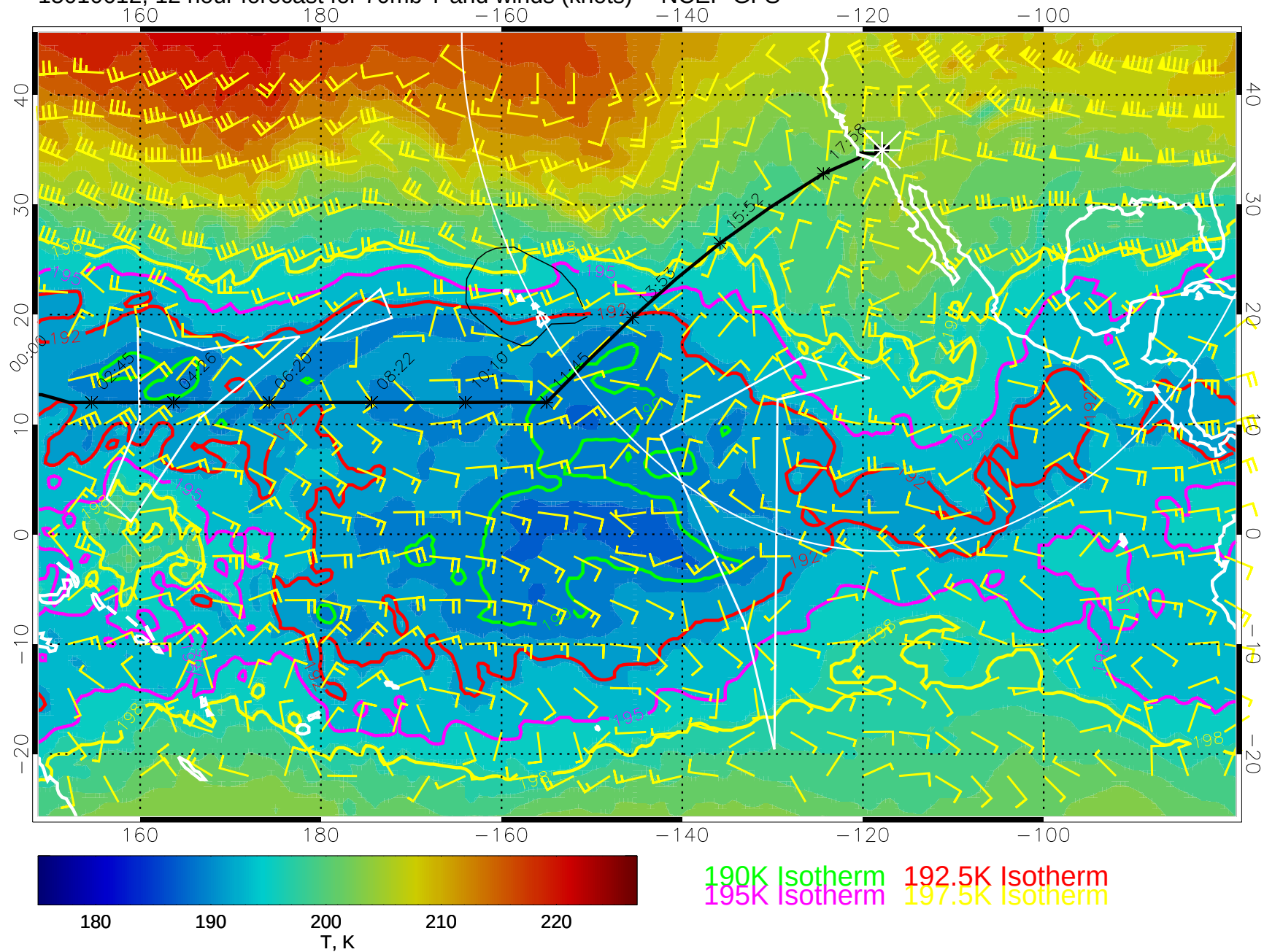
15010612, 12 hour forecast for 70mb T and winds (knots) -- NCEP GFS
