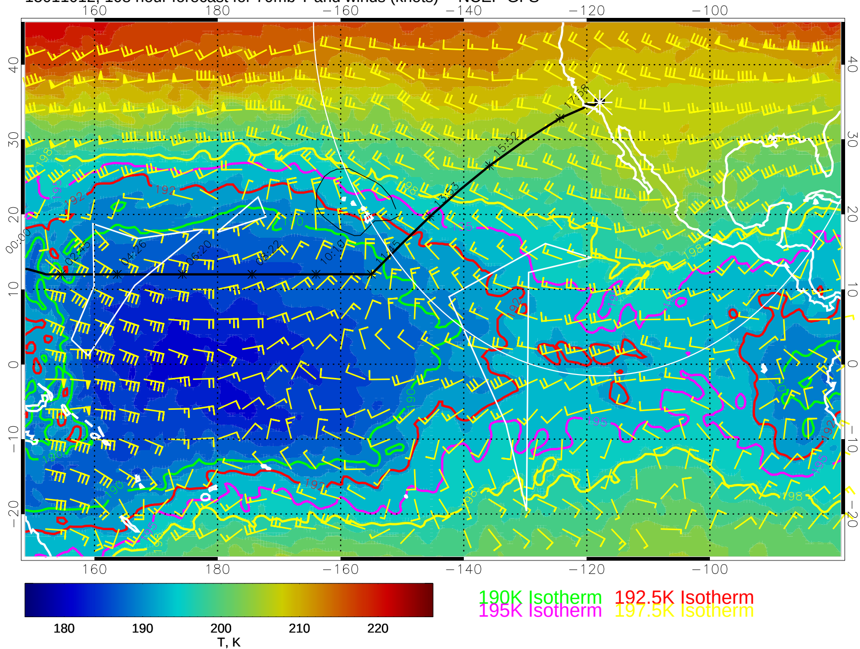
15011012, 108 hour forecast for 70mb T and winds (knots) -- NCEP GFS
