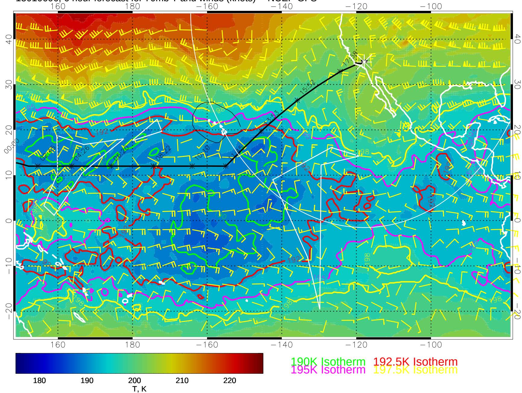
15010606, 6 hour forecast for 70mb T and winds (knots) -- NCEP GFS
