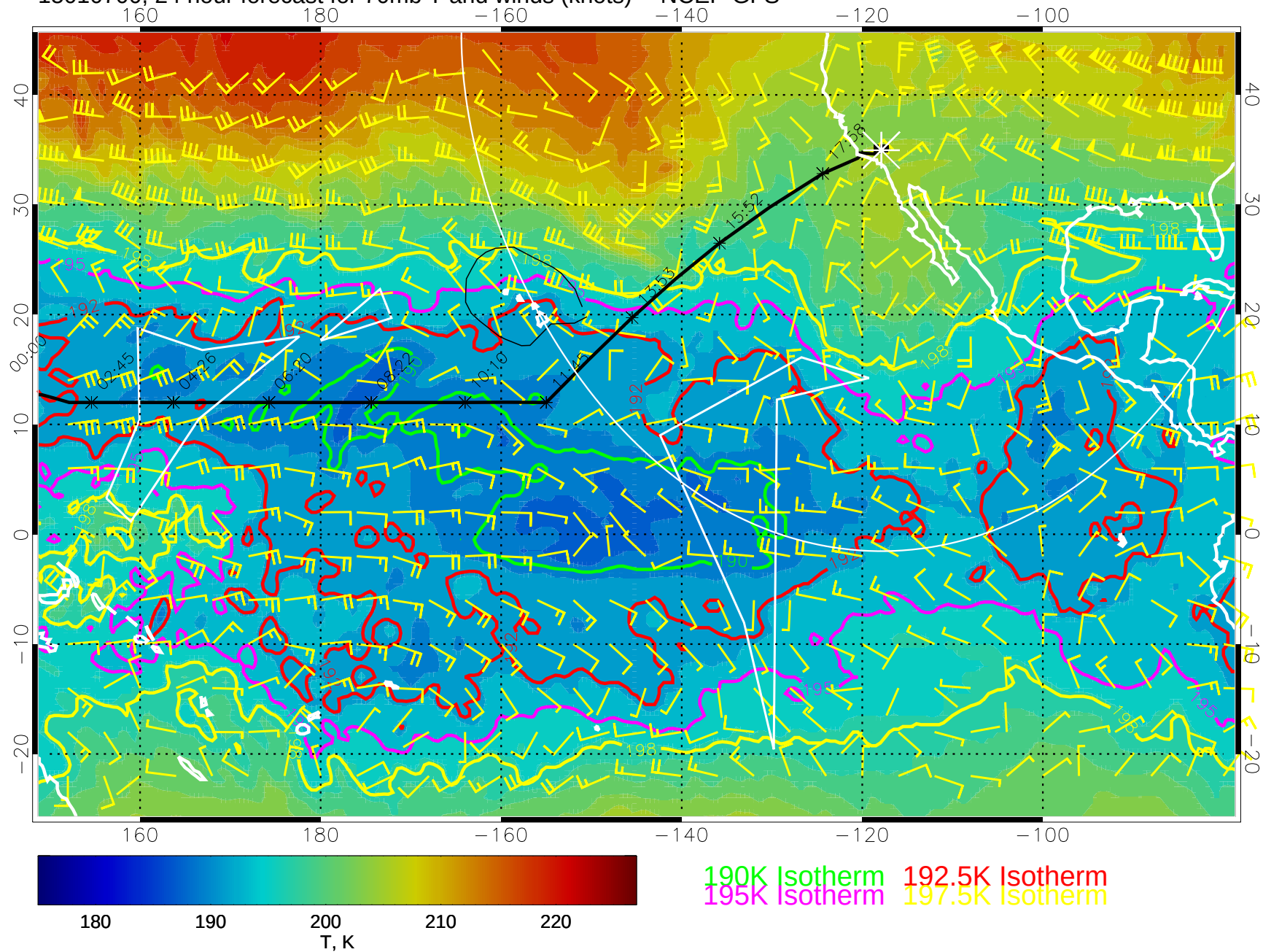
15010700, 24 hour forecast for 70mb T and winds (knots) -- NCEP GFS
