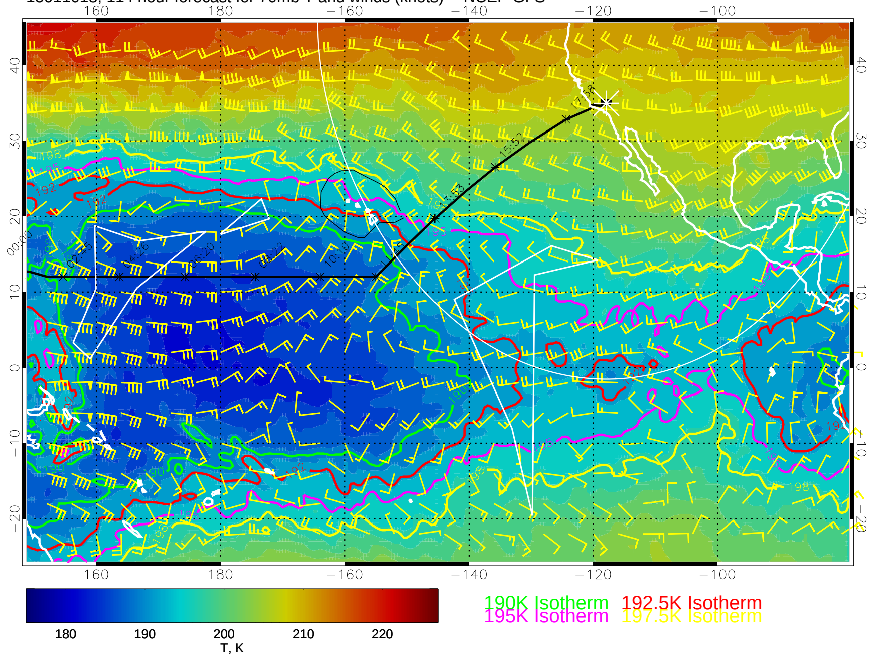
15011018, 114 hour forecast for 70mb T and winds (knots) -- NCEP GFS
