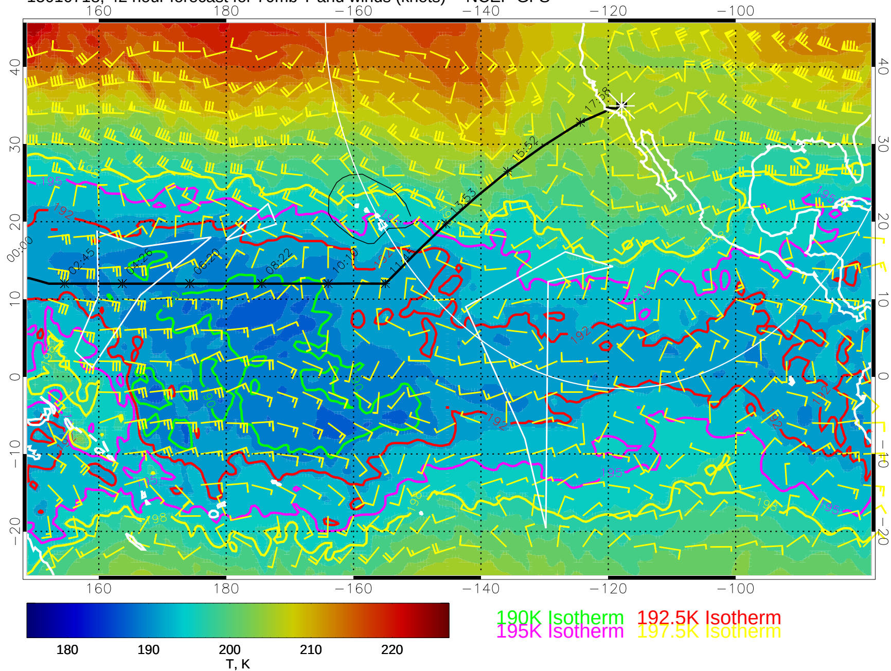
15010718, 42 hour forecast for 70mb T and winds (knots) -- NCEP GFS
