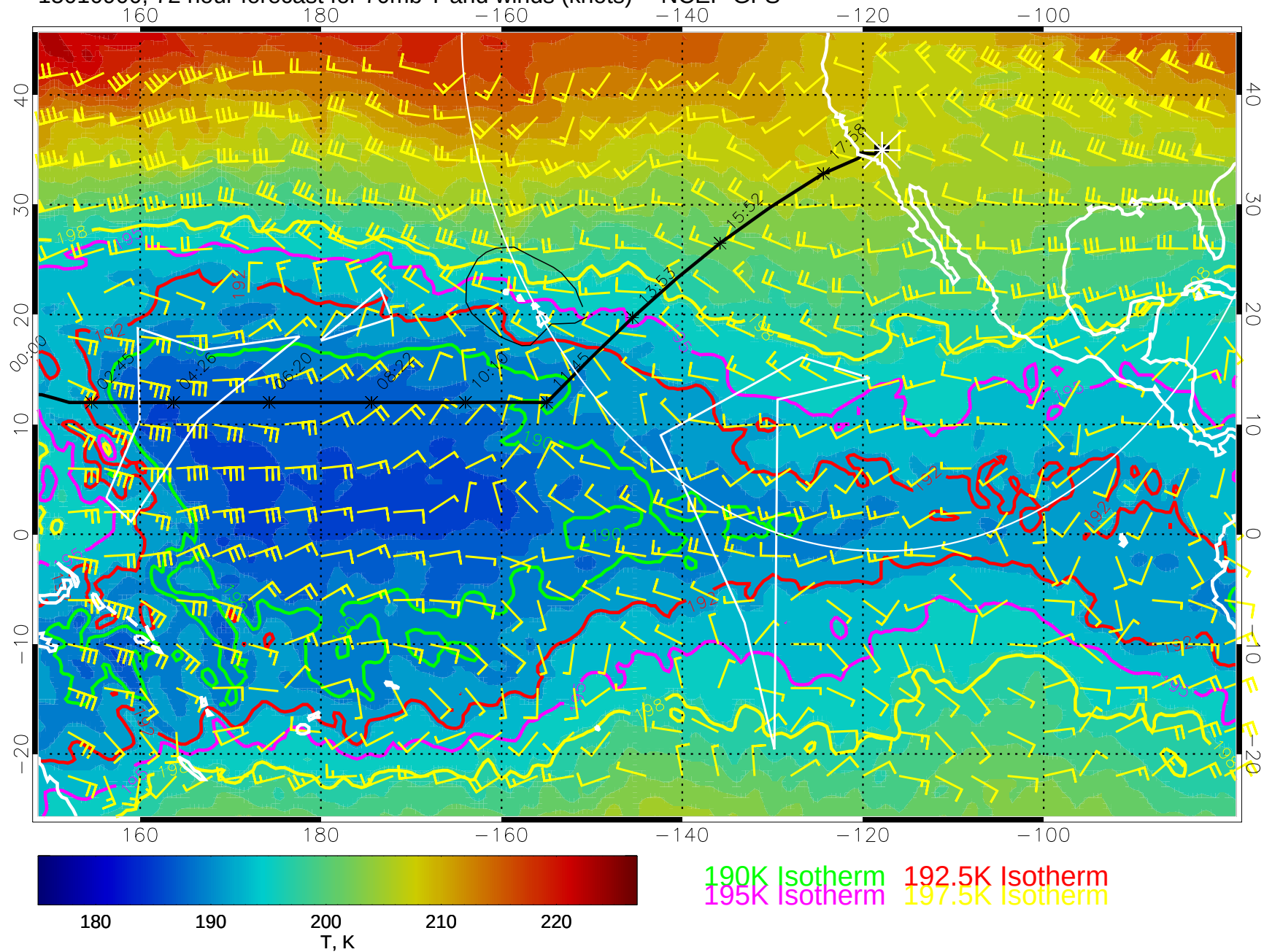
15010900, 72 hour forecast for 70mb T and winds (knots) -- NCEP GFS
