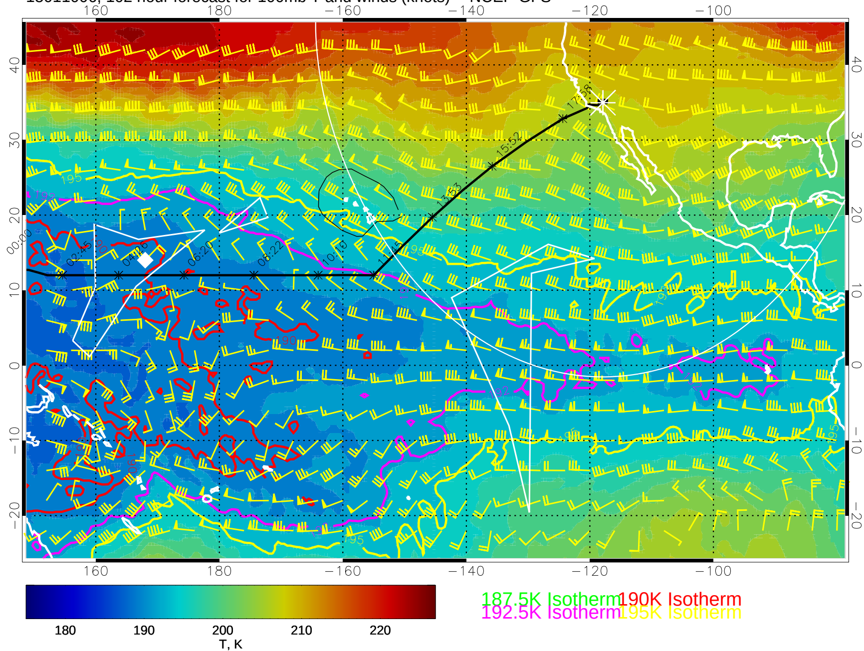
15011006, 102 hour forecast for 100mb T and winds (knots) -- NCEP GFS
