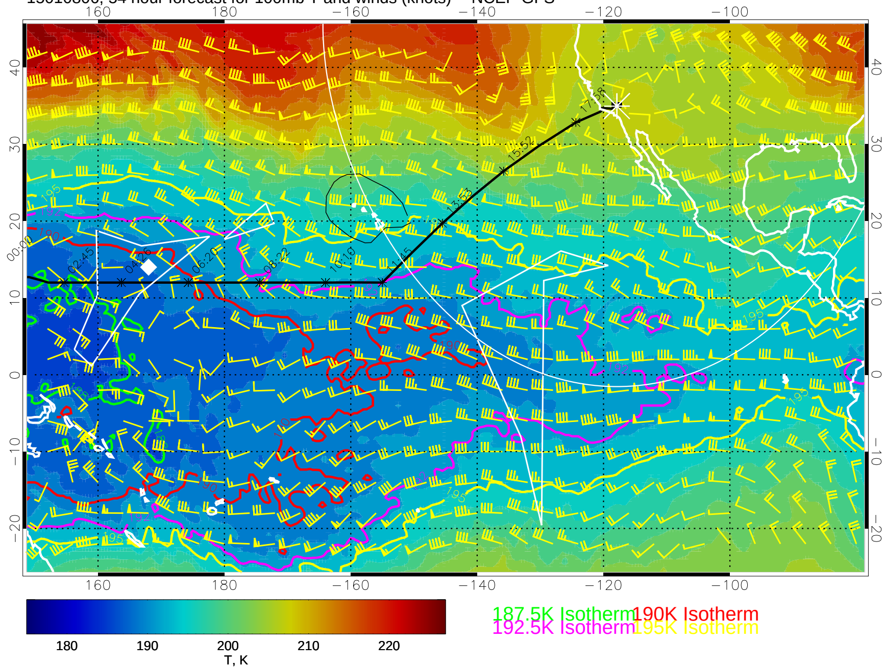
15010806, 54 hour forecast for 100mb T and winds (knots) -- NCEP GFS
