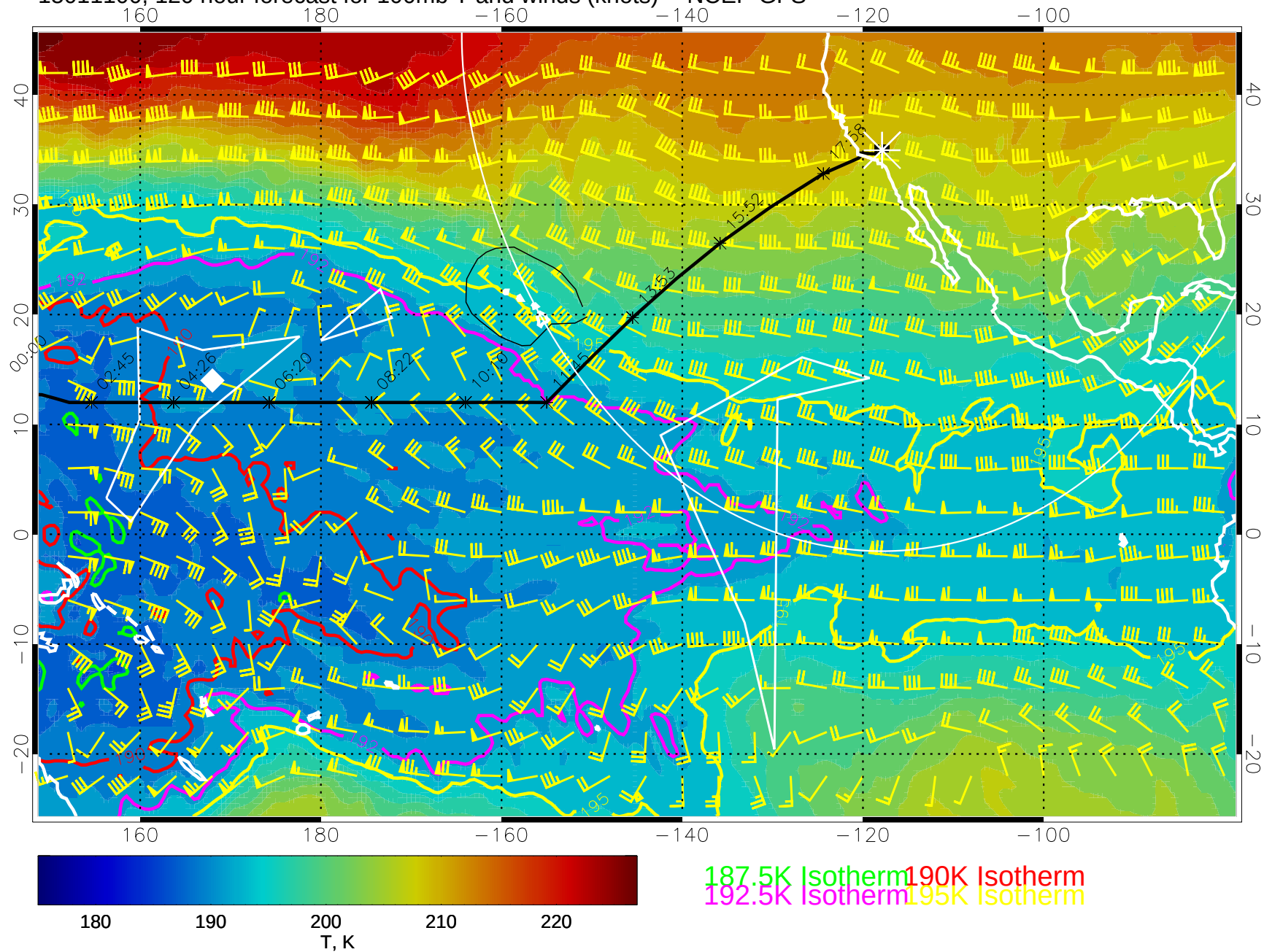
15011100, 120 hour forecast for 100mb T and winds (knots) -- NCEP GFS
