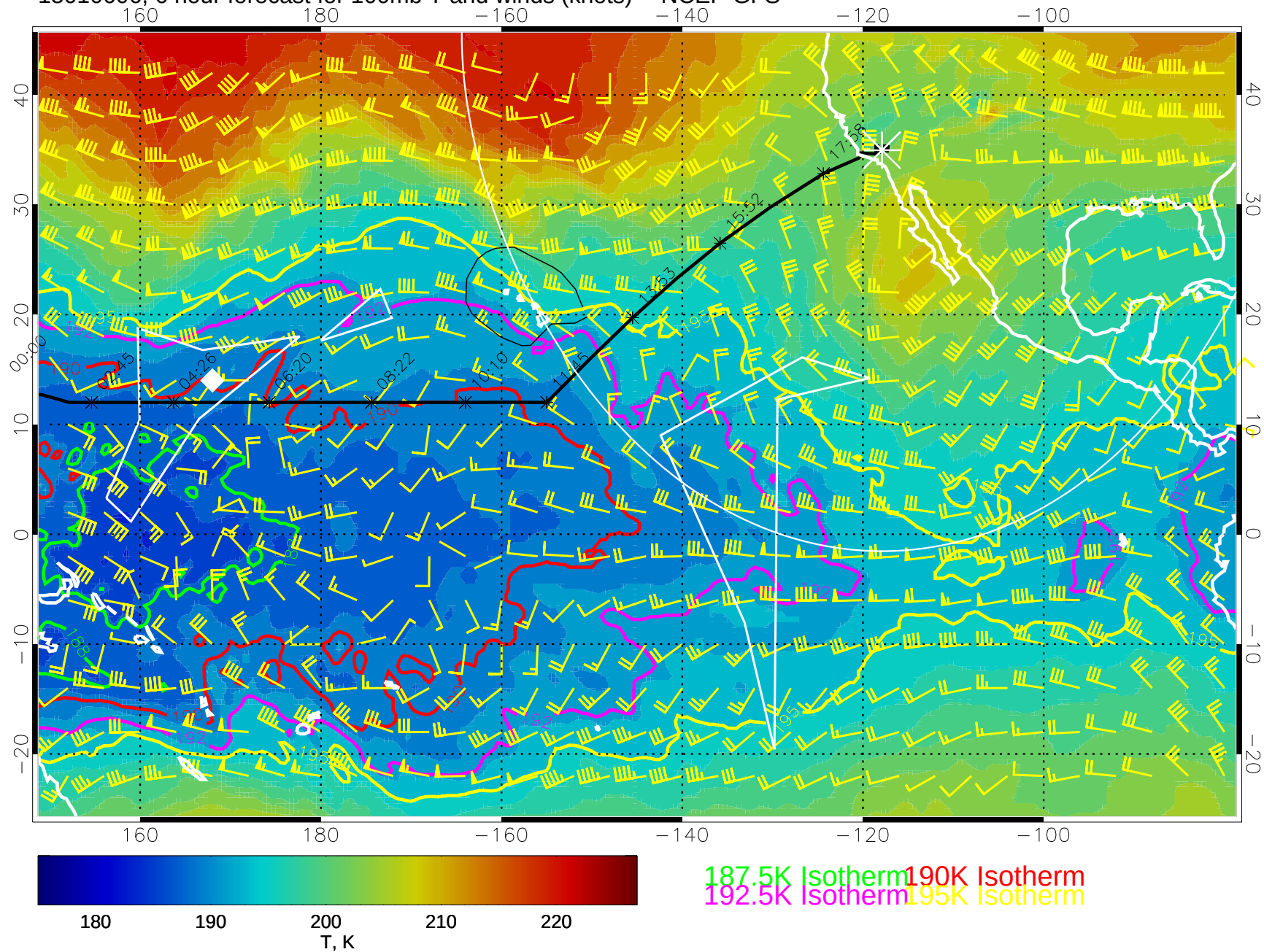
15010606, 6 hour forecast for 100mb T and winds (knots) -- NCEP GFS
