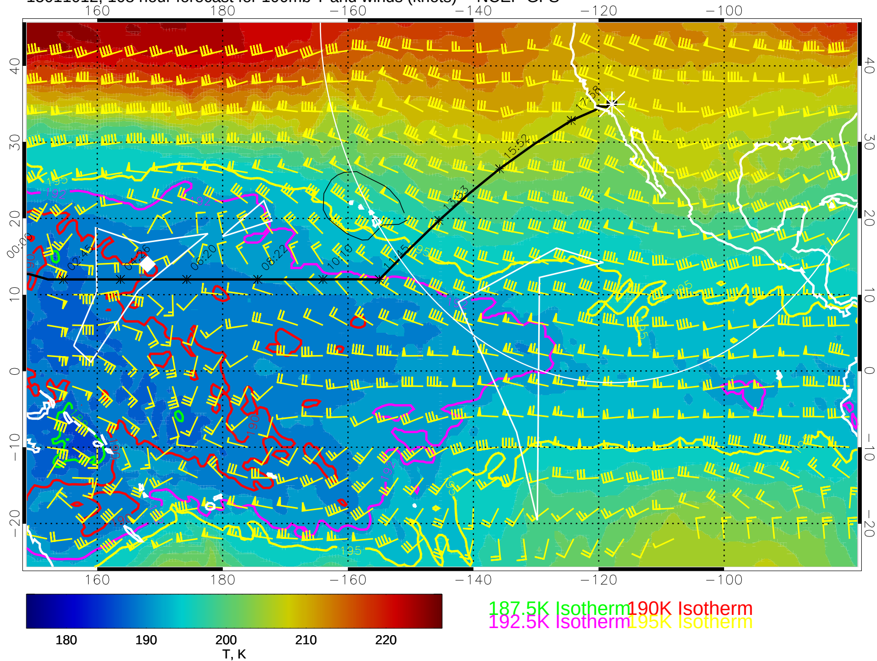
15011012, 108 hour forecast for 100mb T and winds (knots) -- NCEP GFS
