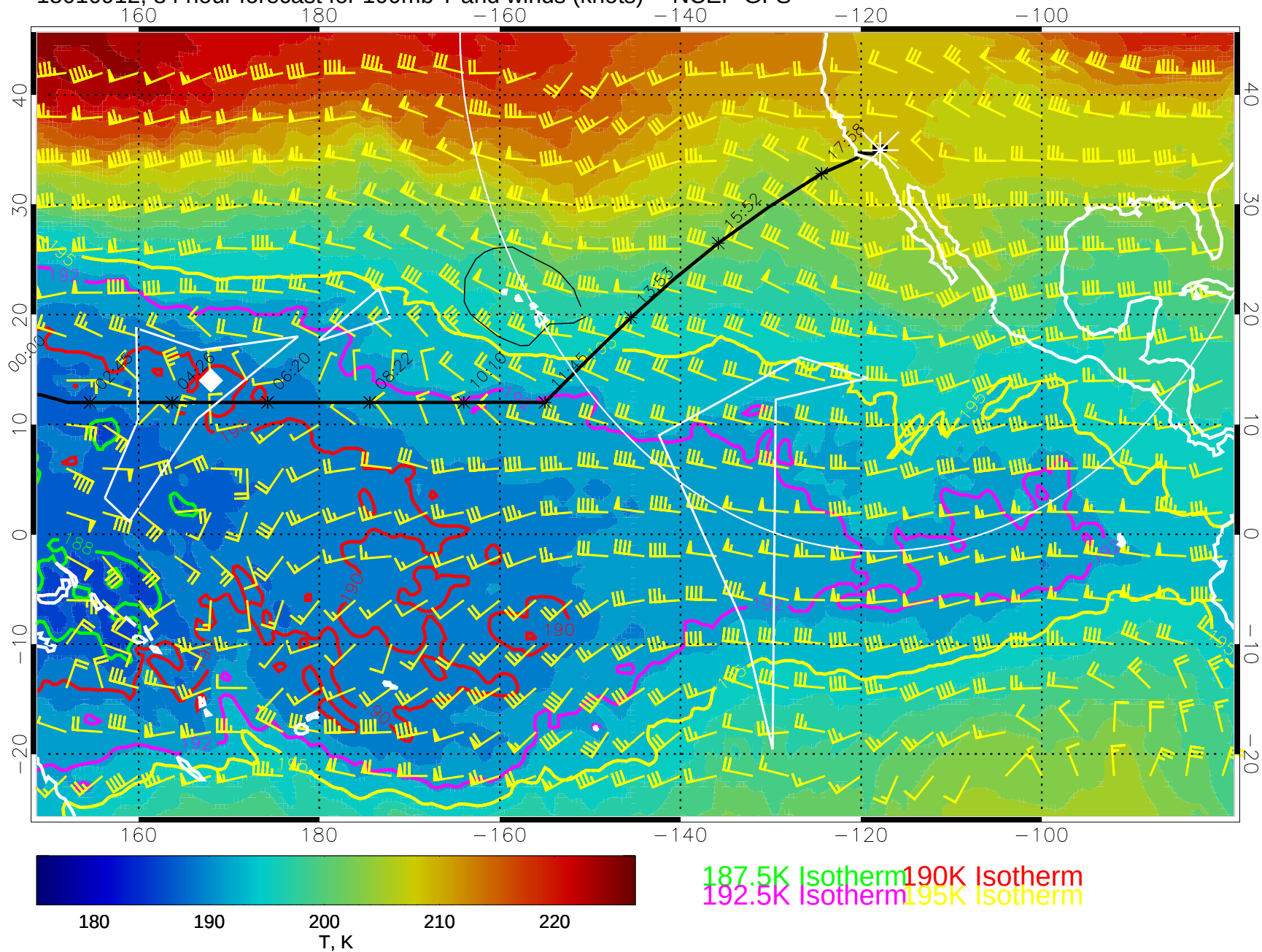
15010912, 84 hour forecast for 100mb T and winds (knots) -- NCEP GFS
