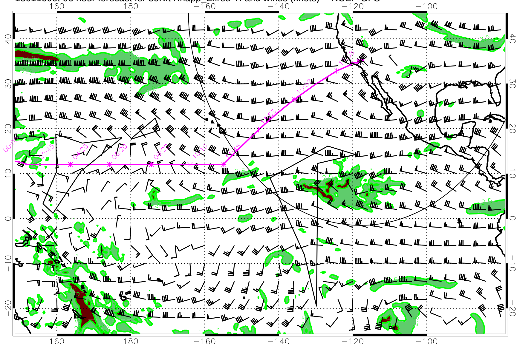
15011000, 96 hour forecast for 39Kft Knapp_Ellrod TI and winds (knots) -- NCEP GFS
