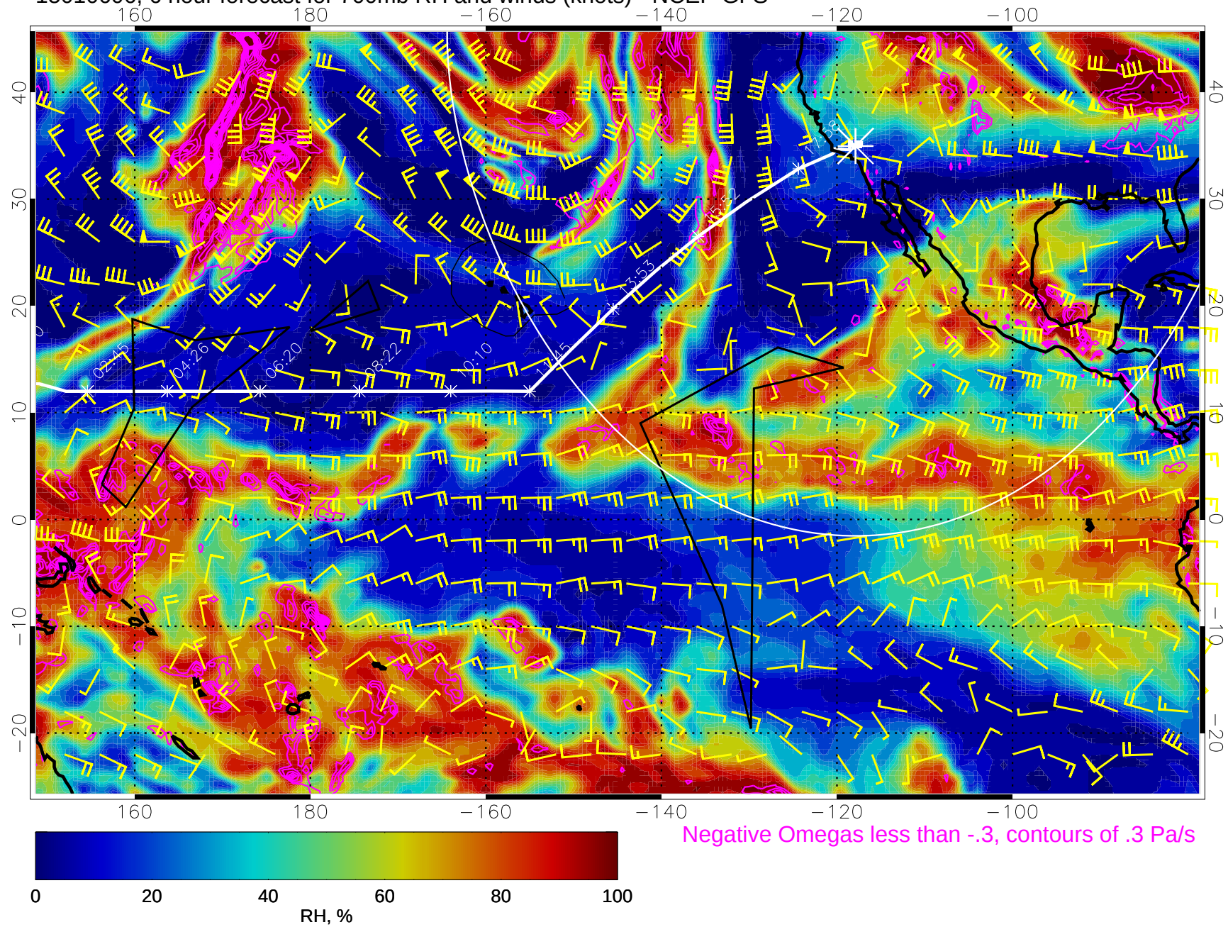
15010606, 6 hour forecast for 700mb RH and winds (knots) - NCEP GFS
