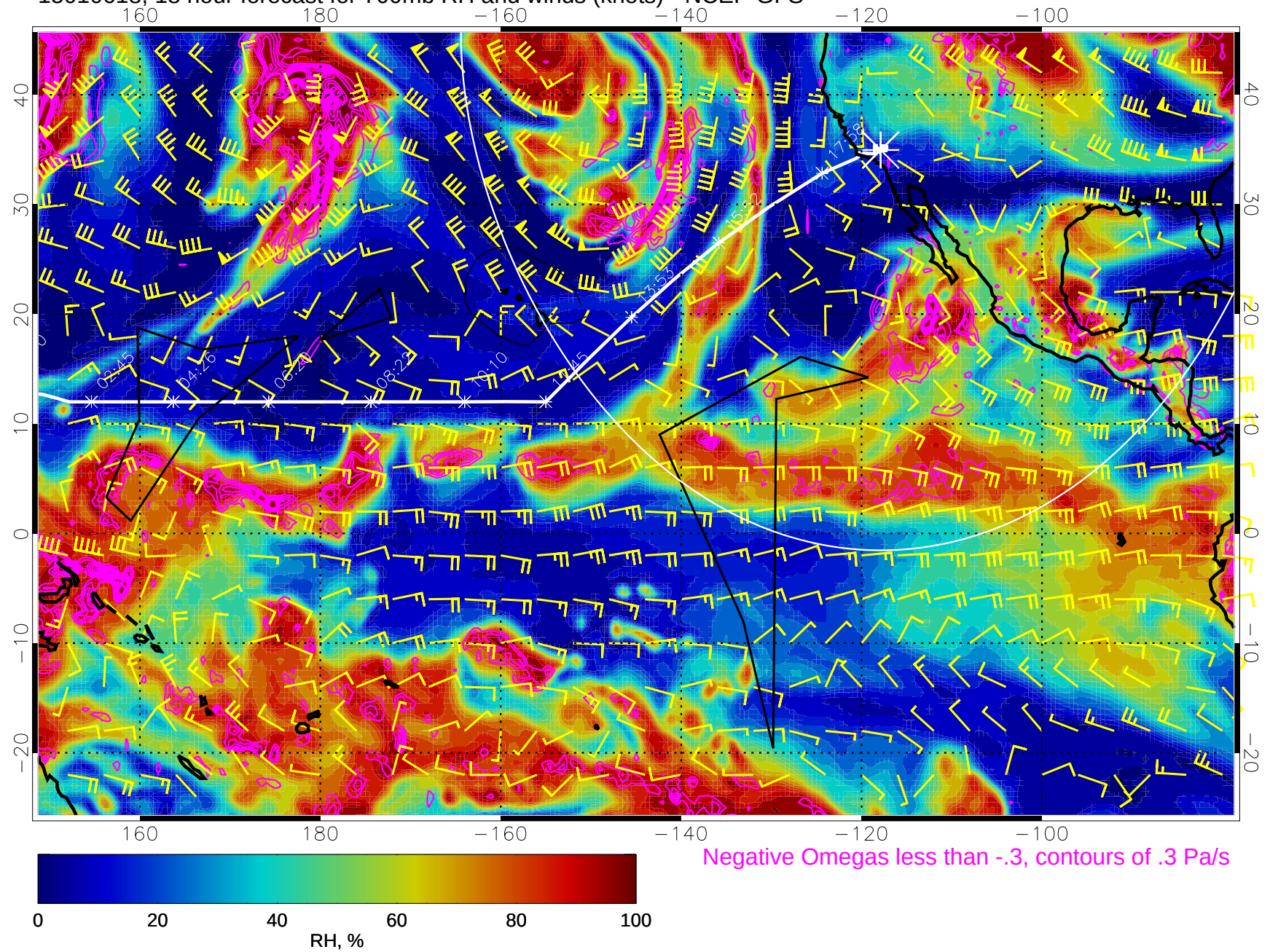
15010618, 18 hour forecast for 700mb RH and winds (knots) - NCEP GFS
