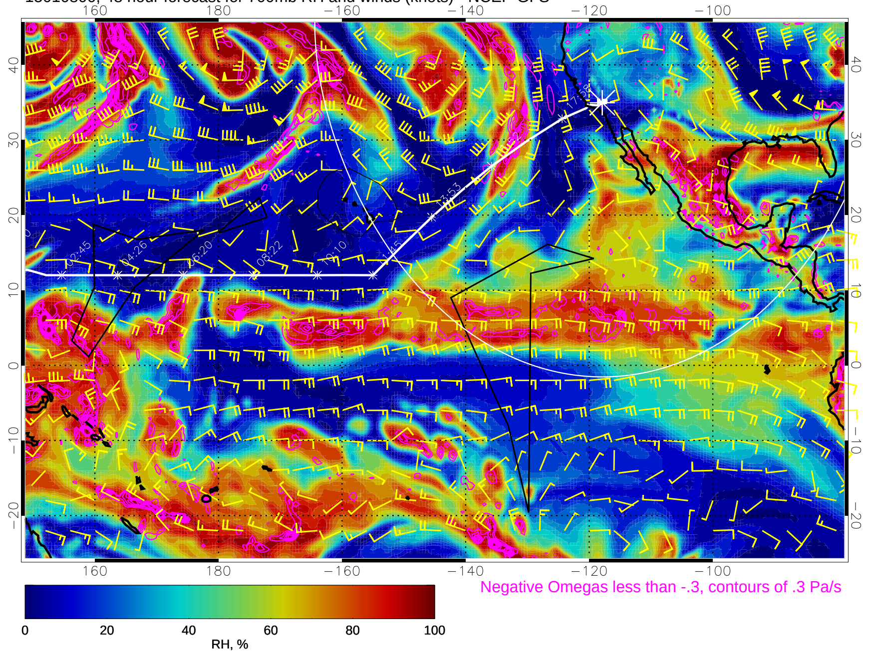
15010800, 48 hour forecast for 700mb RH and winds (knots) - NCEP GFS
