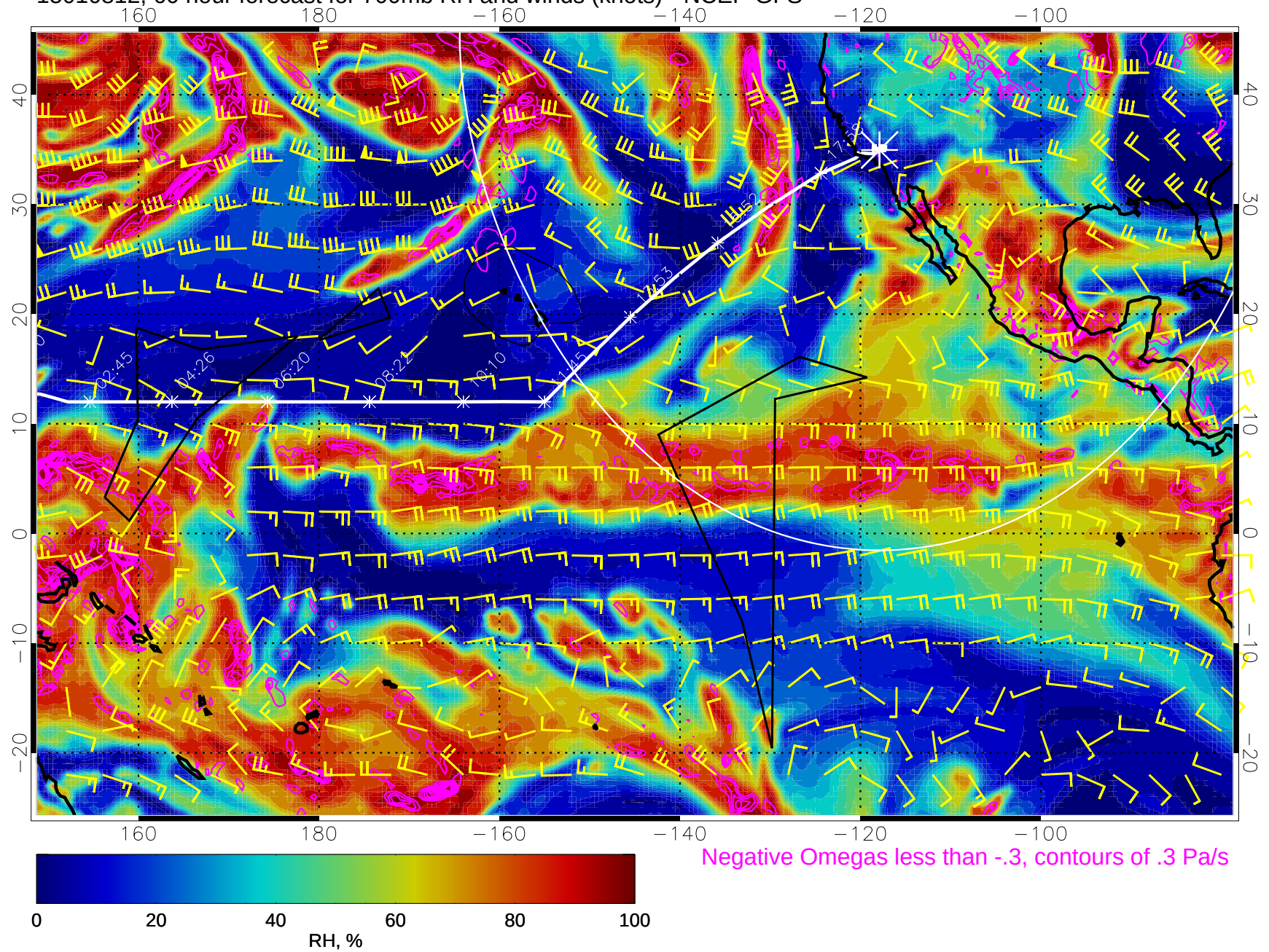
15010812, 60 hour forecast for 700mb RH and winds (knots) - NCEP GFS
