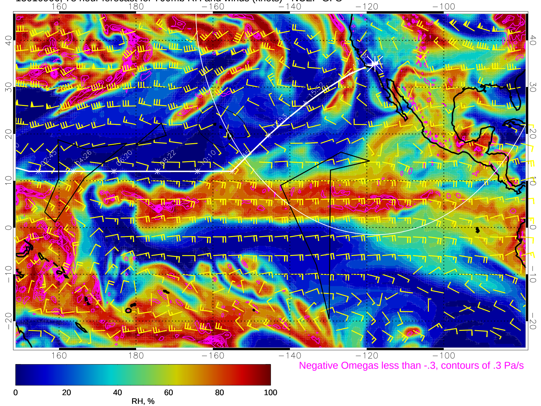
15010906, 78 hour forecast for 700mb RH and winds (knots) - NCEP GFS
