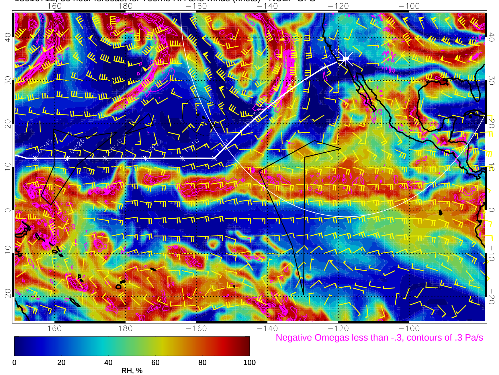
15010712, 36 hour forecast for 700mb RH and winds (knots) - NCEP GFS
