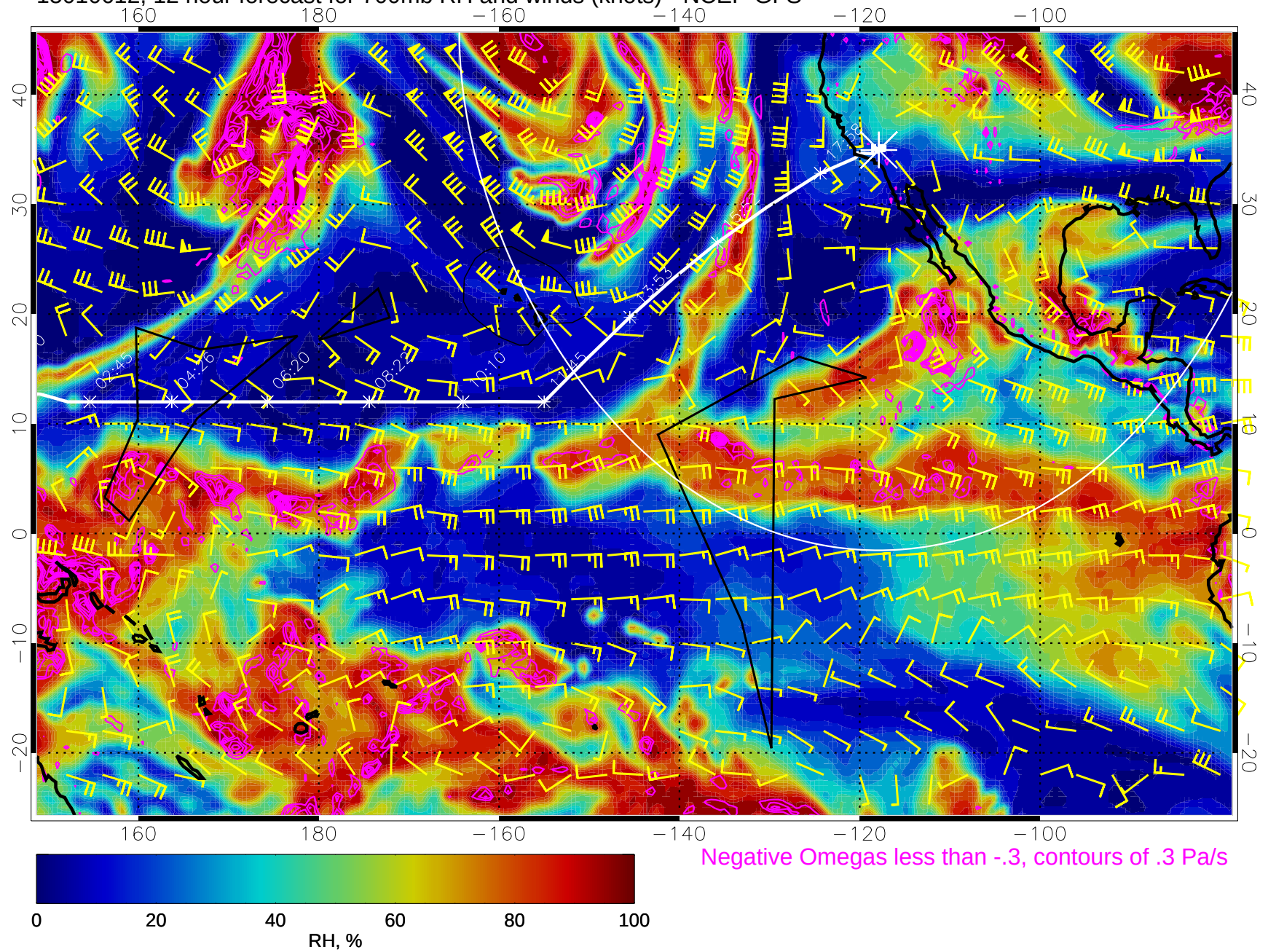
15010612, 12 hour forecast for 700mb RH and winds (knots) - NCEP GFS
