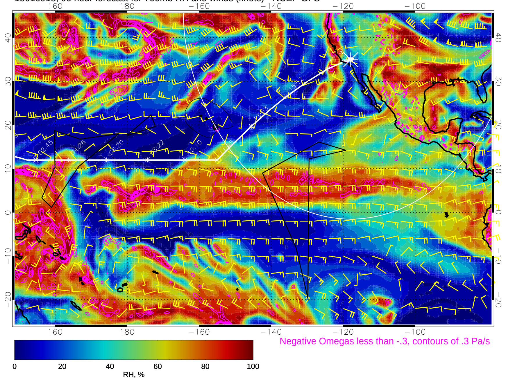
15010918, 90 hour forecast for 700mb RH and winds (knots) - NCEP GFS
