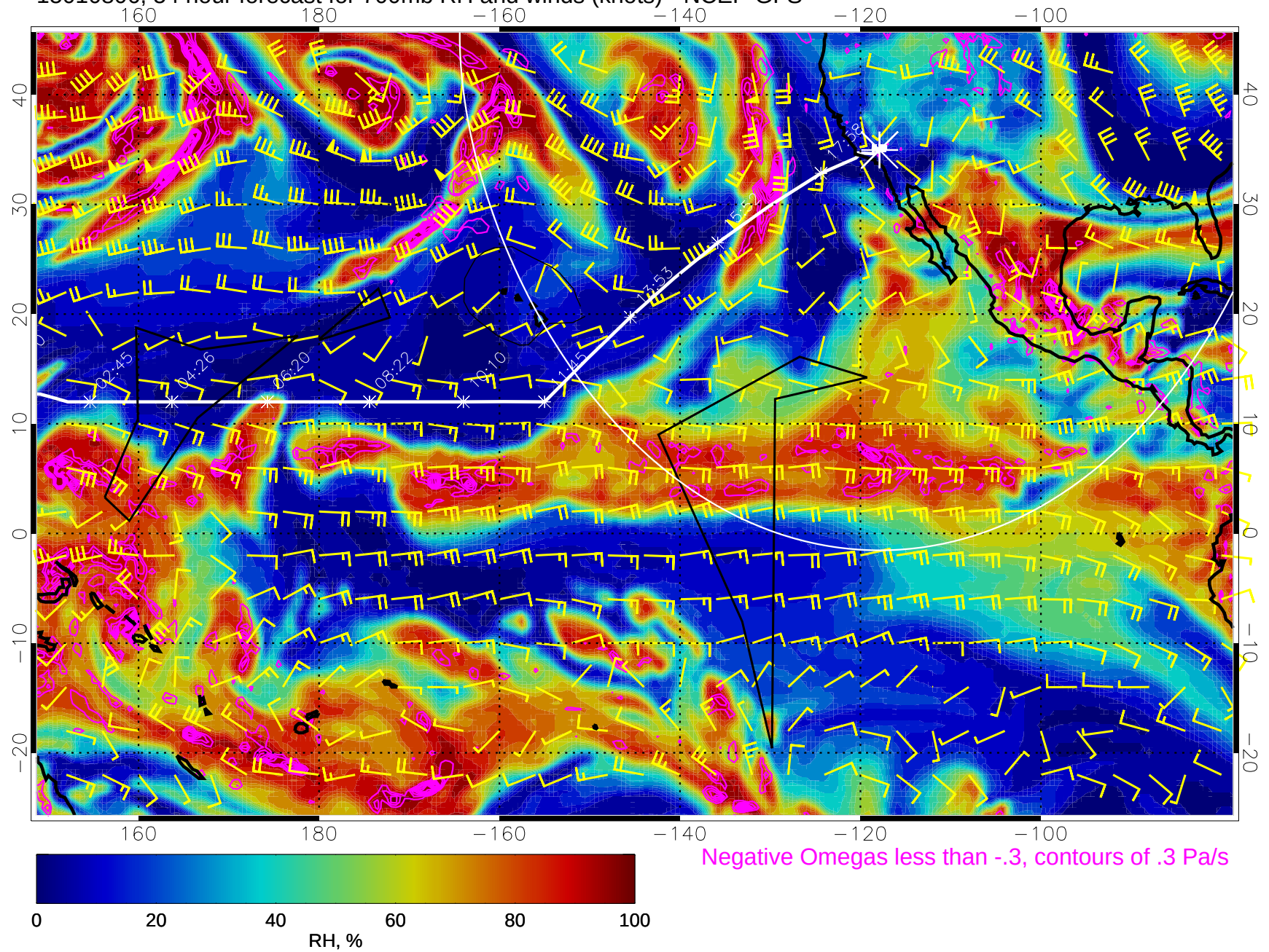
15010806, 54 hour forecast for 700mb RH and winds (knots) - NCEP GFS
