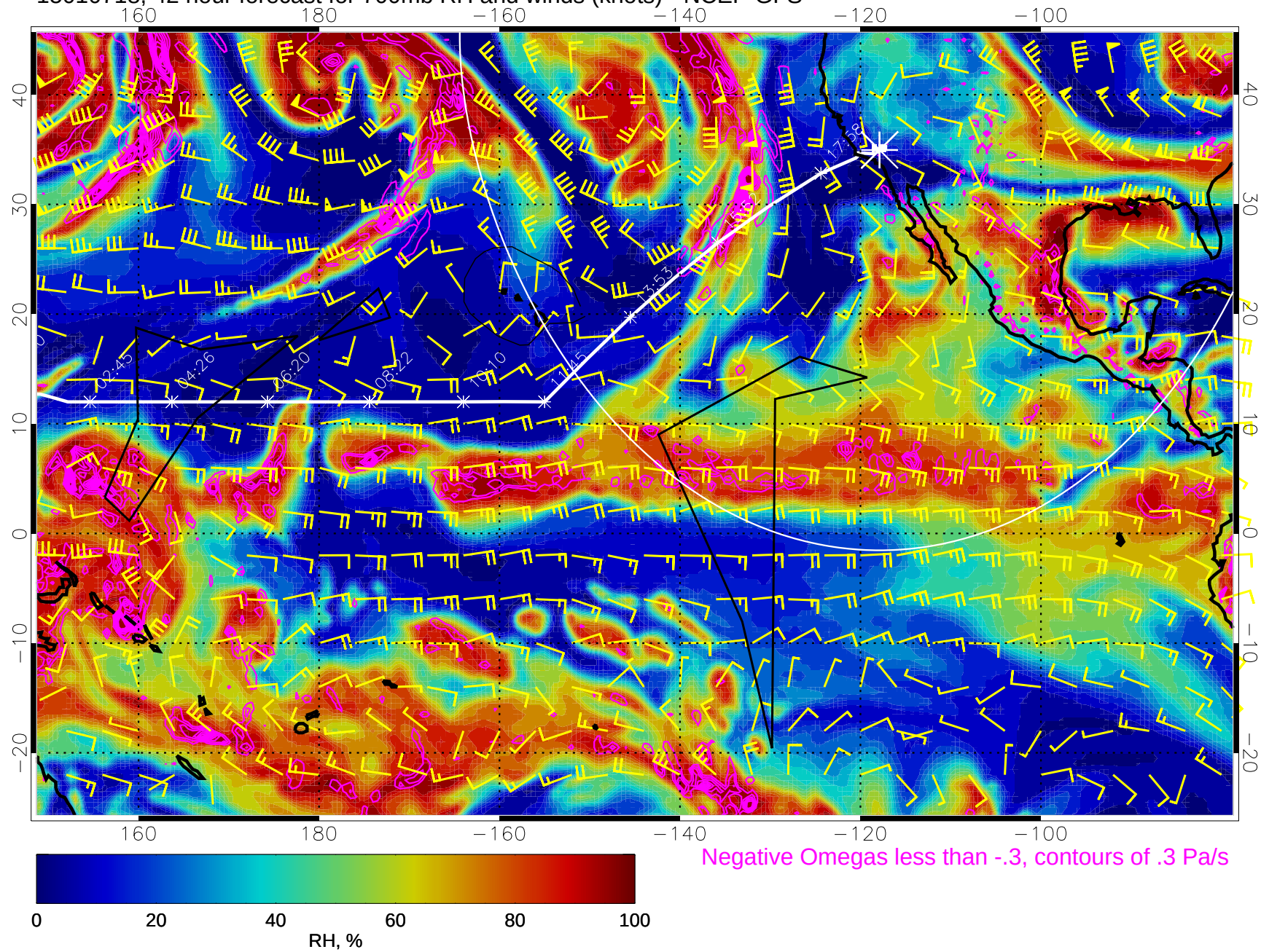
15010718, 42 hour forecast for 700mb RH and winds (knots) - NCEP GFS
