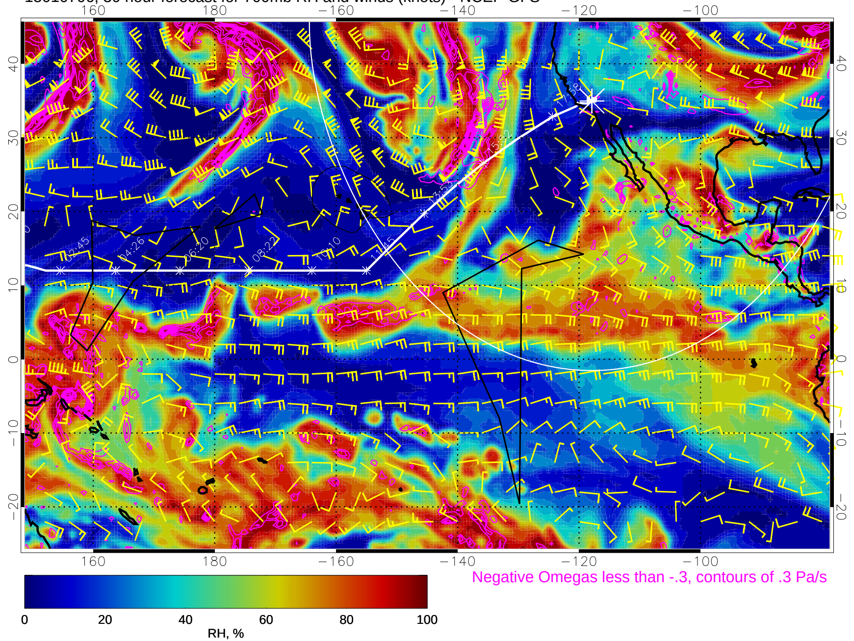
15010706, 30 hour forecast for 700mb RH and winds (knots) - NCEP GFS
