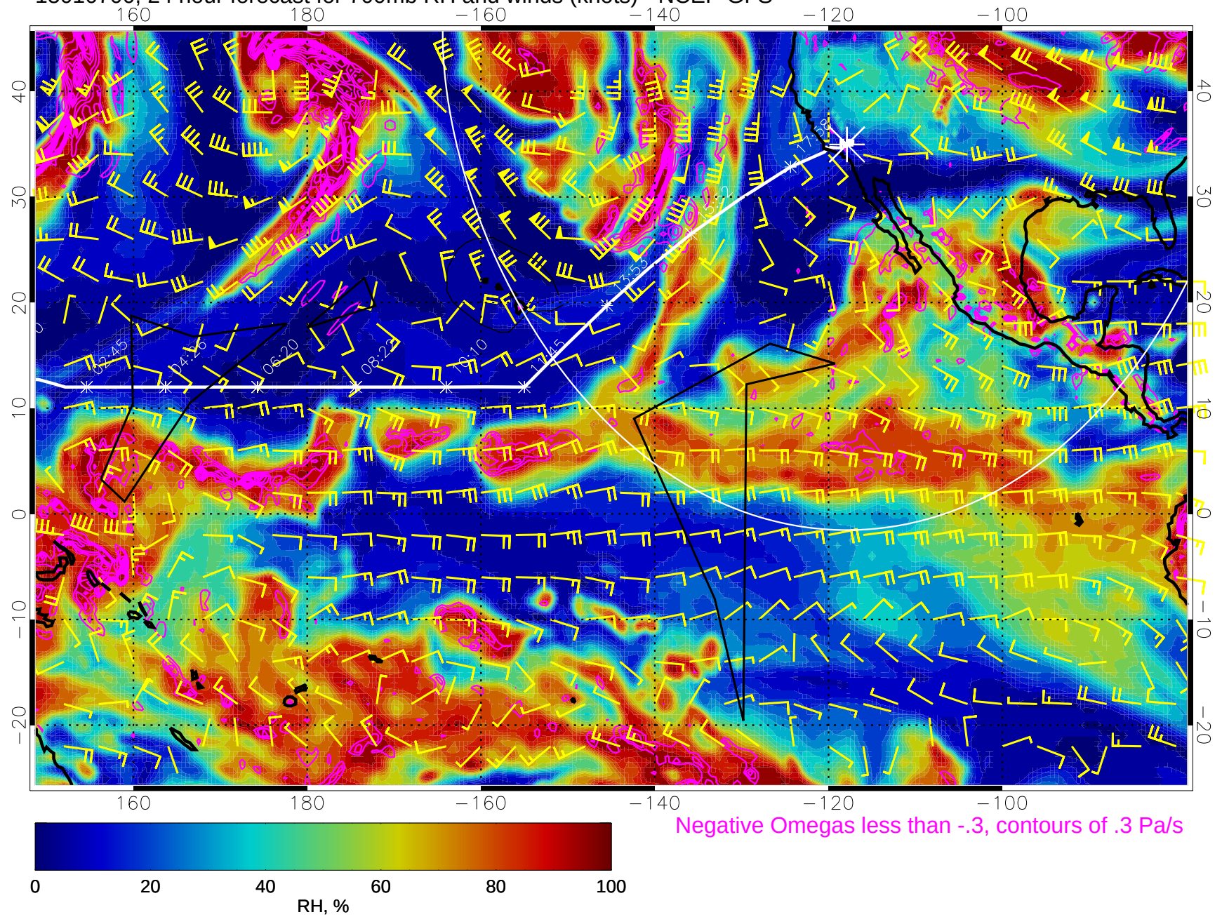
15010700, 24 hour forecast for 700mb RH and winds (knots) - NCEP GFS
