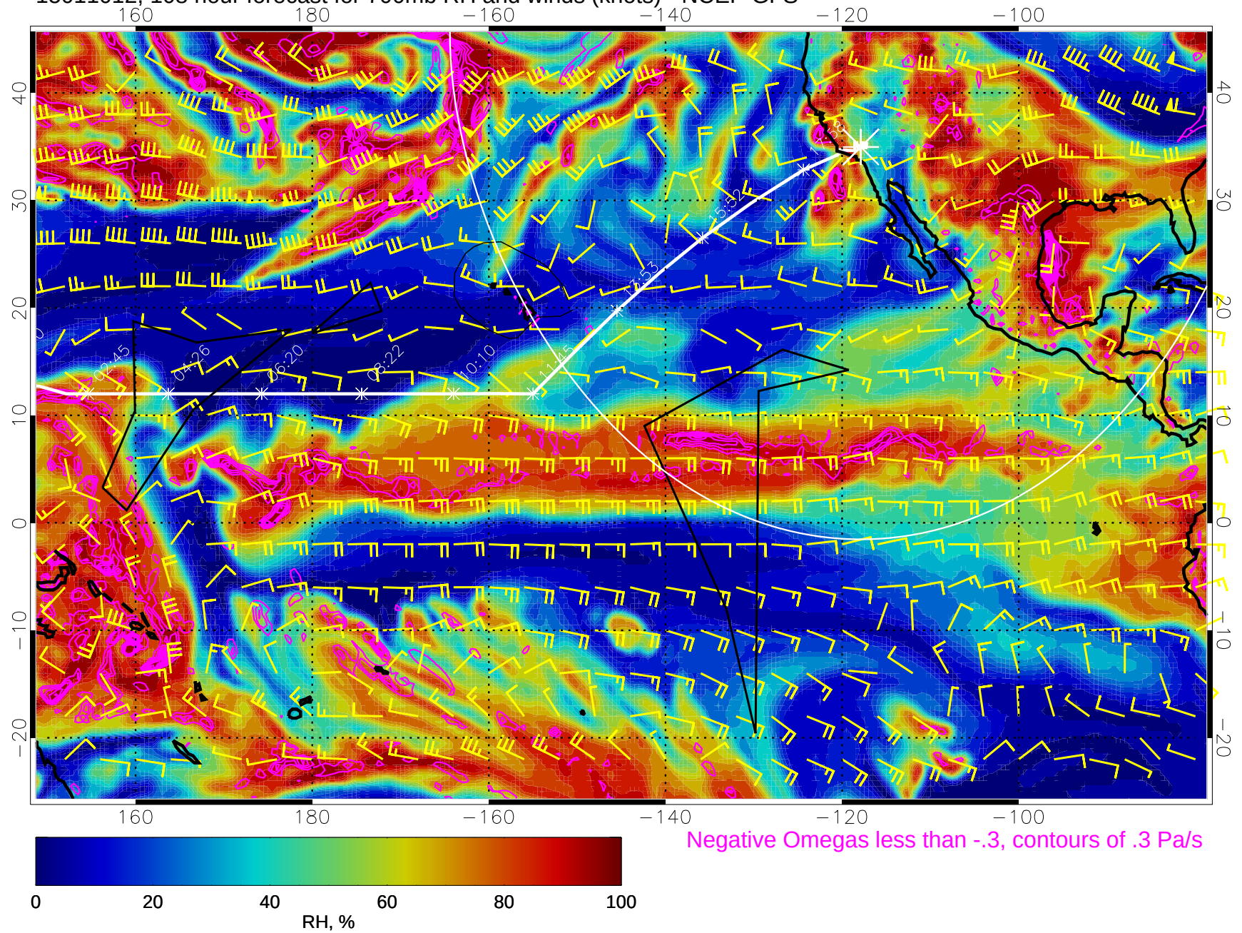
15011012, 108 hour forecast for 700mb RH and winds (knots) - NCEP GFS
