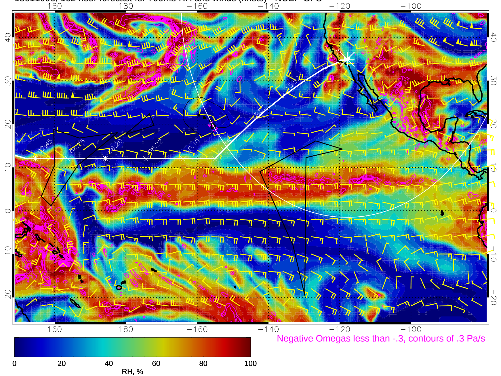
15011006, 102 hour forecast for 700mb RH and winds (knots) - NCEP GFS
