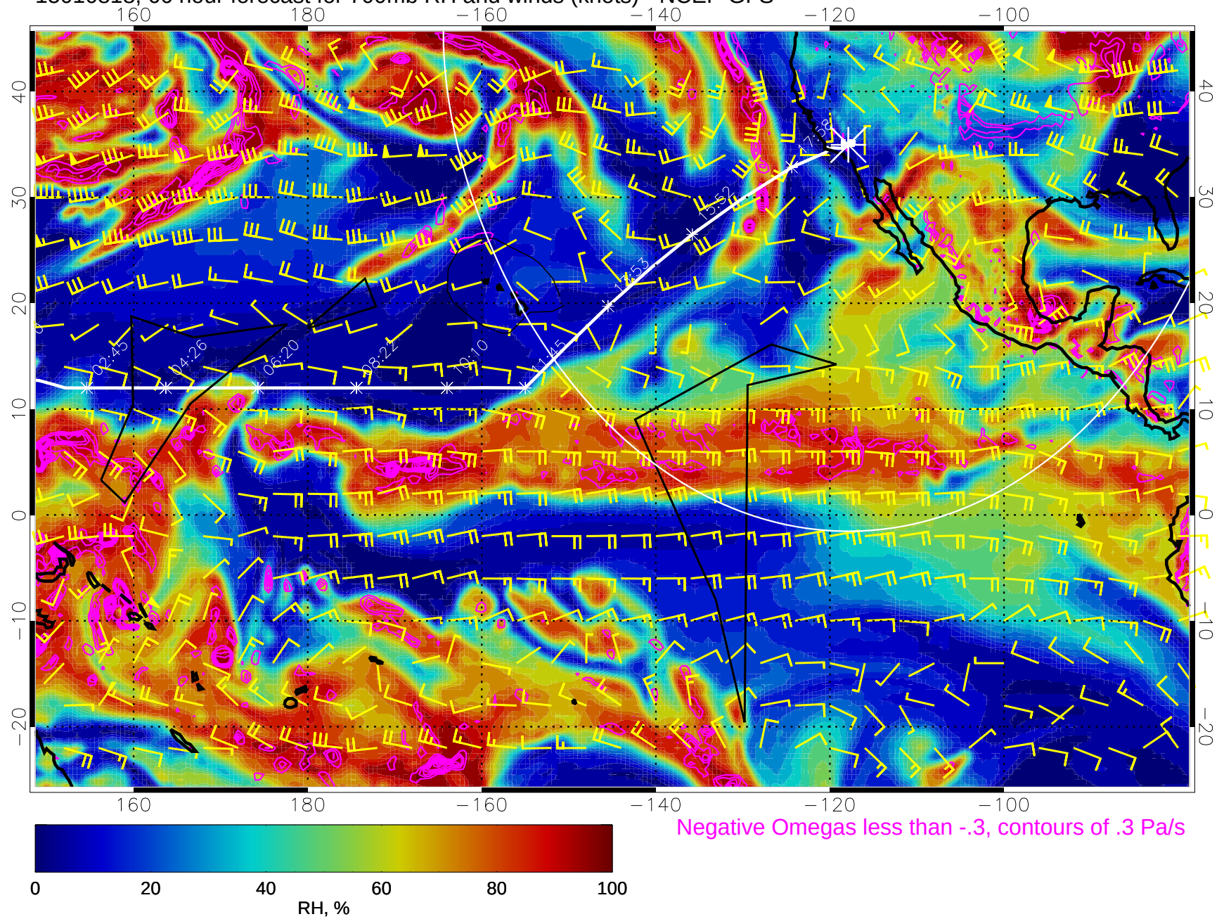
15010818, 66 hour forecast for 700mb RH and winds (knots) - NCEP GFS
