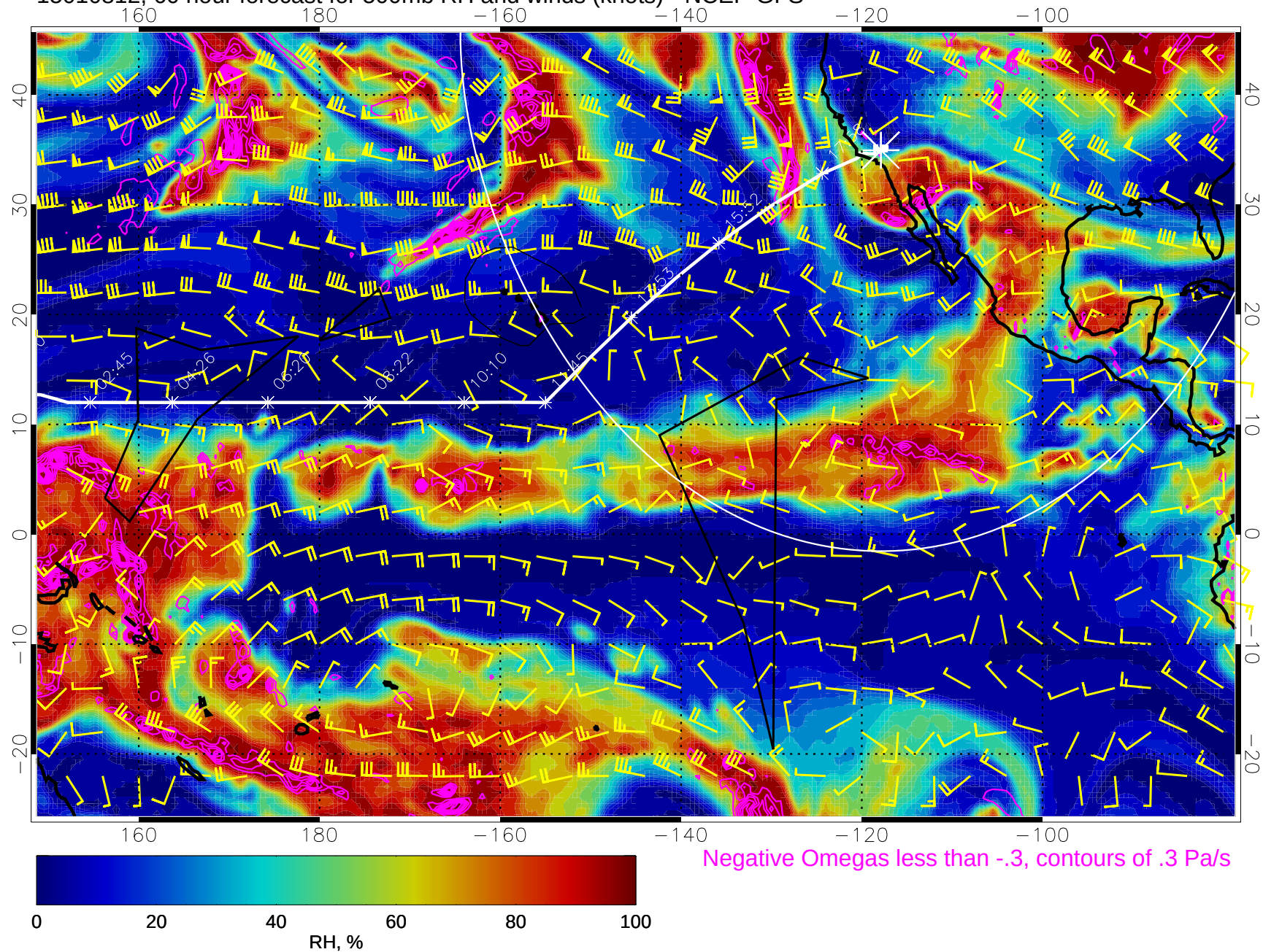
15010812, 60 hour forecast for 500mb RH and winds (knots) - NCEP GFS
