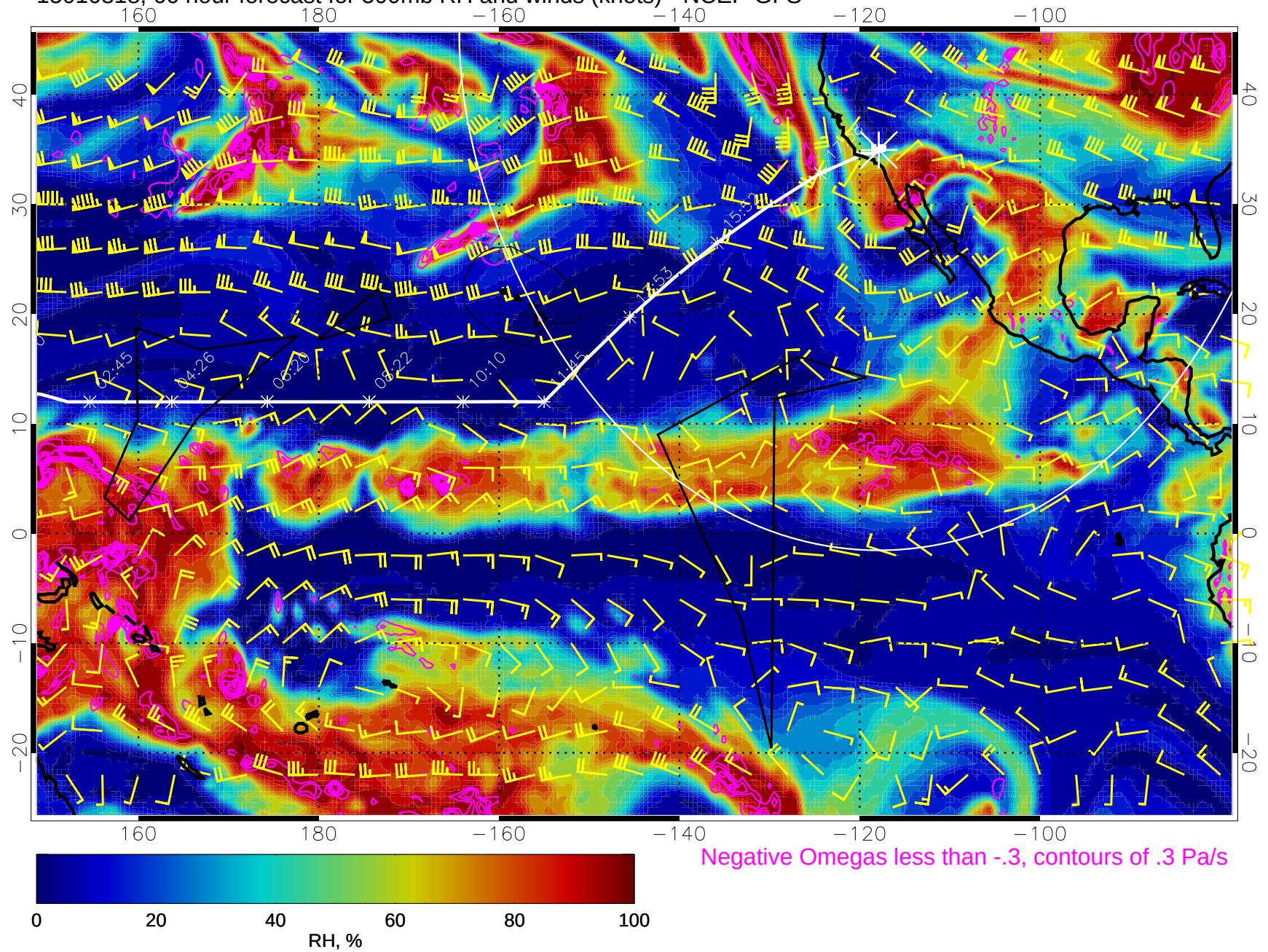
15010818, 66 hour forecast for 500mb RH and winds (knots) - NCEP GFS
