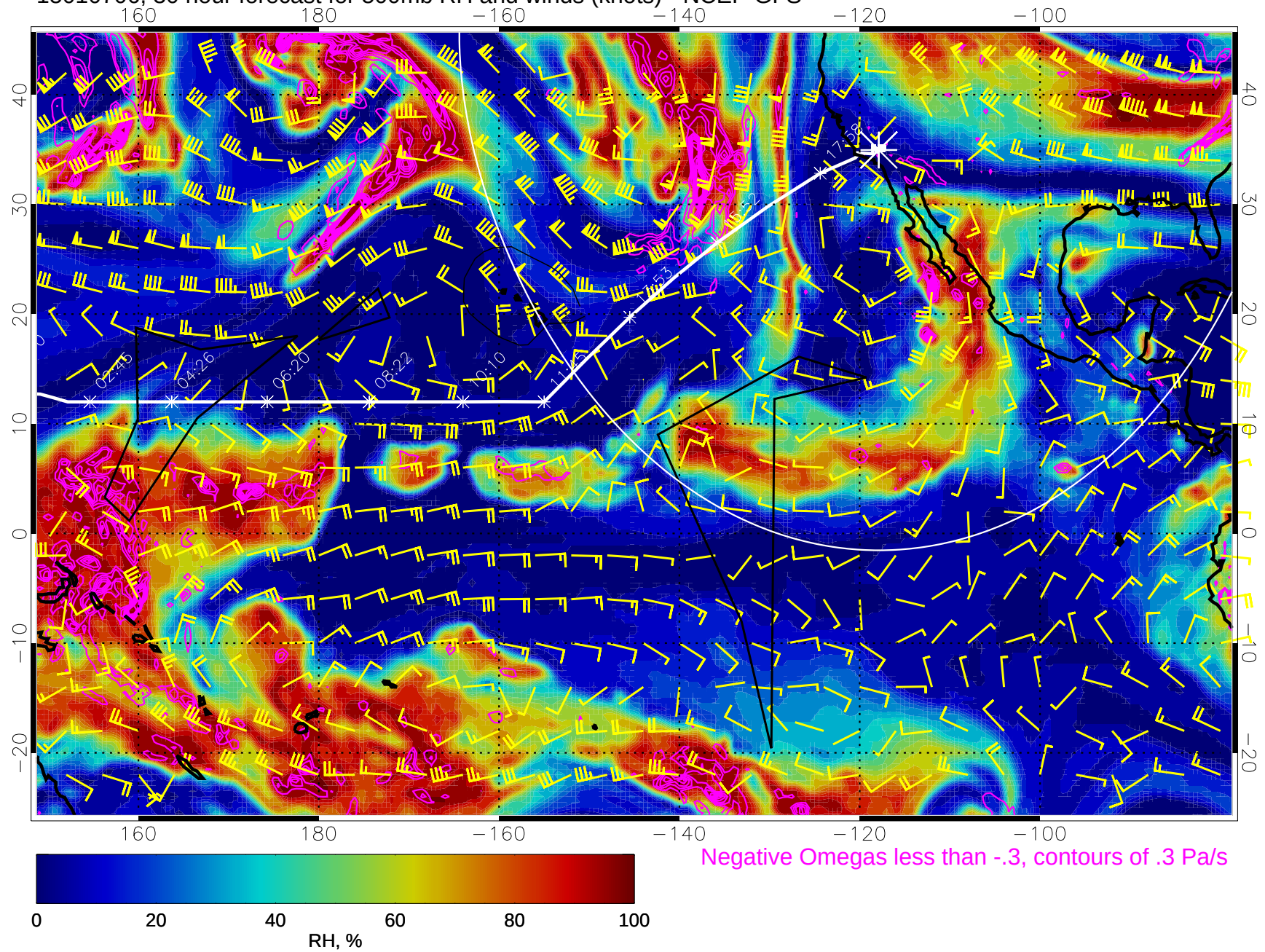
15010706, 30 hour forecast for 500mb RH and winds (knots) - NCEP GFS
