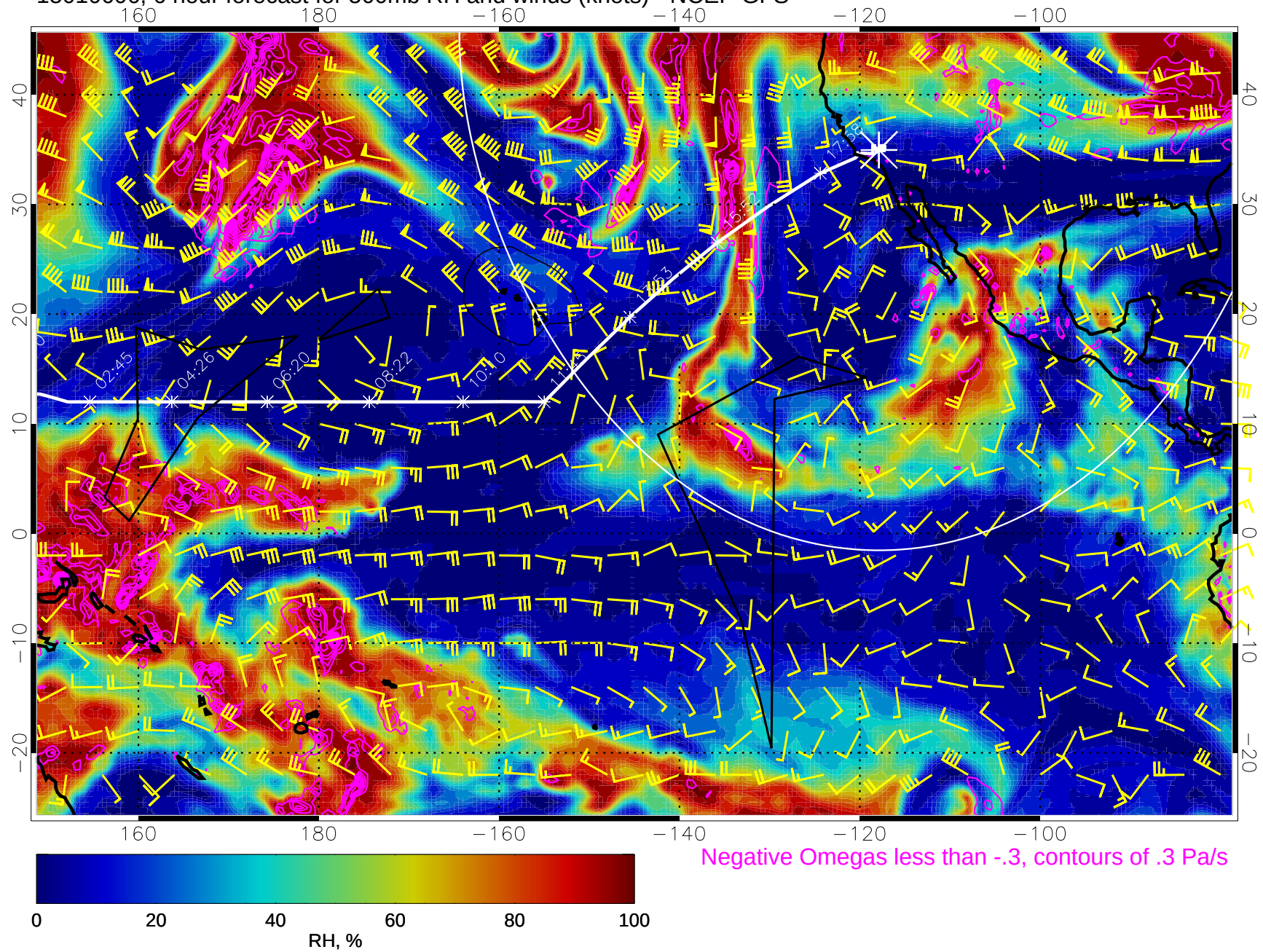
15010606, 6 hour forecast for 500mb RH and winds (knots) - NCEP GFS
