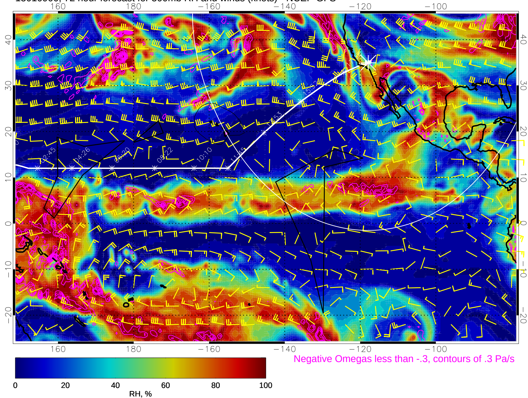
15010900, 72 hour forecast for 500mb RH and winds (knots) - NCEP GFS
