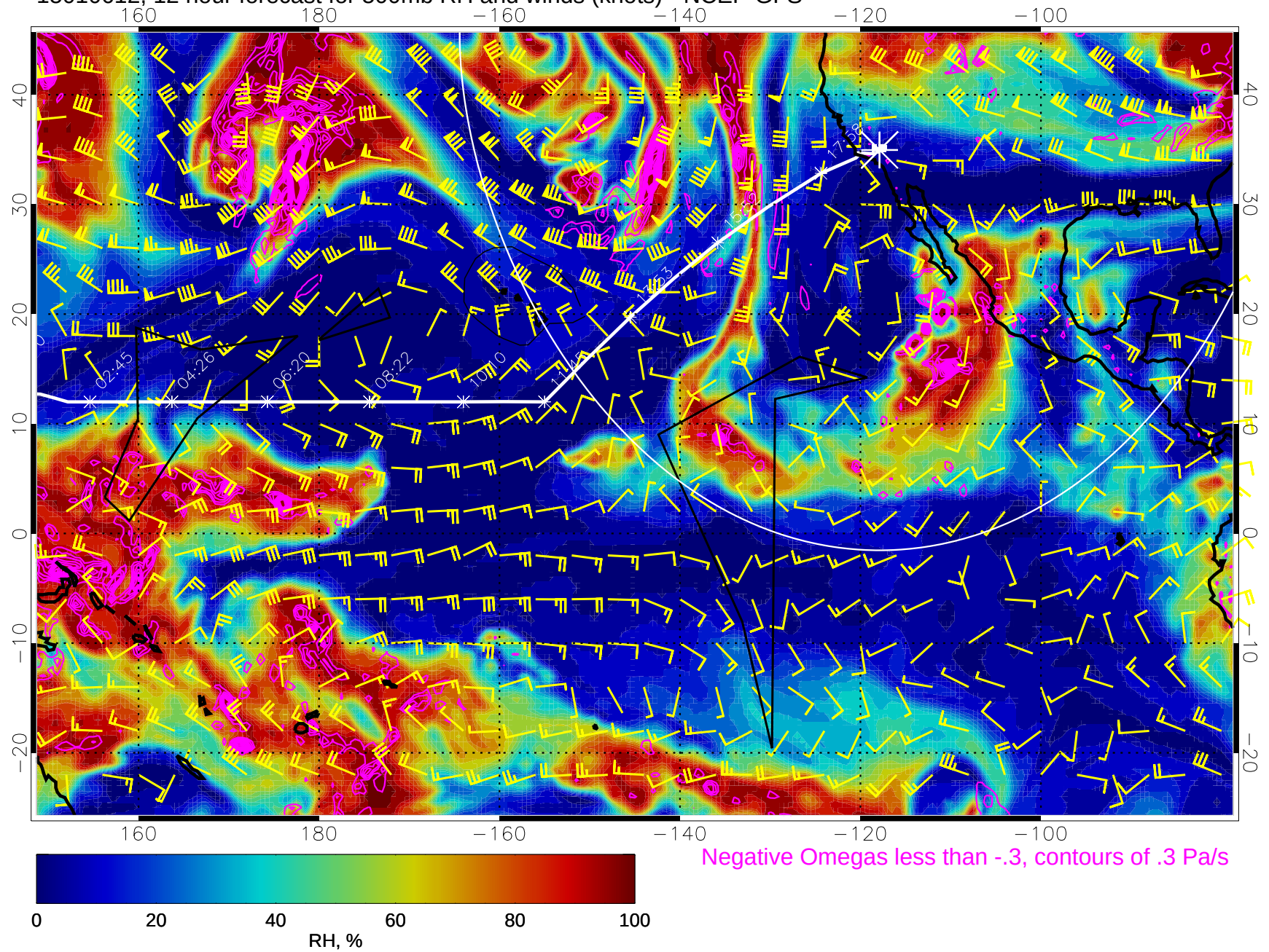
15010612, 12 hour forecast for 500mb RH and winds (knots) - NCEP GFS
