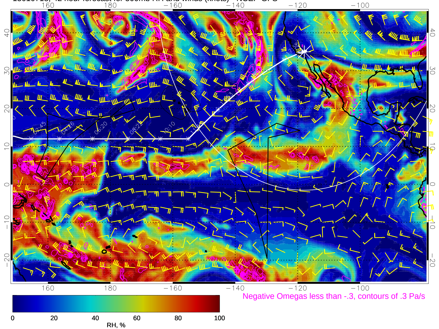
15010718, 42 hour forecast for 500mb RH and winds (knots) - NCEP GFS
