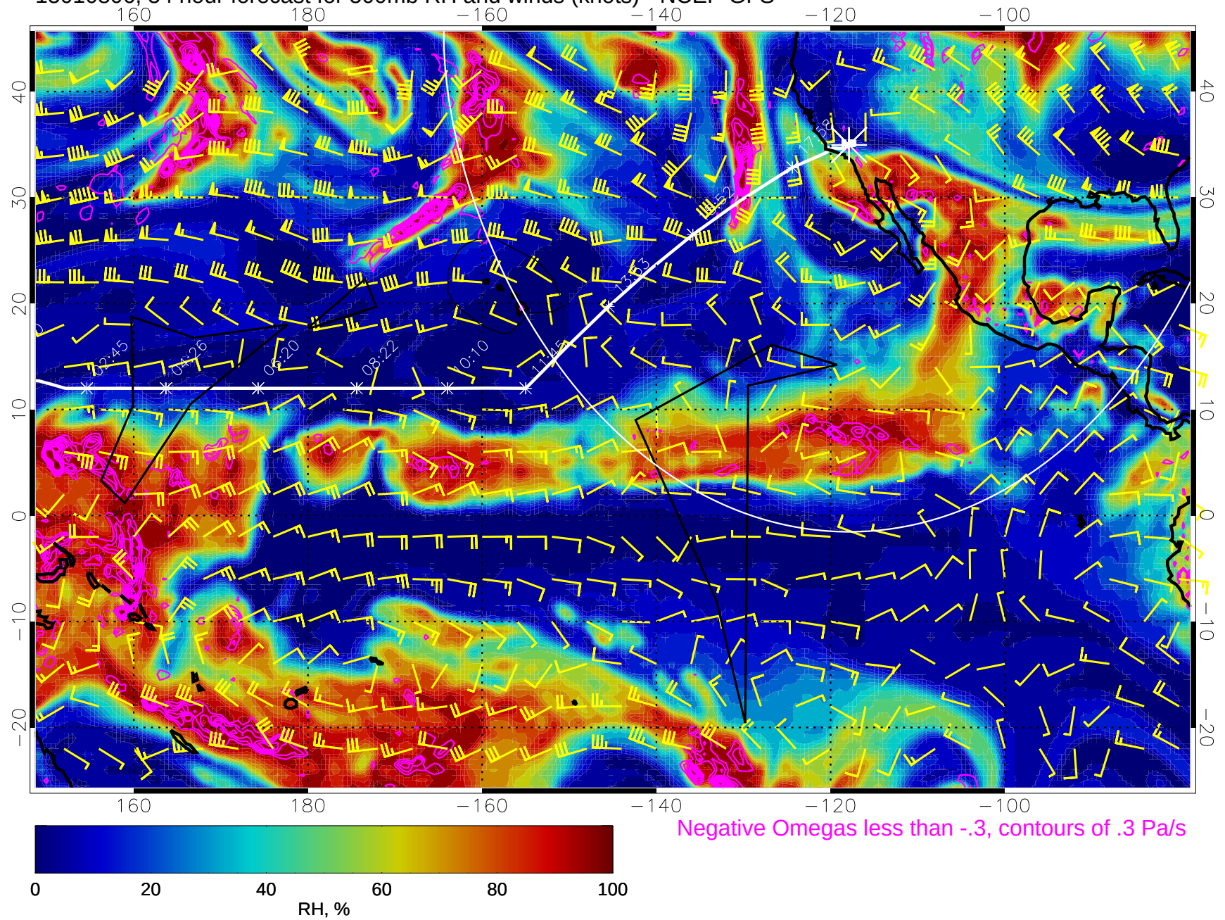
15010806, 54 hour forecast for 500mb RH and winds (knots) - NCEP GFS
