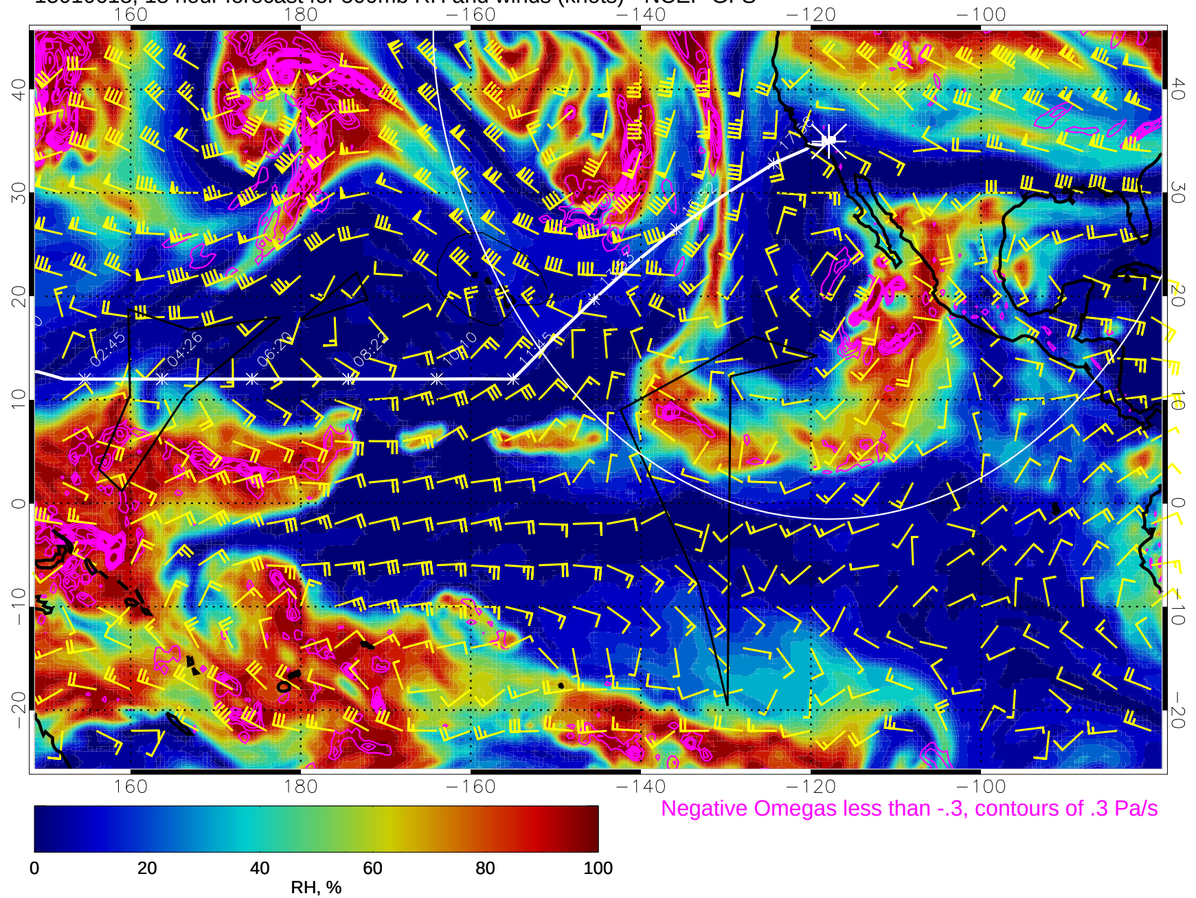
15010618, 18 hour forecast for 500mb RH and winds (knots) - NCEP GFS
