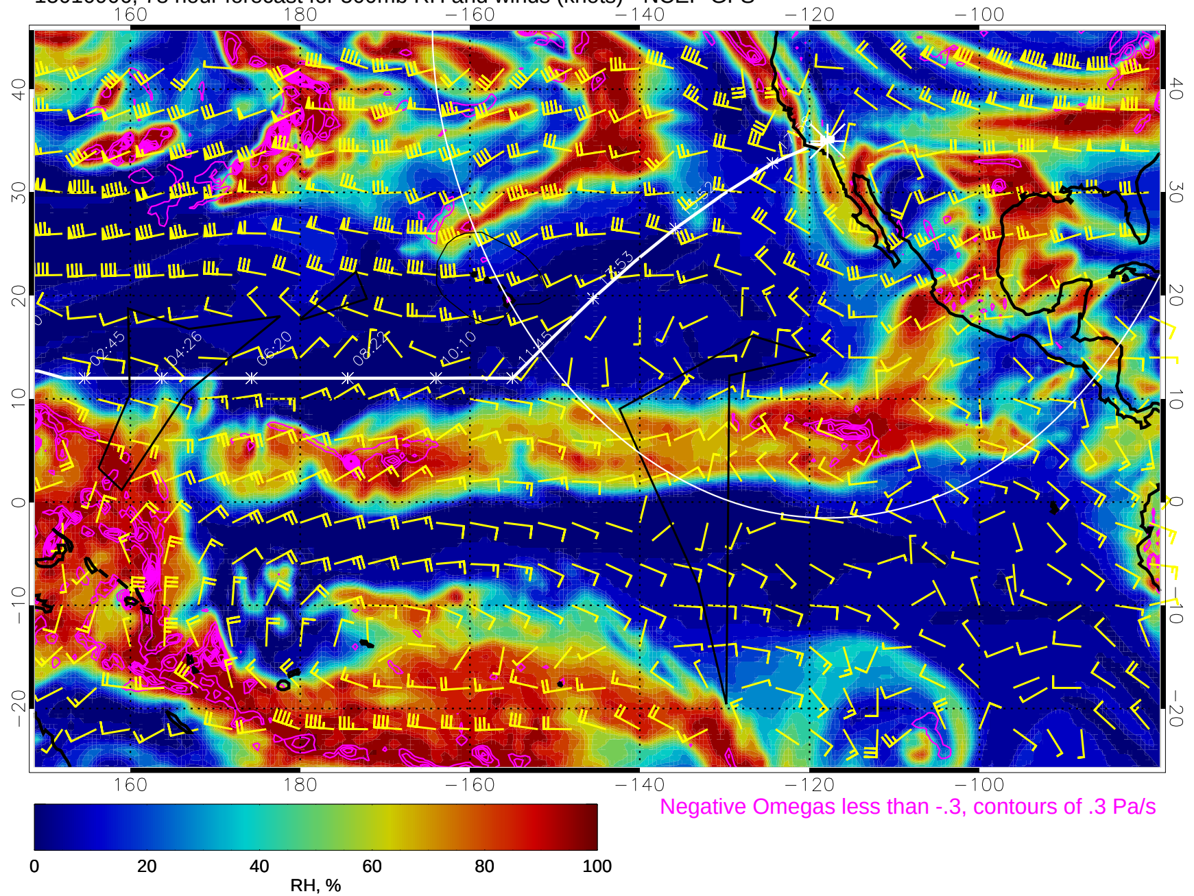
15010906, 78 hour forecast for 500mb RH and winds (knots) - NCEP GFS
