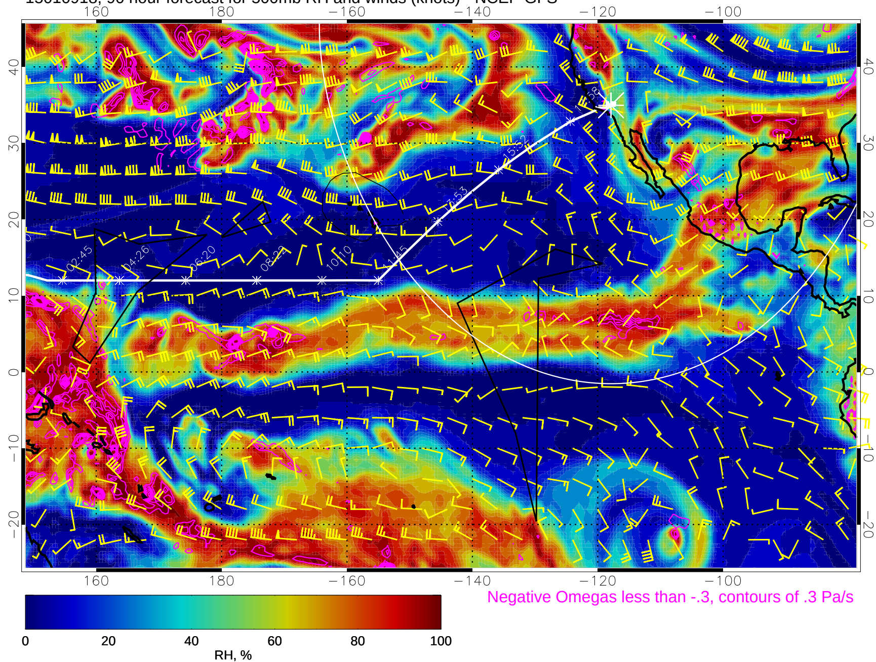
15010918, 90 hour forecast for 500mb RH and winds (knots) - NCEP GFS
