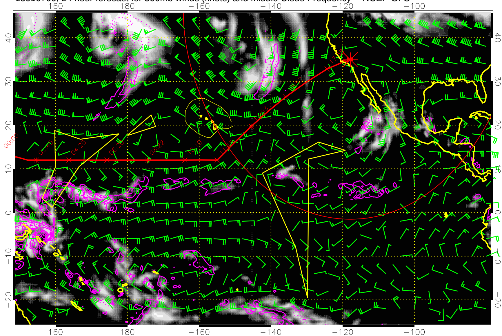
15010700, 24 hour forecast for 500mb winds (knots) and Middle Cloud Frequency -- NCEP GFS
