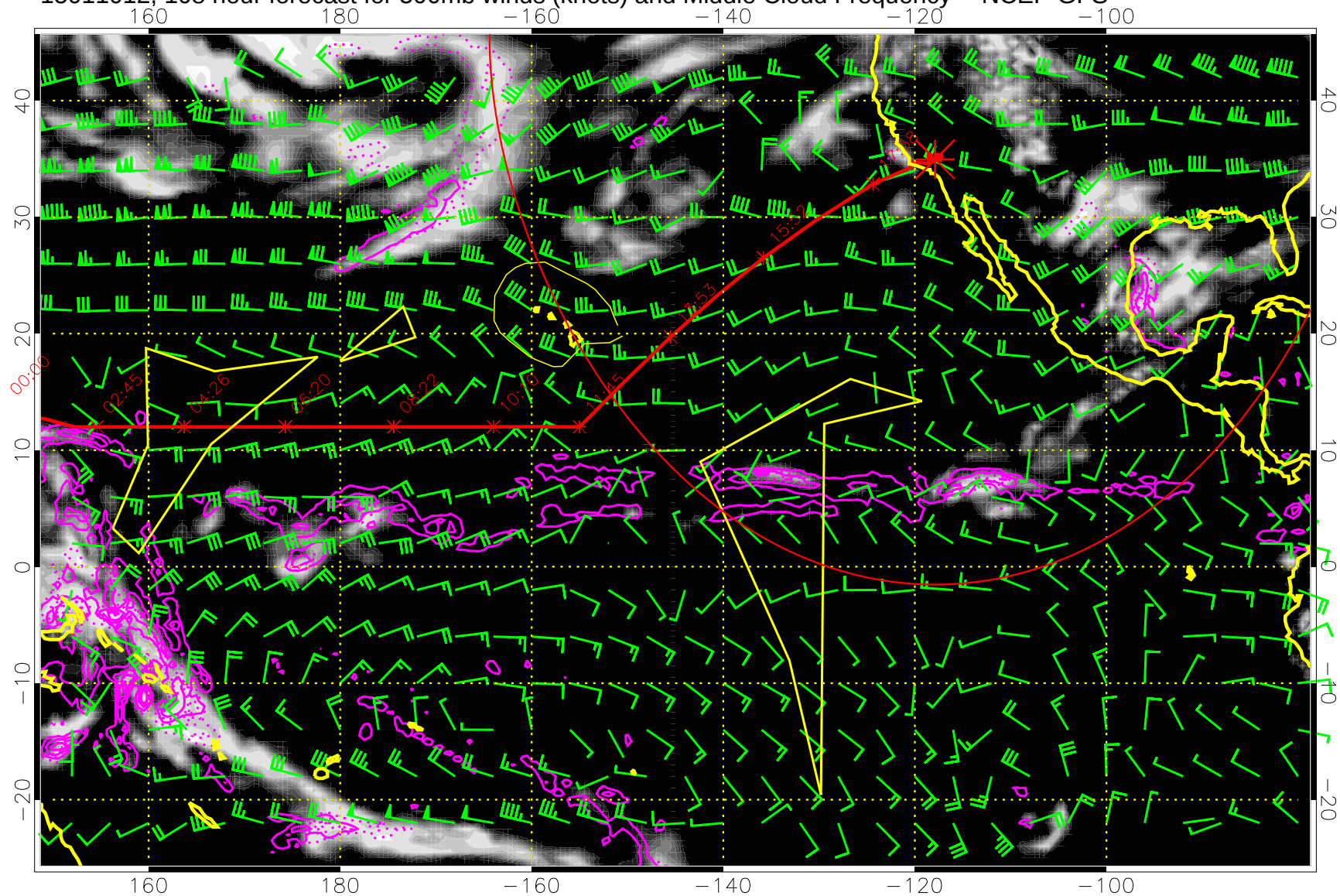
15011012, 108 hour forecast for 500mb winds (knots) and Middle Cloud Frequency -- NCEP GFS
