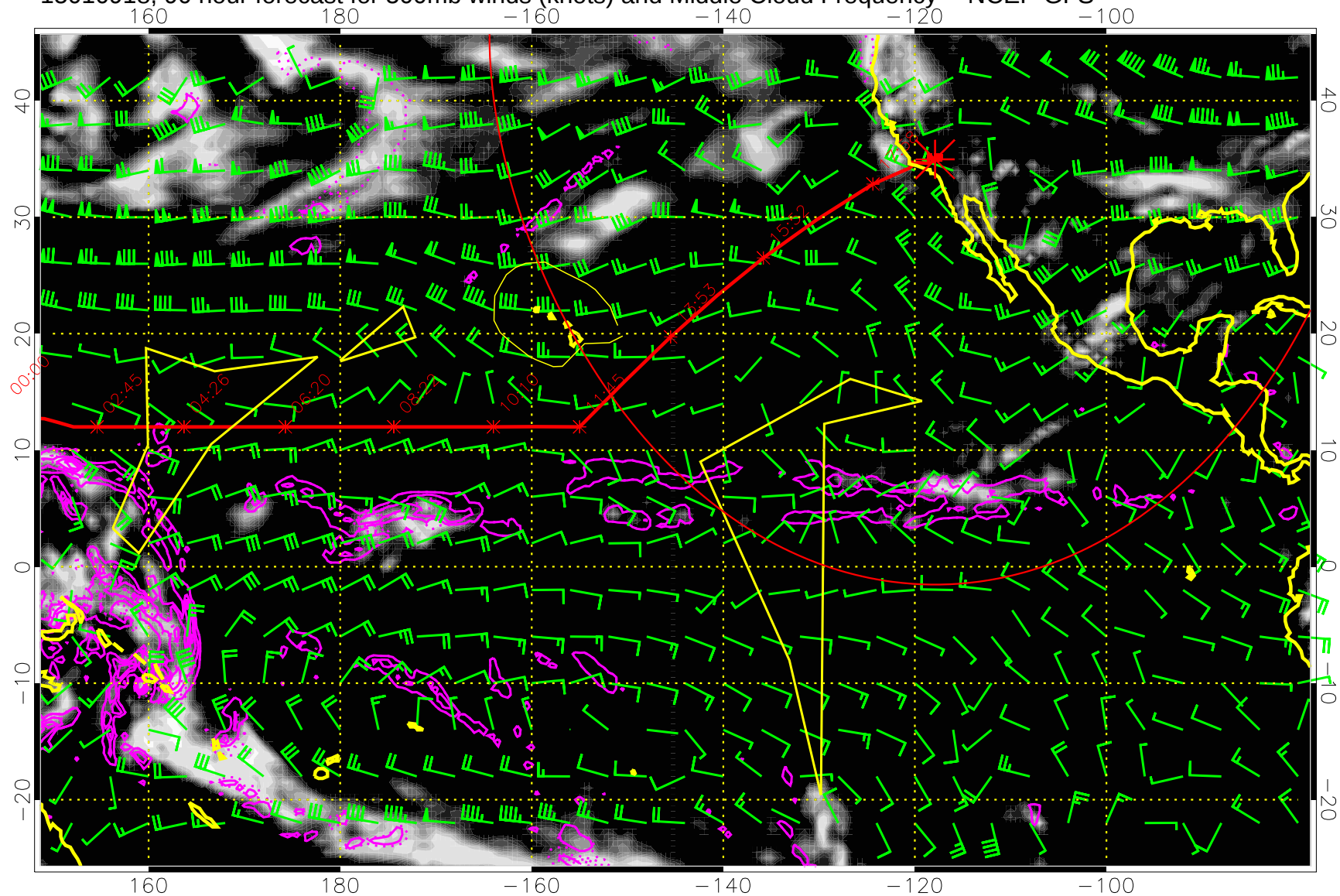
15010918, 90 hour forecast for 500mb winds (knots) and Middle Cloud Frequency -- NCEP GFS
