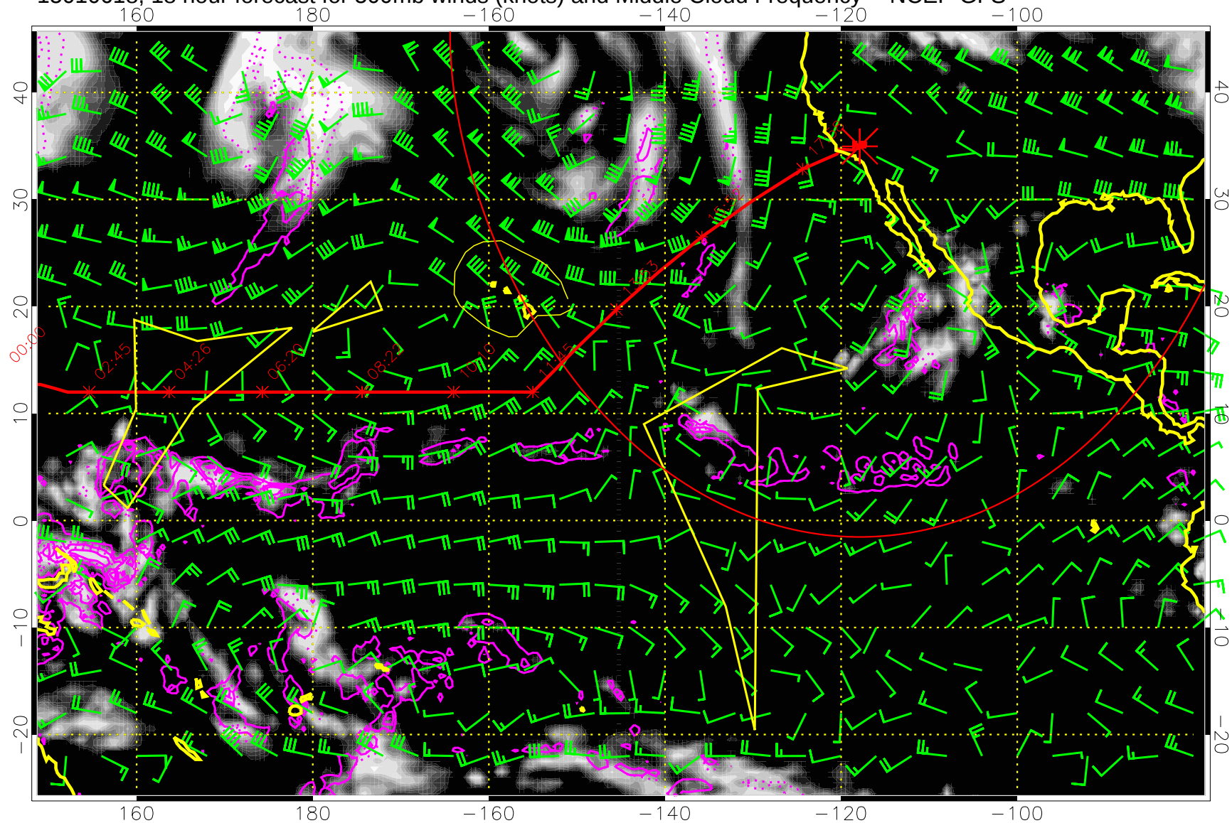
15010618, 18 hour forecast for 500mb winds (knots) and Middle Cloud Frequency -- NCEP GFS
