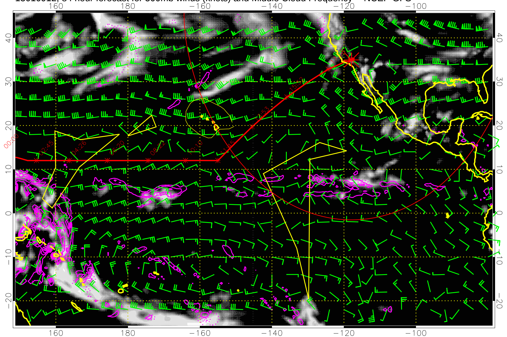
15010912, 84 hour forecast for 500mb winds (knots) and Middle Cloud Frequency -- NCEP GFS
