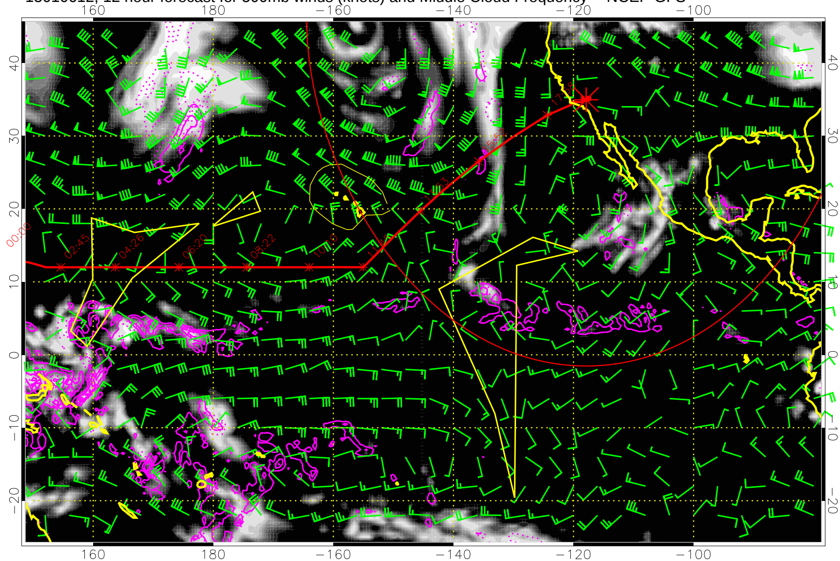
15010612, 12 hour forecast for 500mb winds (knots) and Middle Cloud Frequency -- NCEP GFS
