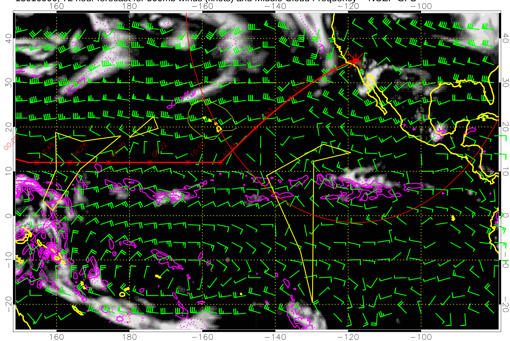
15010900, 72 hour forecast for 500mb winds (knots) and Middle Cloud Frequency -- NCEP GFS
