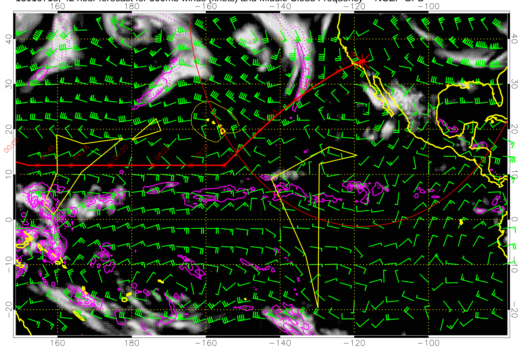
15010718, 42 hour forecast for 500mb winds (knots) and Middle Cloud Frequency -- NCEP GFS
