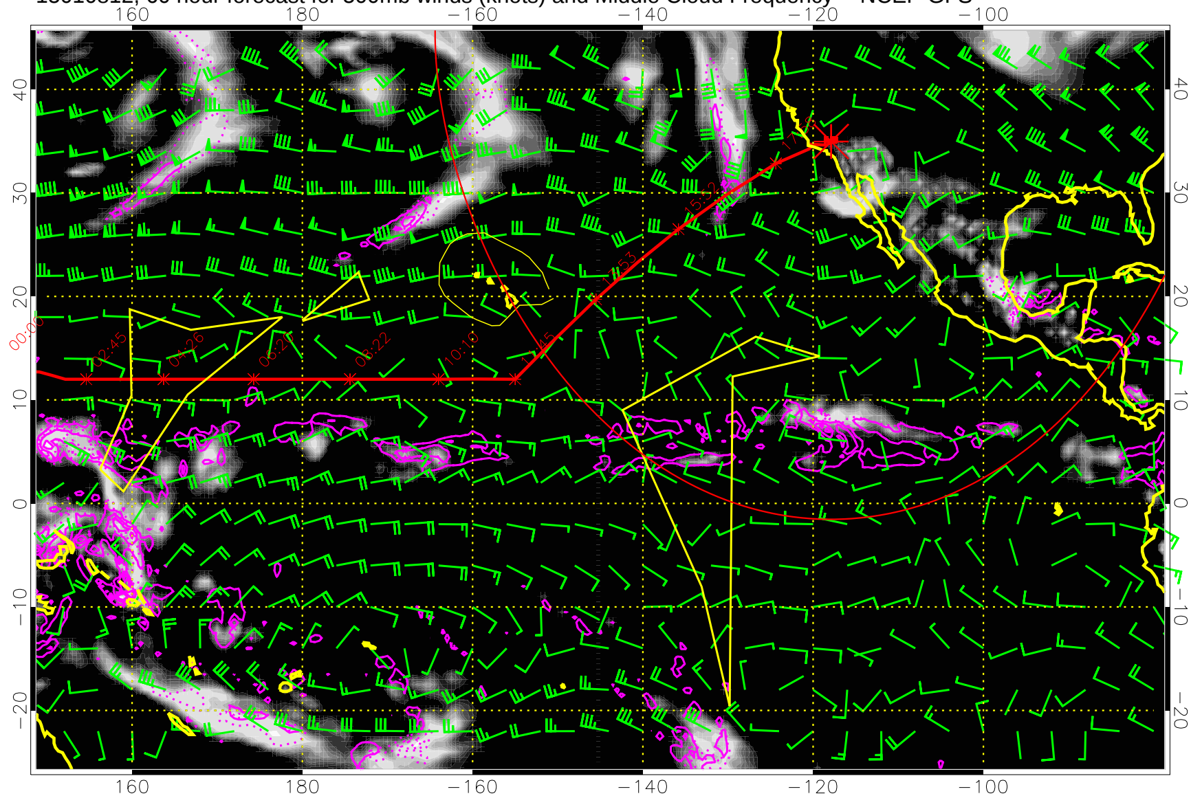
15010812, 60 hour forecast for 500mb winds (knots) and Middle Cloud Frequency -- NCEP GFS
