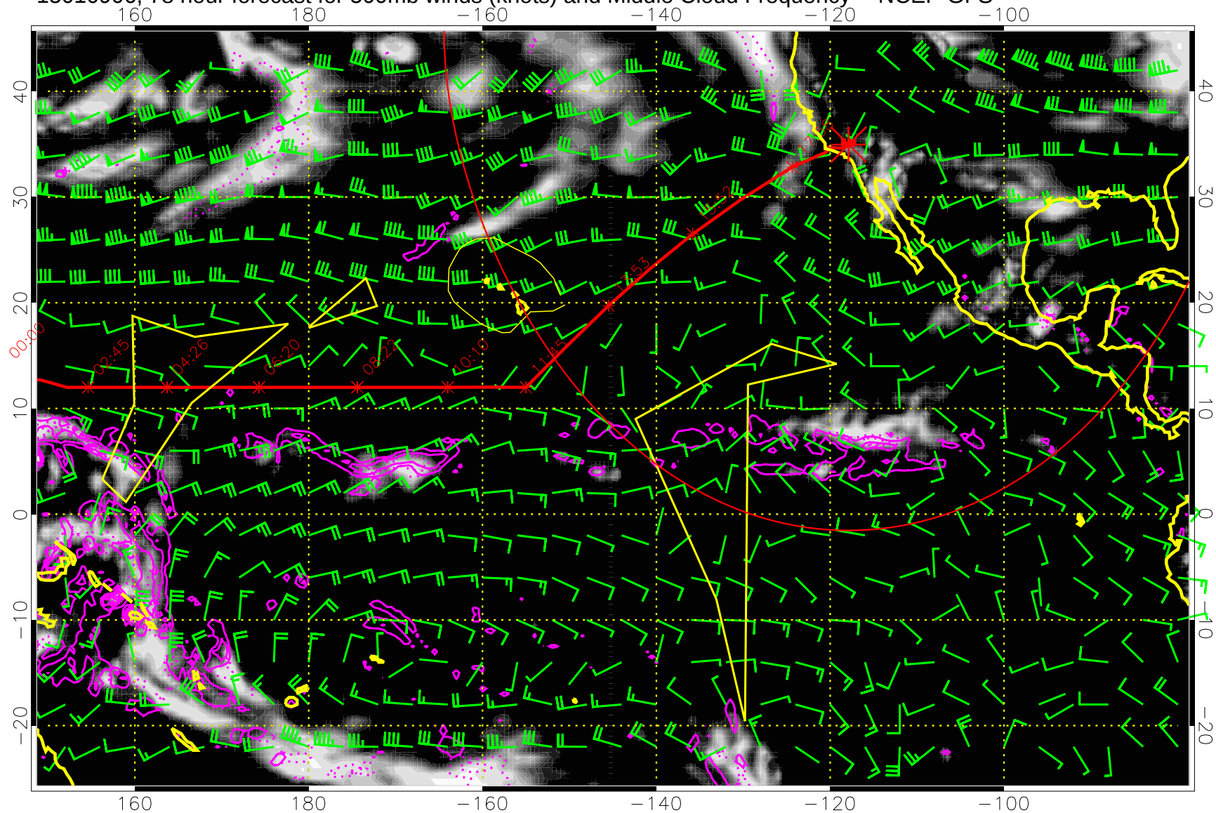
15010906, 78 hour forecast for 500mb winds (knots) and Middle Cloud Frequency -- NCEP GFS
