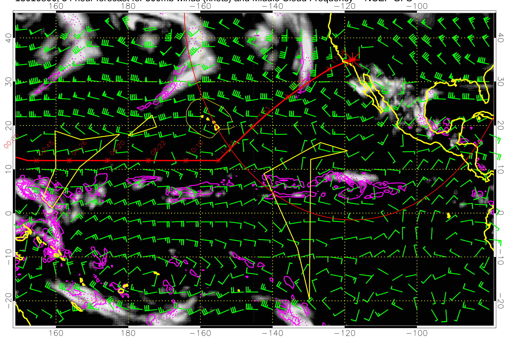
15010806, 54 hour forecast for 500mb winds (knots) and Middle Cloud Frequency -- NCEP GFS
