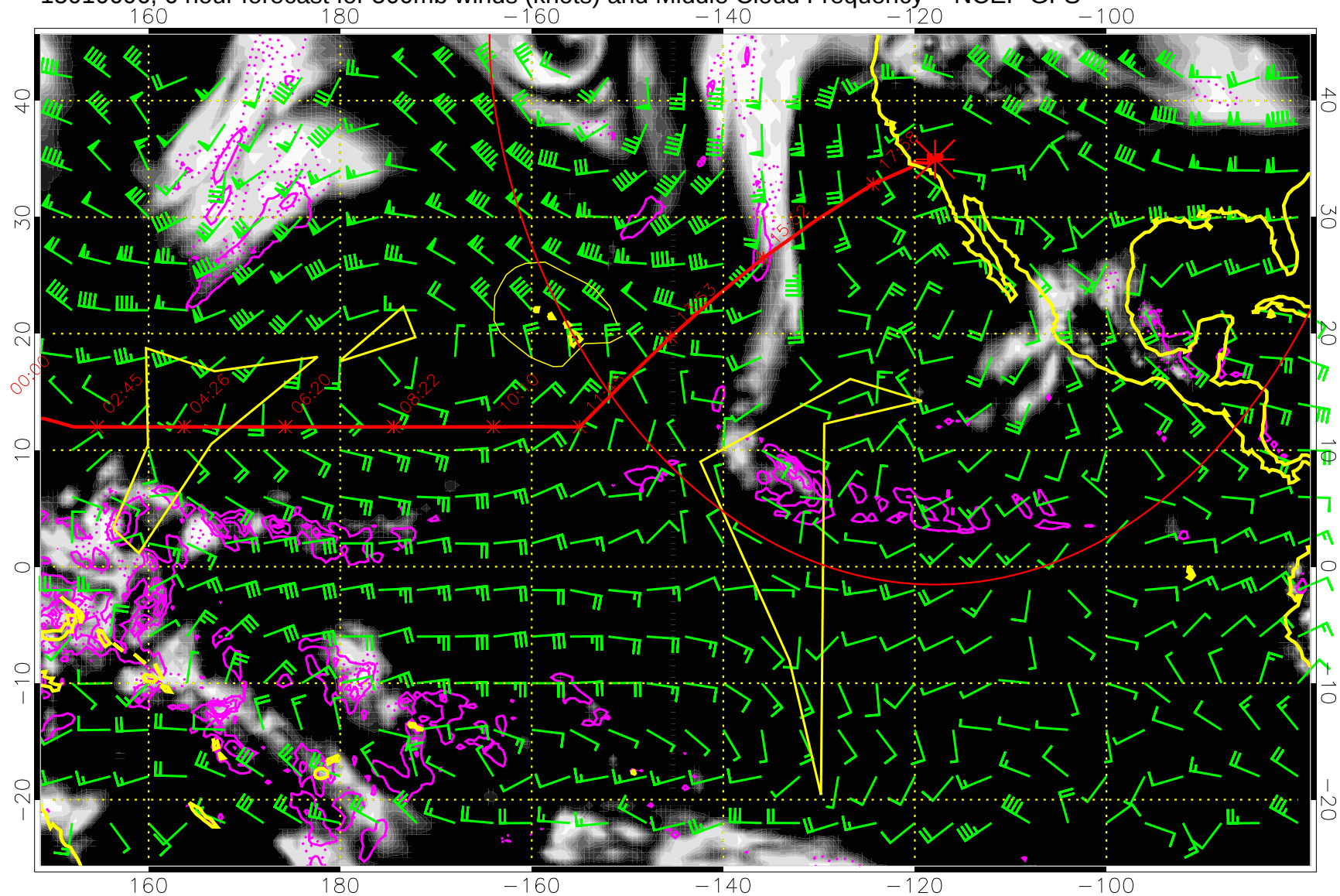
15010606, 6 hour forecast for 500mb winds (knots) and Middle Cloud Frequency -- NCEP GFS
