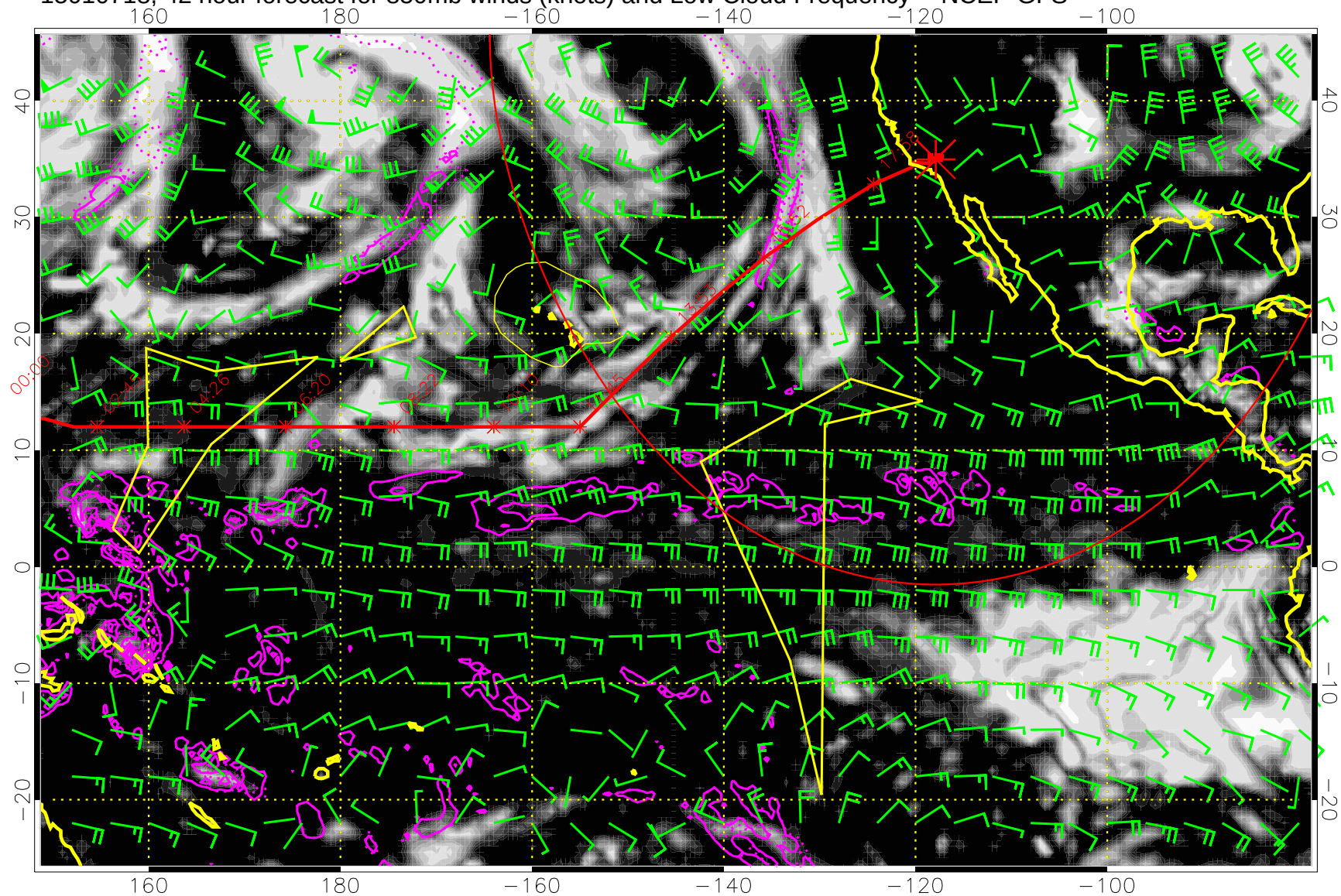
15010718, 42 hour forecast for 850mb winds (knots) and Low Cloud Frequency -- NCEP GFS
