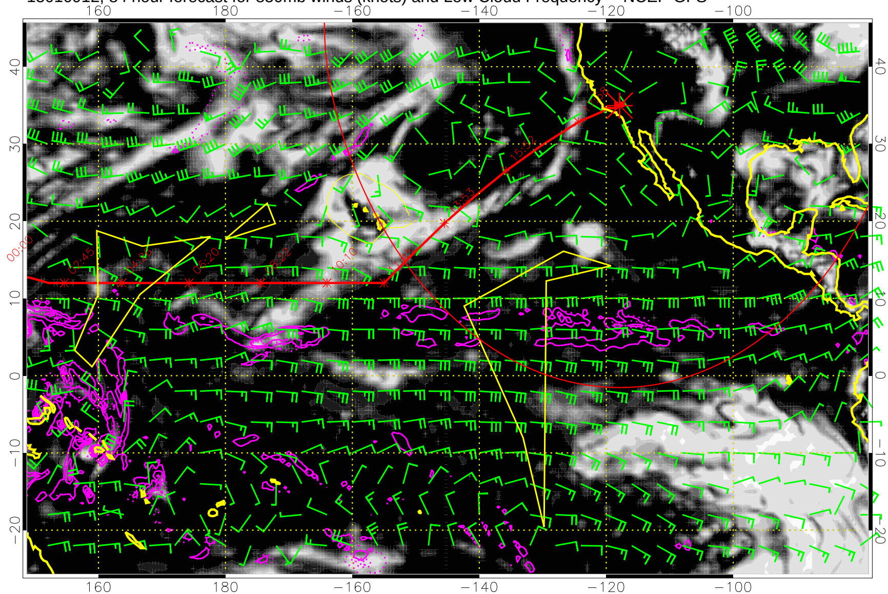
15010912, 84 hour forecast for 850mb winds (knots) and Low Cloud Frequency -- NCEP GFS
