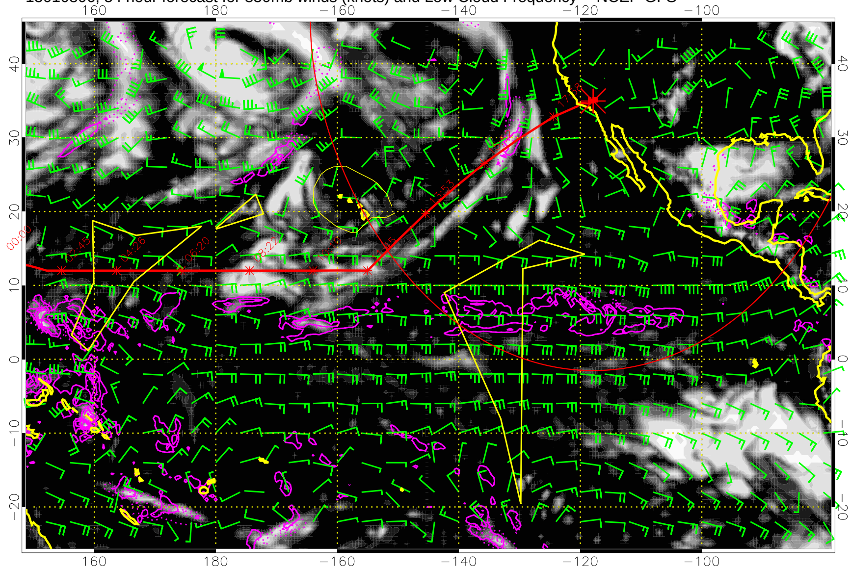
15010806, 54 hour forecast for 850mb winds (knots) and Low Cloud Frequency -- NCEP GFS
