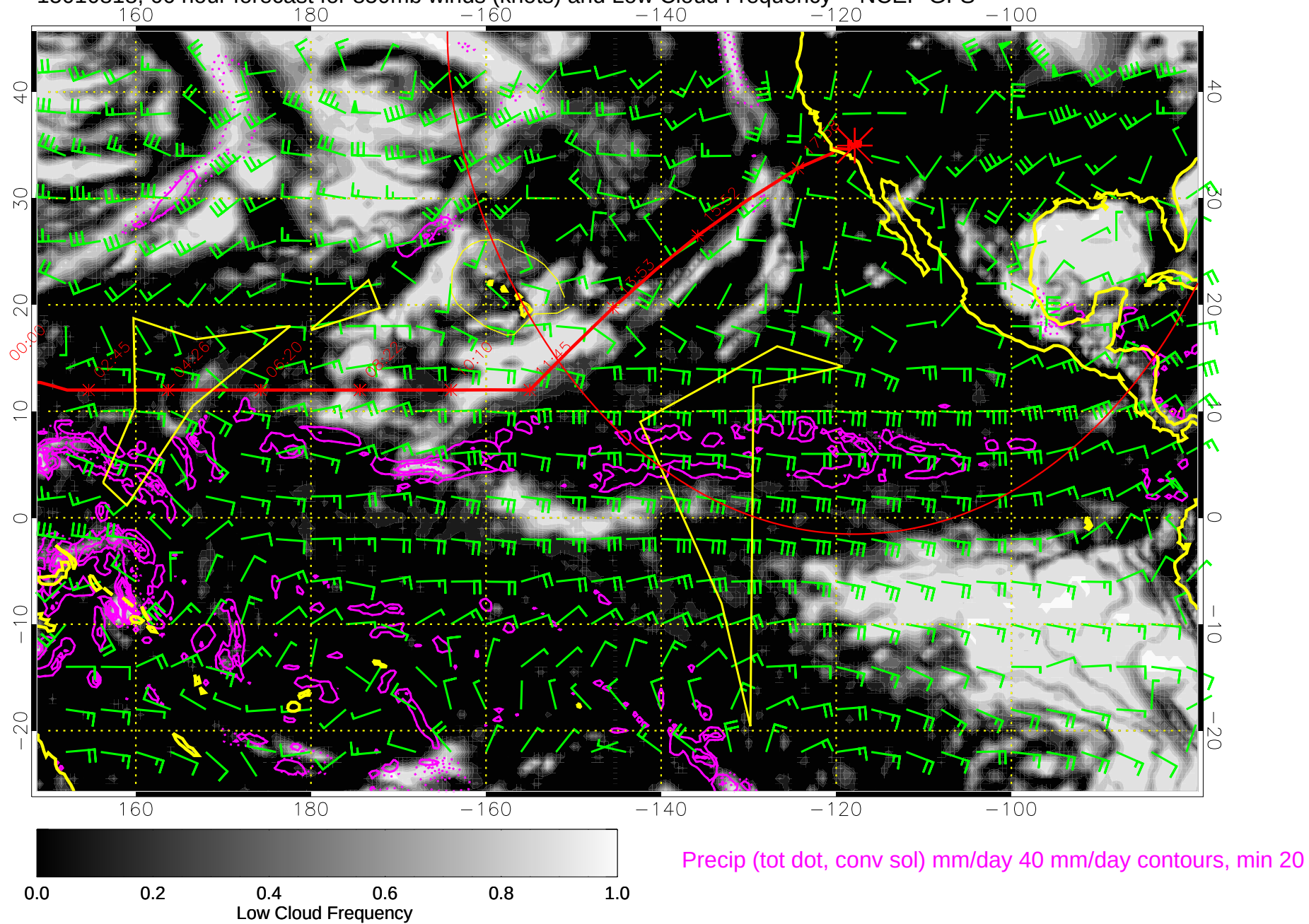
15010818, 66 hour forecast for 850mb winds (knots) and Low Cloud Frequency -- NCEP GFS
