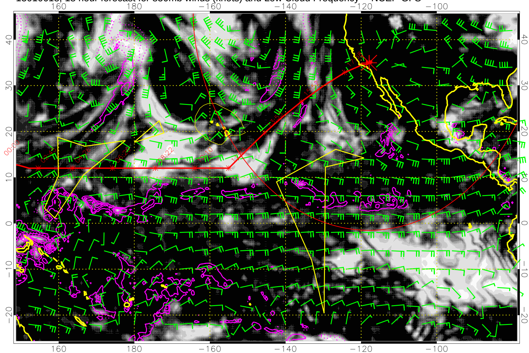
15010618, 18 hour forecast for 850mb winds (knots) and Low Cloud Frequency -- NCEP GFS
