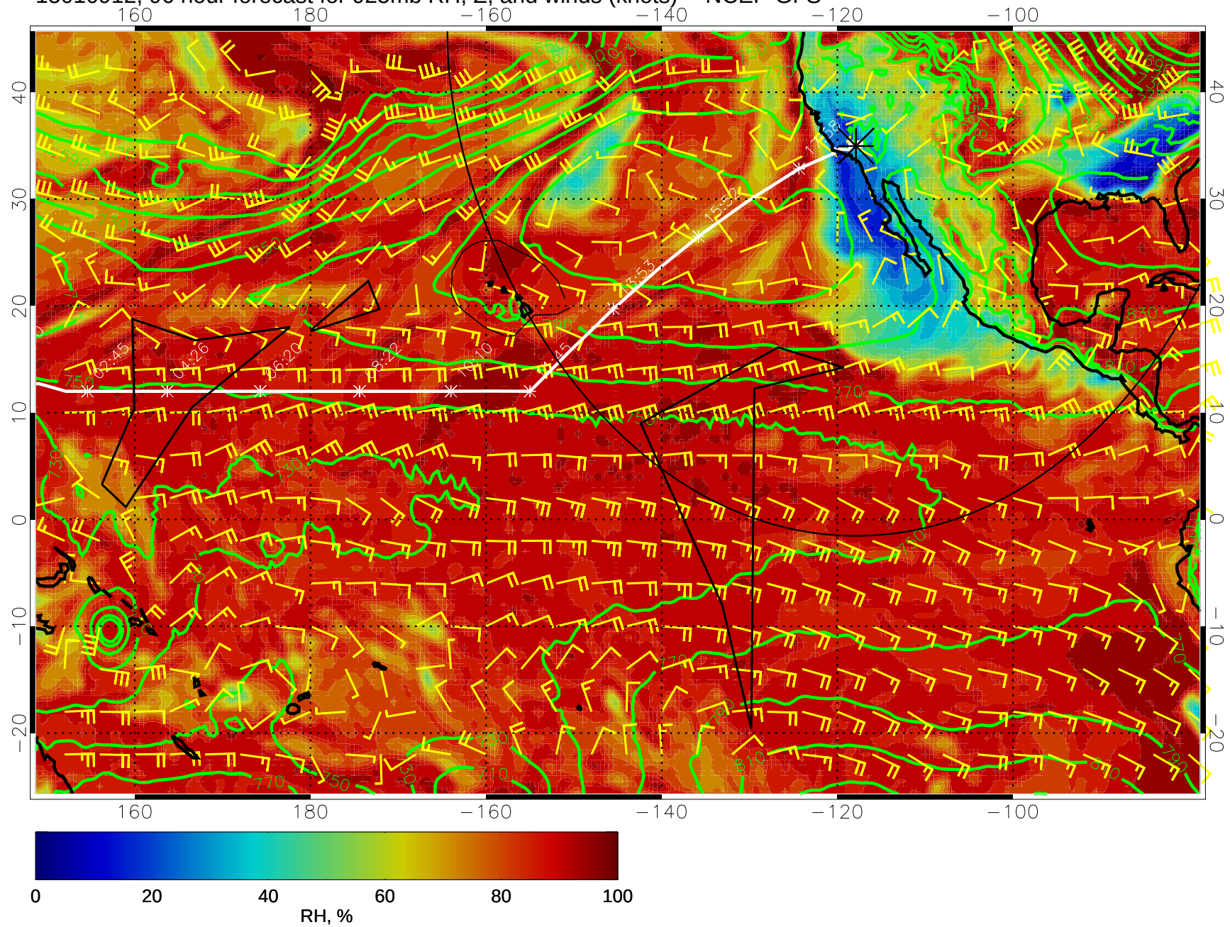
15010912, 96 hour forecast for 925mb RH, Z, and winds (knots) -- NCEP GFS
