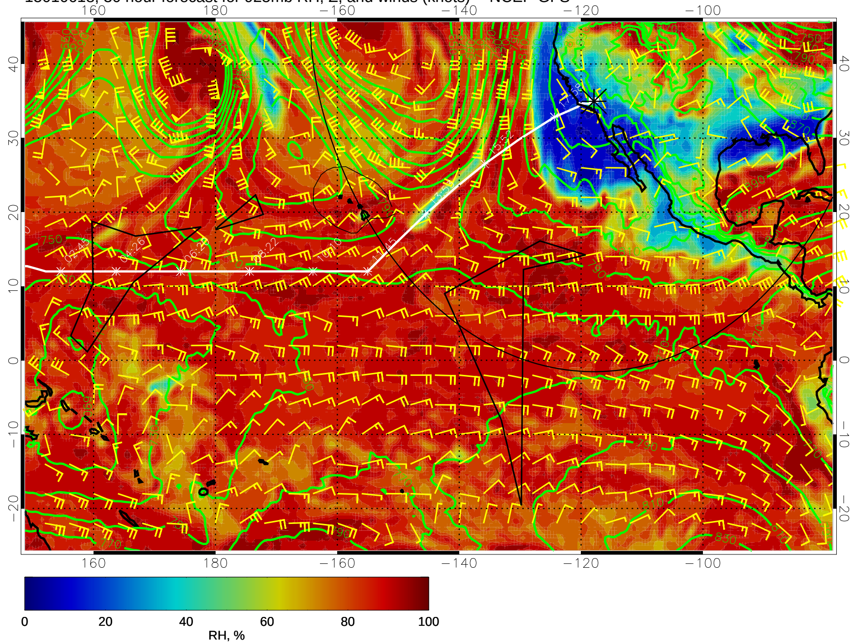
15010618, 30 hour forecast for 925mb RH, Z, and winds (knots) -- NCEP GFS
