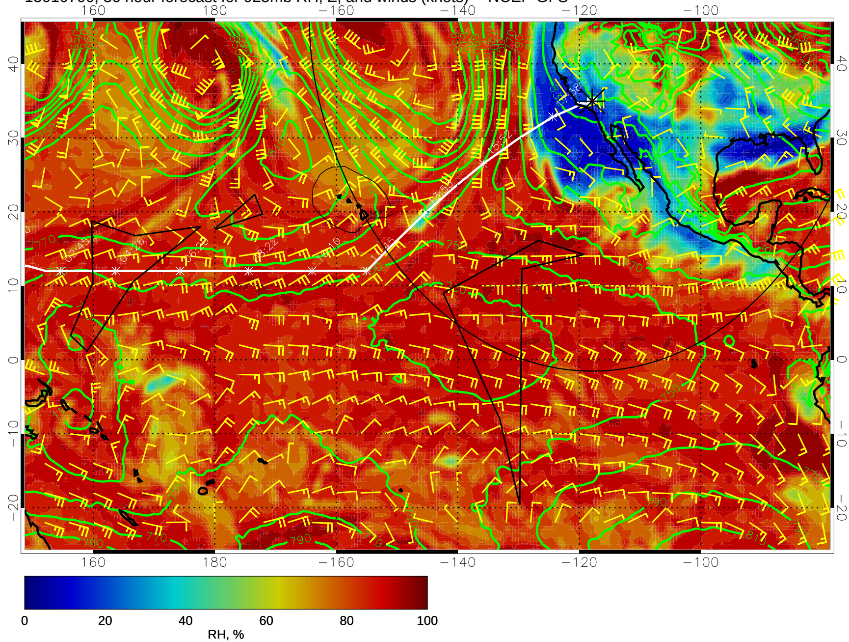
15010700, 36 hour forecast for 925mb RH, Z, and winds (knots) -- NCEP GFS
