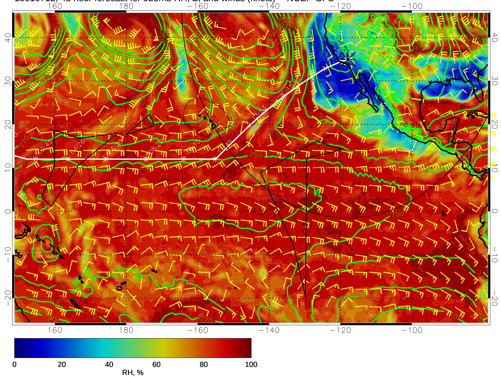
15010712, 48 hour forecast for 925mb RH, Z, and winds (knots) -- NCEP GFS
