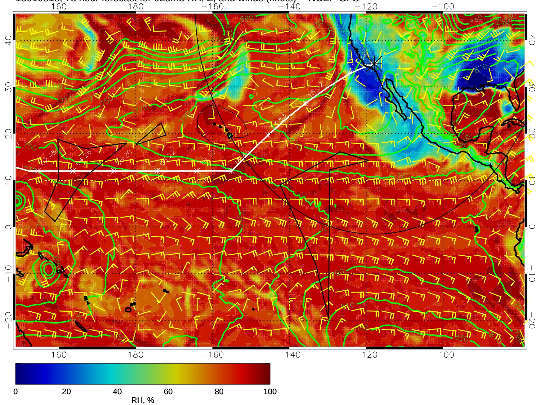
15010818, 78 hour forecast for 925mb RH, Z, and winds (knots) -- NCEP GFS
