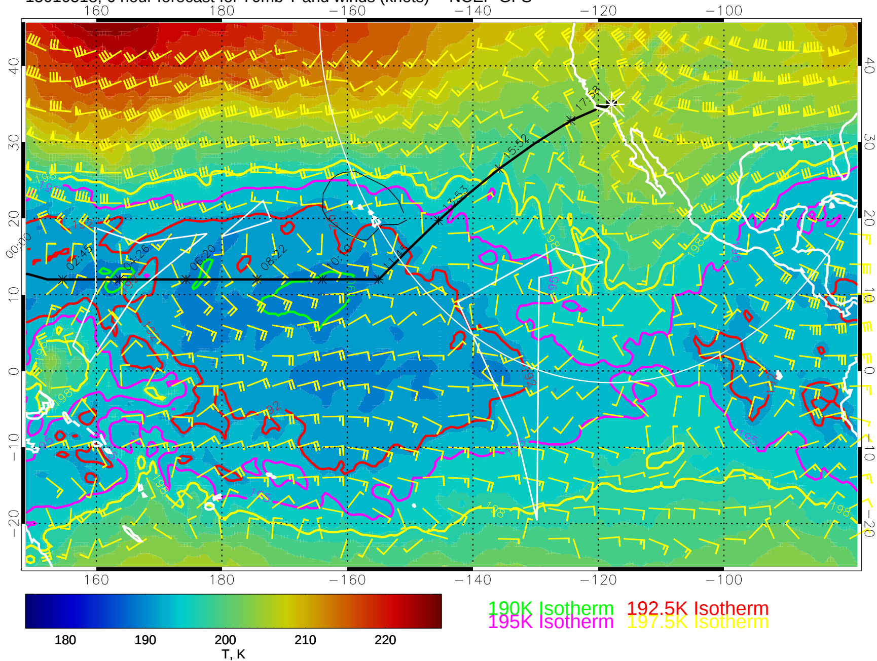
15010518, 6 hour forecast for 70mb T and winds (knots) -- NCEP GFS
