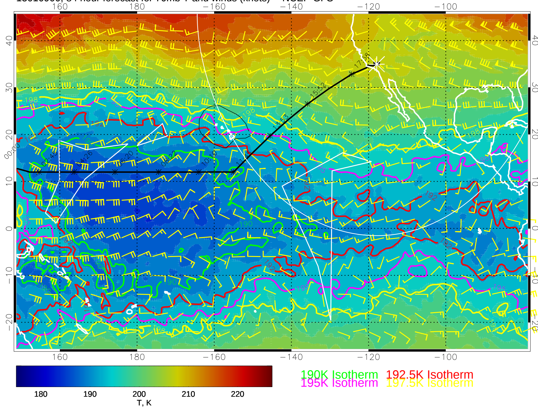
15010900, 84 hour forecast for 70mb T and winds (knots) -- NCEP GFS
