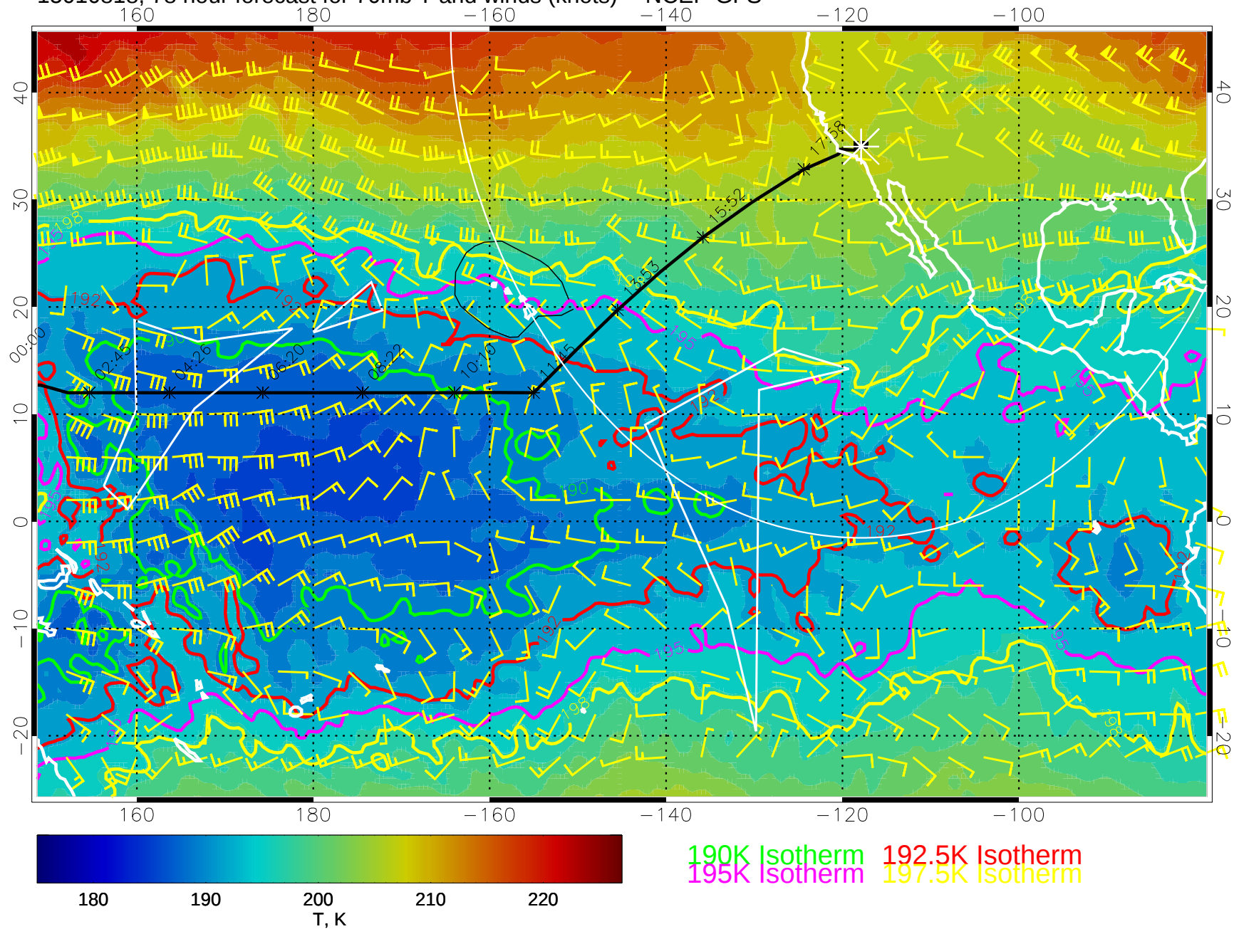
15010818, 78 hour forecast for 70mb T and winds (knots) -- NCEP GFS
