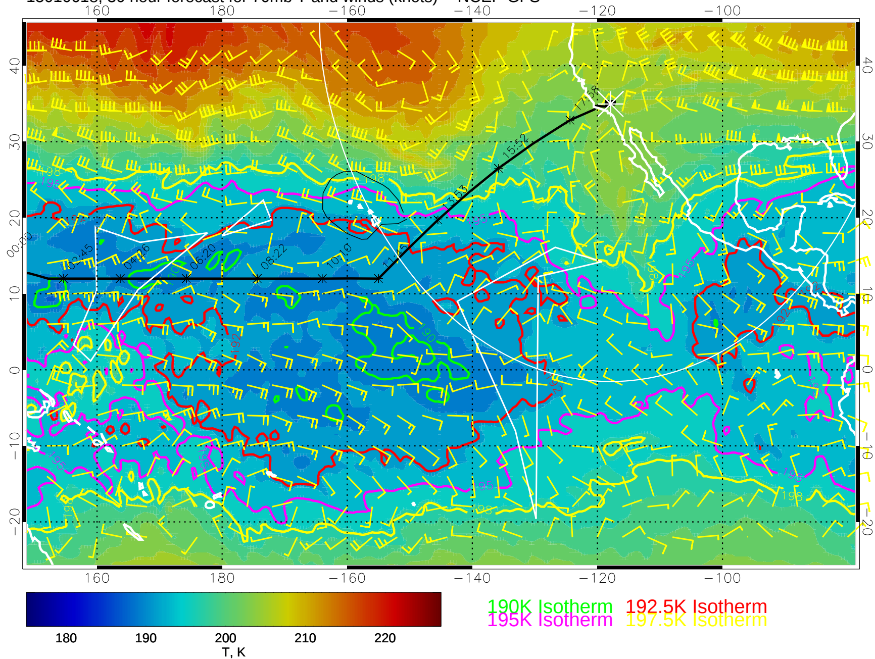
15010618, 30 hour forecast for 70mb T and winds (knots) -- NCEP GFS
