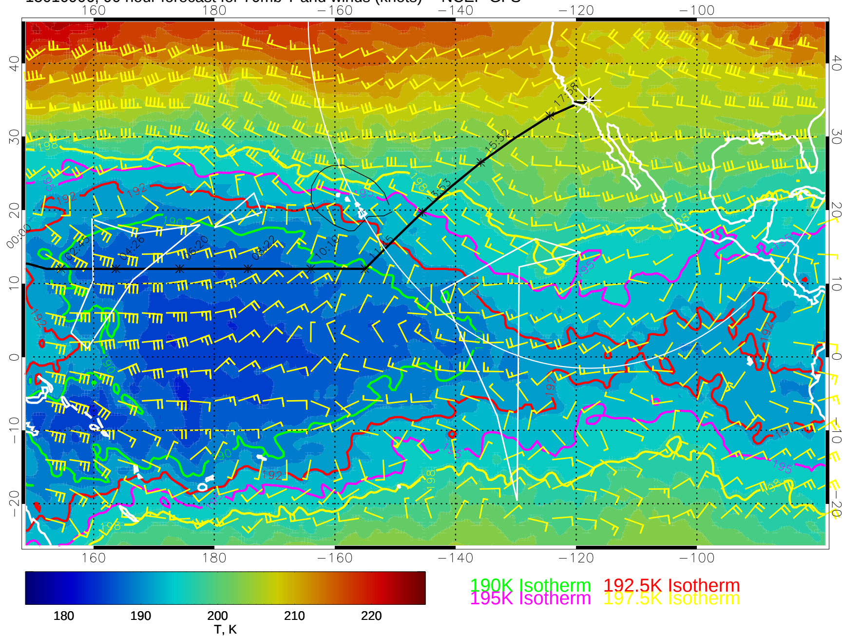
15010906, 90 hour forecast for 70mb T and winds (knots) -- NCEP GFS
