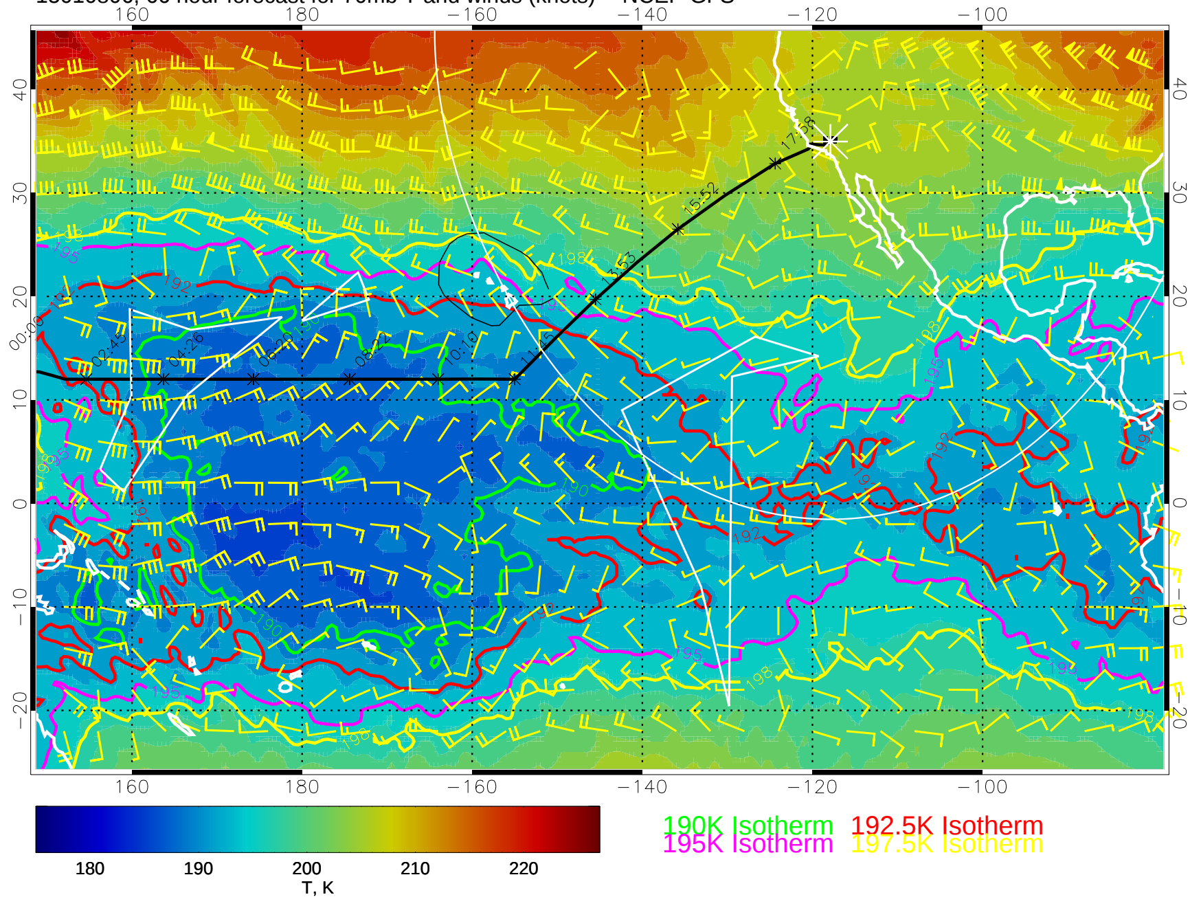
15010806, 66 hour forecast for 70mb T and winds (knots) -- NCEP GFS
