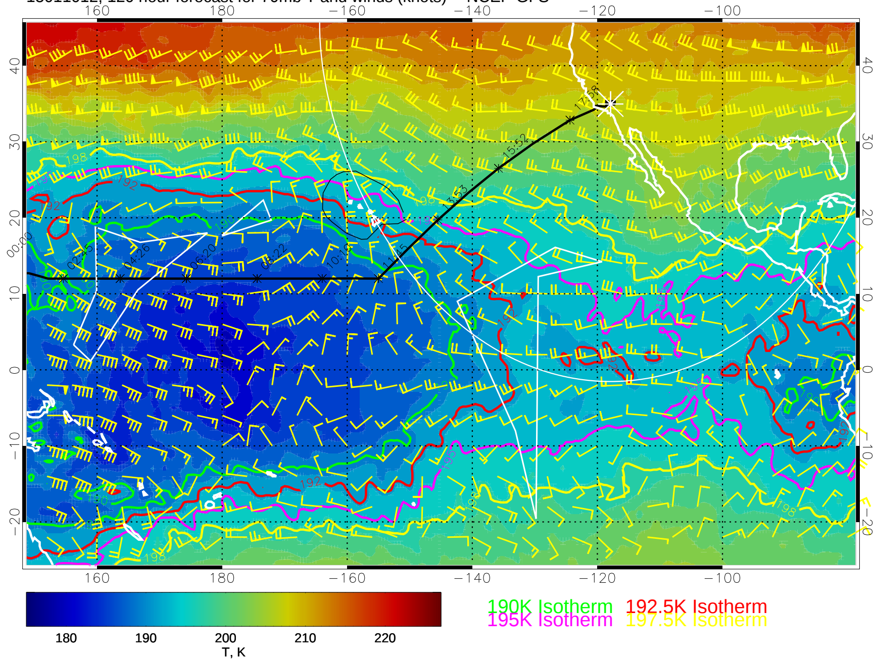
15011012, 120 hour forecast for 70mb T and winds (knots) -- NCEP GFS
