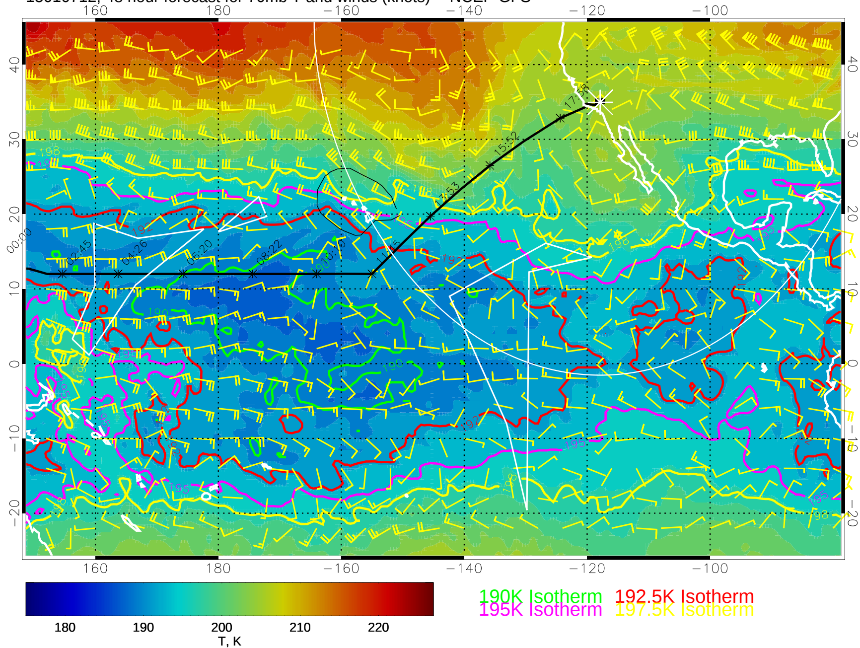
15010712, 48 hour forecast for 70mb T and winds (knots) -- NCEP GFS
