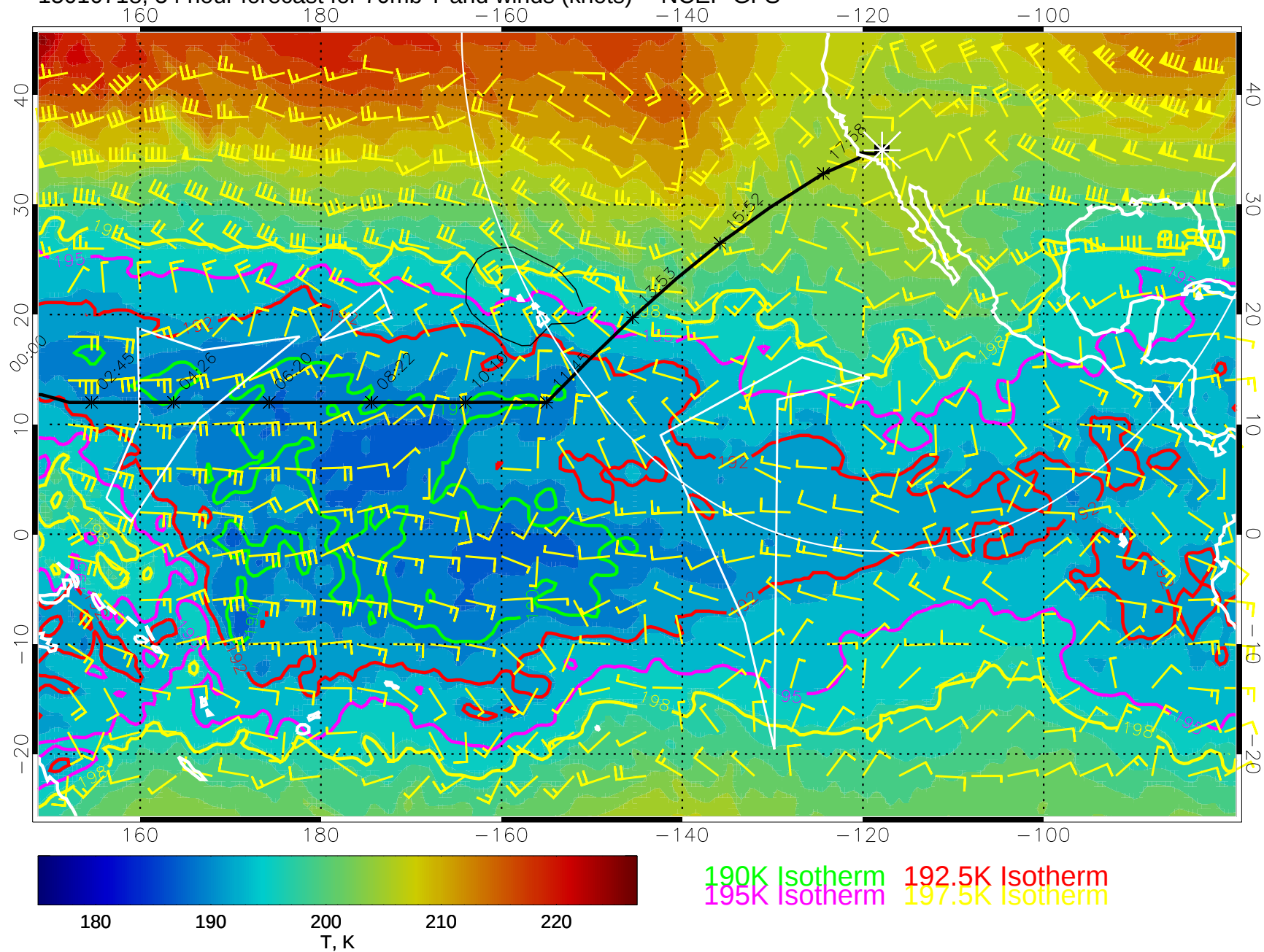
15010718, 54 hour forecast for 70mb T and winds (knots) -- NCEP GFS
