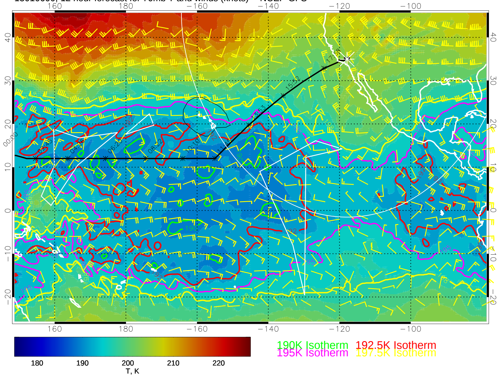
15010600, 12 hour forecast for 70mb T and winds (knots) -- NCEP GFS
