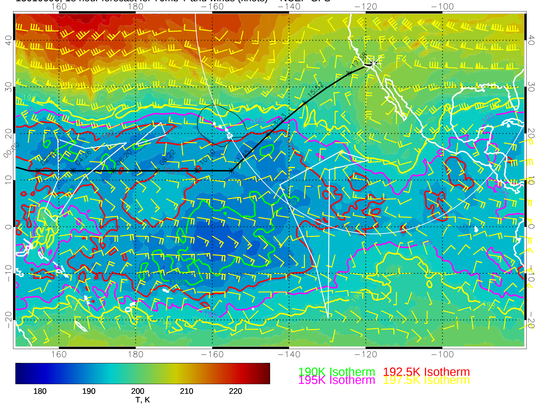
15010606, 18 hour forecast for 70mb T and winds (knots) -- NCEP GFS
