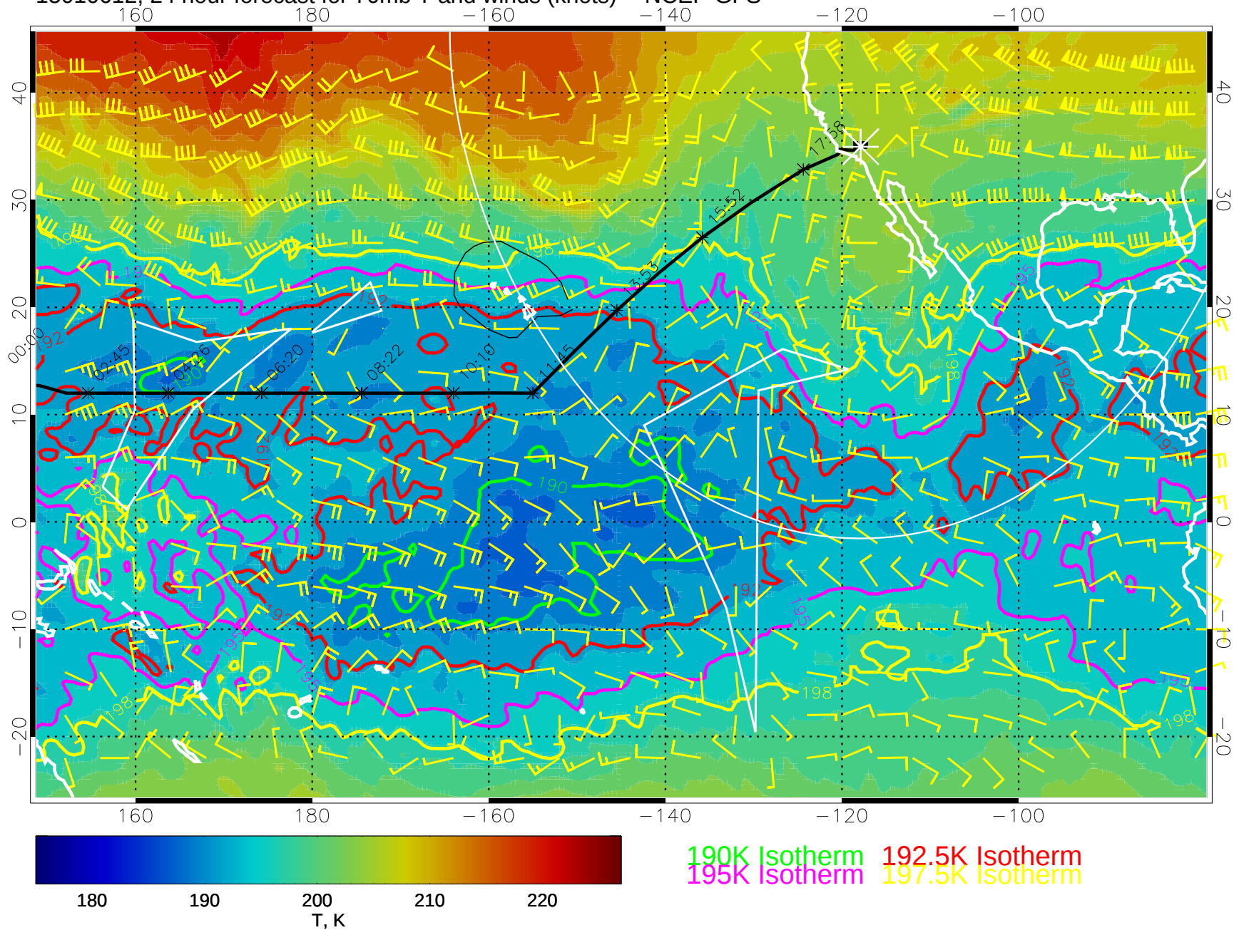
15010612, 24 hour forecast for 70mb T and winds (knots) -- NCEP GFS
