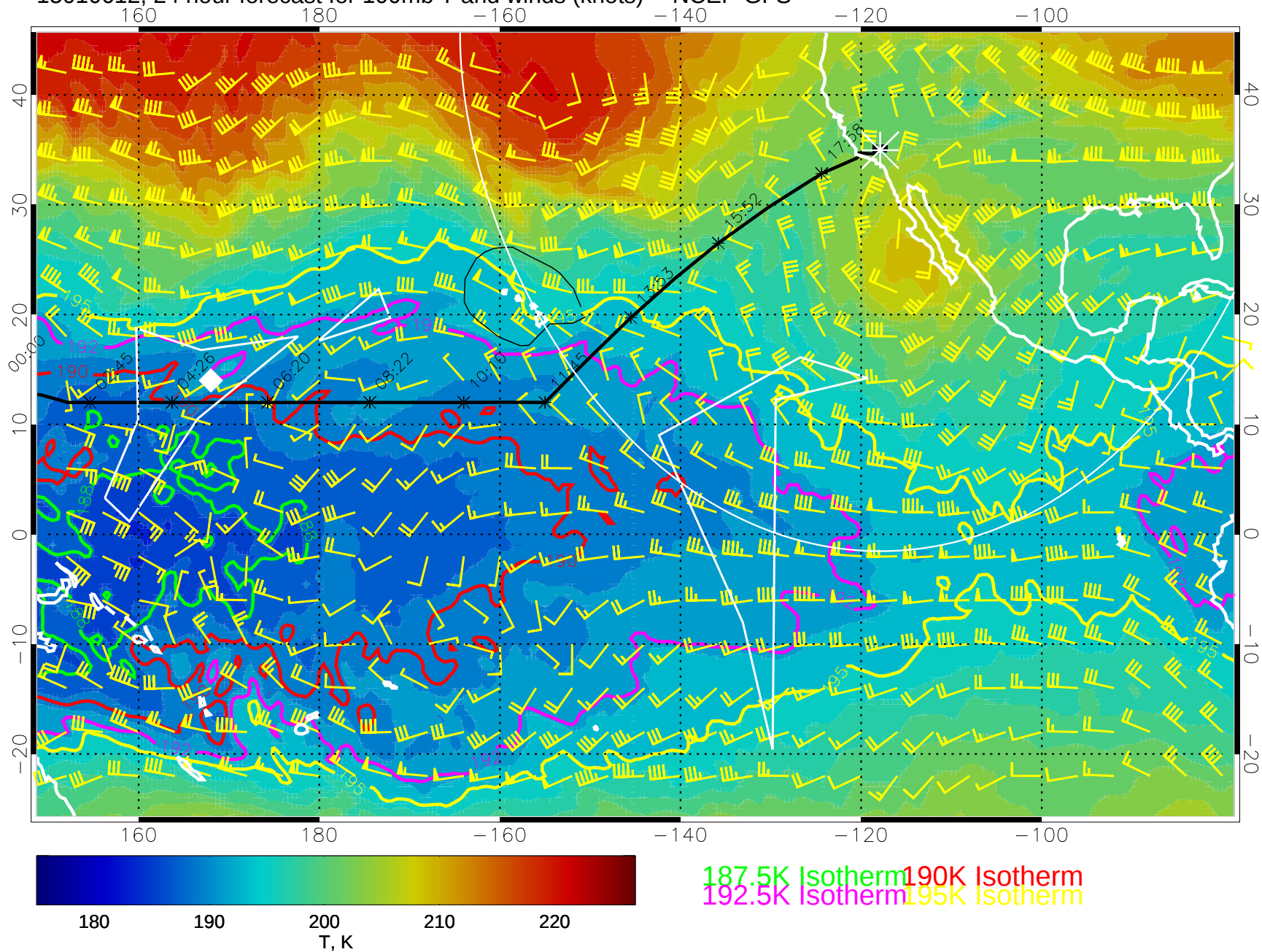
15010612, 24 hour forecast for 100mb T and winds (knots) -- NCEP GFS
