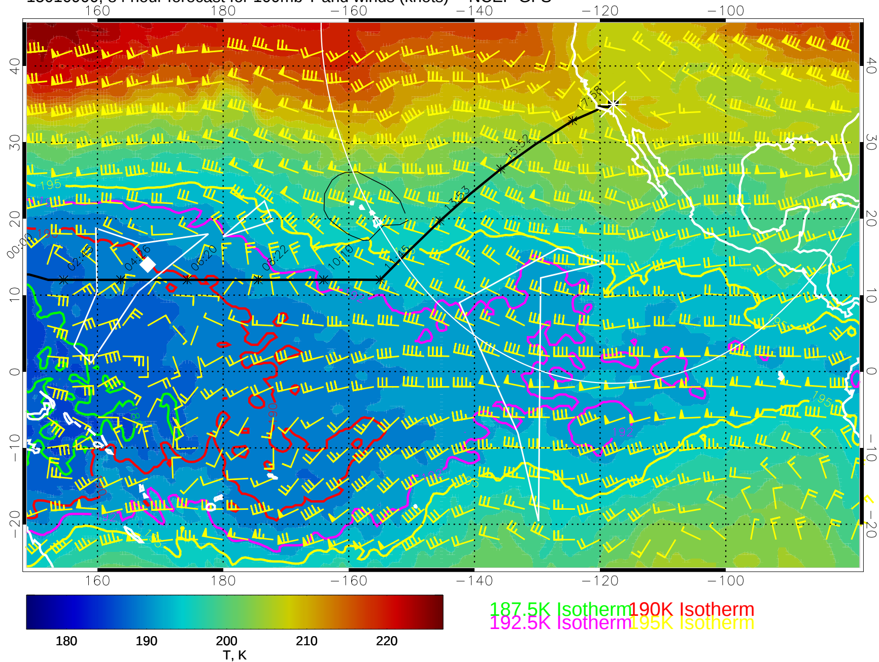
15010900, 84 hour forecast for 100mb T and winds (knots) -- NCEP GFS
