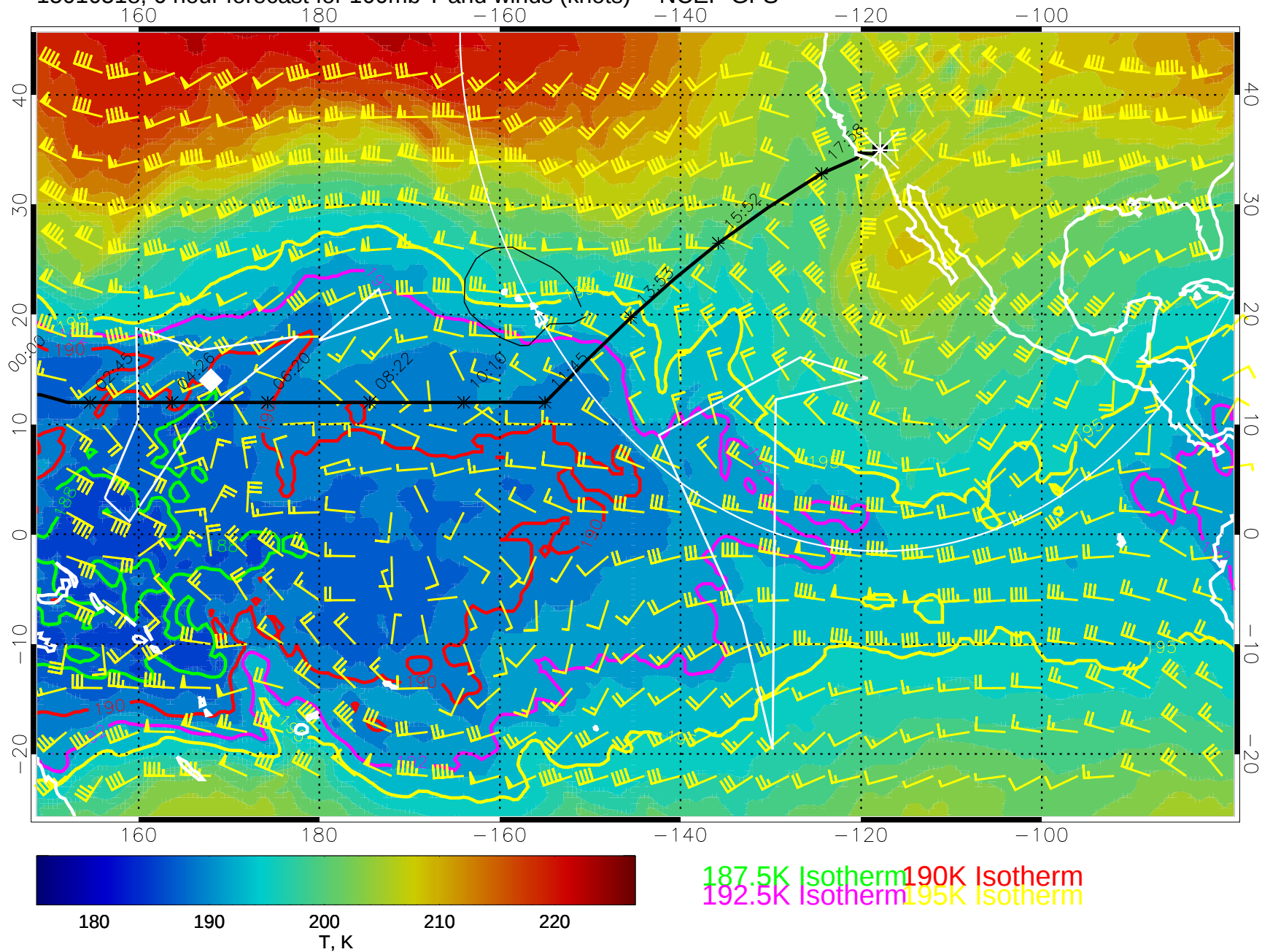
15010518, 6 hour forecast for 100mb T and winds (knots) -- NCEP GFS
