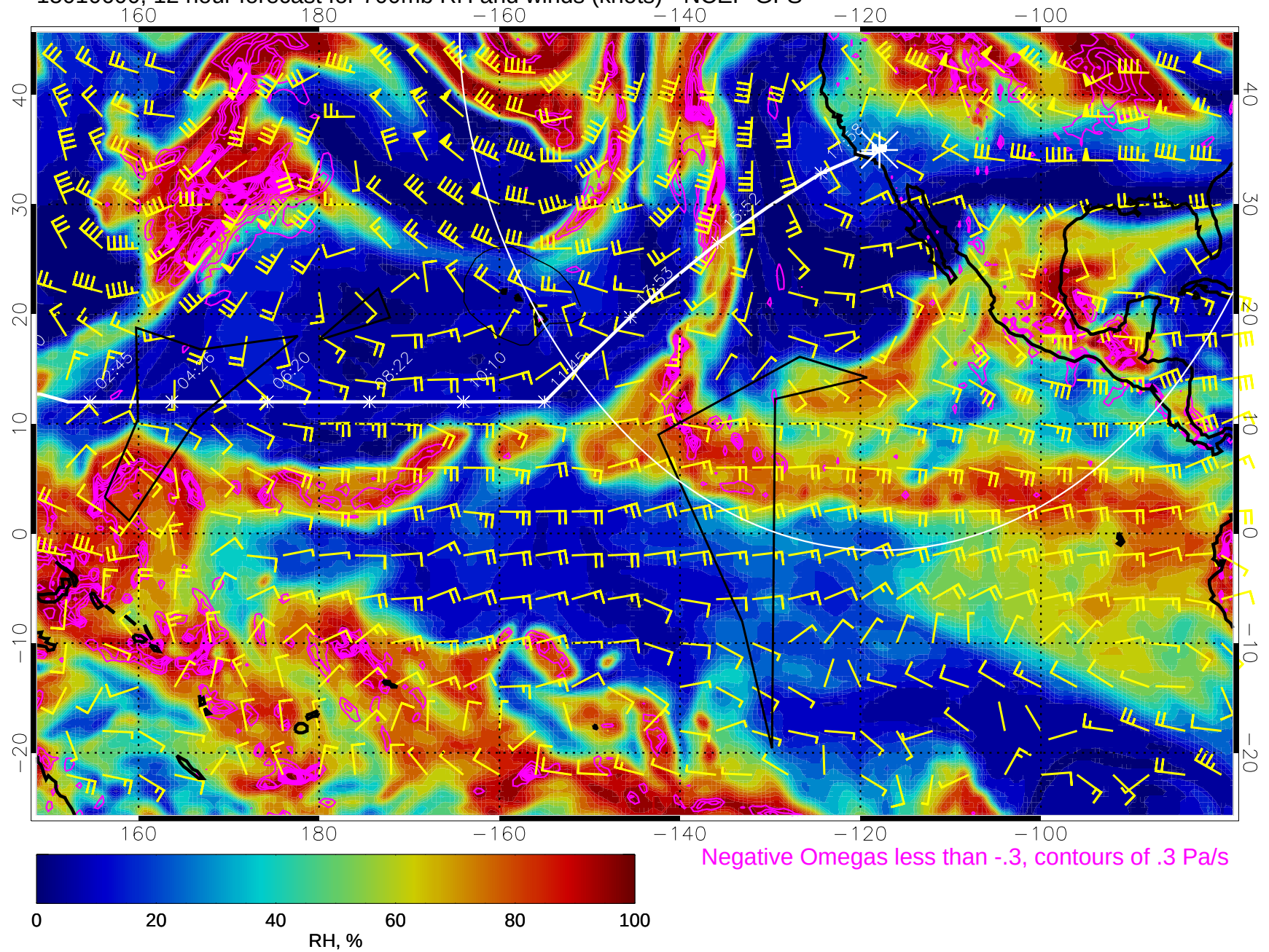
15010600, 12 hour forecast for 700mb RH and winds (knots) - NCEP GFS
