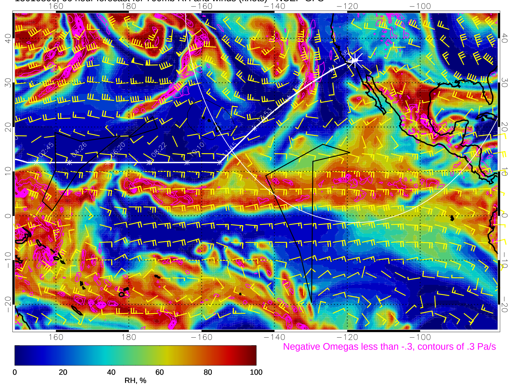
15010806, 66 hour forecast for 700mb RH and winds (knots) - NCEP GFS
