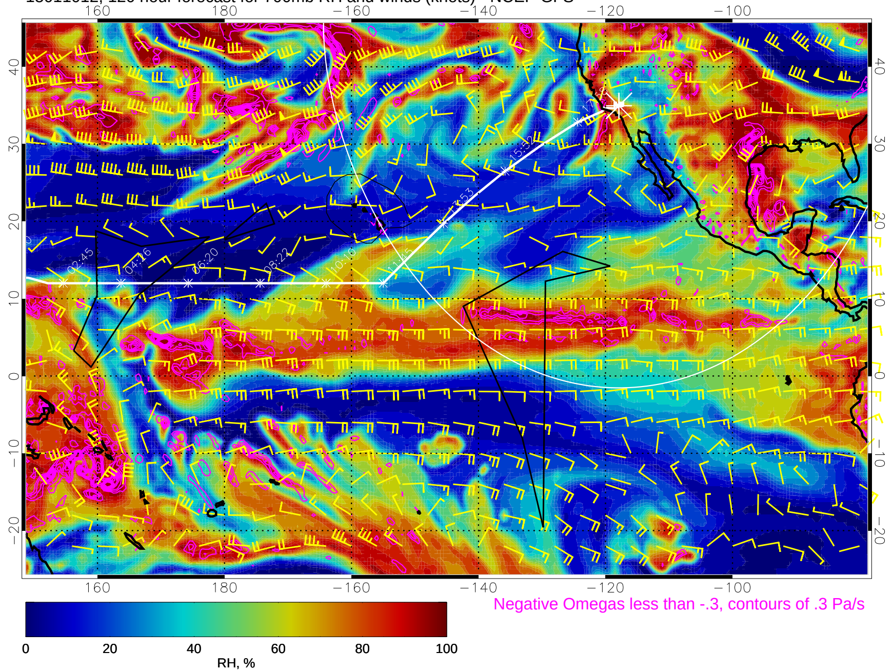
15011012, 120 hour forecast for 700mb RH and winds (knots) - NCEP GFS
