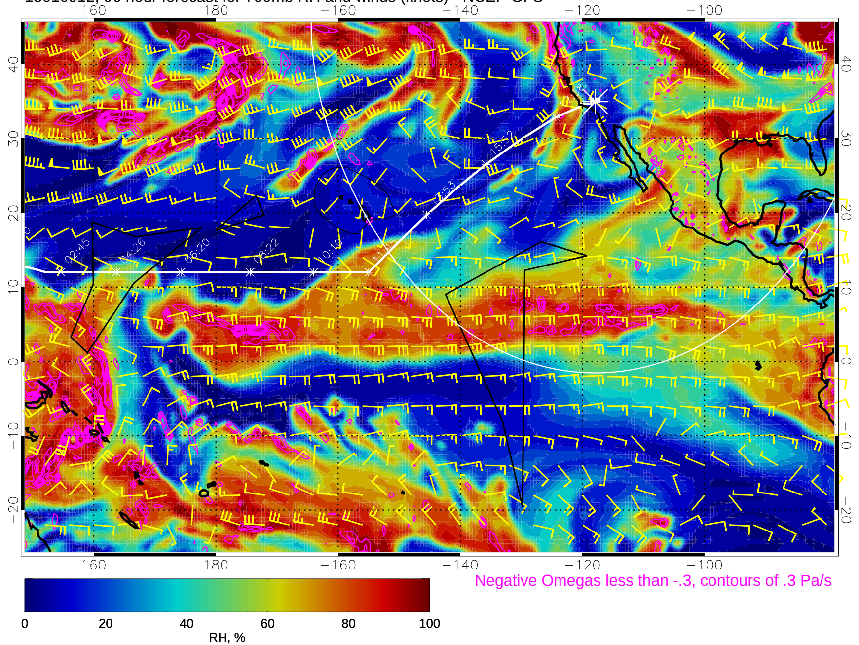
15010912, 96 hour forecast for 700mb RH and winds (knots) - NCEP GFS
