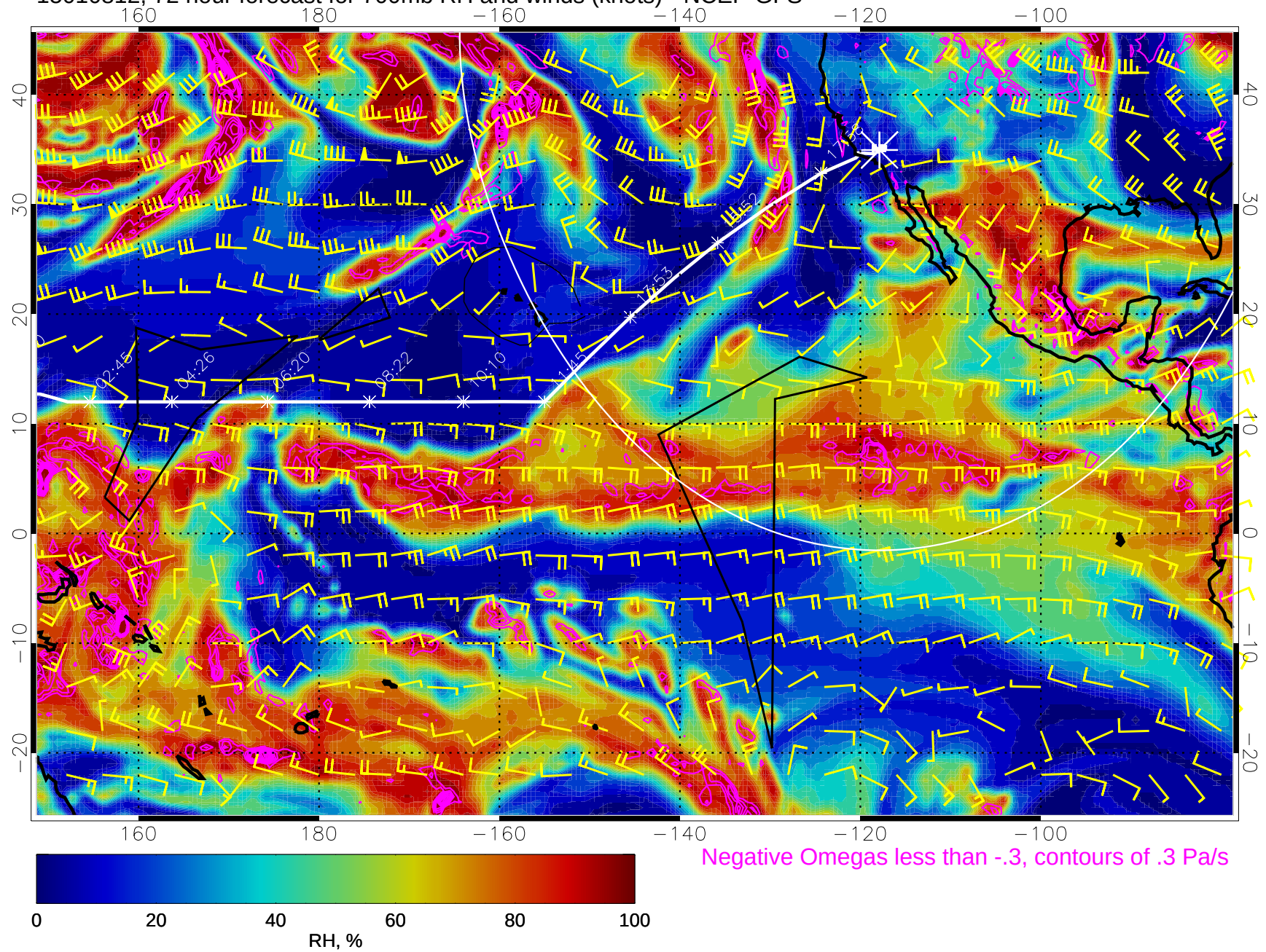
15010812, 72 hour forecast for 700mb RH and winds (knots) - NCEP GFS
