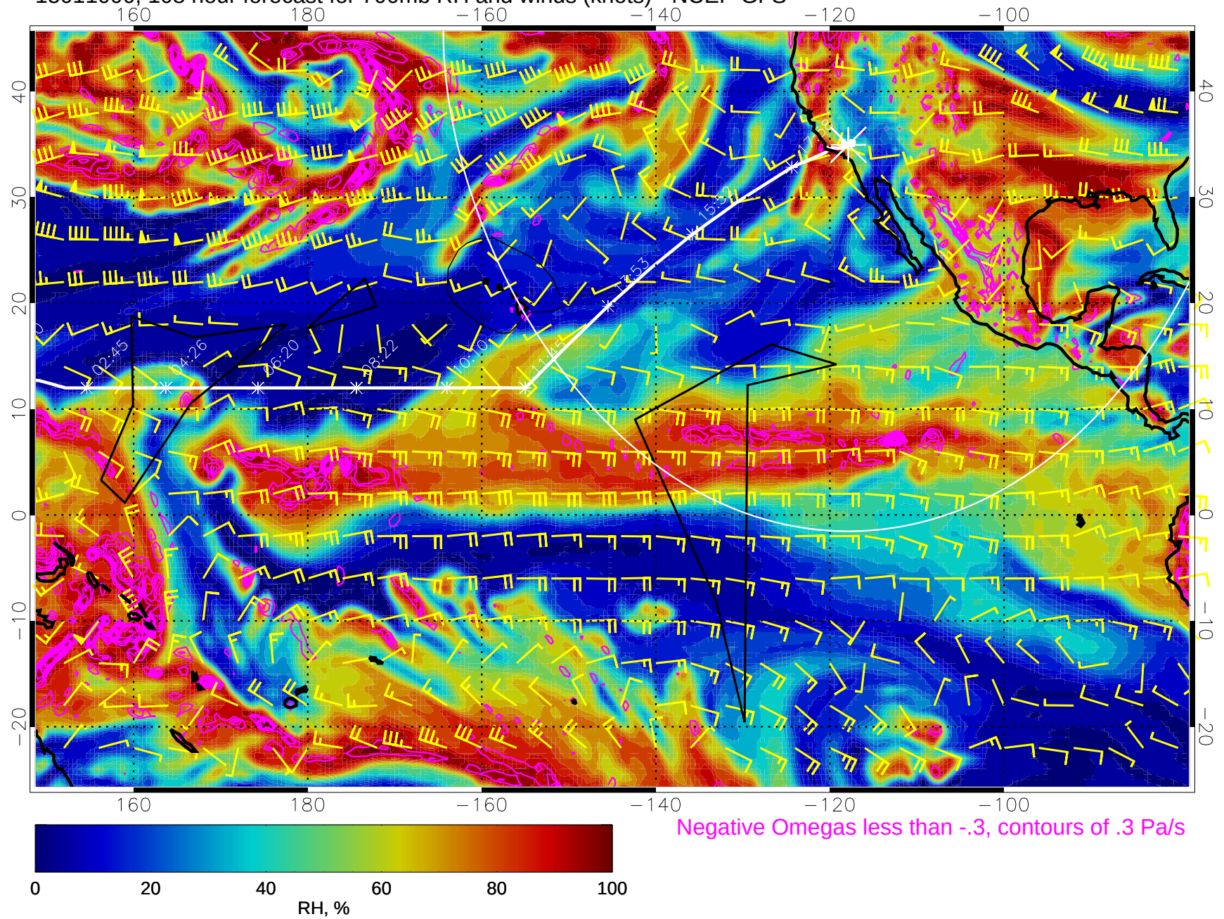
15011000, 108 hour forecast for 700mb RH and winds (knots) - NCEP GFS
