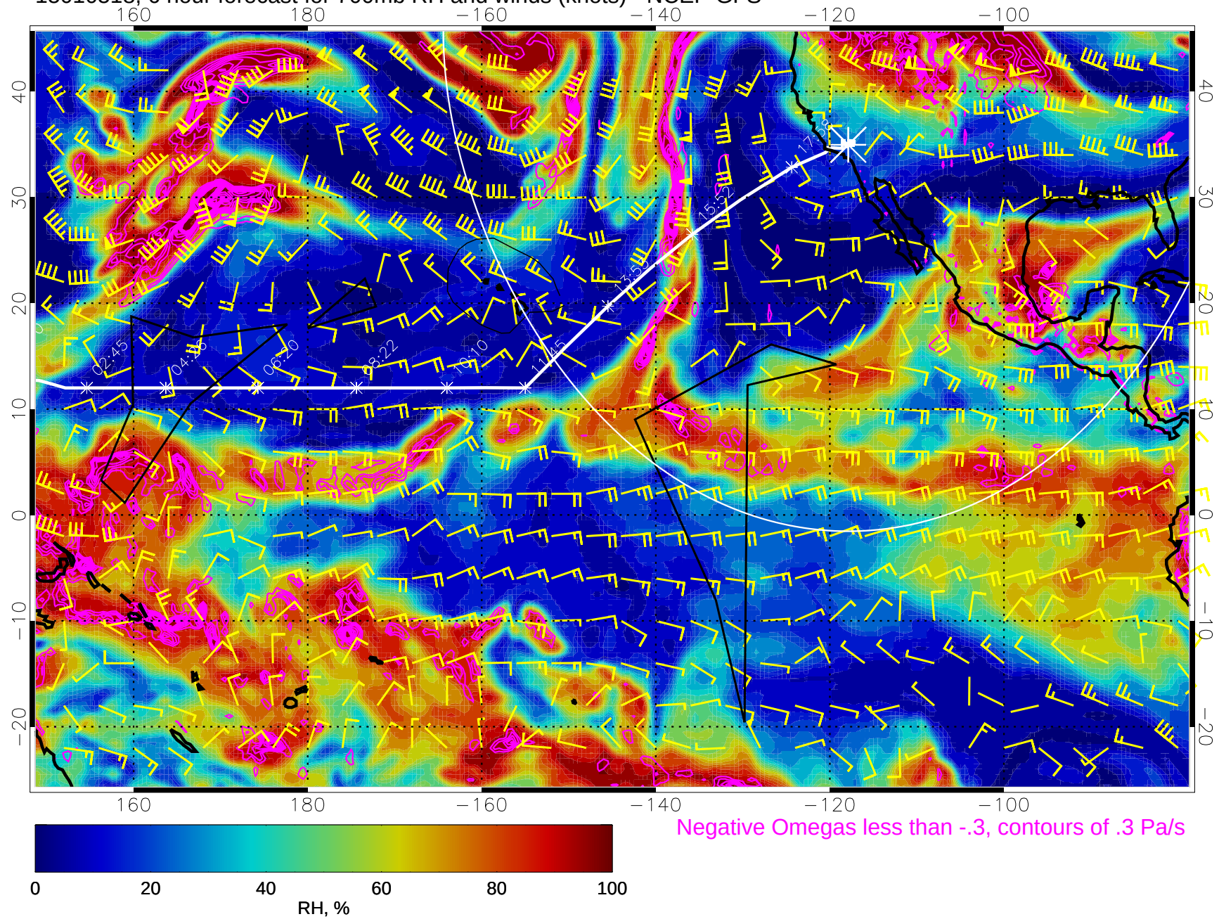
15010518, 6 hour forecast for 700mb RH and winds (knots) - NCEP GFS
