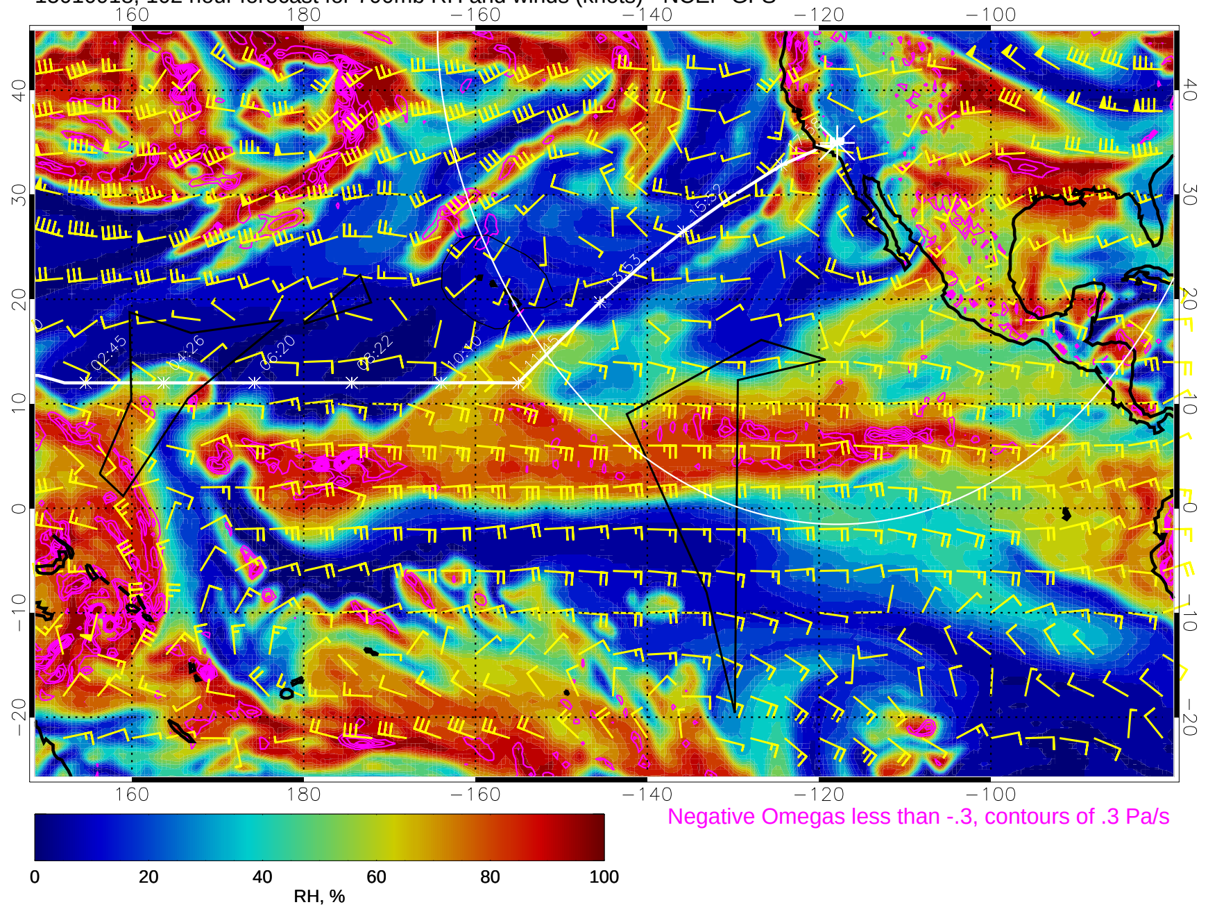
15010918, 102 hour forecast for 700mb RH and winds (knots) - NCEP GFS
