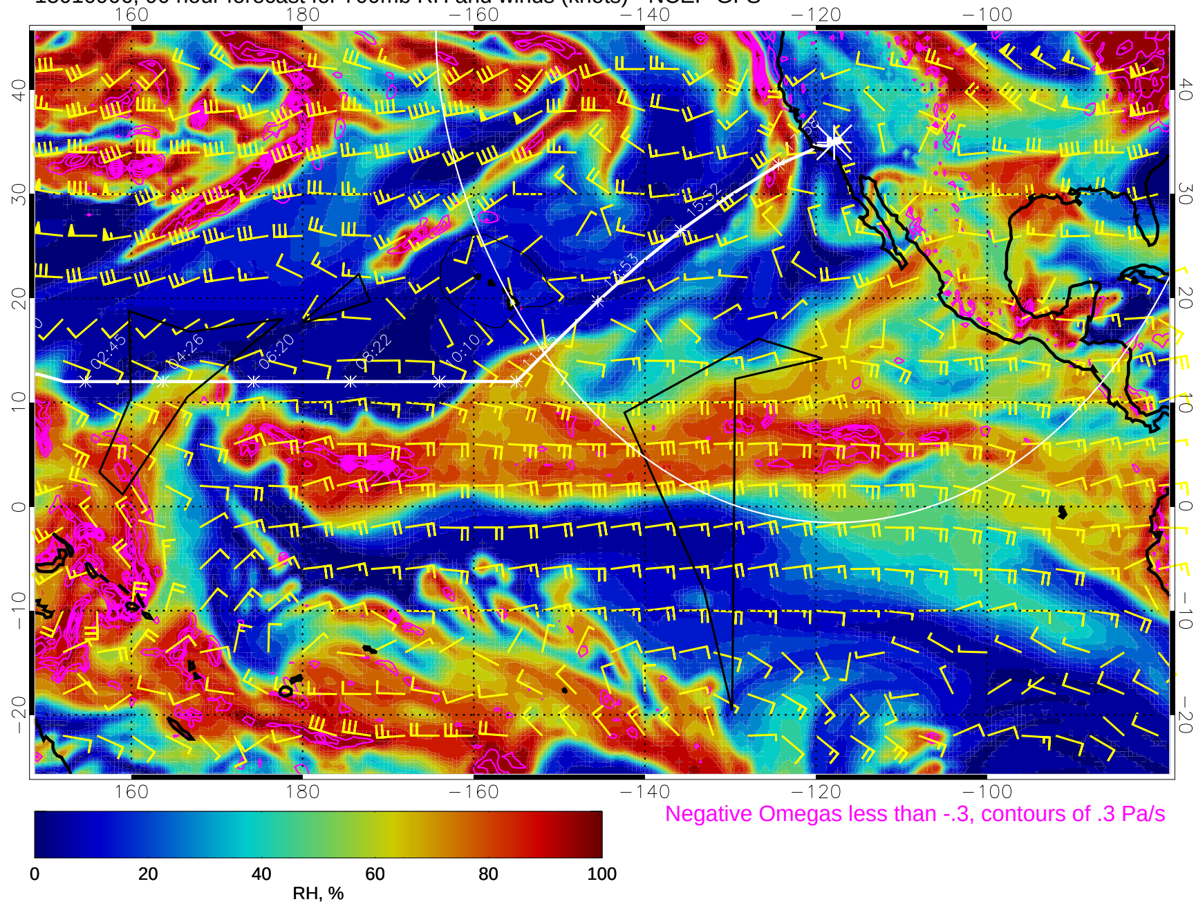
15010906, 90 hour forecast for 700mb RH and winds (knots) - NCEP GFS
