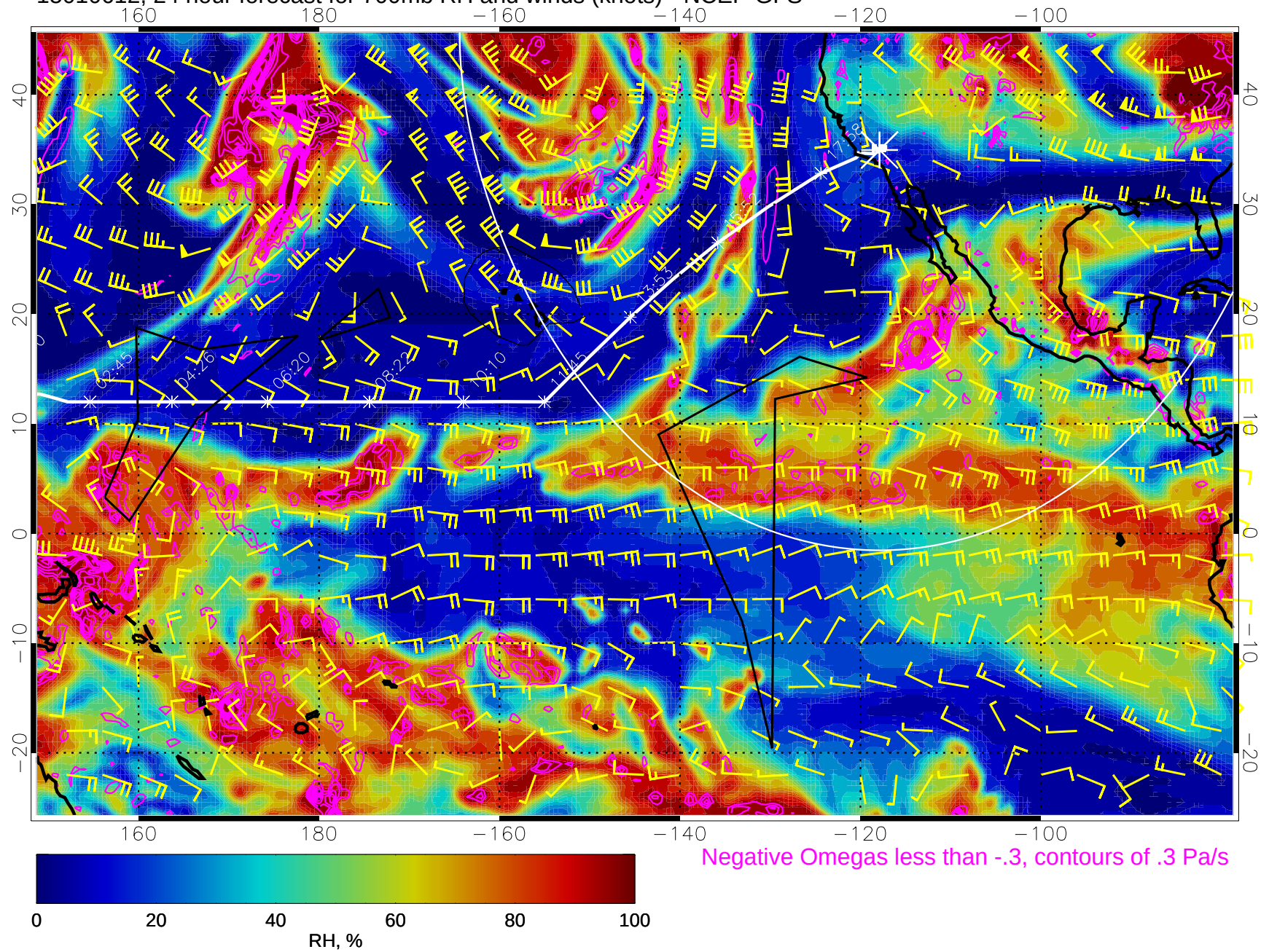
15010612, 24 hour forecast for 700mb RH and winds (knots) - NCEP GFS
