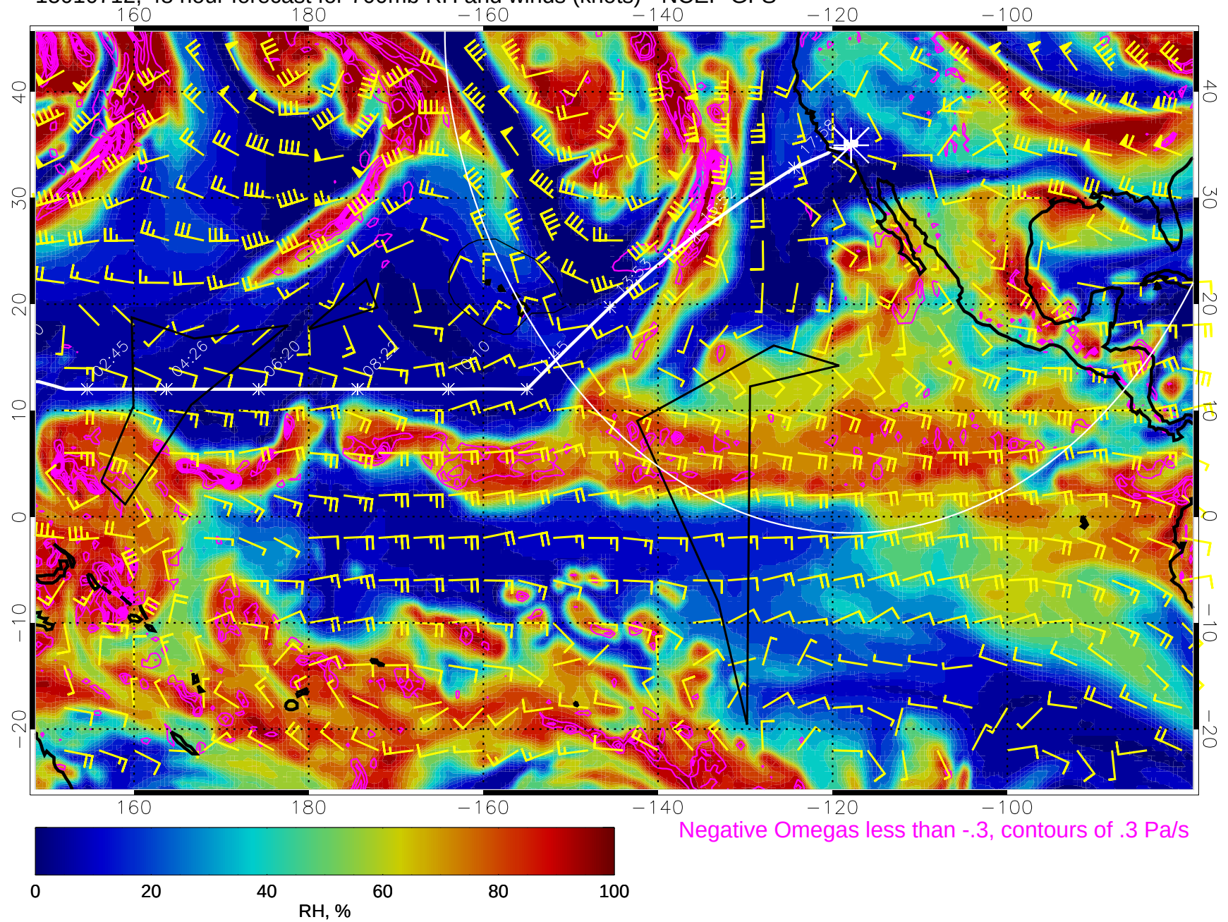
15010712, 48 hour forecast for 700mb RH and winds (knots) - NCEP GFS
