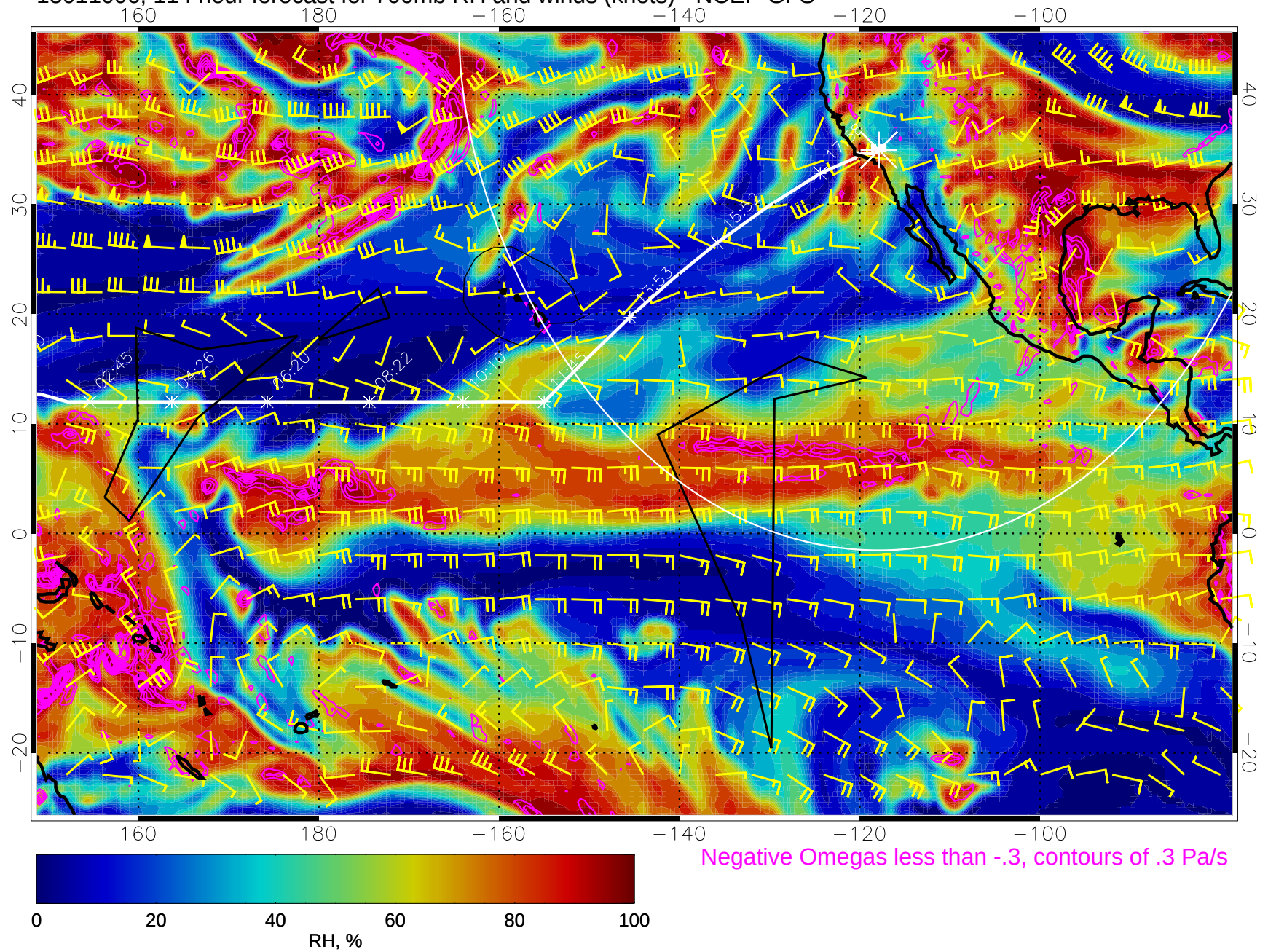
15011006, 114 hour forecast for 700mb RH and winds (knots) - NCEP GFS
