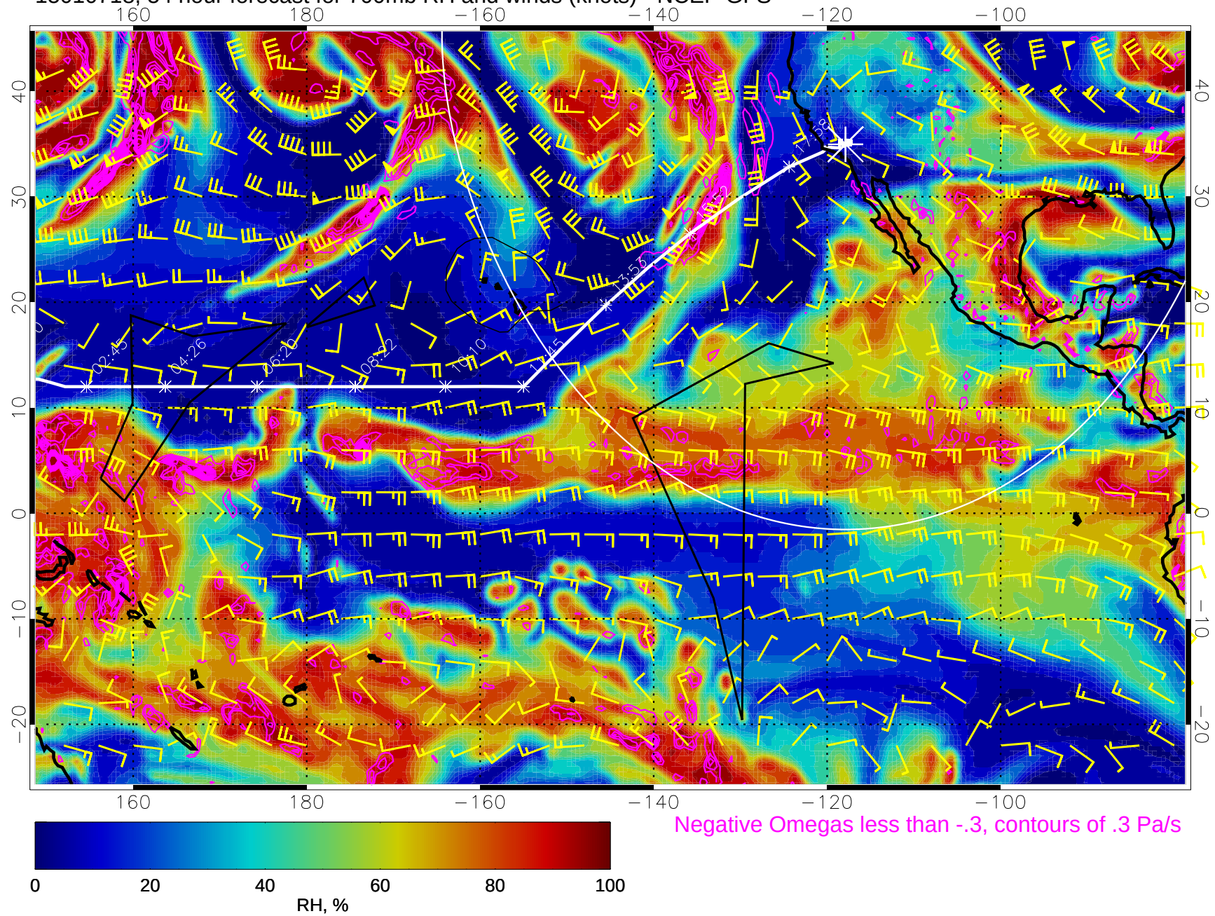
15010718, 54 hour forecast for 700mb RH and winds (knots) - NCEP GFS
