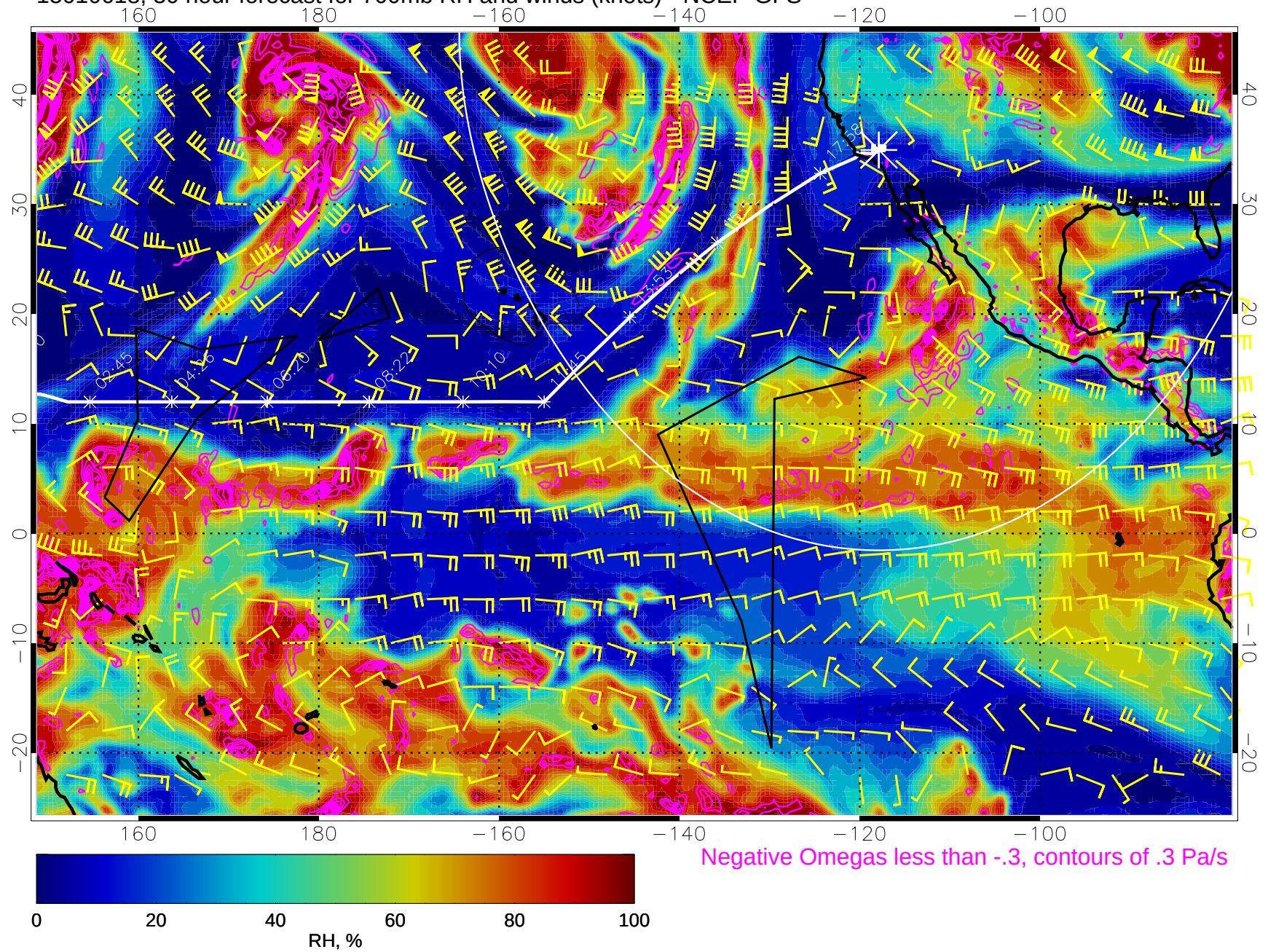
15010618, 30 hour forecast for 700mb RH and winds (knots) - NCEP GFS
