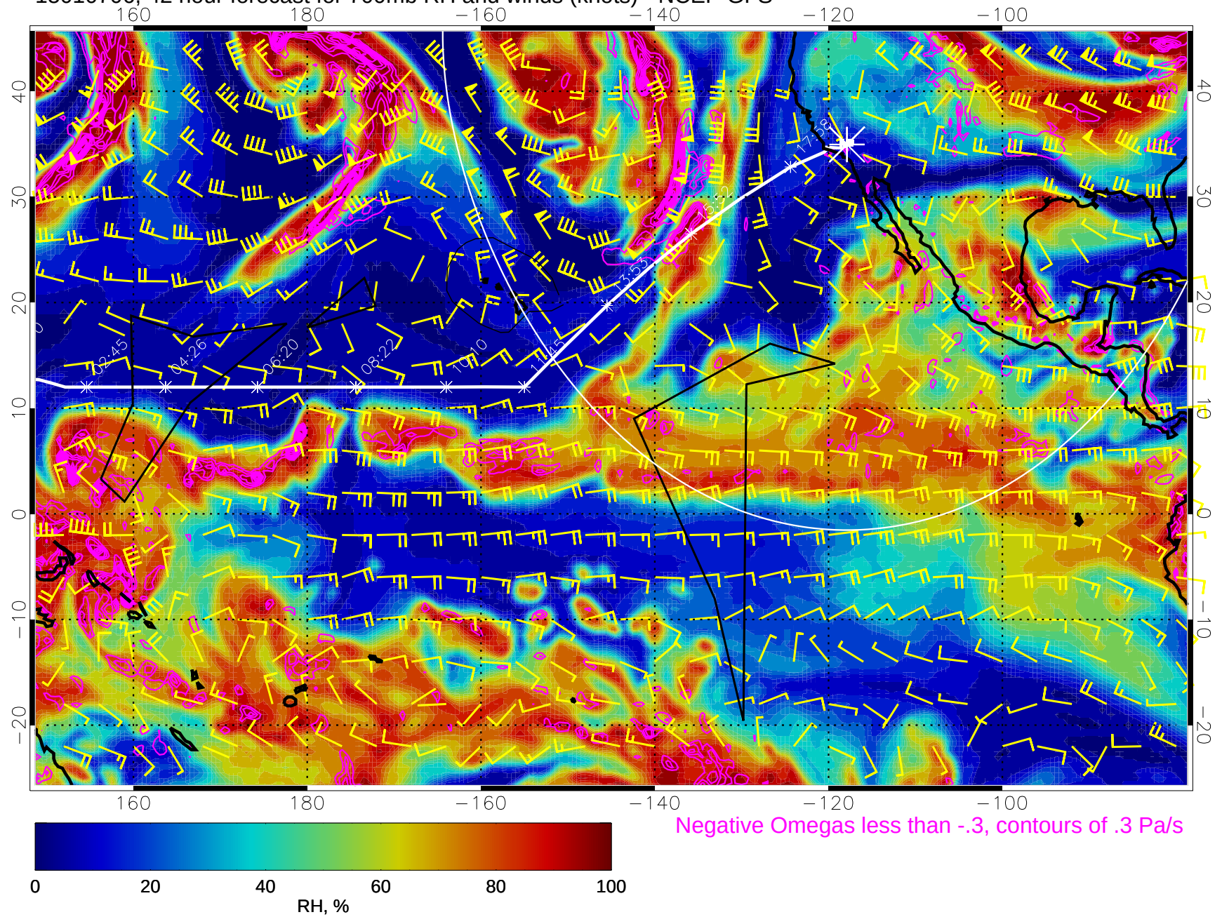
15010706, 42 hour forecast for 700mb RH and winds (knots) - NCEP GFS
